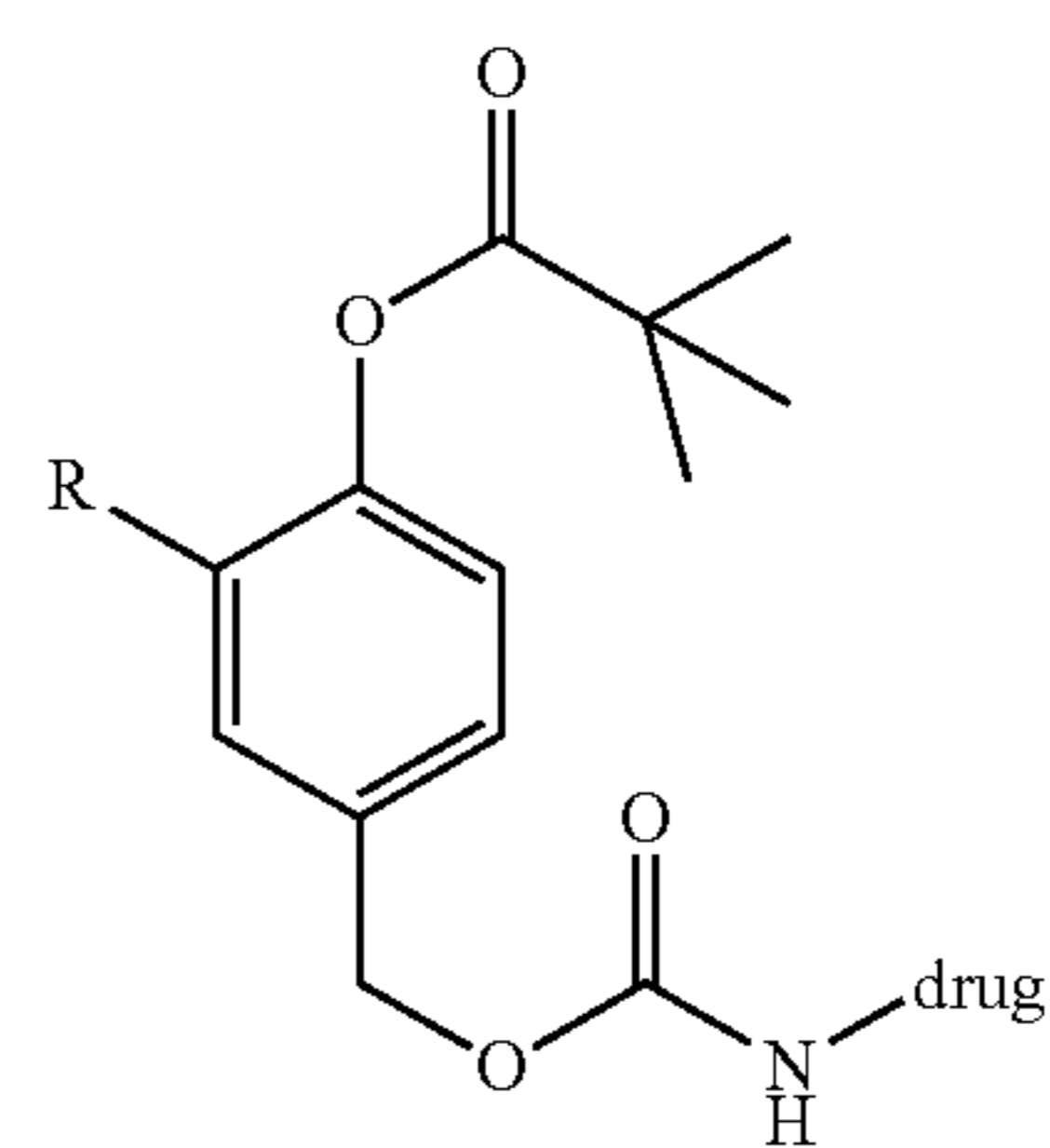
Scheme 2: X = O, N, S
