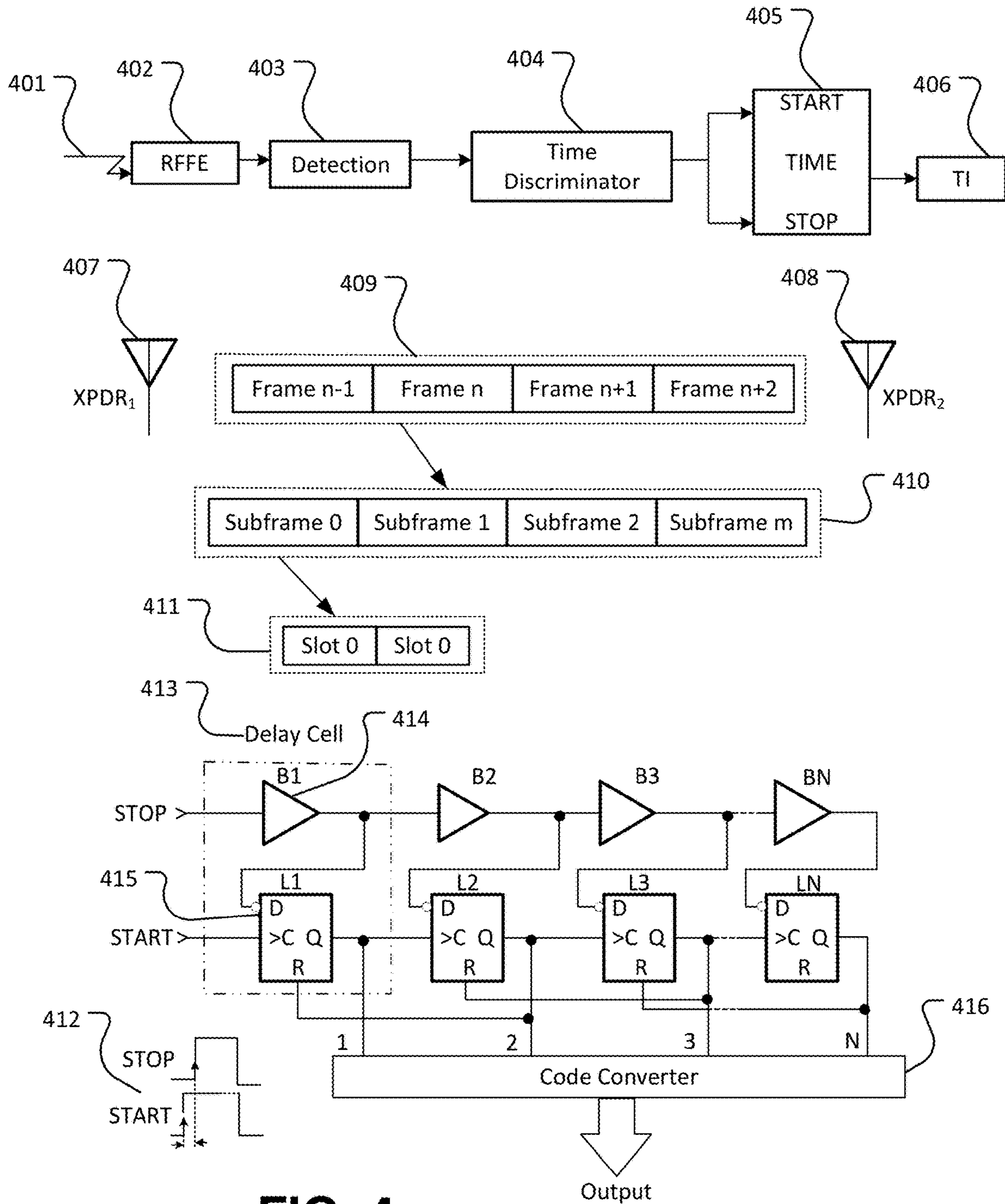
FIG. 4 (PRIOR ART)
