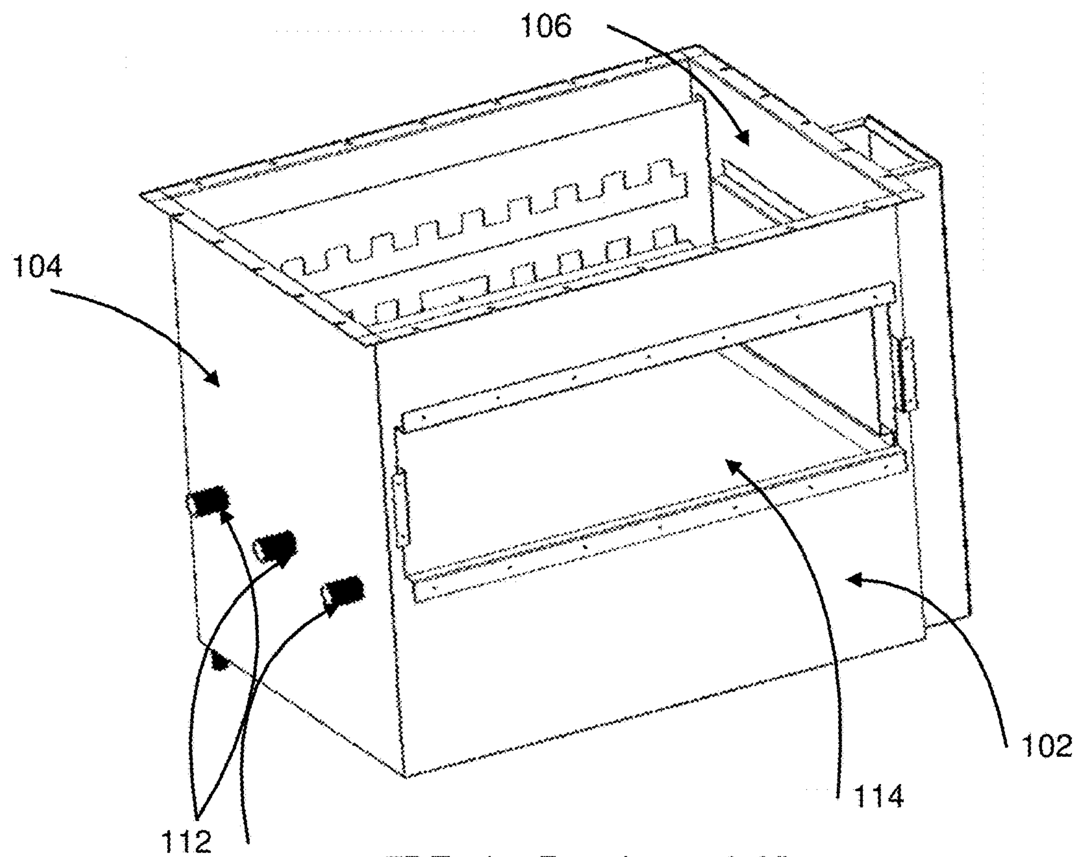
FIGURE 7B Tank – Front Isometric View
