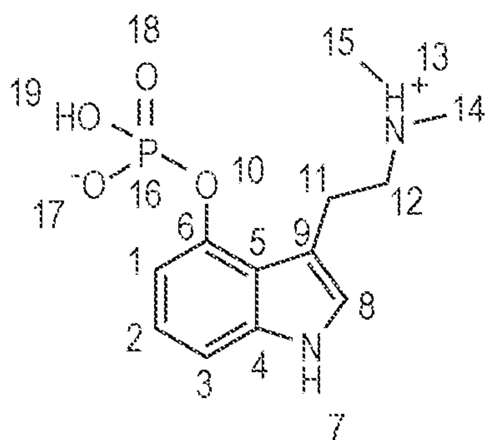
Psilocybin C_{12}H_{17}N_2O_4P Exact Mass: 284.09 Mol. Wt.: 284.25
