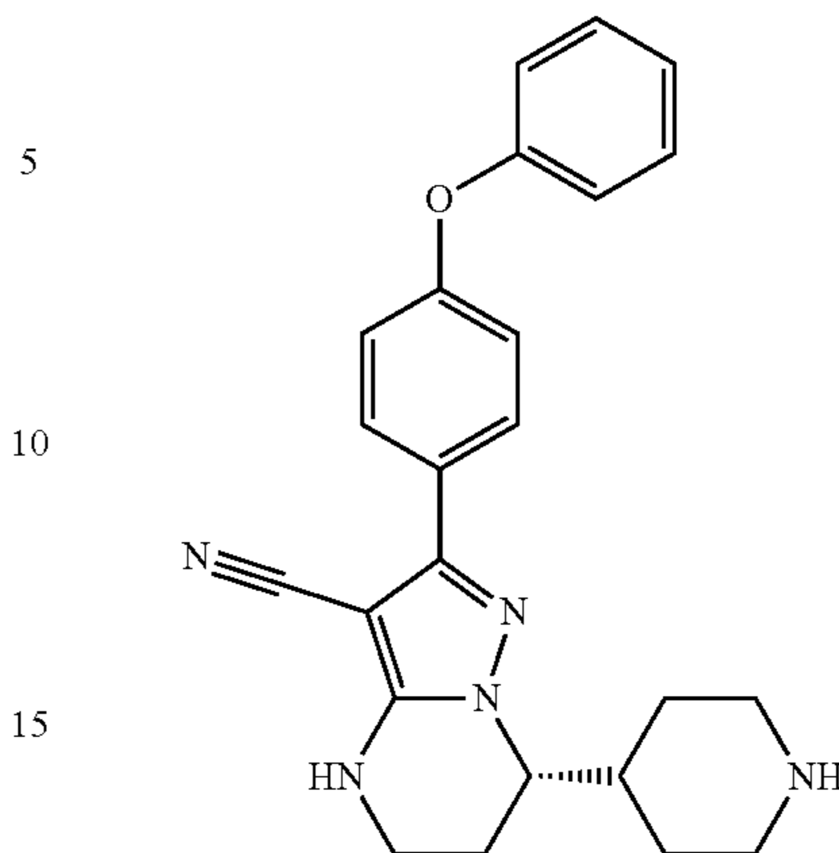
Compound 1
