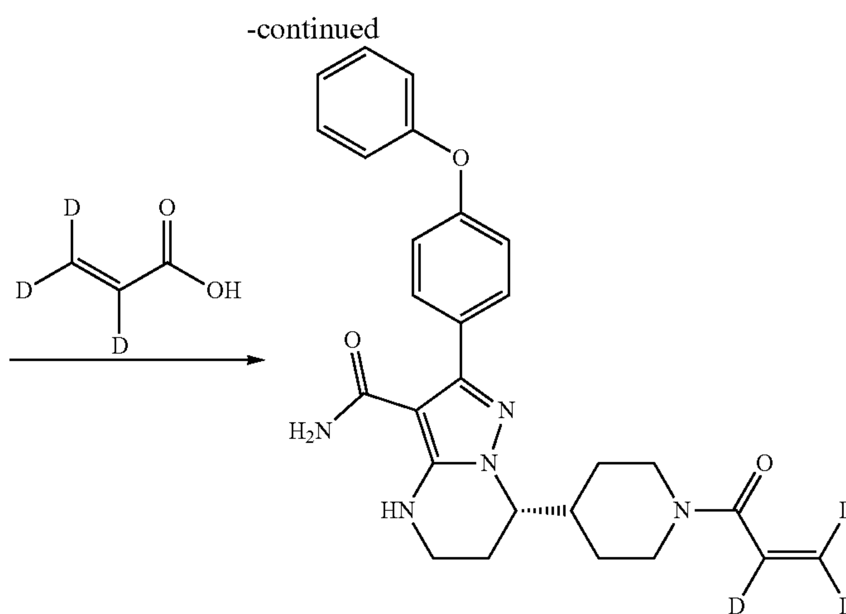
Deuterium-Labeled Compound 1
