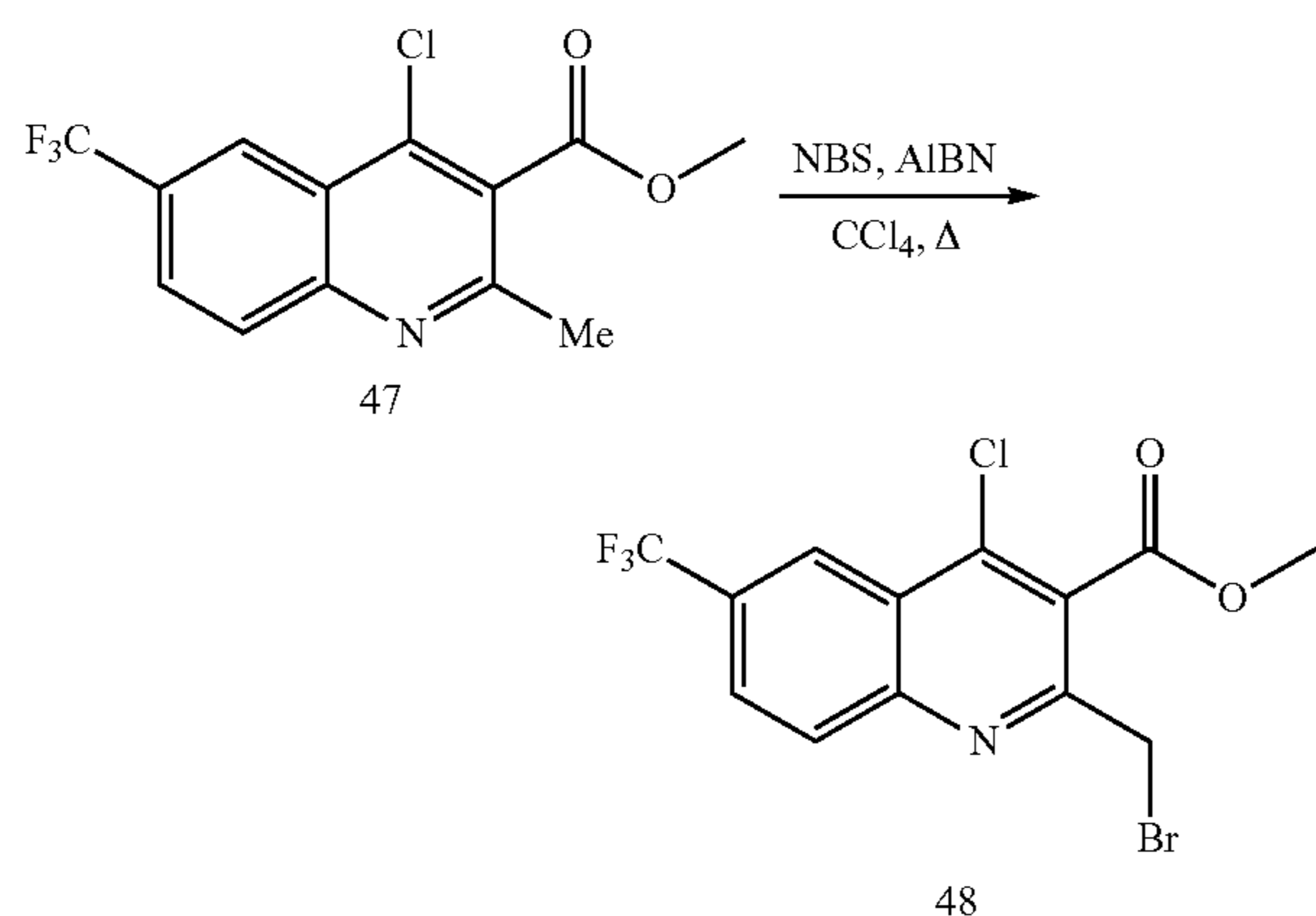
Methyl 2-(bromomethyl)-4-chloro-6-(trifluoromethyl)quinoline-3-carboxylate 48
