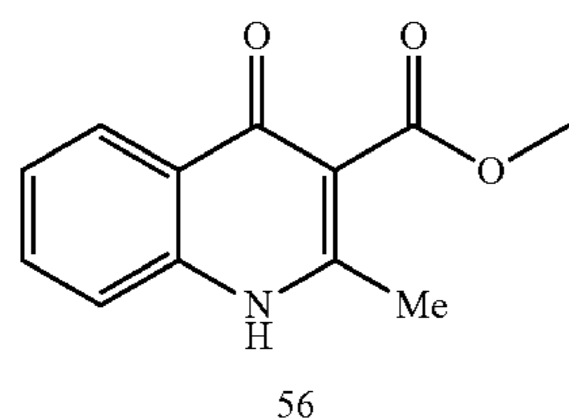
Methyl 2-methyl-4-oxo-1,4-dihydroquinoline-3-carboxylate 56
