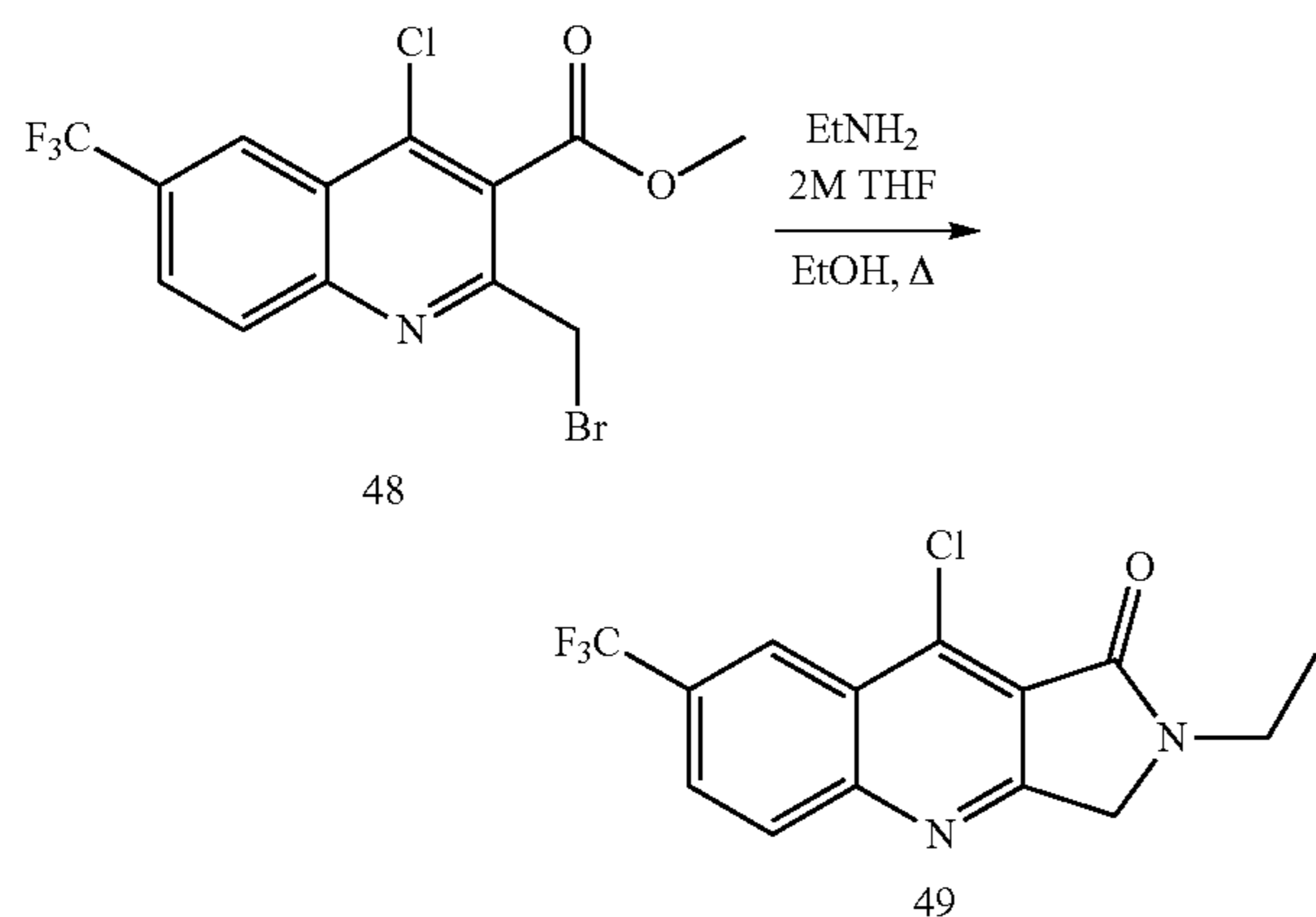
9-chloro-2-ethyl-7-(trifluoromethyl)-2,3-dihydro-1H-pyrrolo[3,4-b]quinolin-1-one 49
