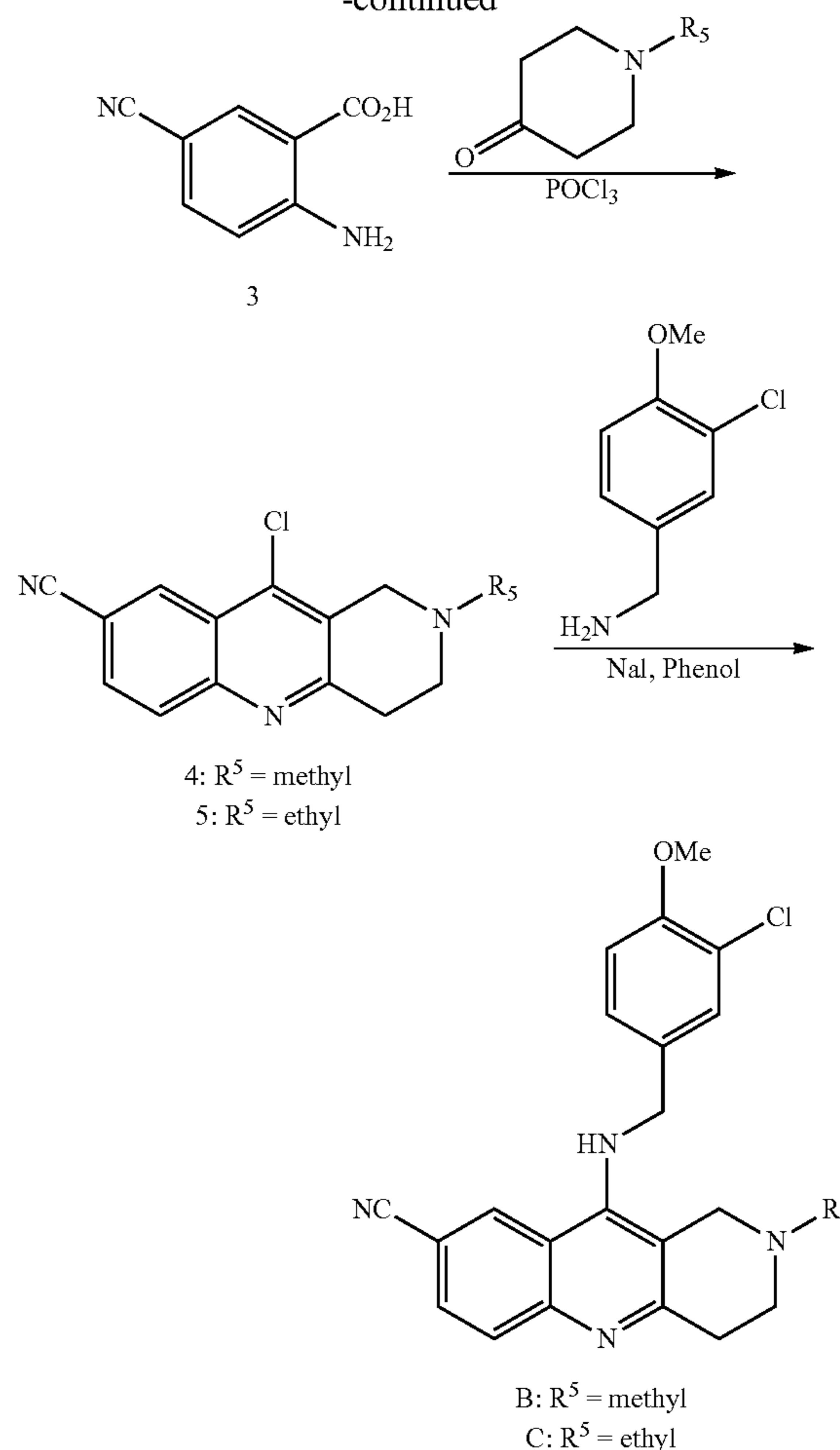
2-amino-5-cyanobenzoic Acid, 3
