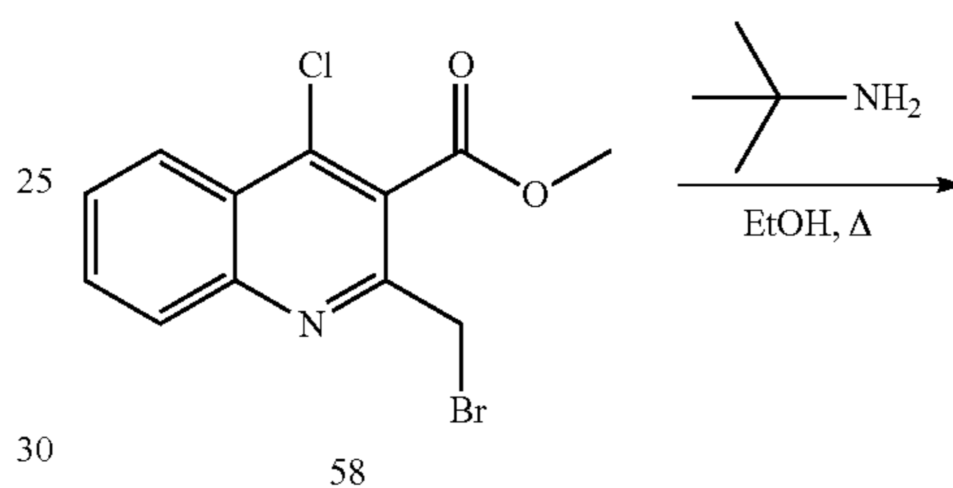
9-chloro-2-ethyl-2,3-dihydro-1H-pyrrolo[3,4-b]quinolin-1-one 59
