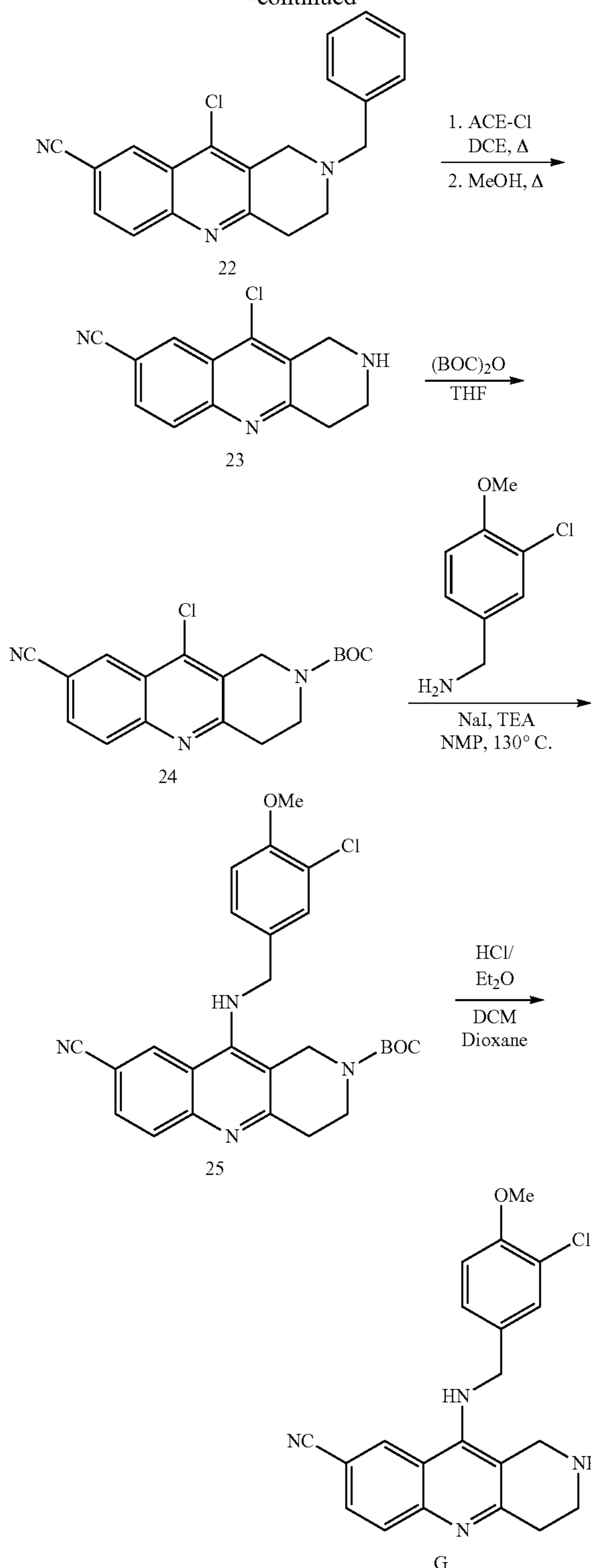
2-benzyl-10-chloro-1,2,3,4-tetrahydrobenzo[b][1,6] naphthyridine-8-carbonitrile, 22
