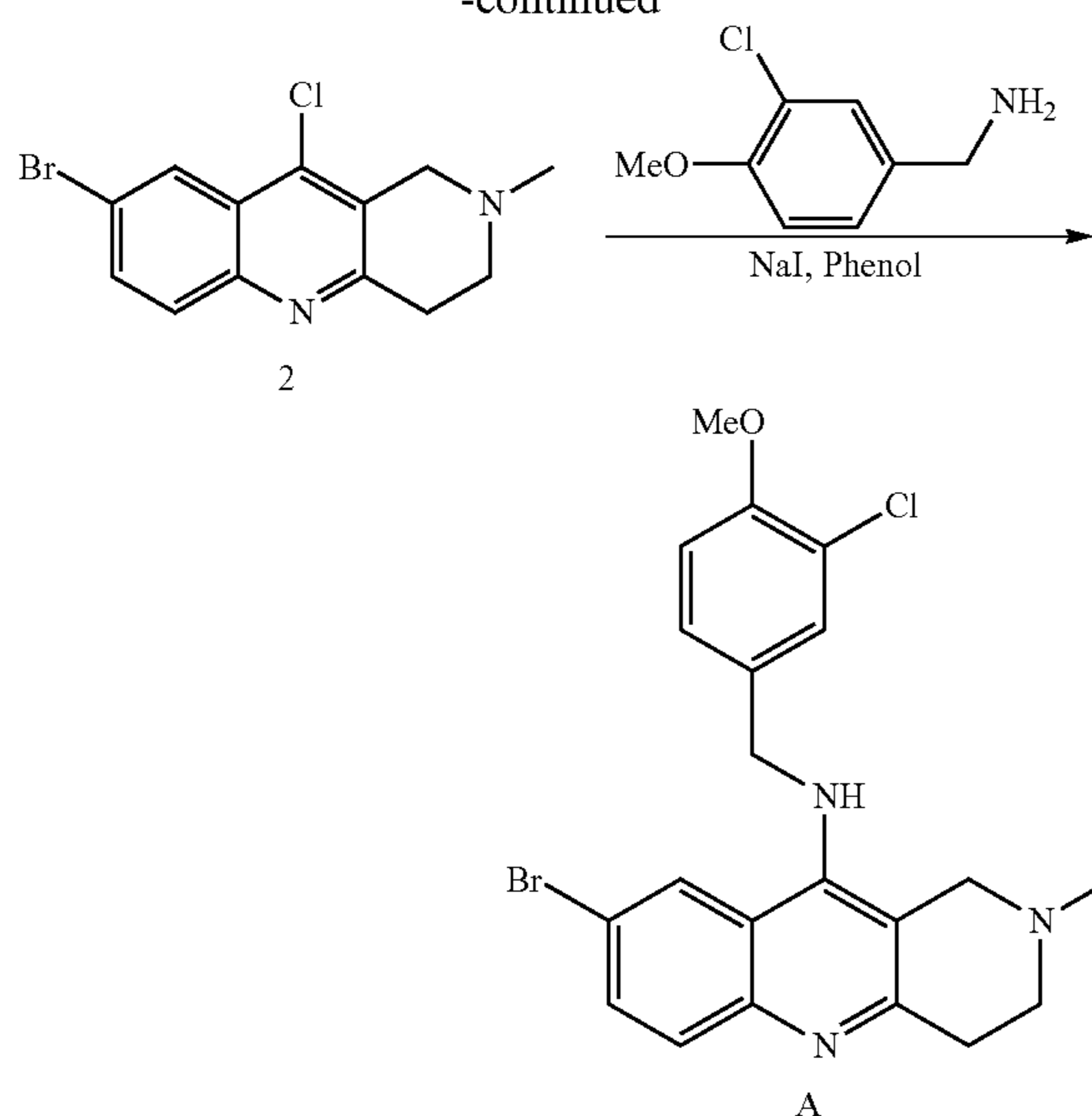
8-bromo-10-chloro-2-methyl-1,2,3,4-tetrahydrobenzo[b][1,6]naphthyridine, 2
