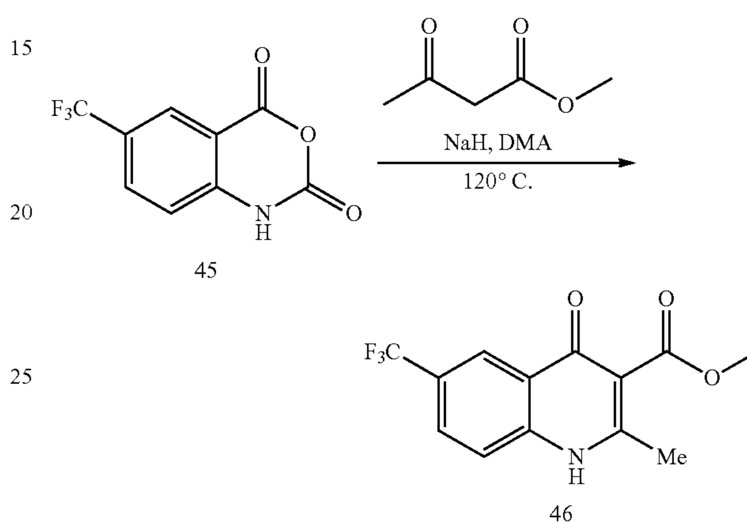
Methyl 2-methyl-4-oxo-6-(trifluoromethyl)-1,4-dihydroquinoline-3-carboxylate 46
