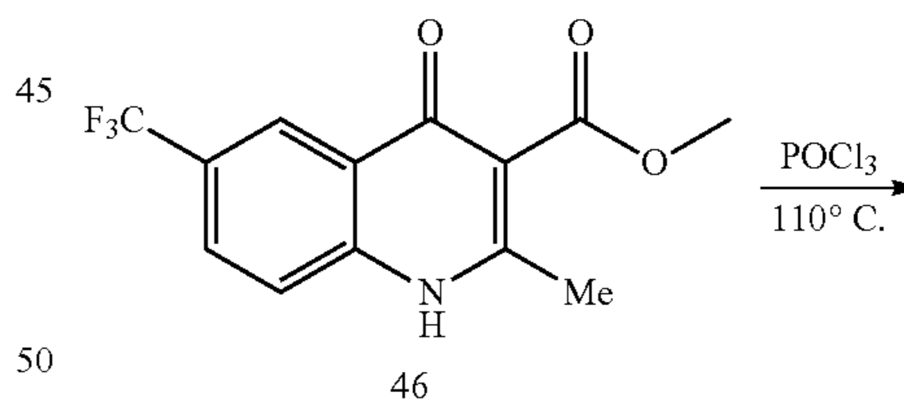
Example 19: 9-[(3-chloro-4-methoxybenzyl)amino]-2-ethyl-7-(trifluoromethyl)-2,3-dihydro-1H-pyrrolo[3,4-b]quinolin-1-one
