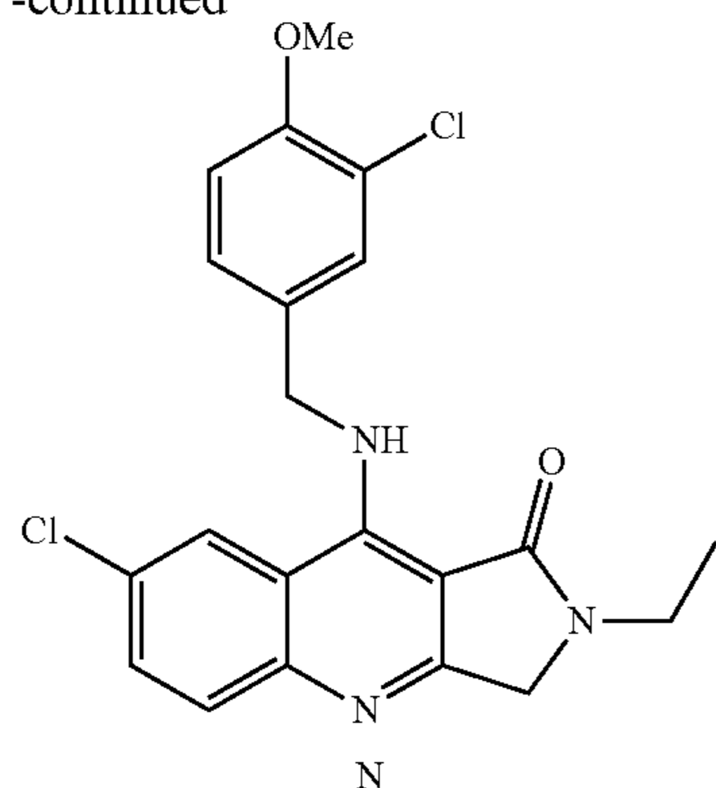
7-chloro-9-[(3-chloro-4-methoxybenzyl)amino]-2-ethyl-2,3-dihydro-1H-pyrrolo[3,4-b]quinolin-1-one N
