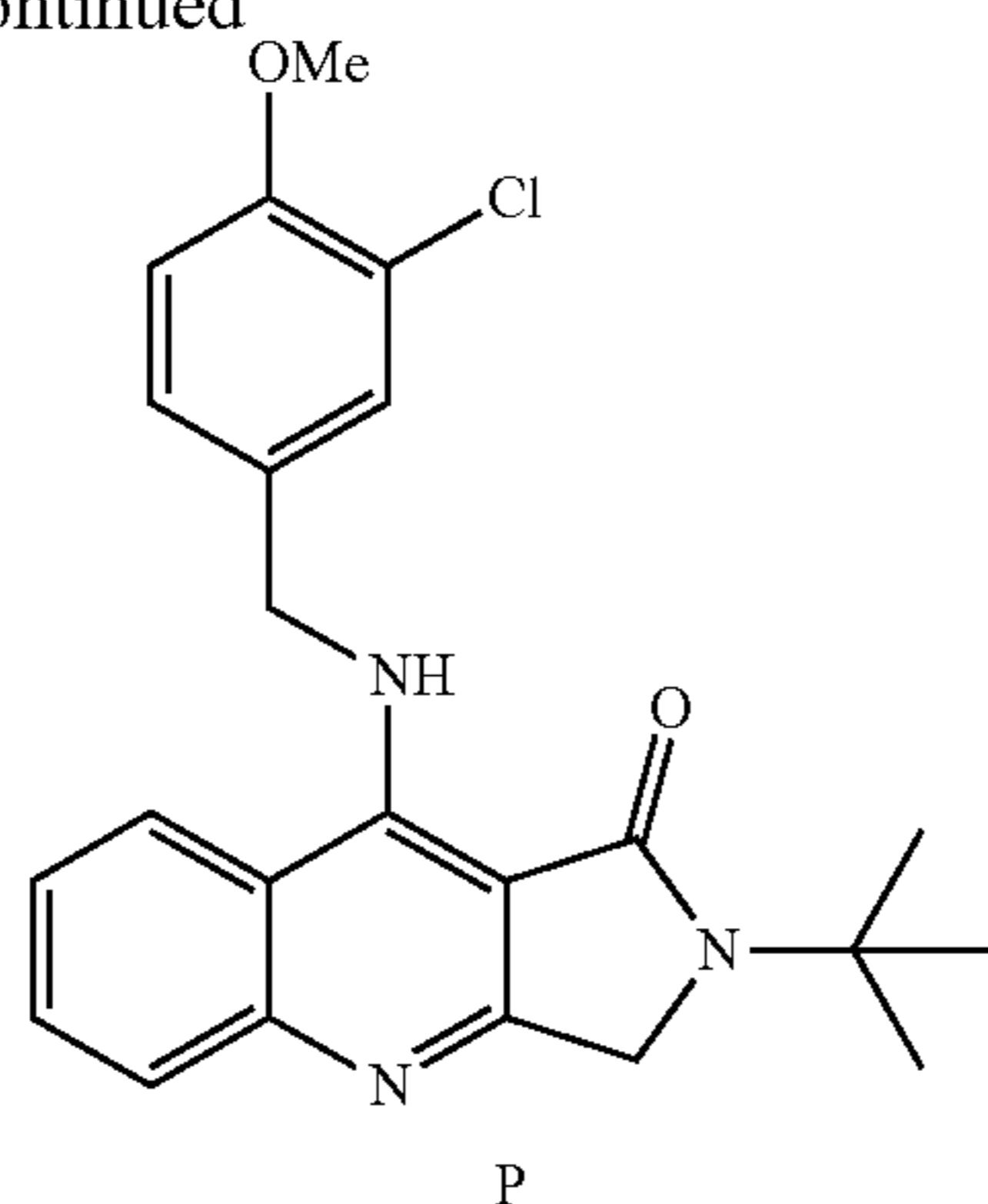
2-(tert-butyl)-9-[(3-chloro-4-methoxybenzyl)amino]-2,3-dihydro-1H-pyrrolo[3,4-b]quinolin-1-one P
