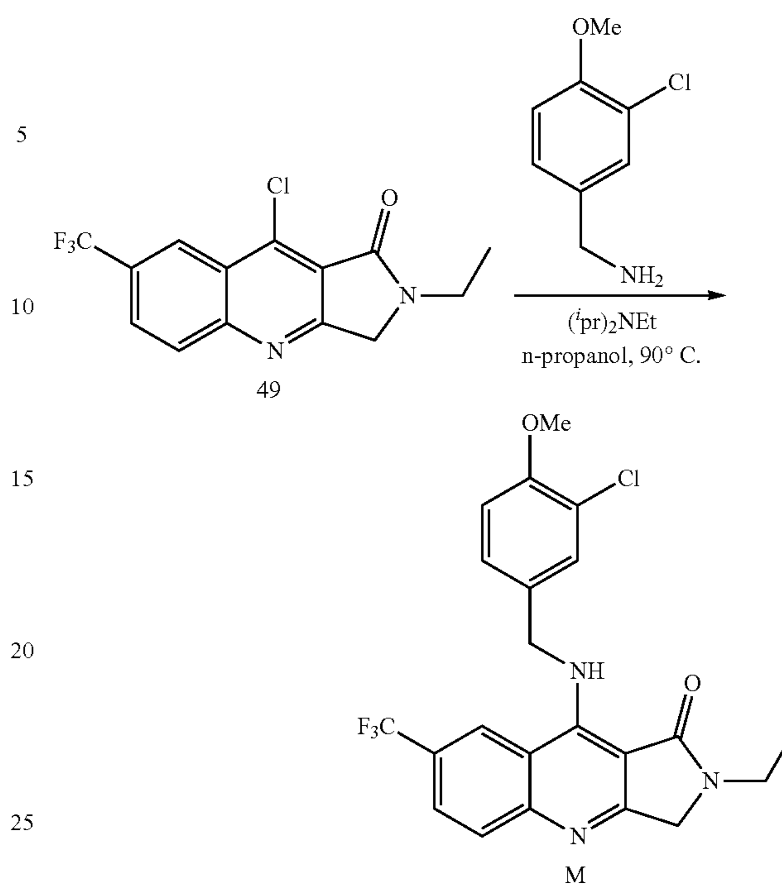
9-[(3-chloro-4-methoxybenzyl)amino]-2-ethyl-7-(trifluoromethyl)-2,3-dihydro-1H-pyrrolo[3,4-b]quinolin-1-one M
