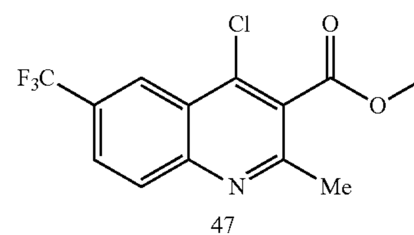
Methyl 4-chloro-2-methyl-6-(trifluoromethyl)quinoline-3-carboxylate 47
