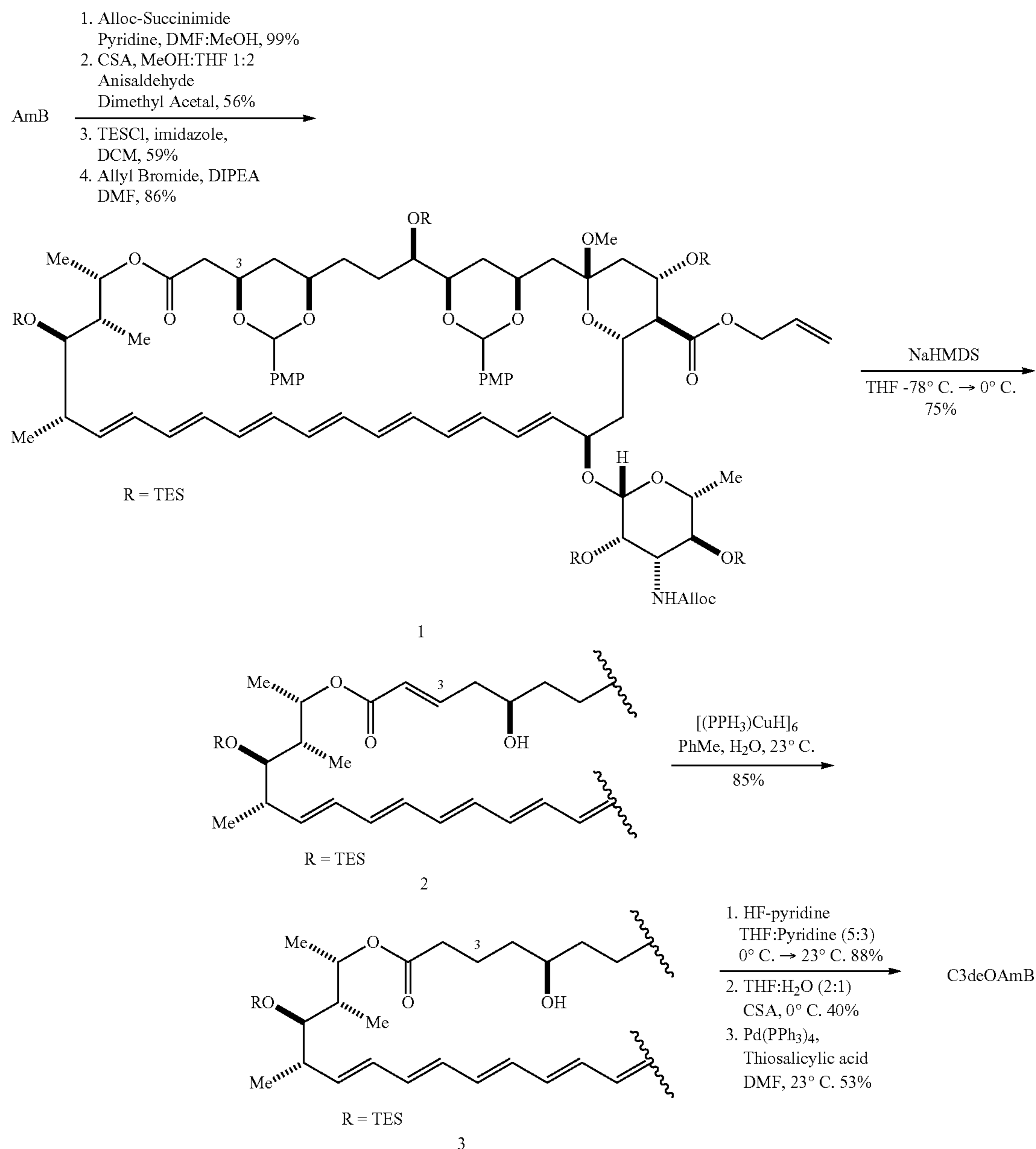
Scheme 1: Synthesis of C3deOAmB
