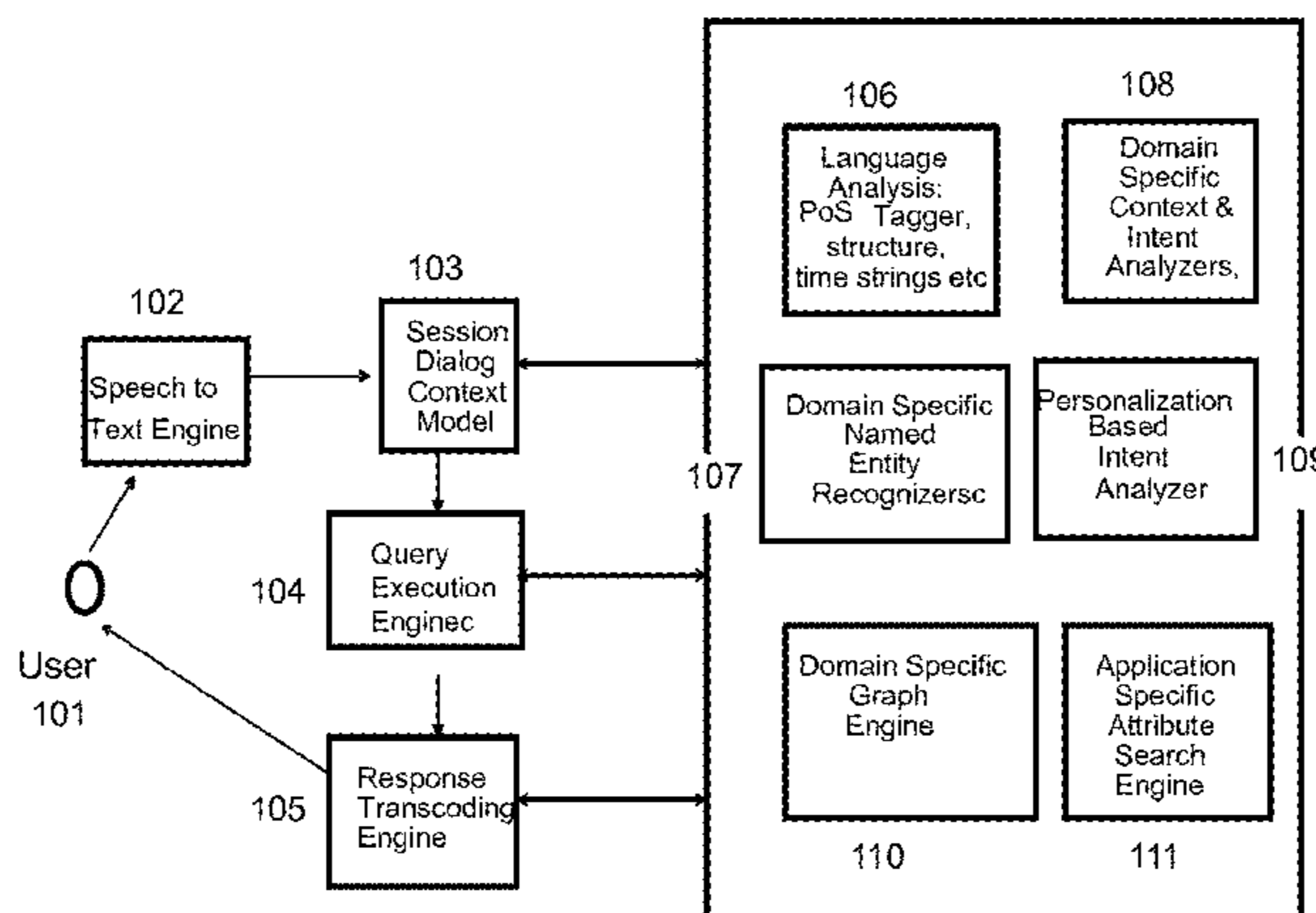
Conversation Interaction Architecture
