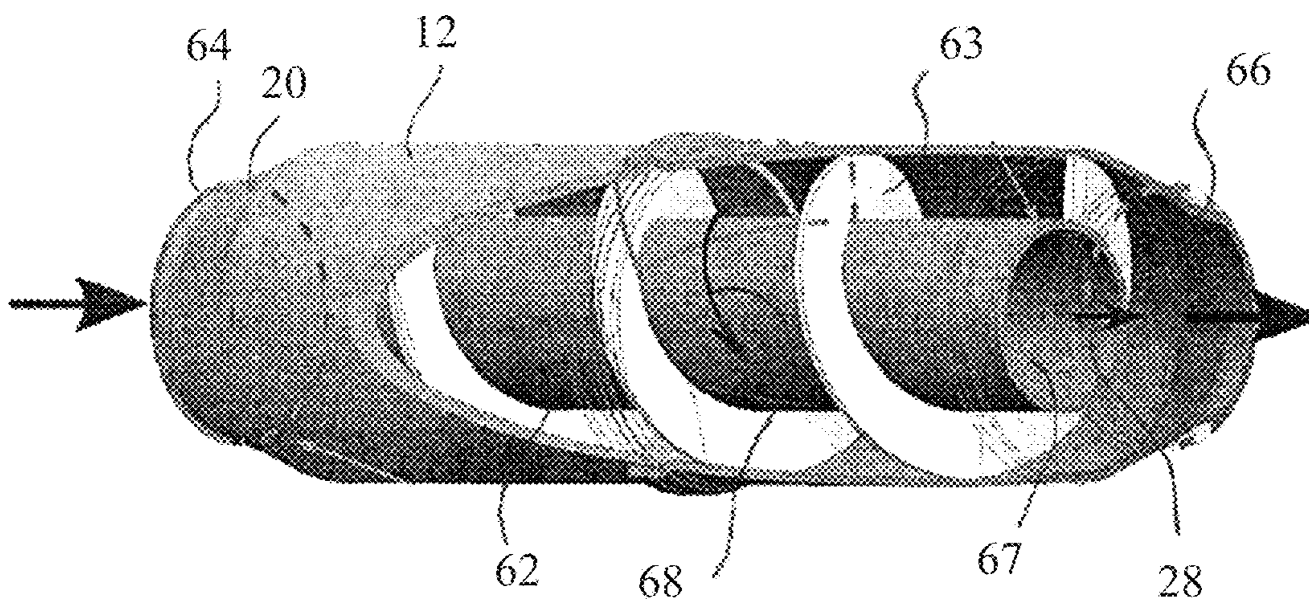
Fig. 1C (Prior Art) US 9,500,108
