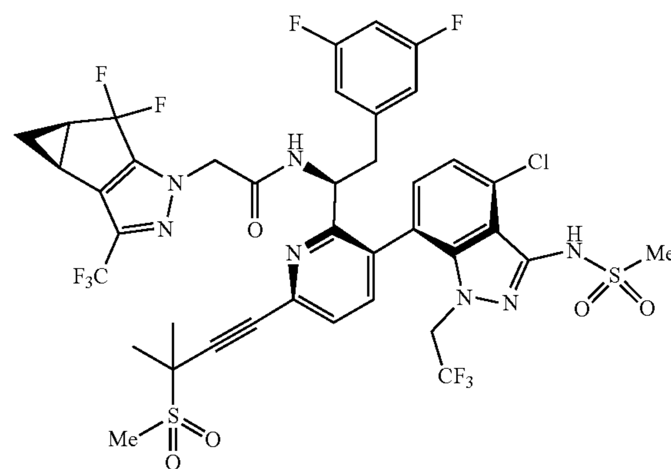
Isomer A
