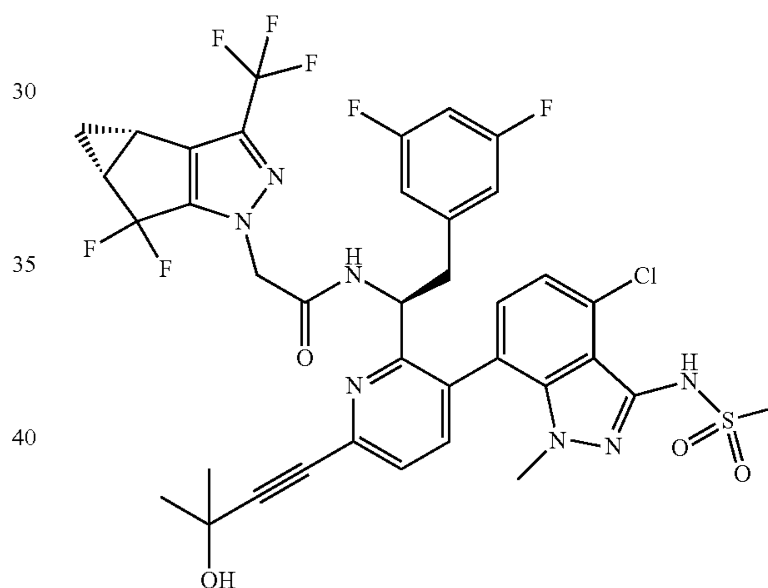
Compound B
