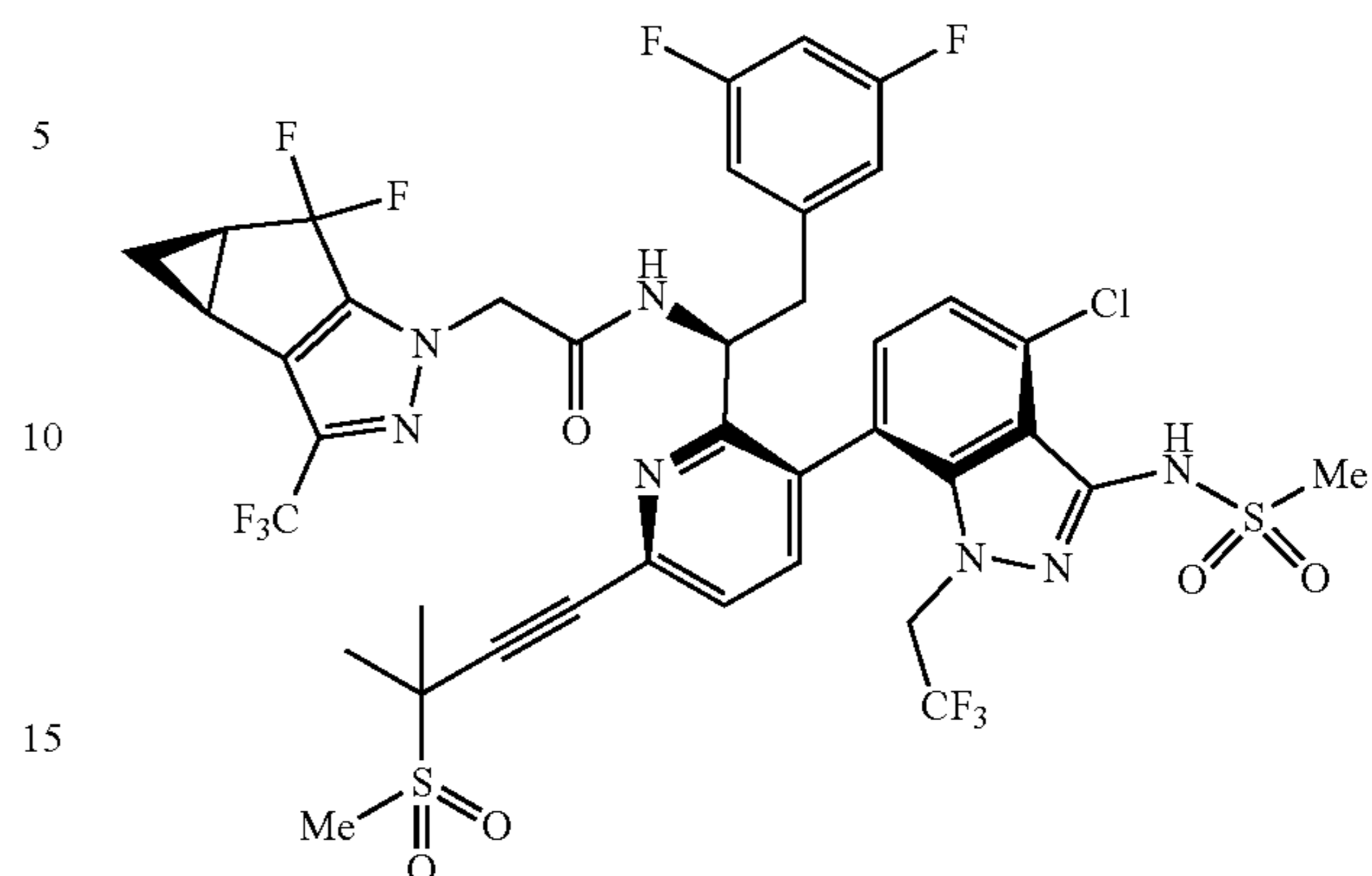
Isomer B
