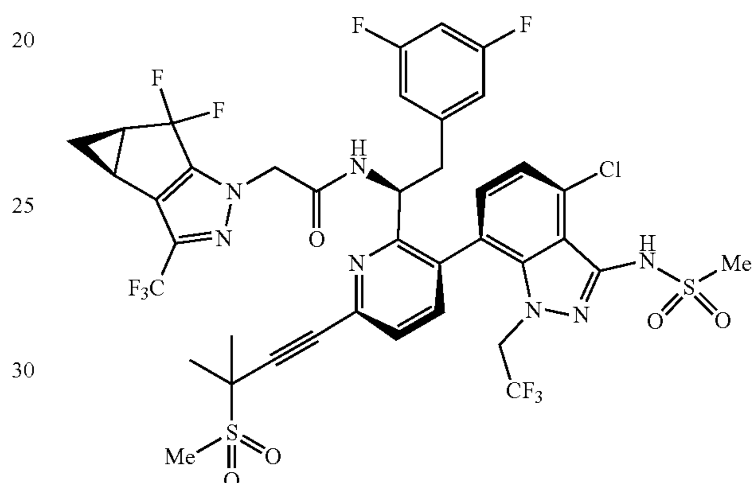
Isomer B
