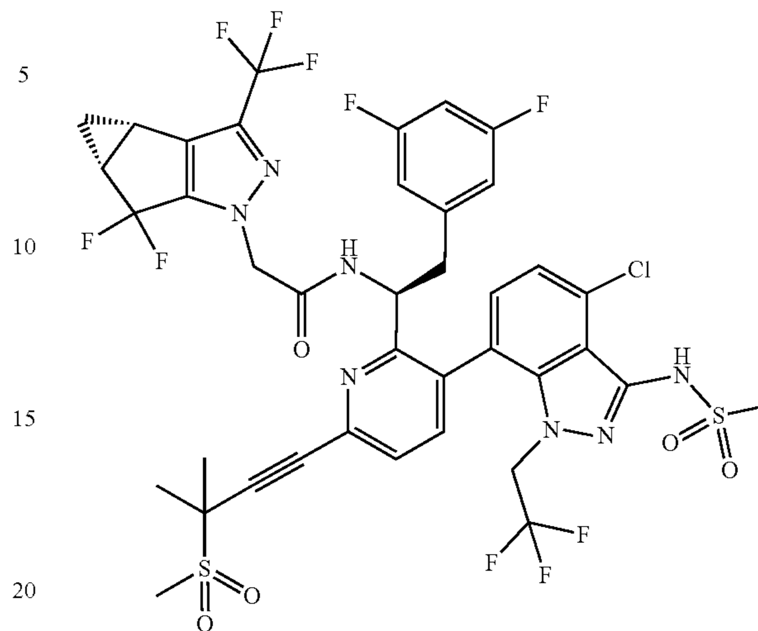
Compound 1
