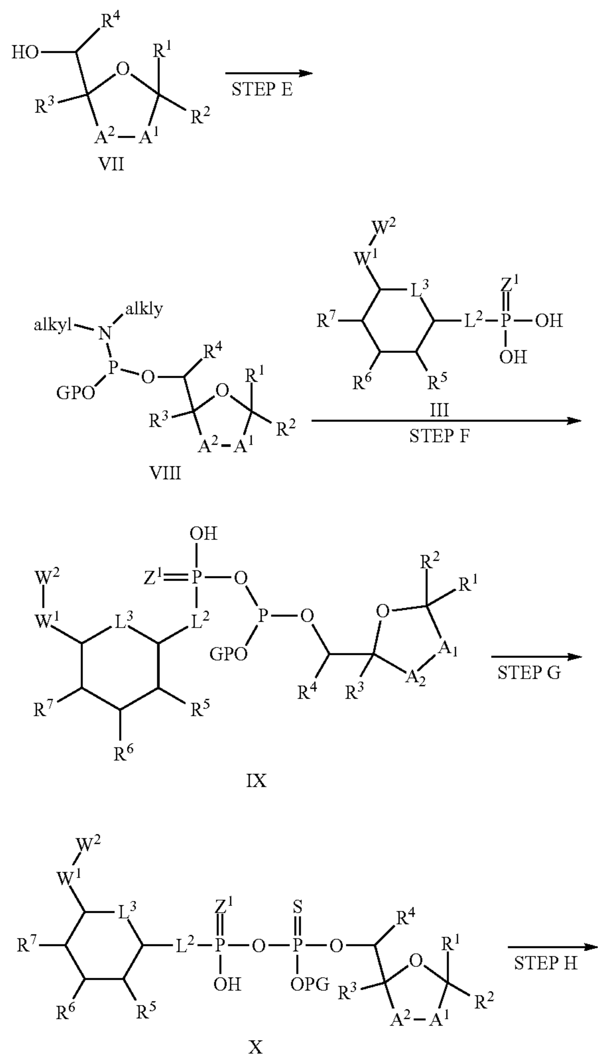
Scheme II
