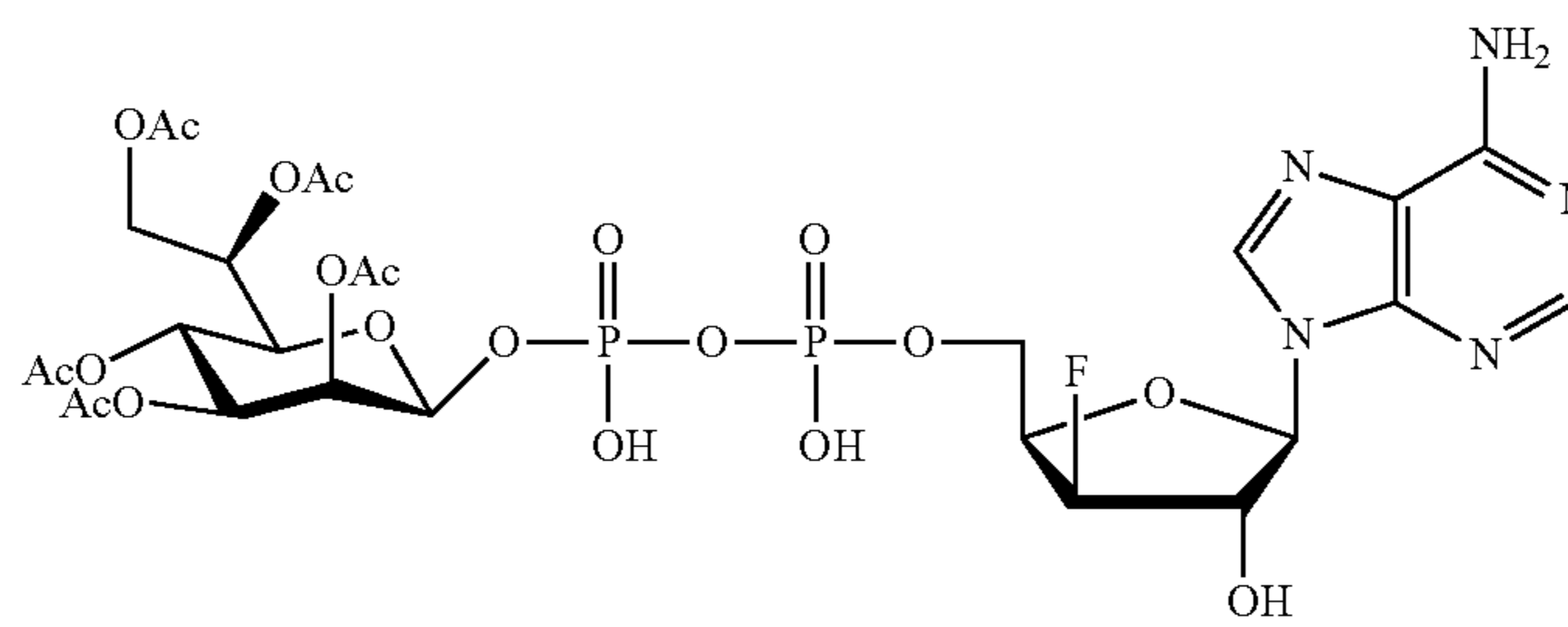
Compound 18
