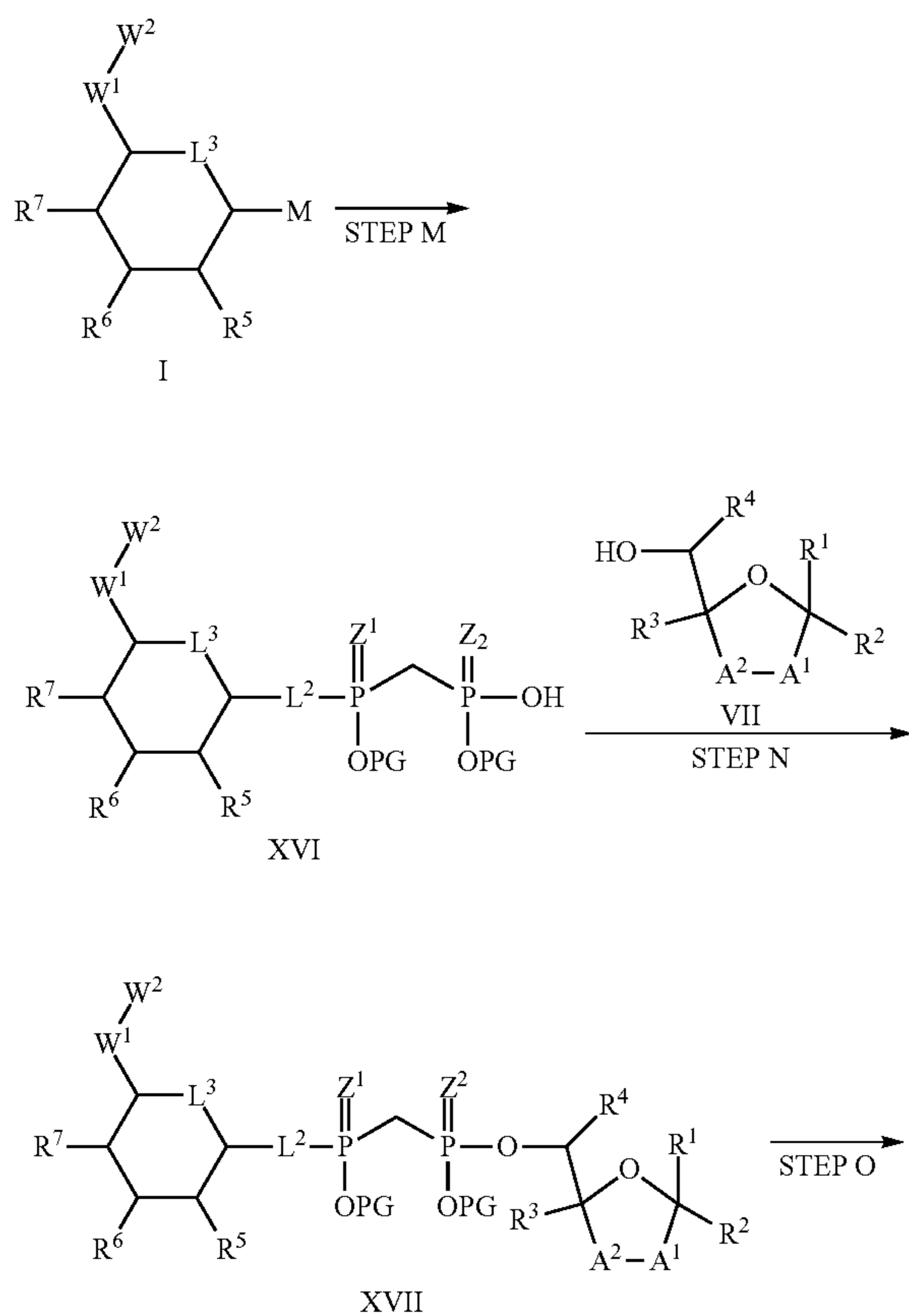
Scheme IV
