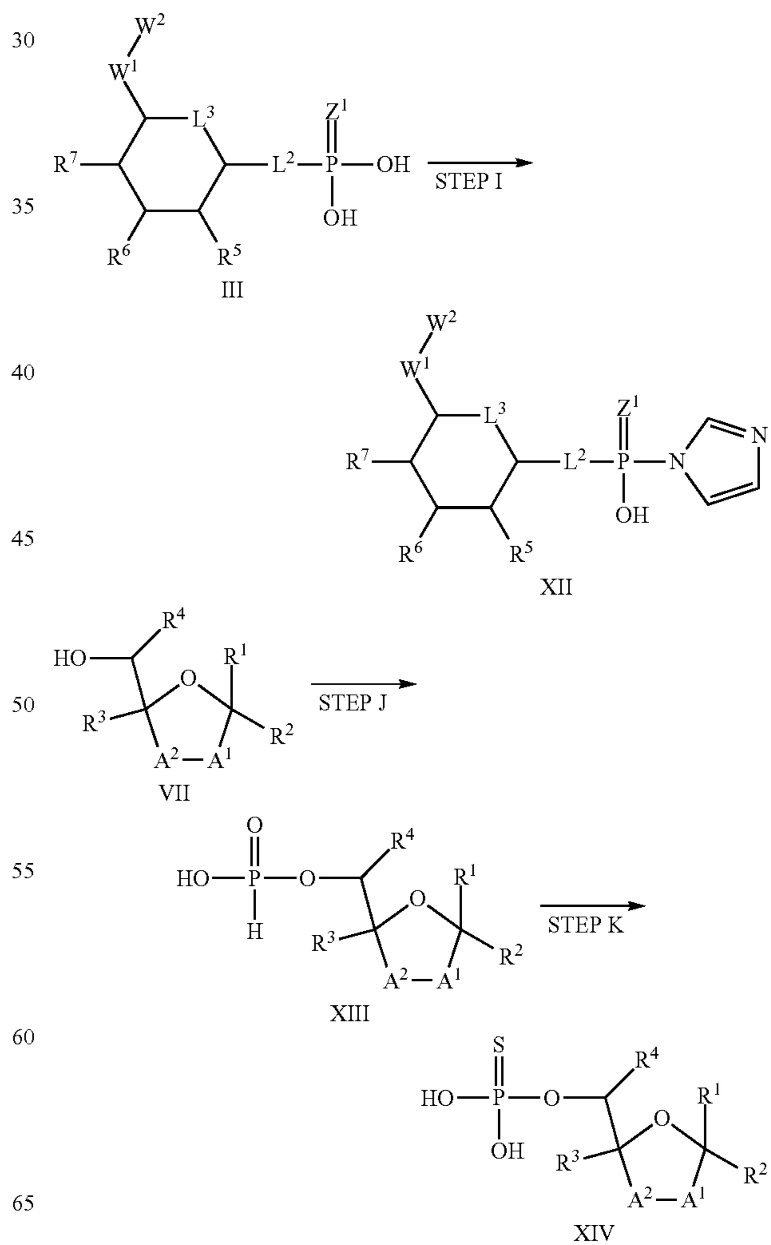
Scheme III
