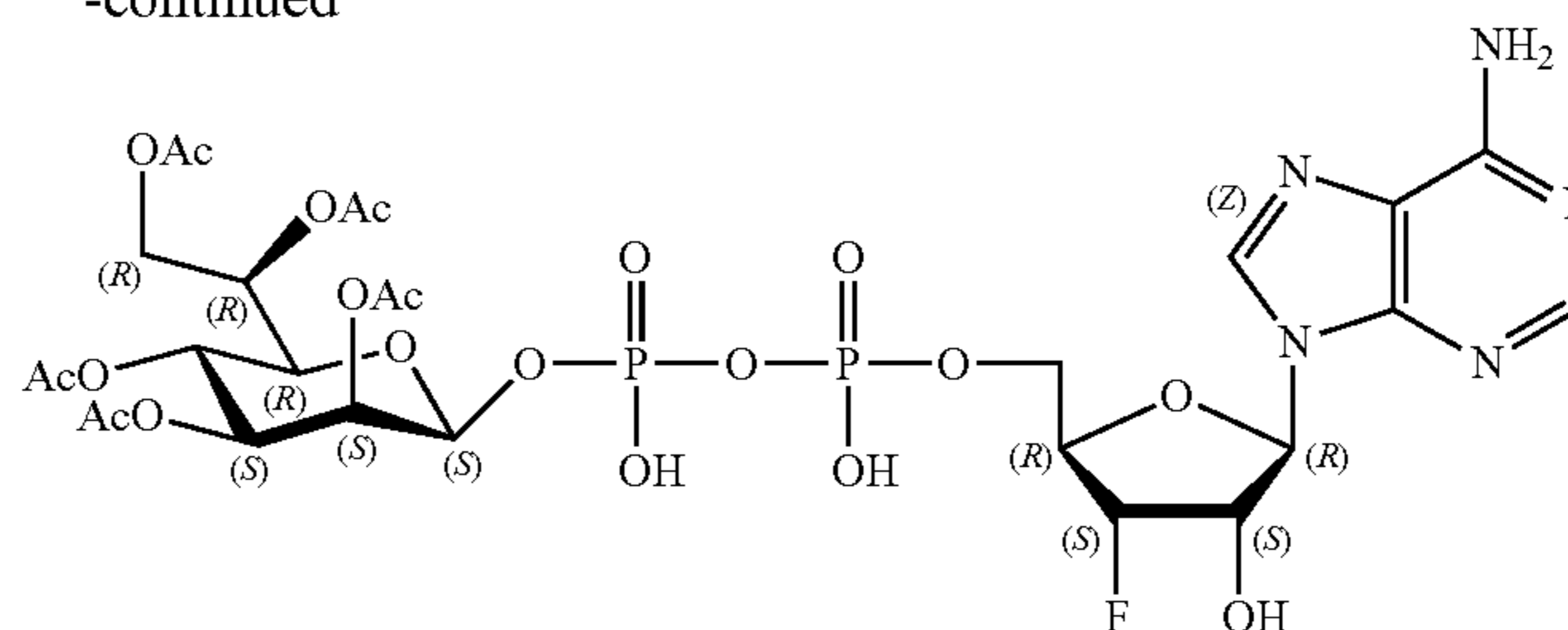
Compound 2
