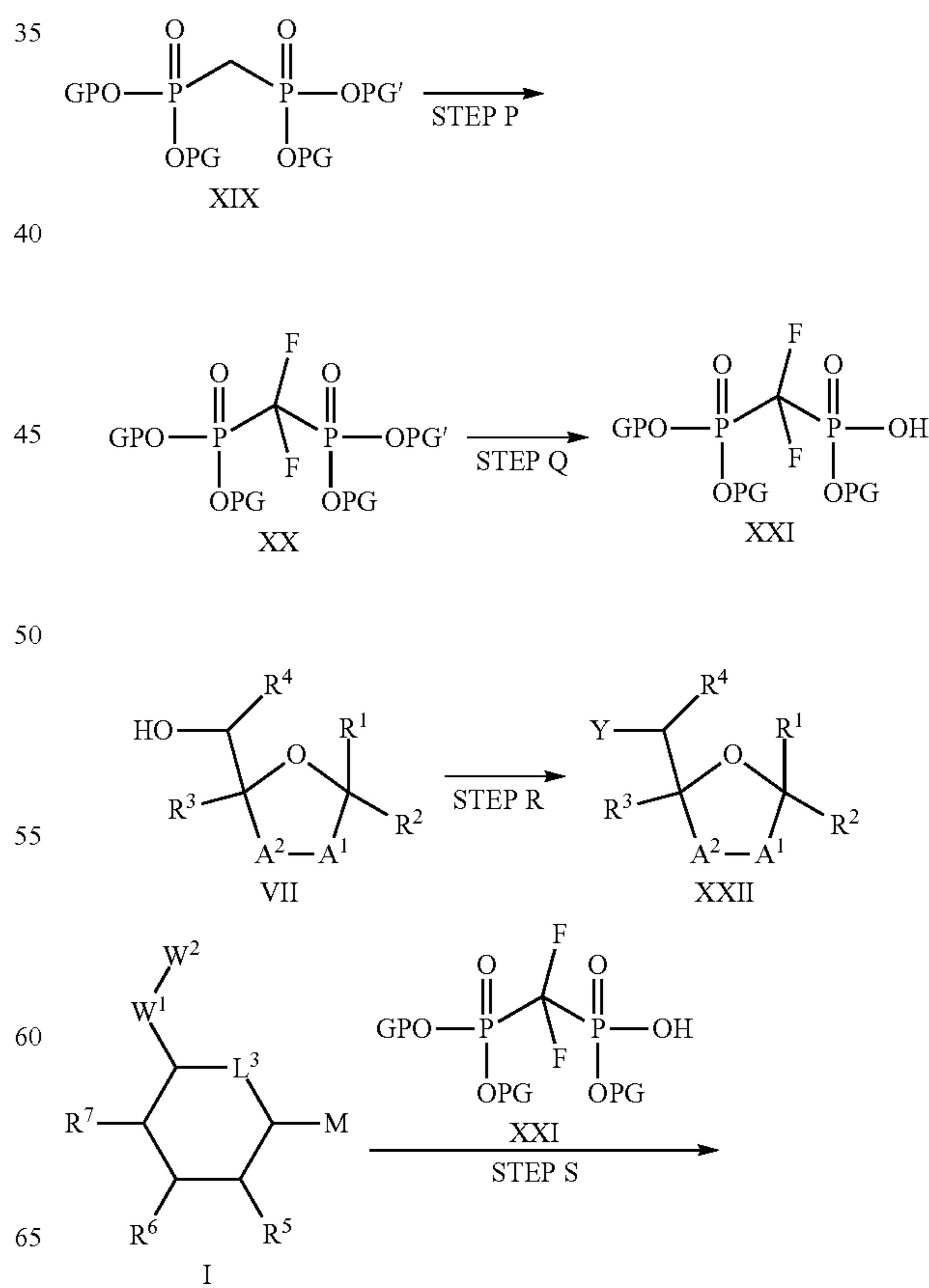
Scheme V
