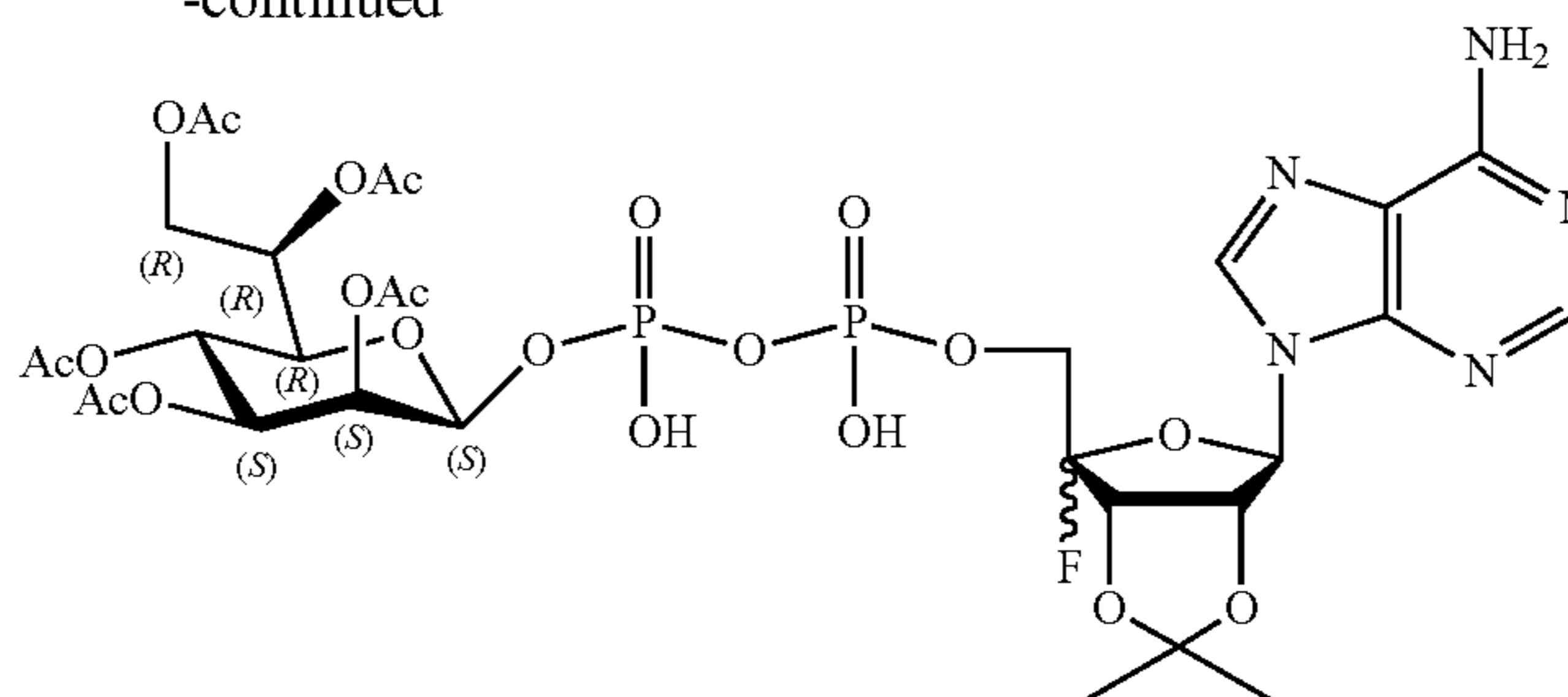
Compound 20
