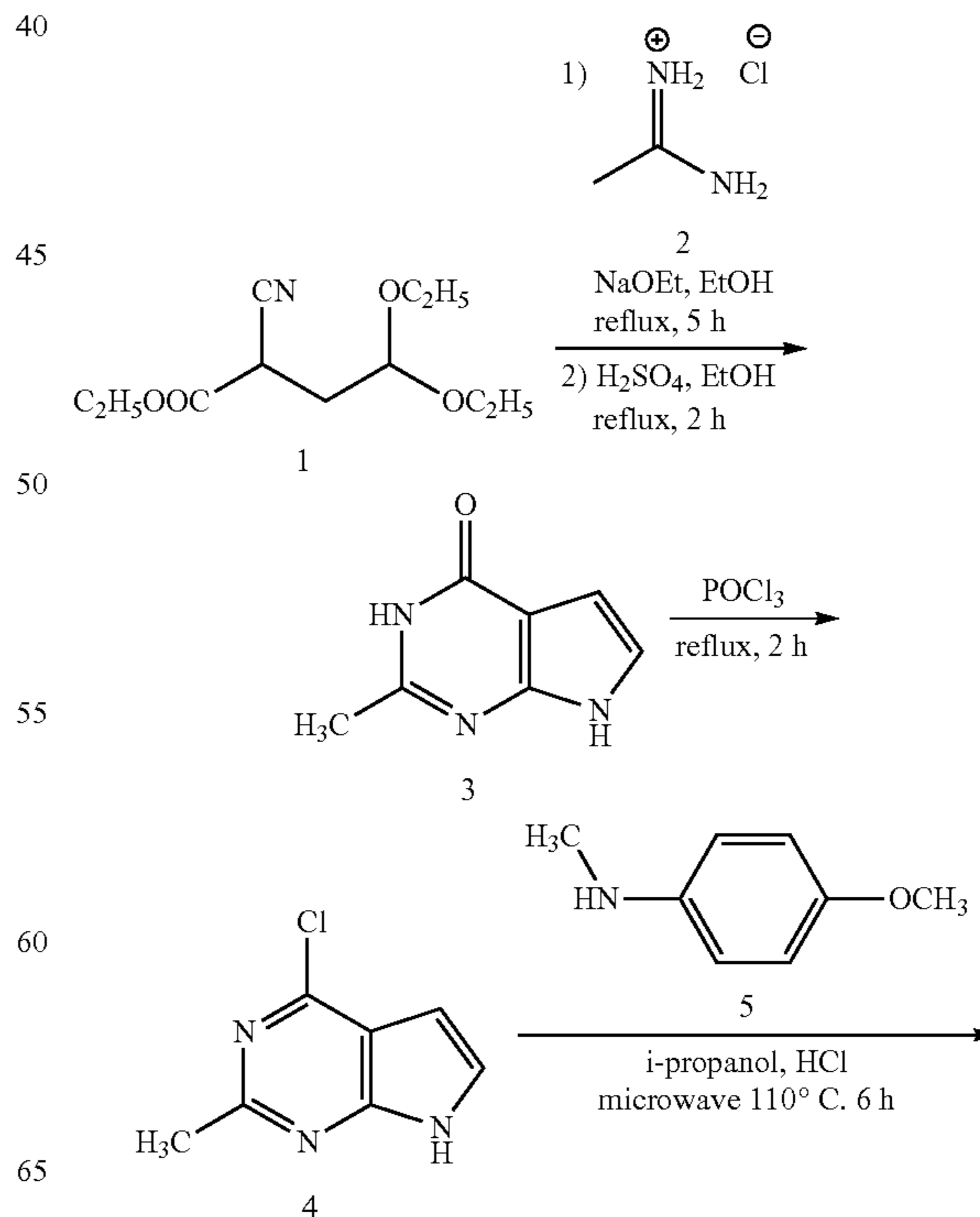
Scheme 5
