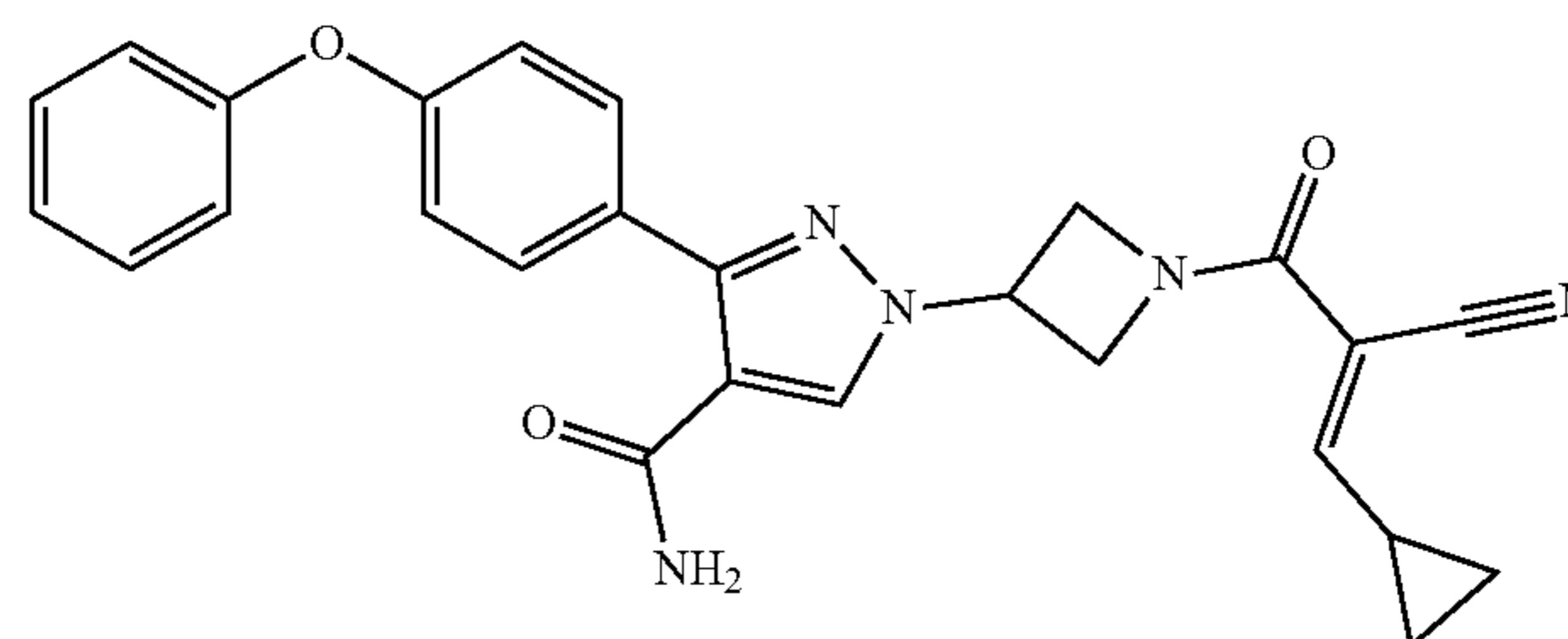
Example 53
