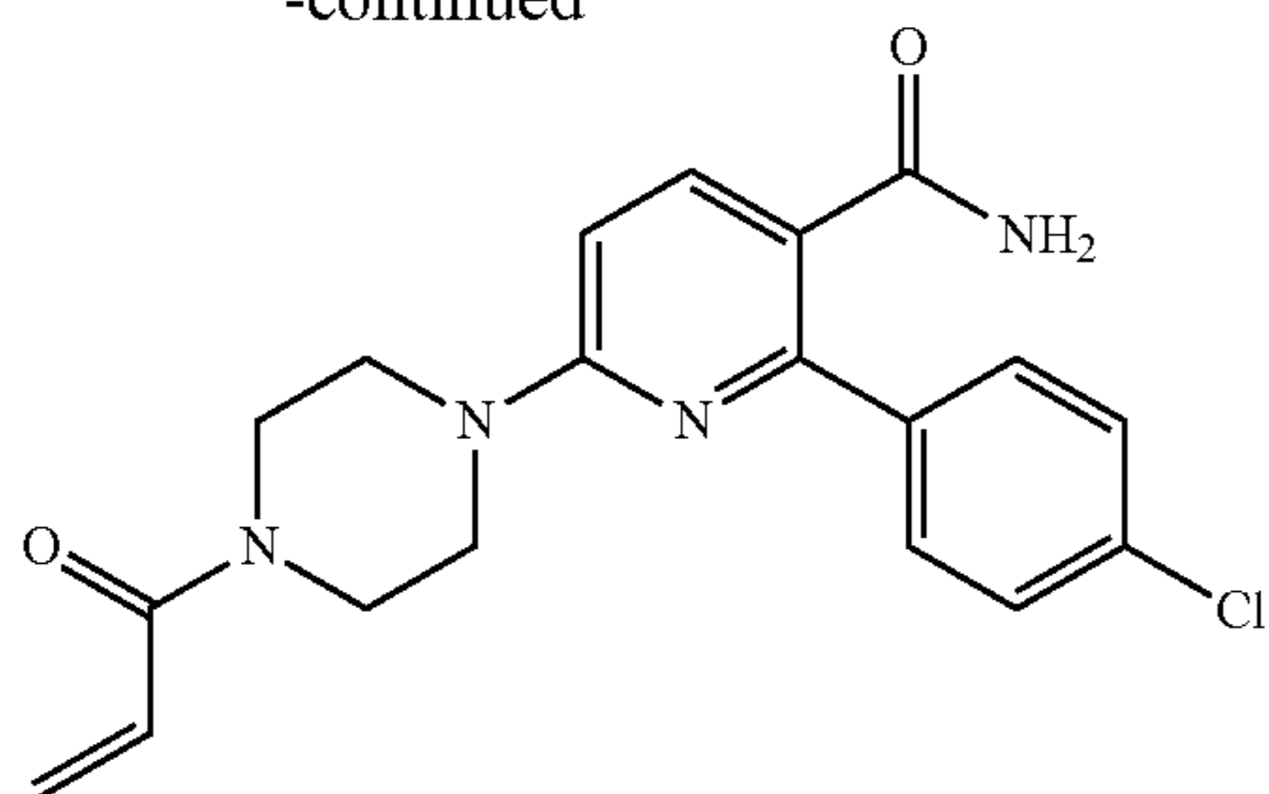
Example 33
