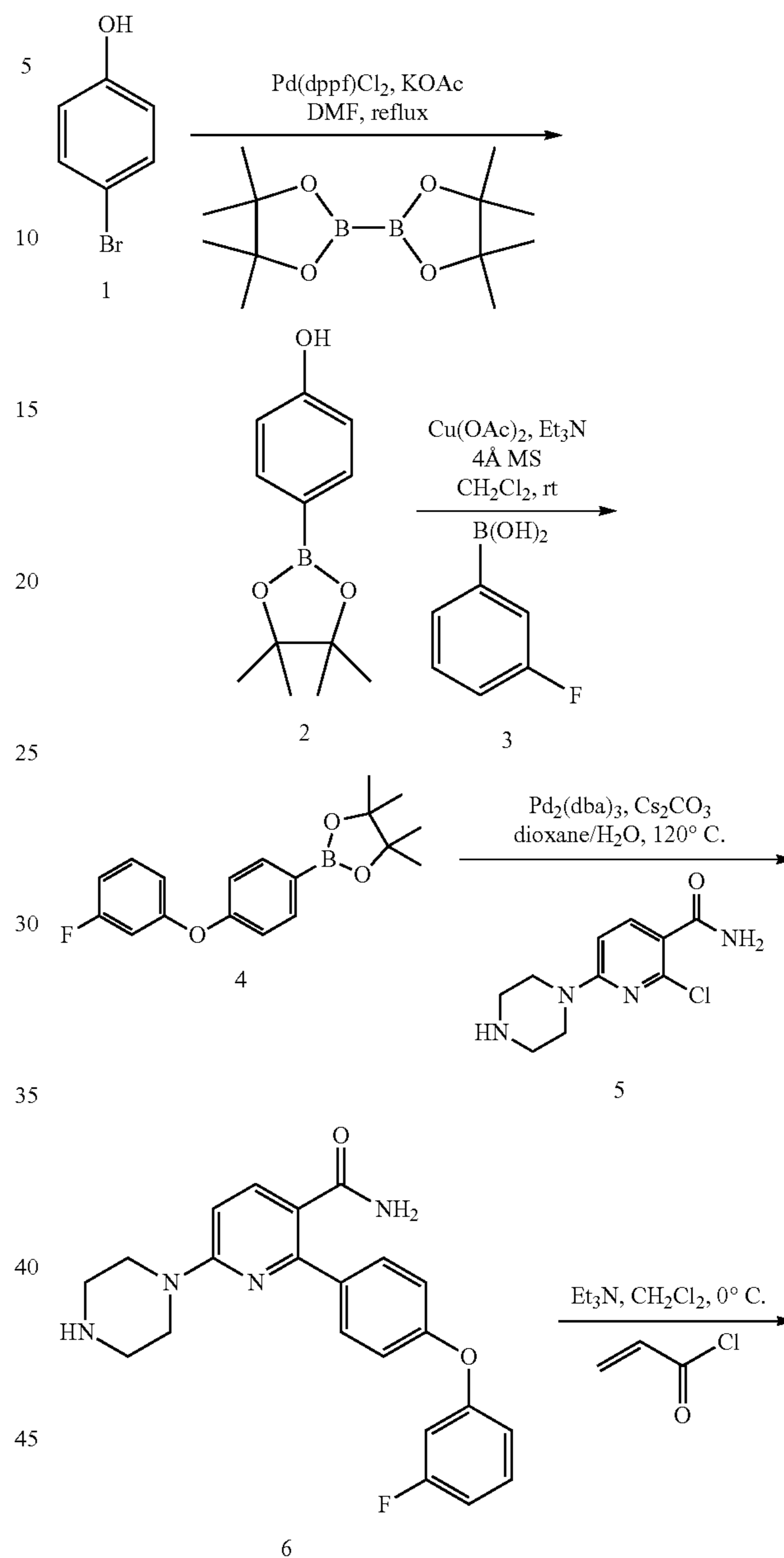
Scheme 25
