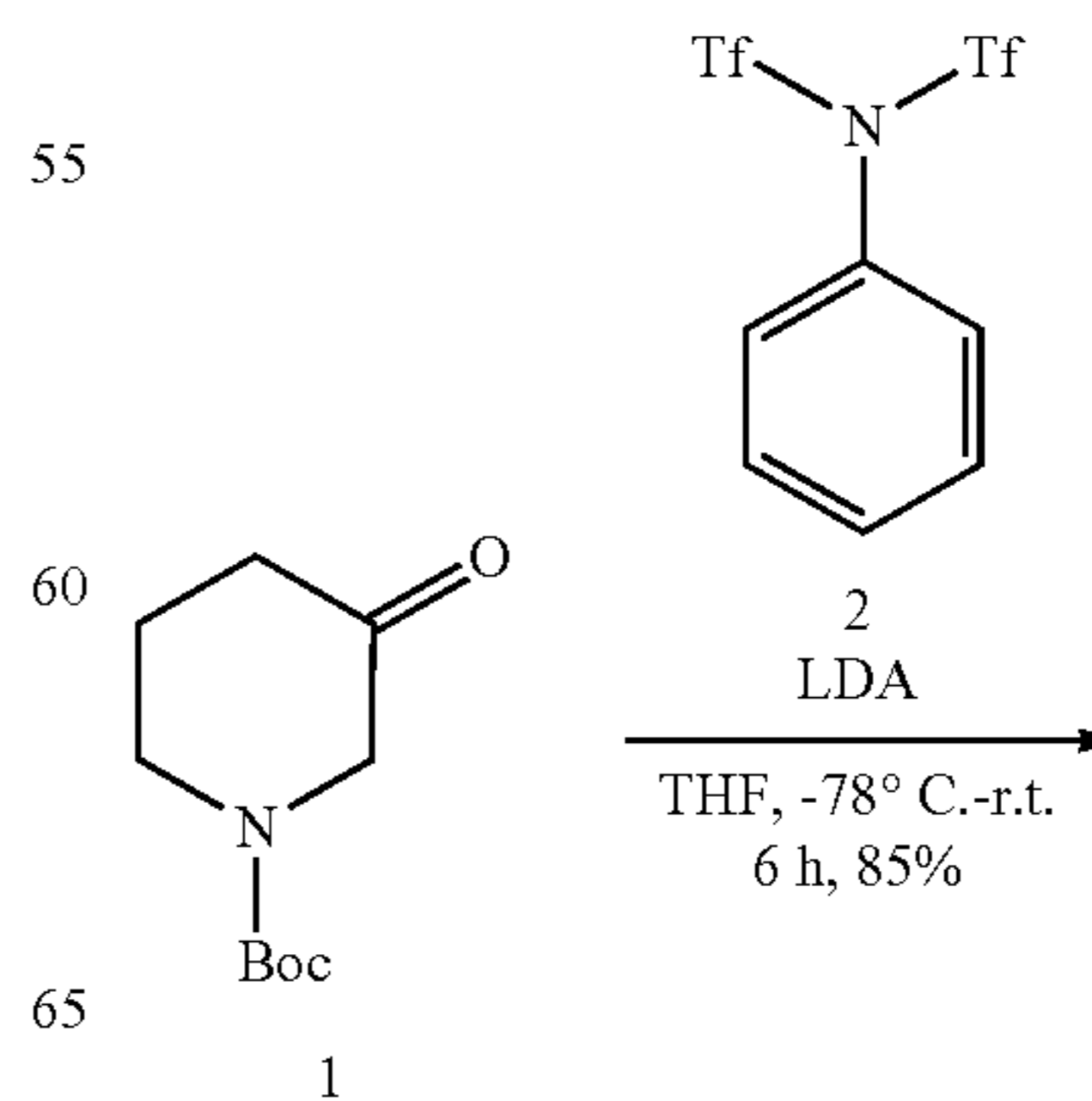
Scheme 6
