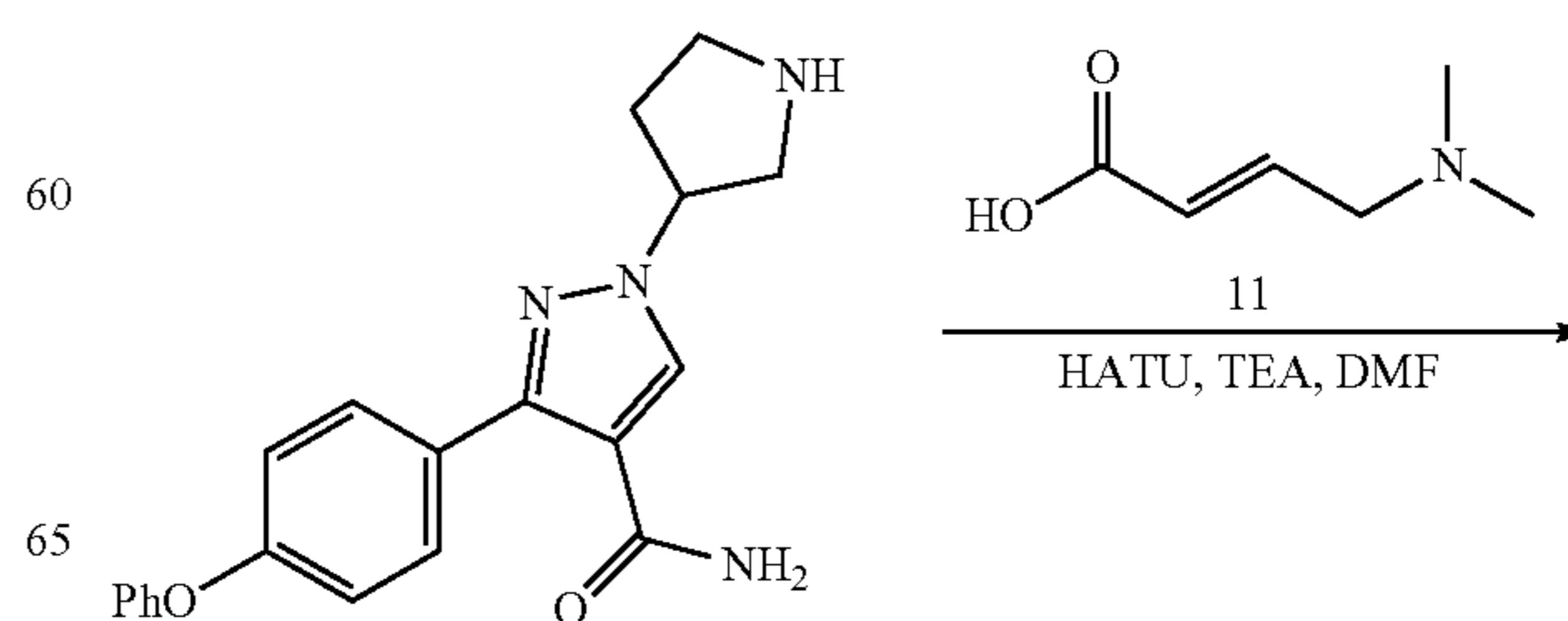
Scheme 24
