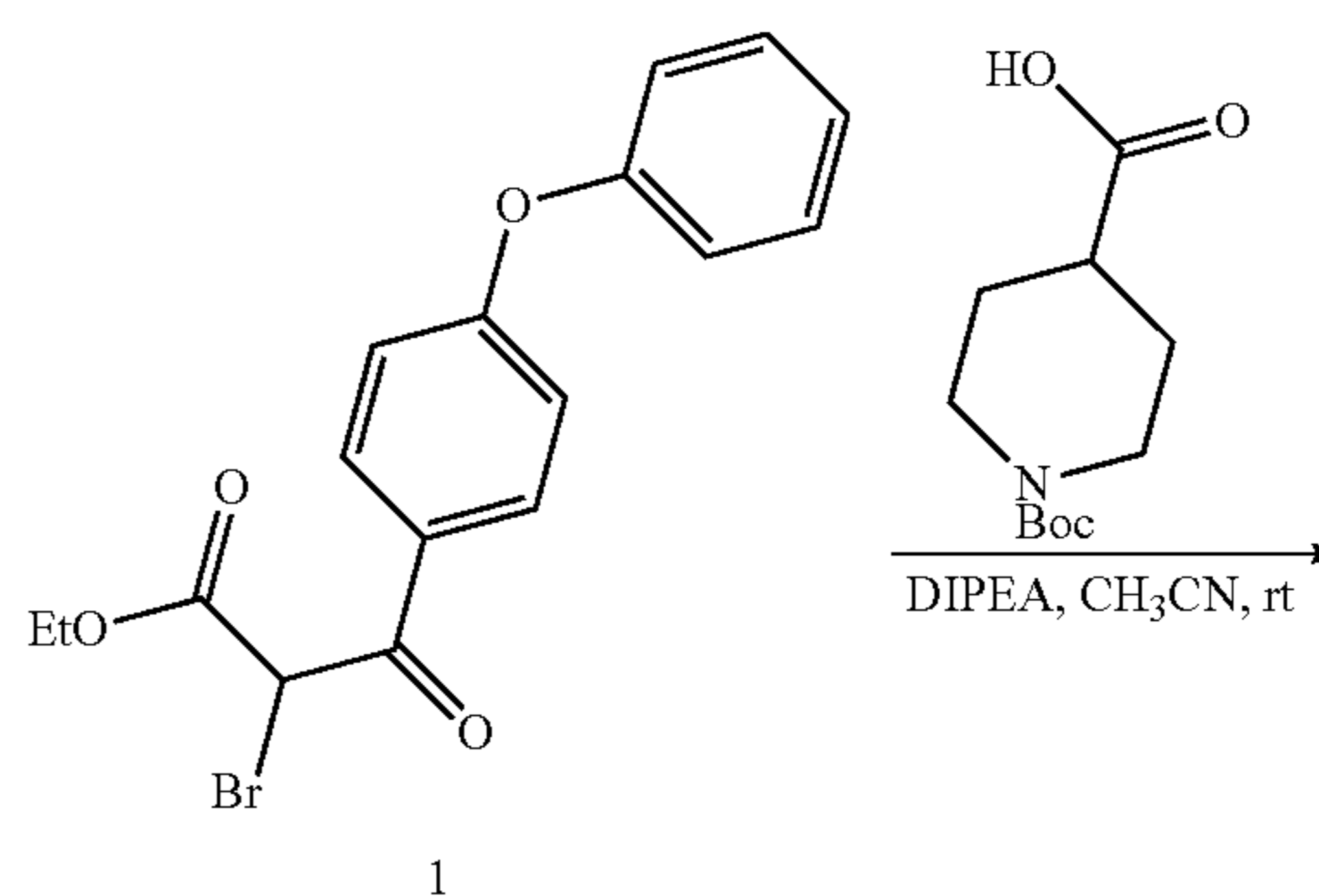
Scheme 36
