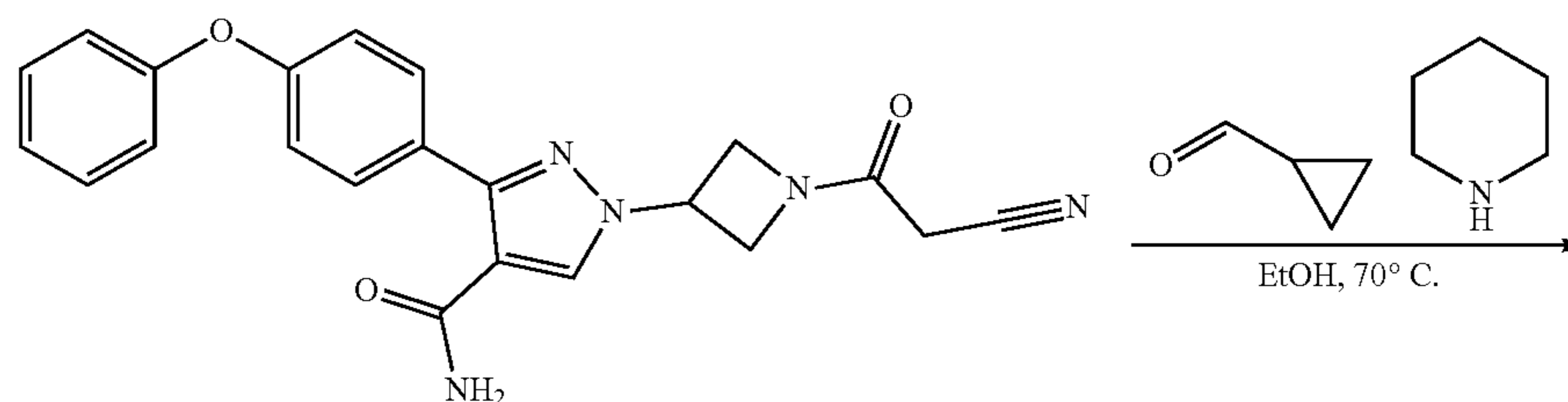
Example 50
