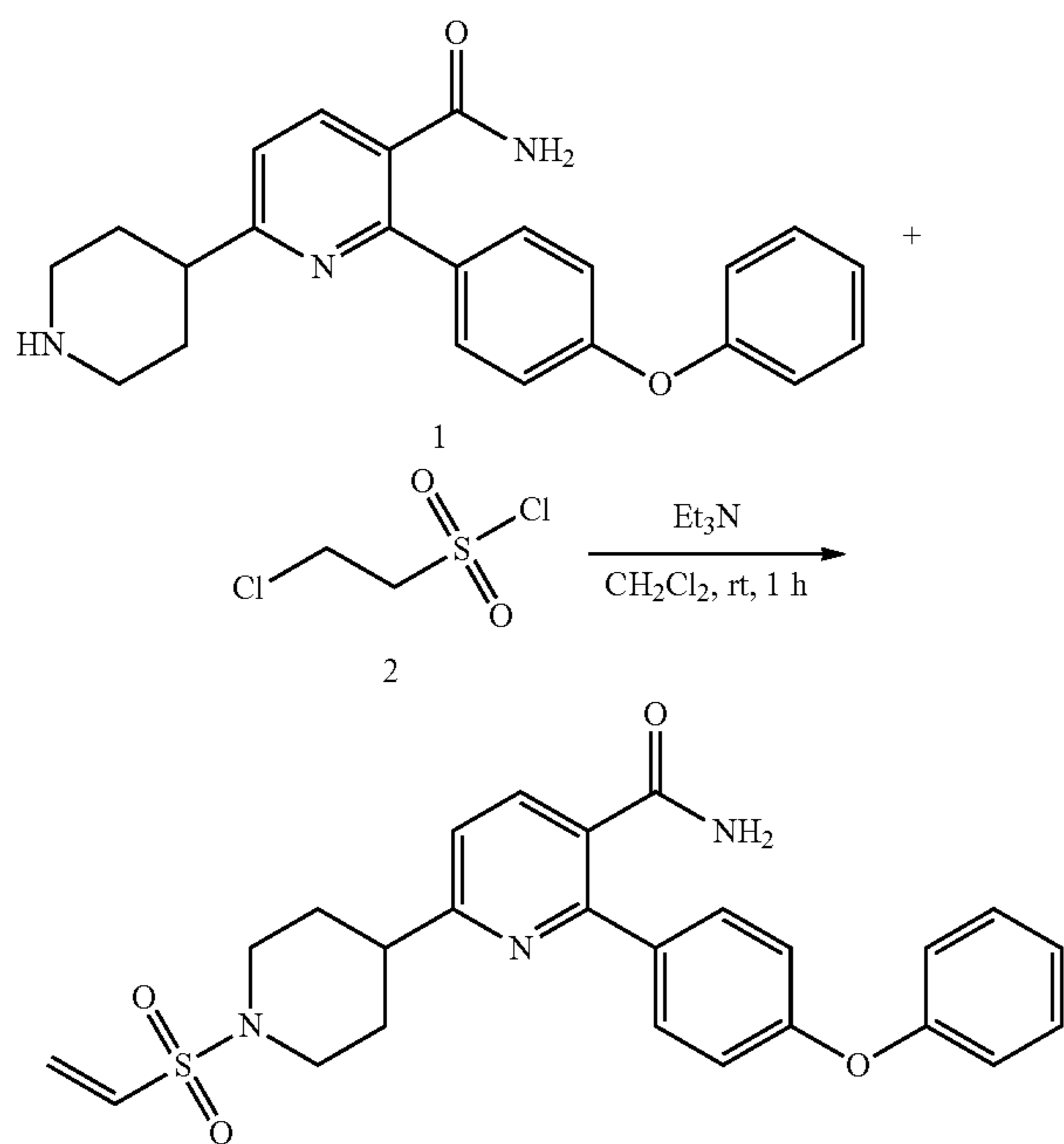
Example 63
