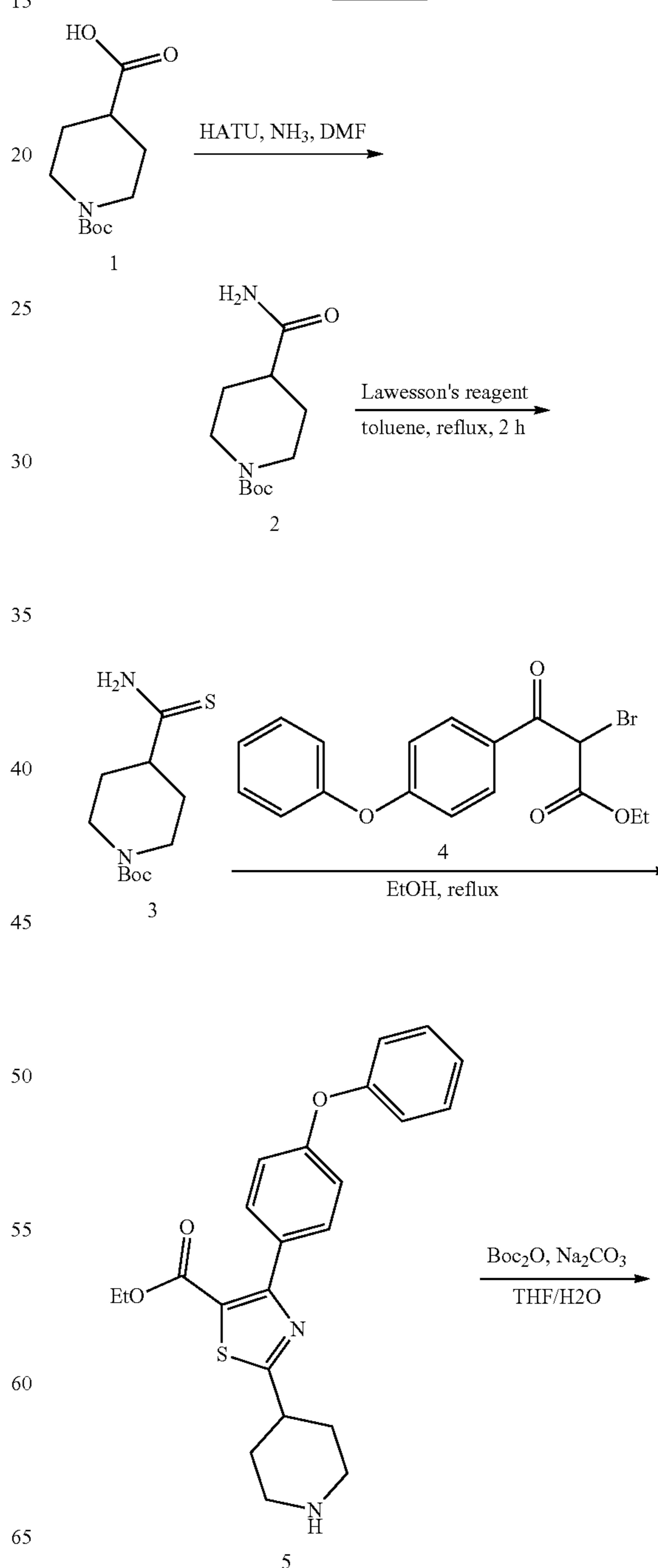
Scheme 42
