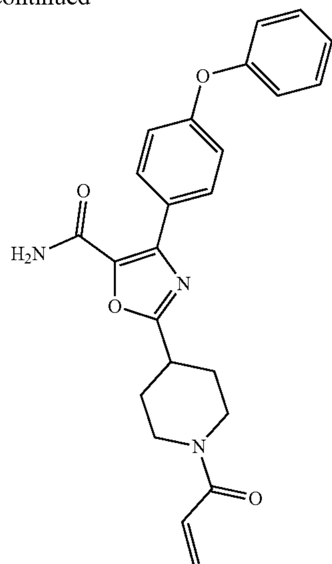
Example 46
