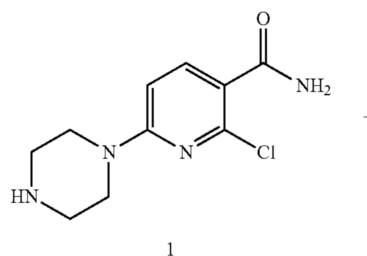
Scheme 18
