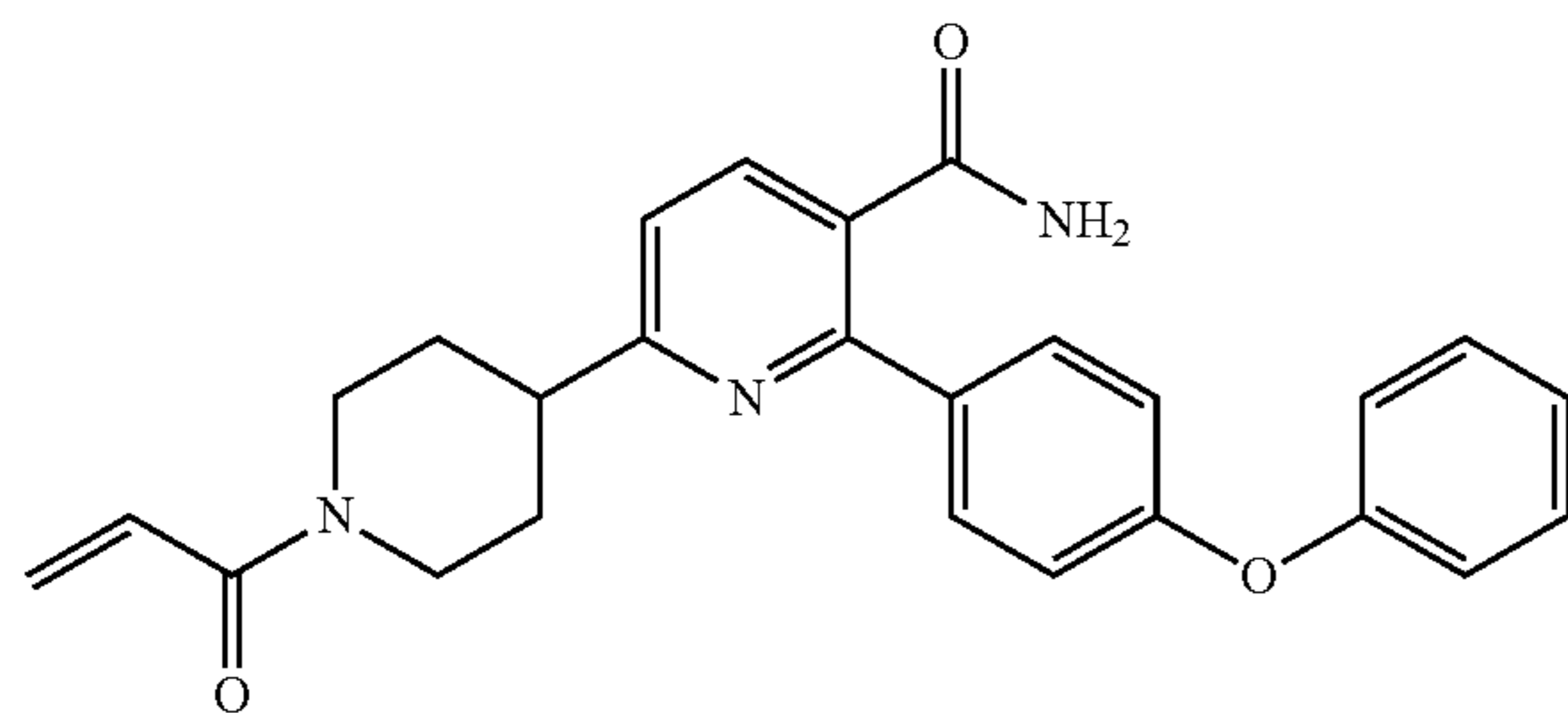
Example 3
