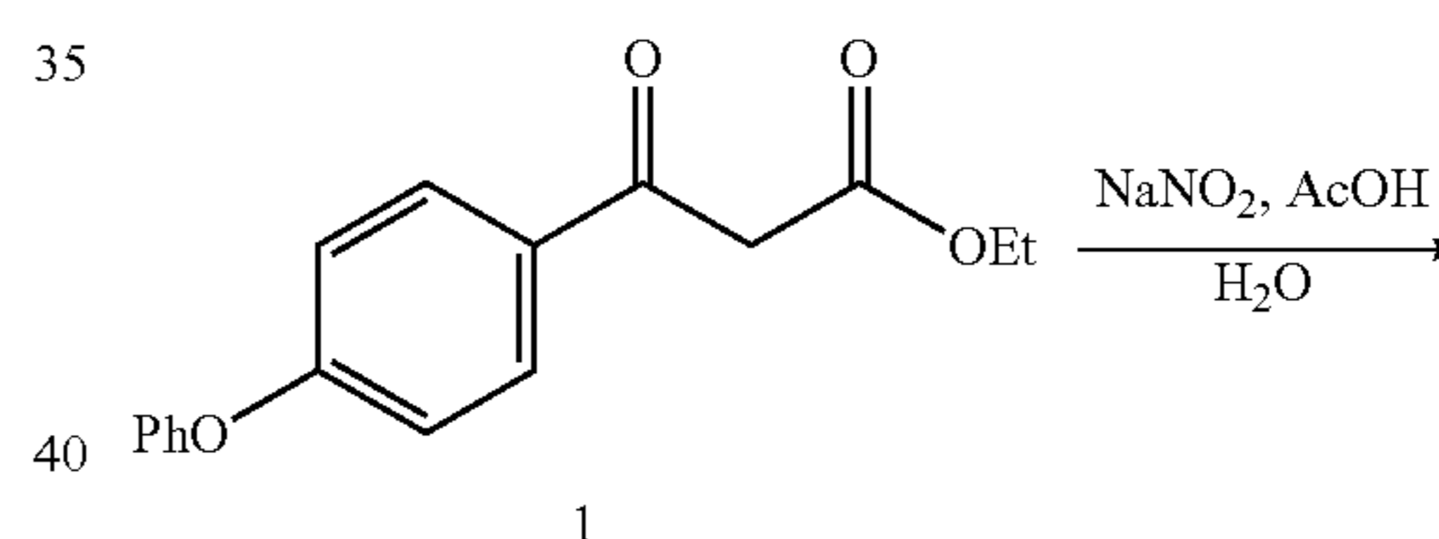
Scheme 35
