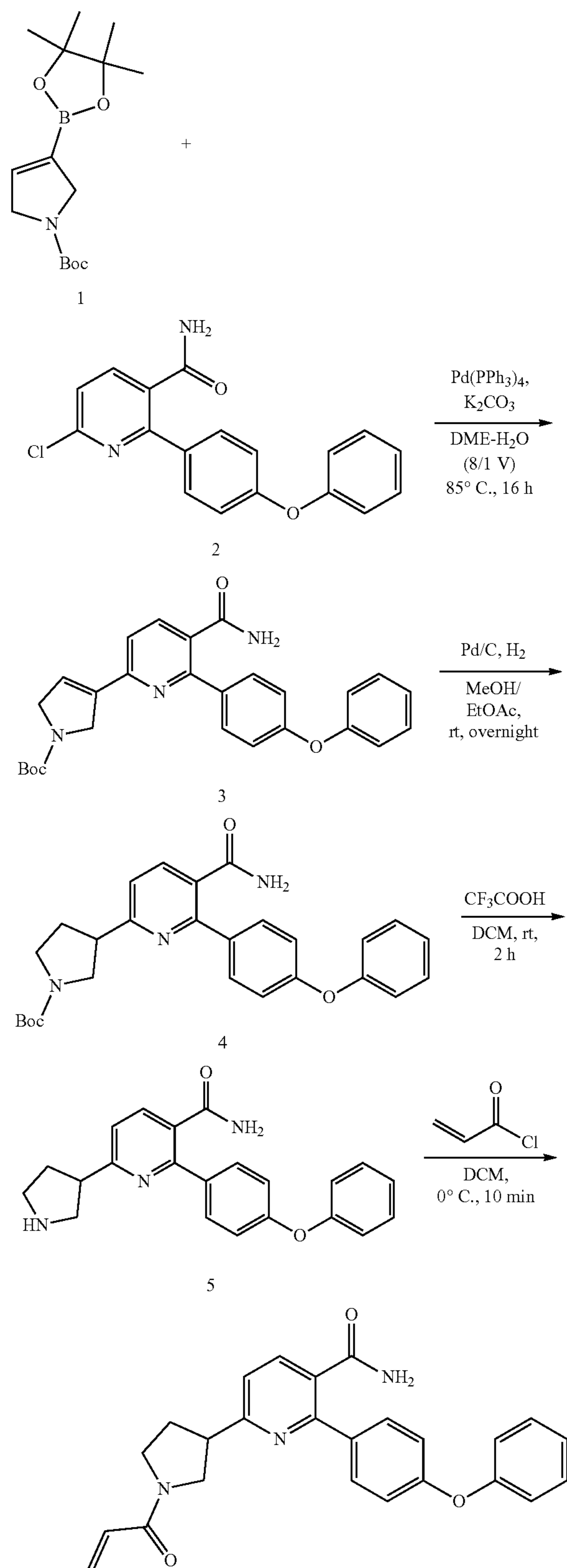
Scheme 12
