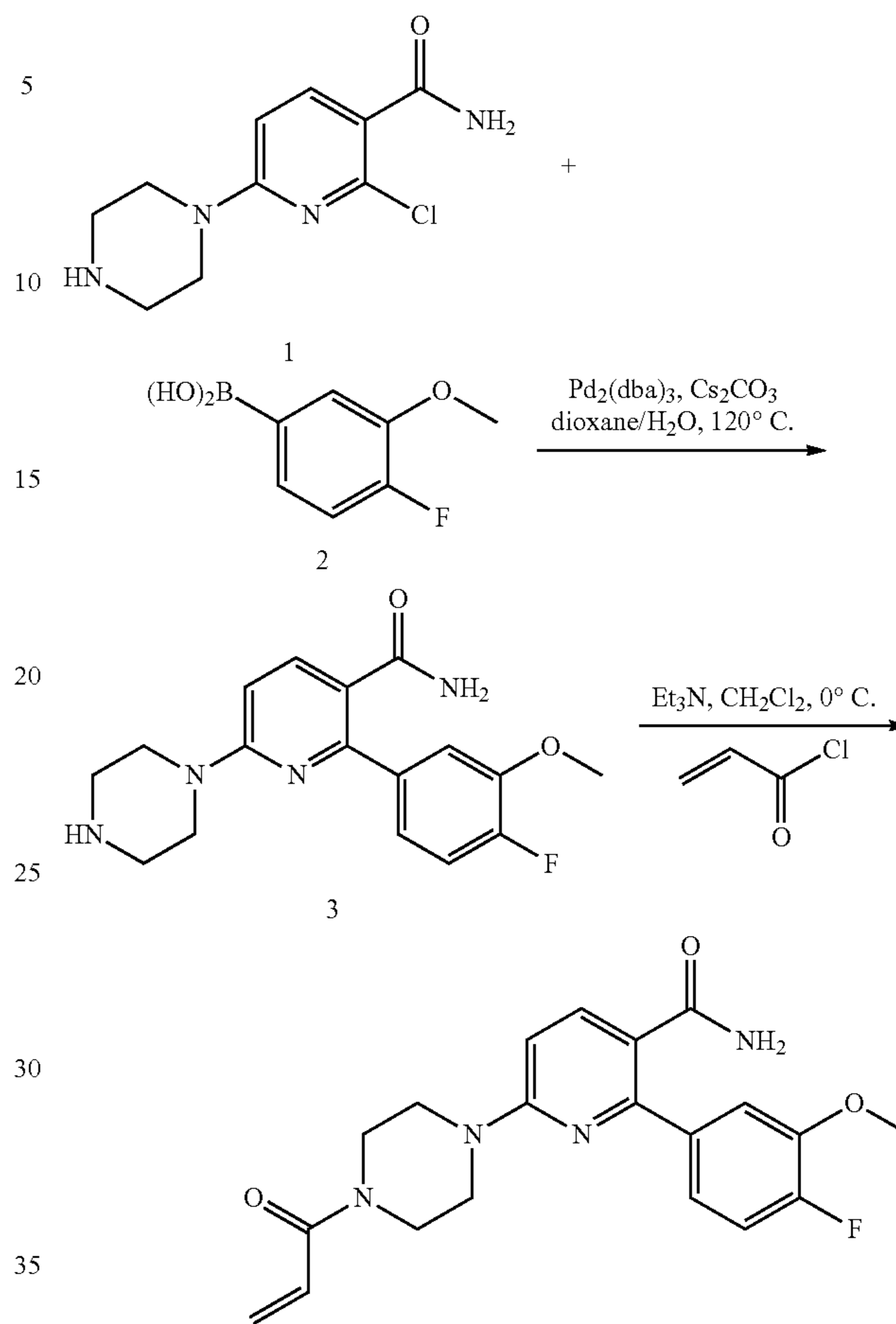
Example 30
