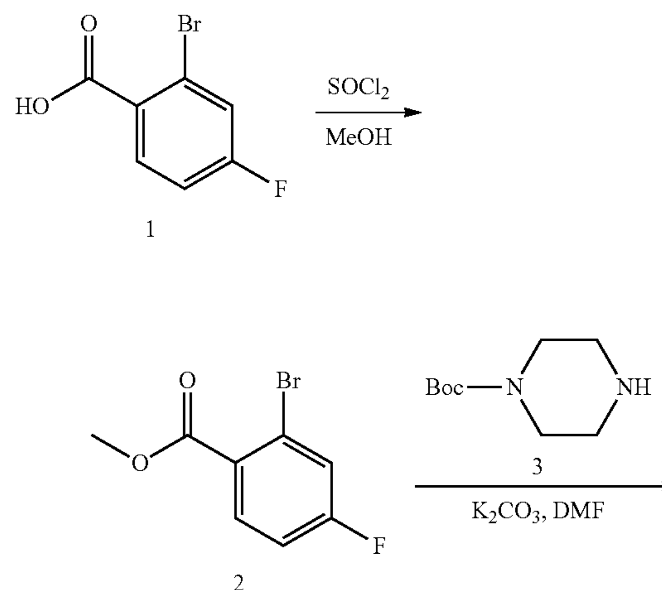
Scheme 47
