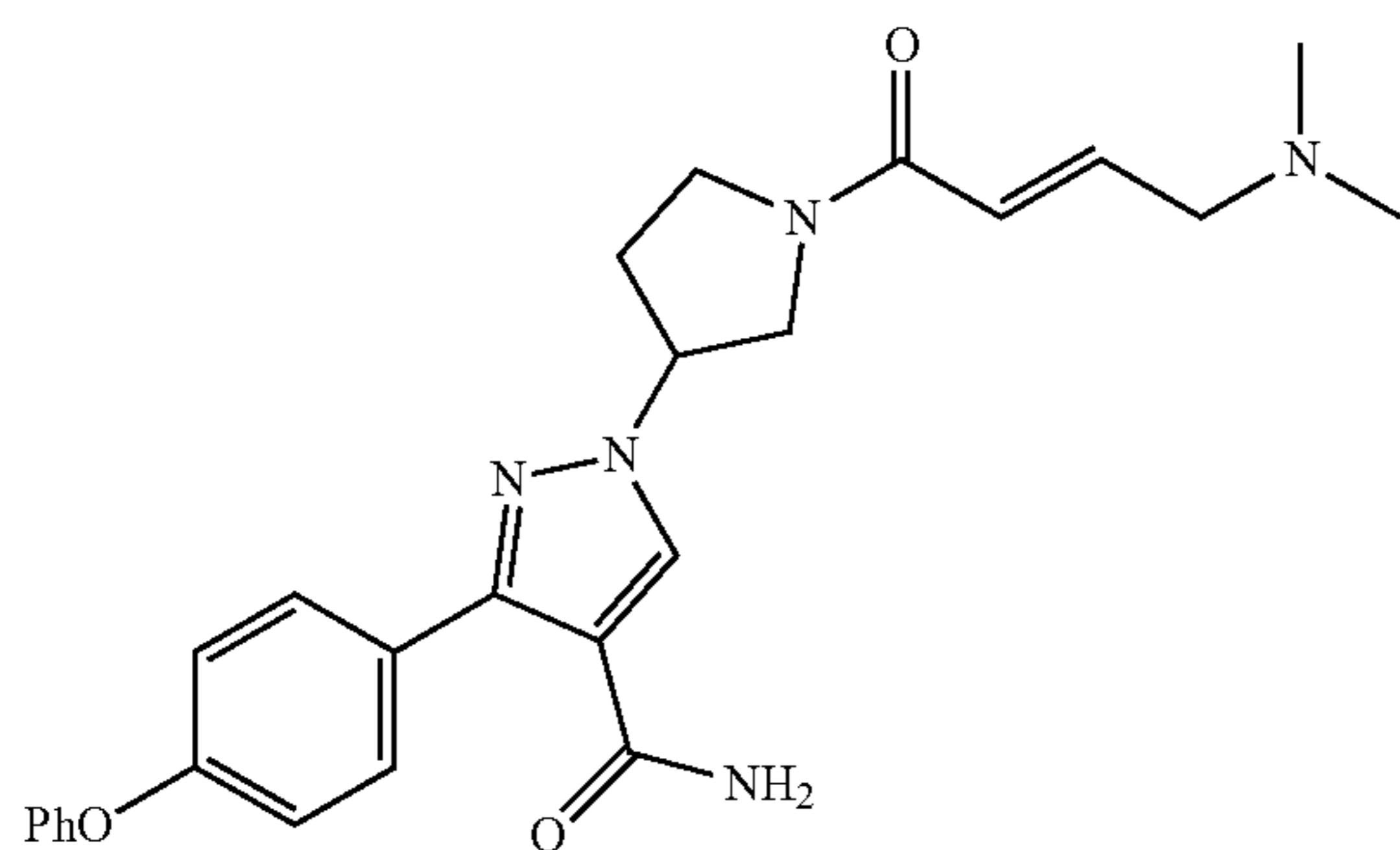
Example 34
