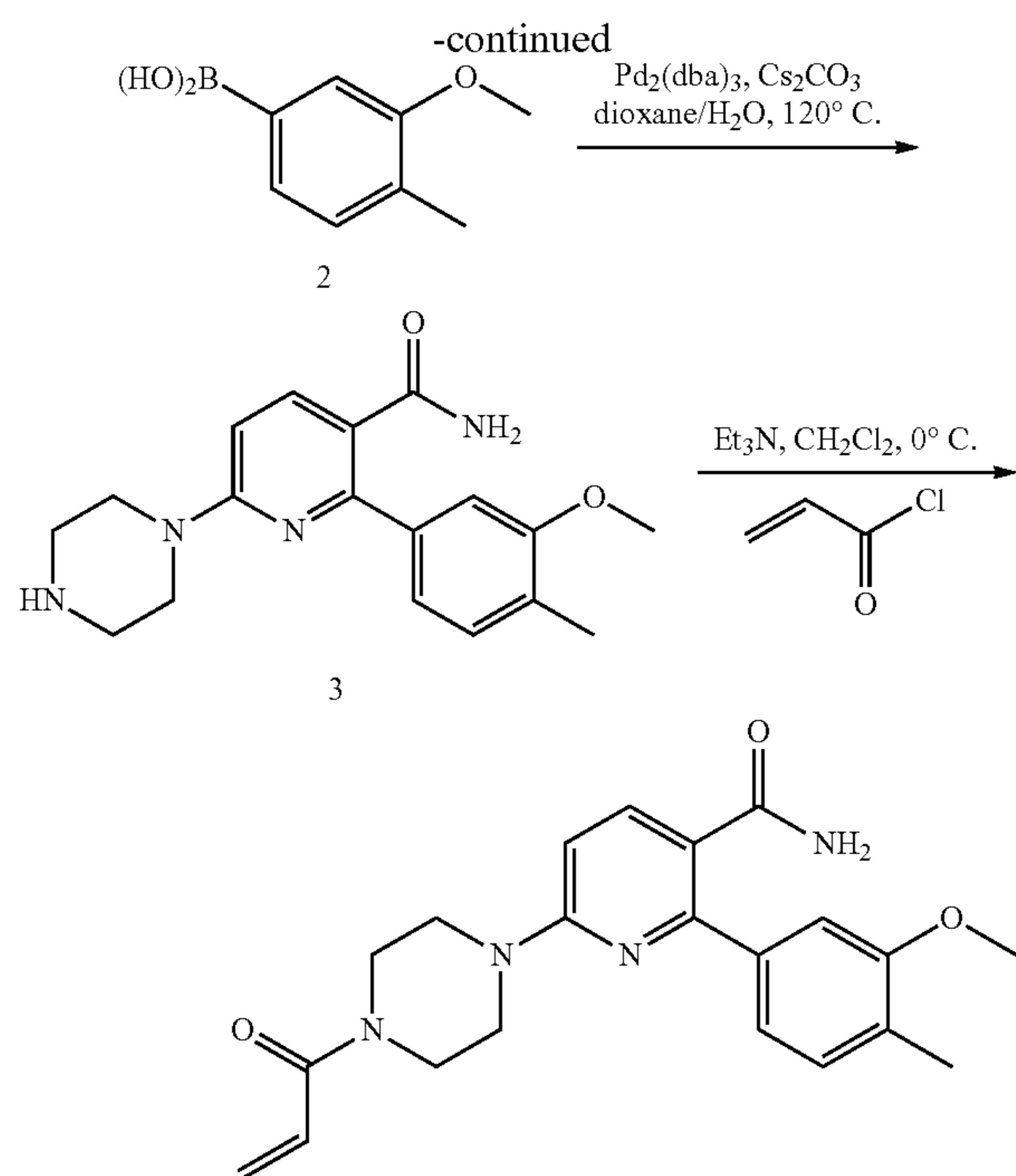
Example 29
