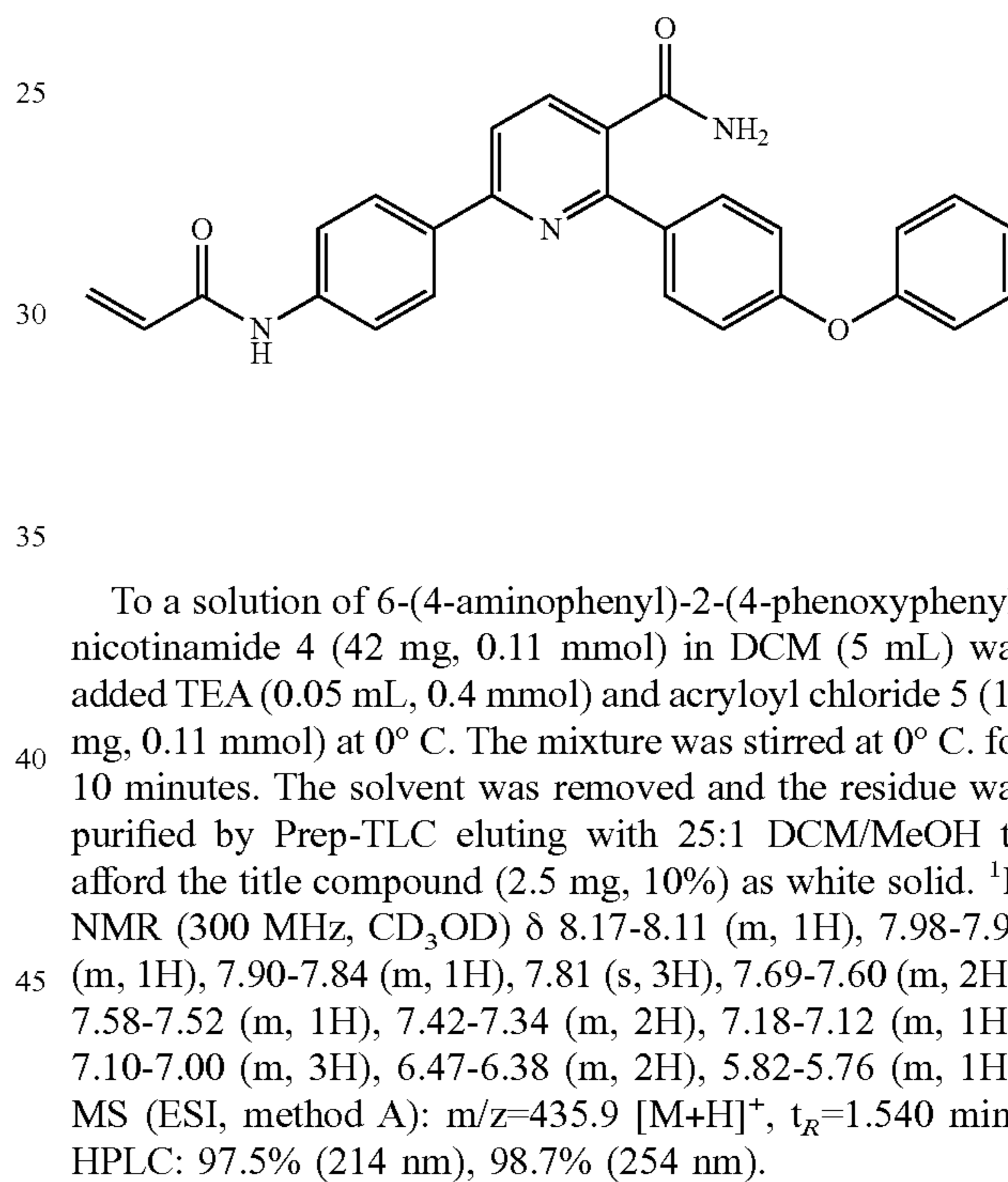
Scheme 6
