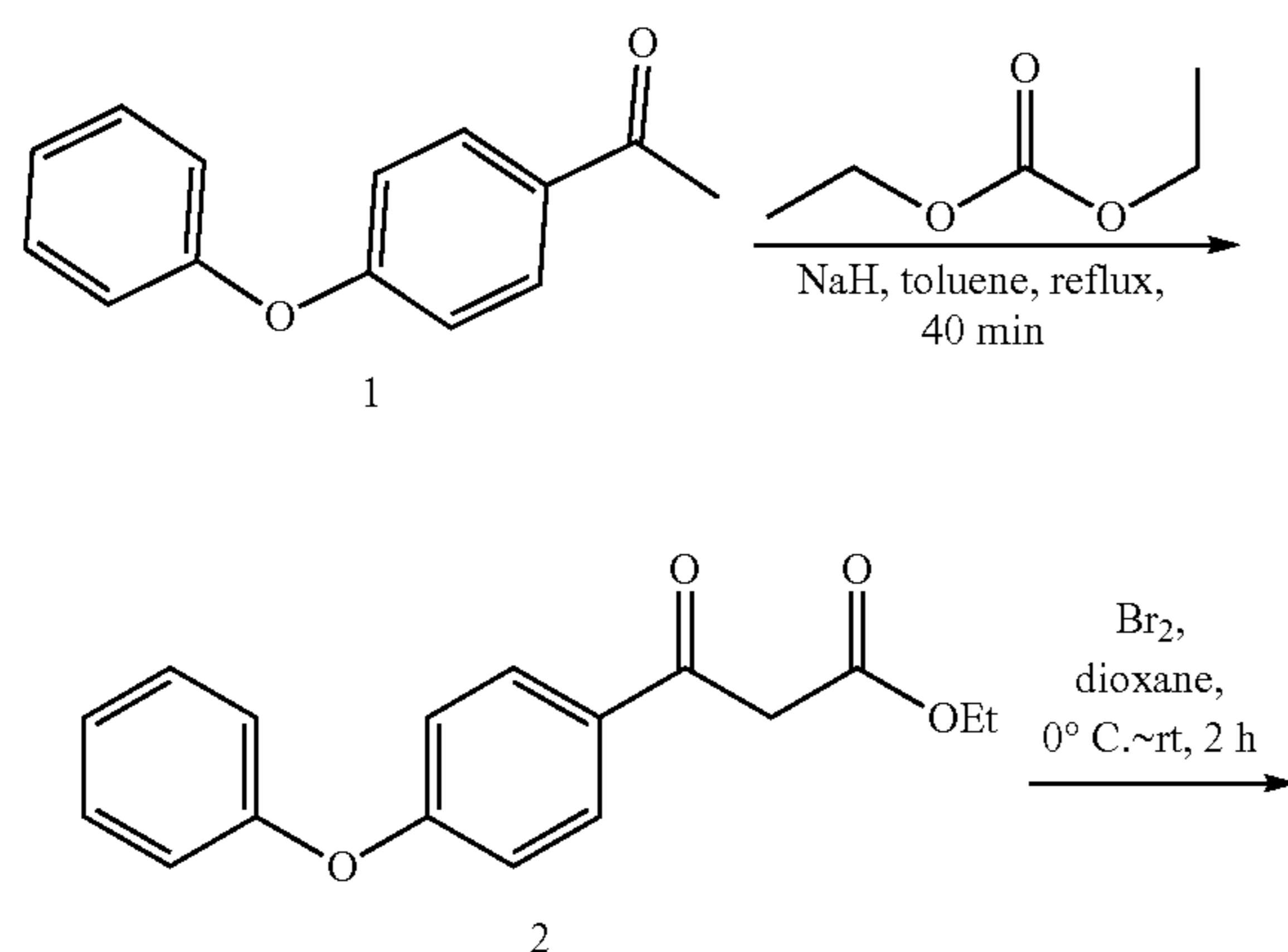
Scheme 32
