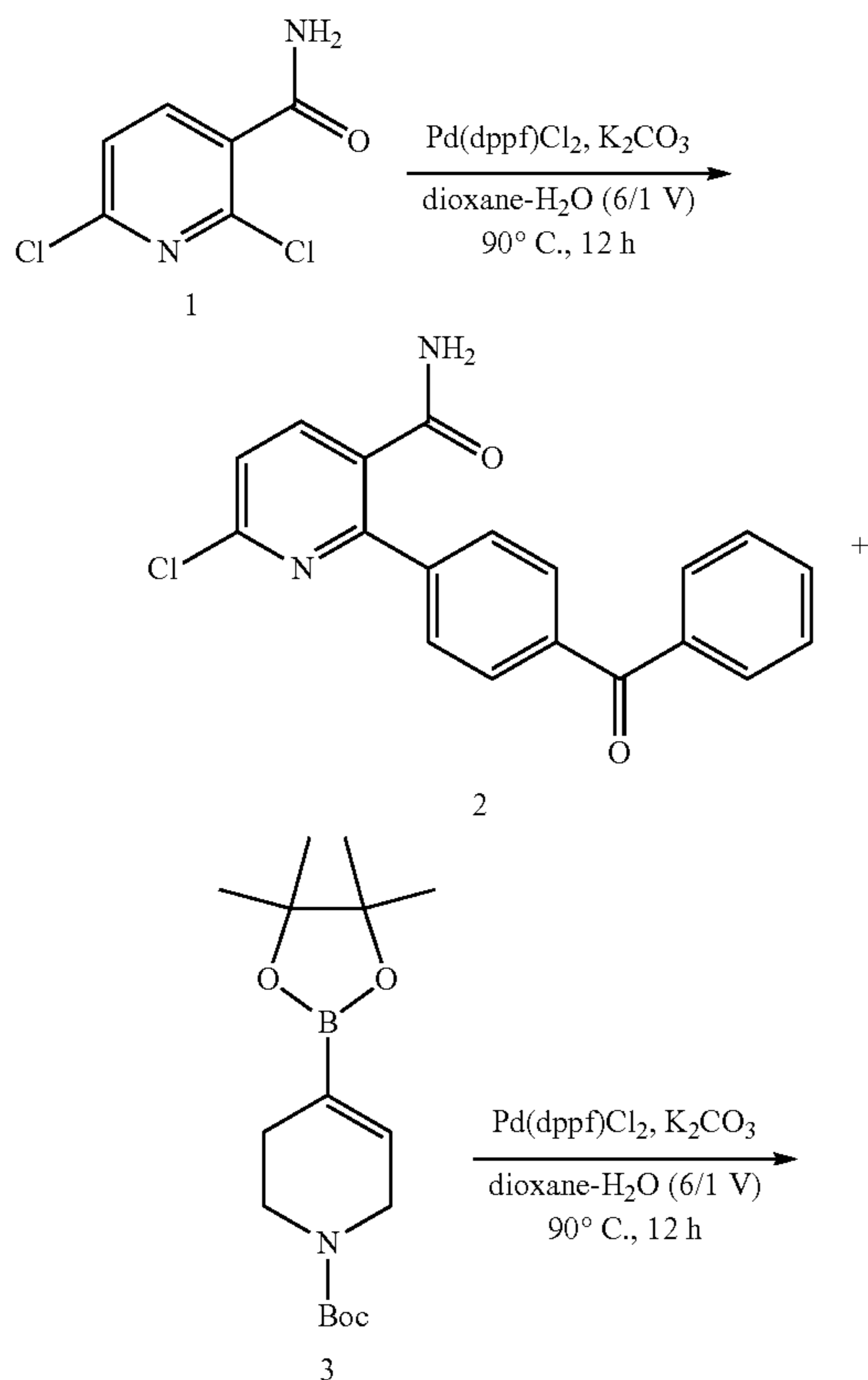
Scheme 48
