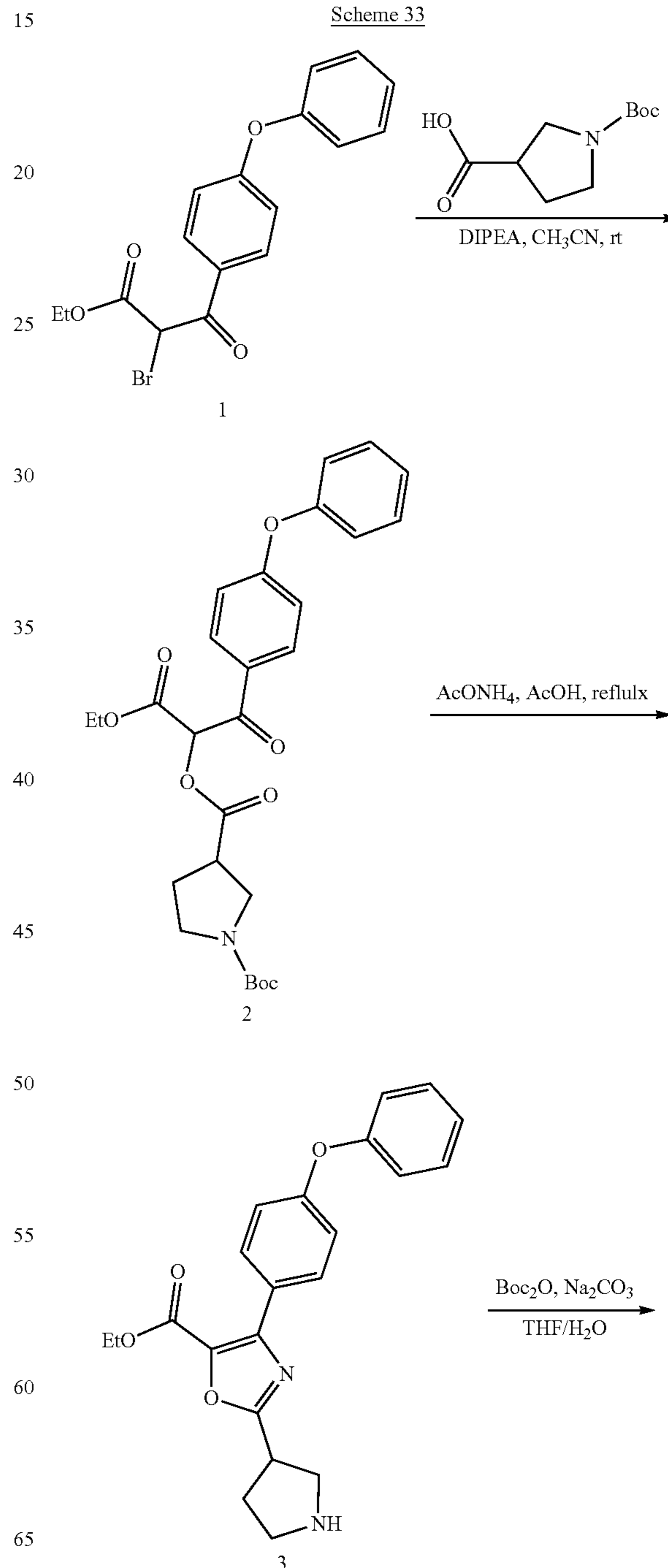
Scheme 33
