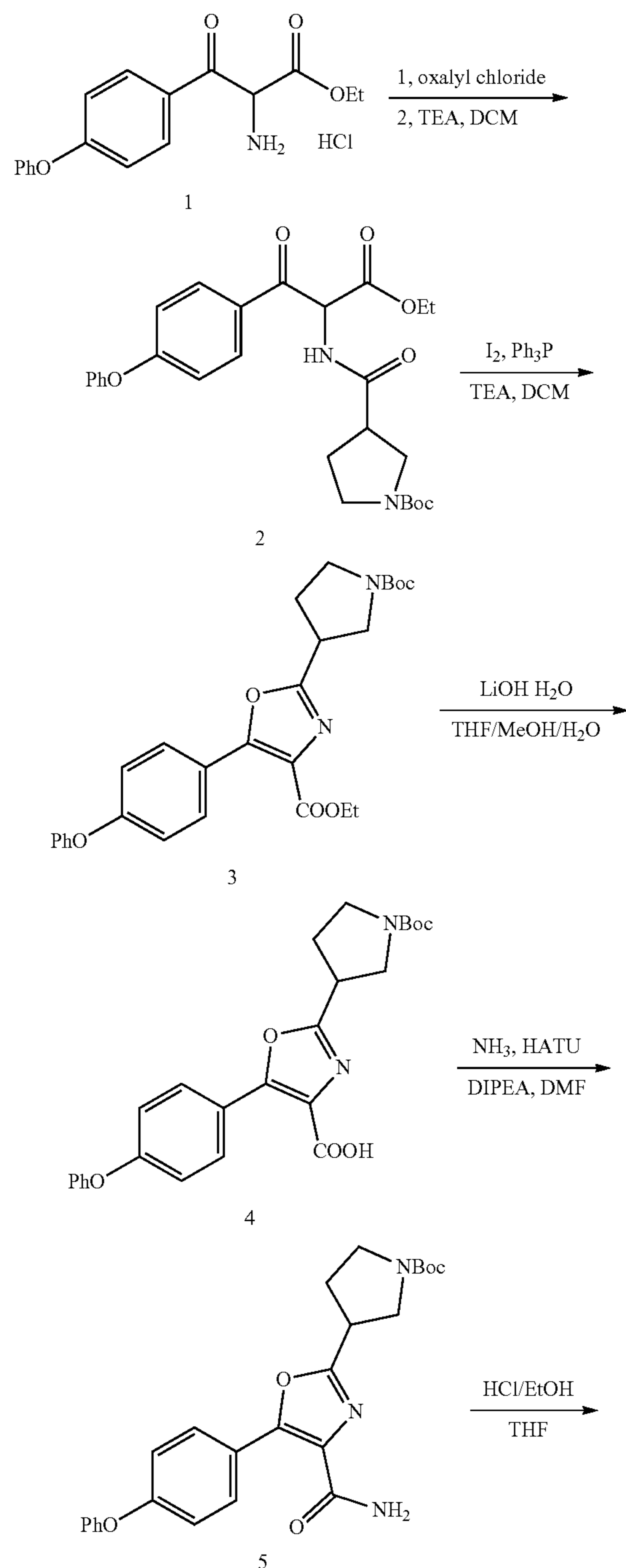
Scheme 38
