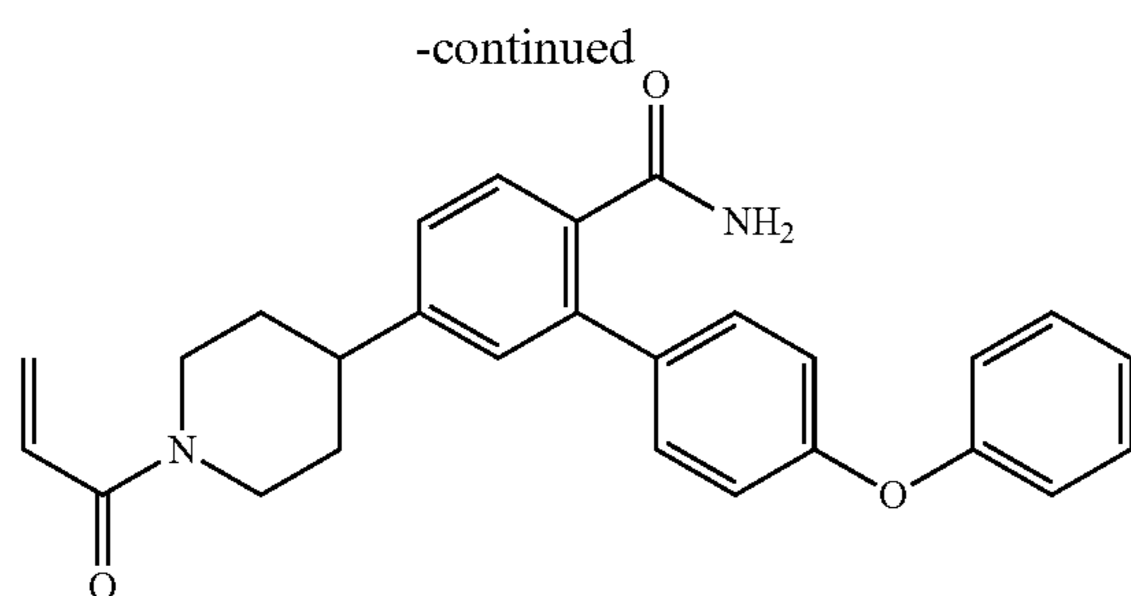
Example 55
