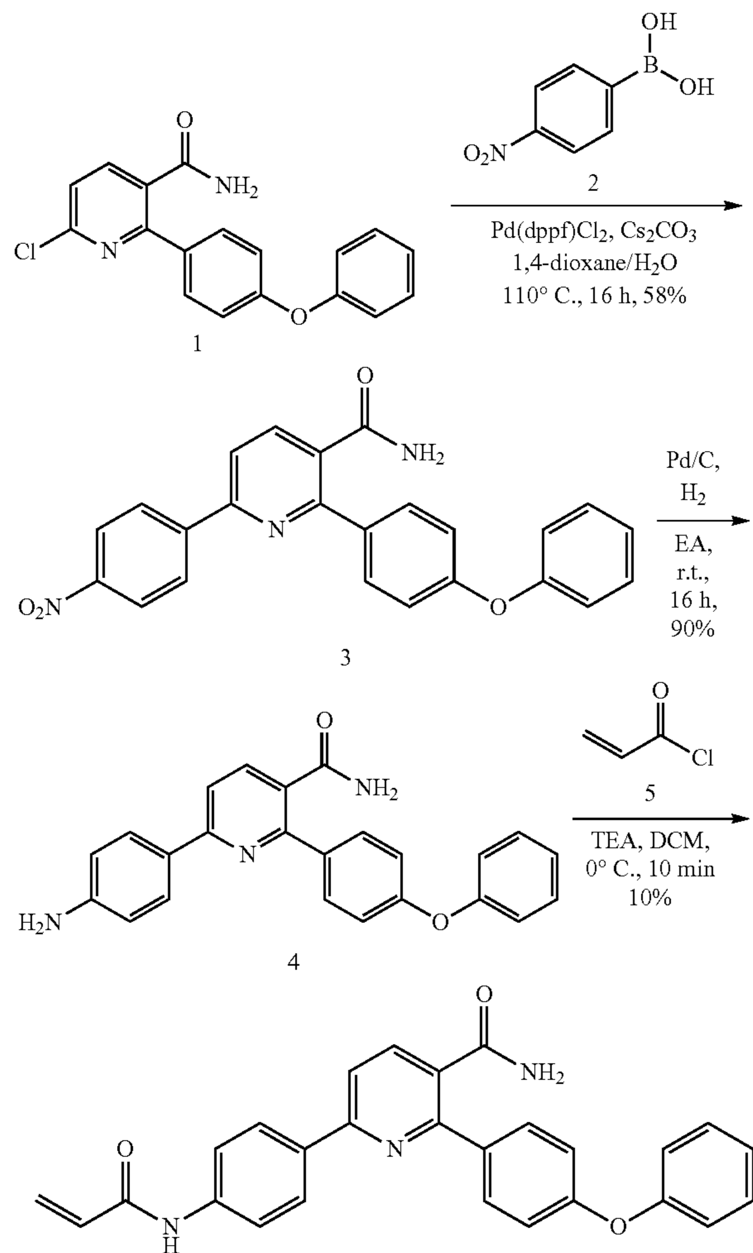
Example 7
