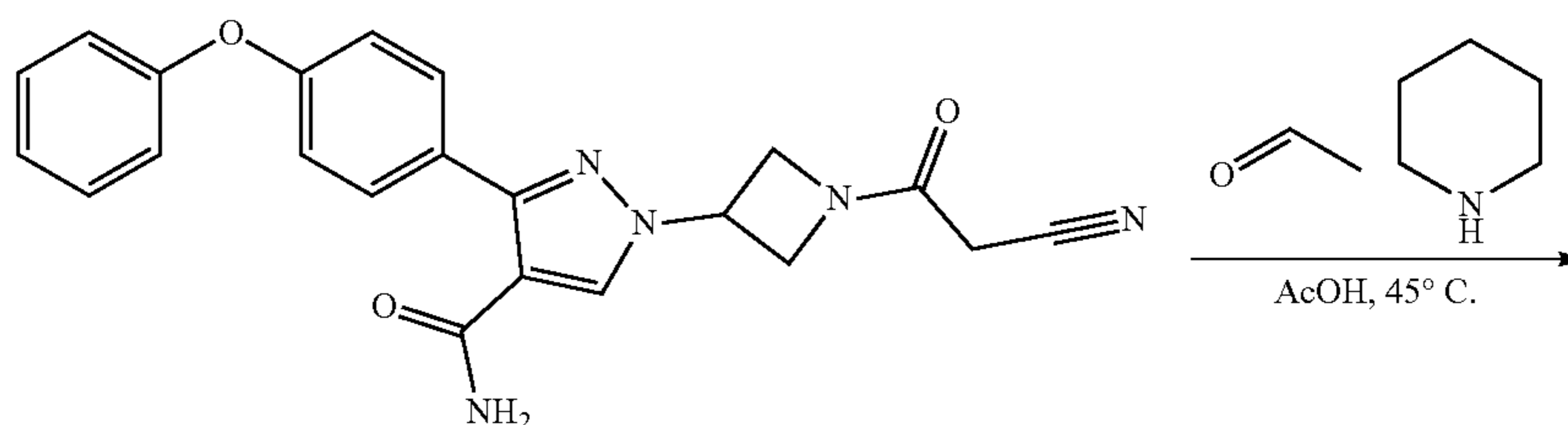
Example 50
