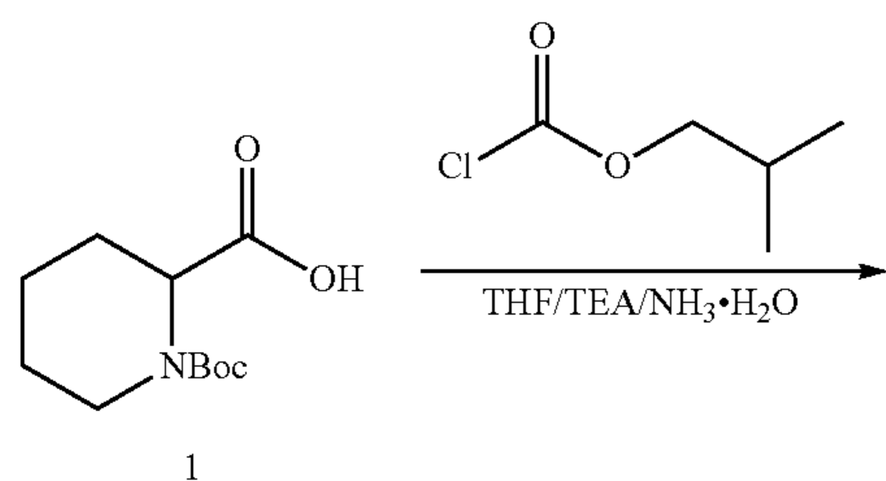
Scheme 30
