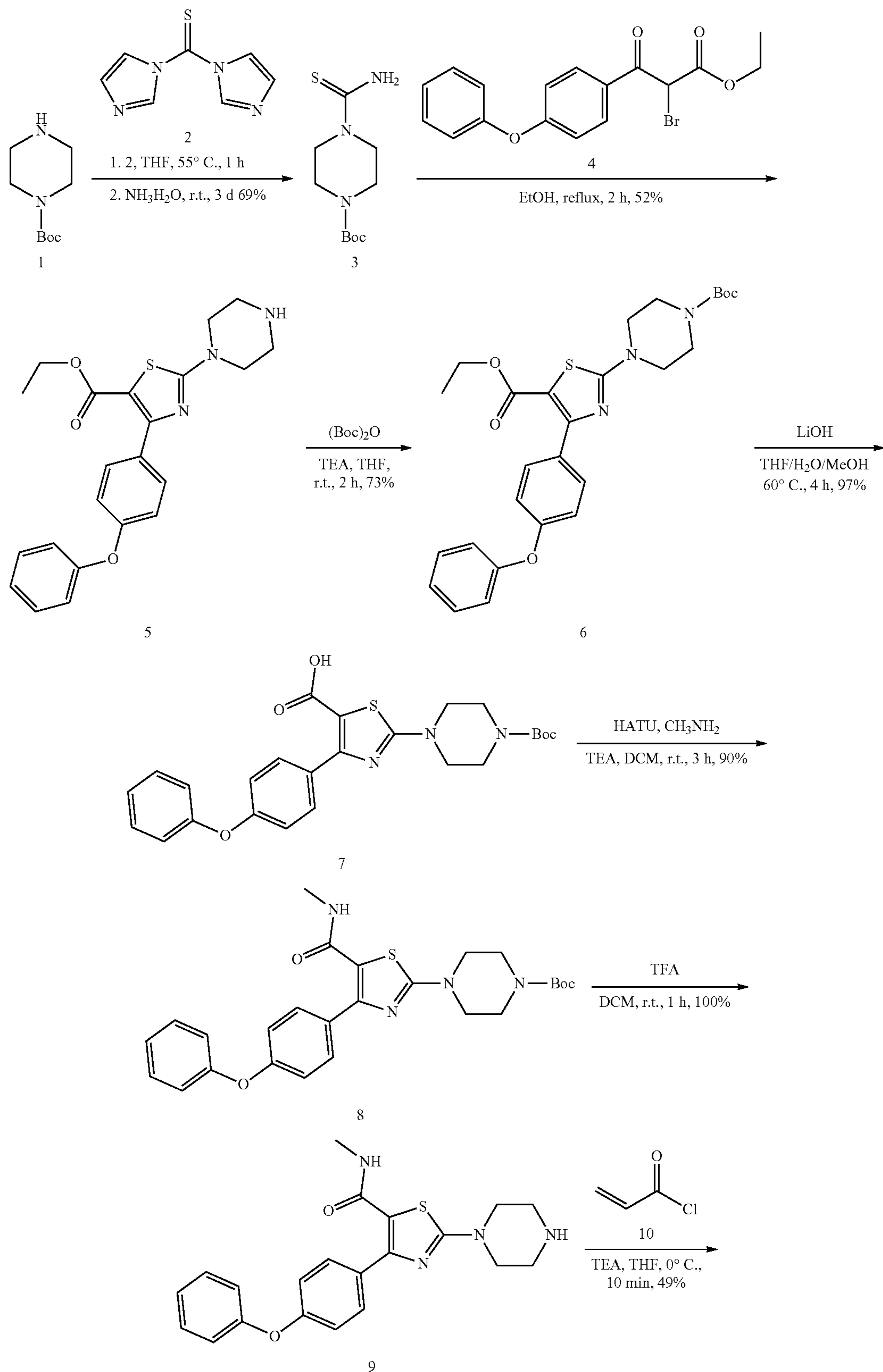
Scheme 37
