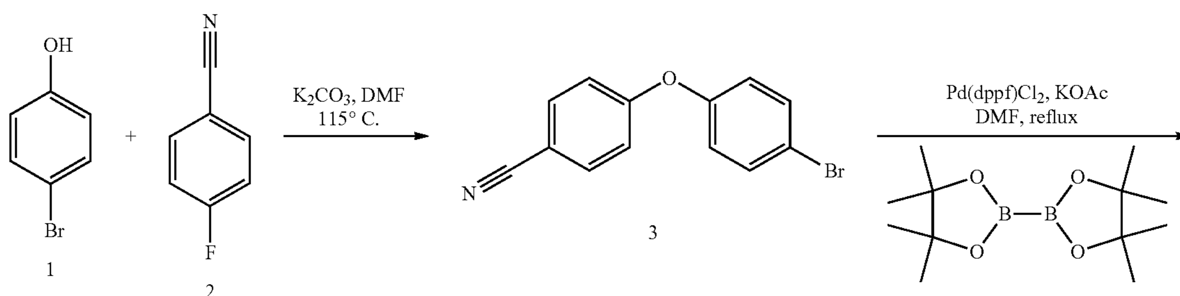
Scheme 16
