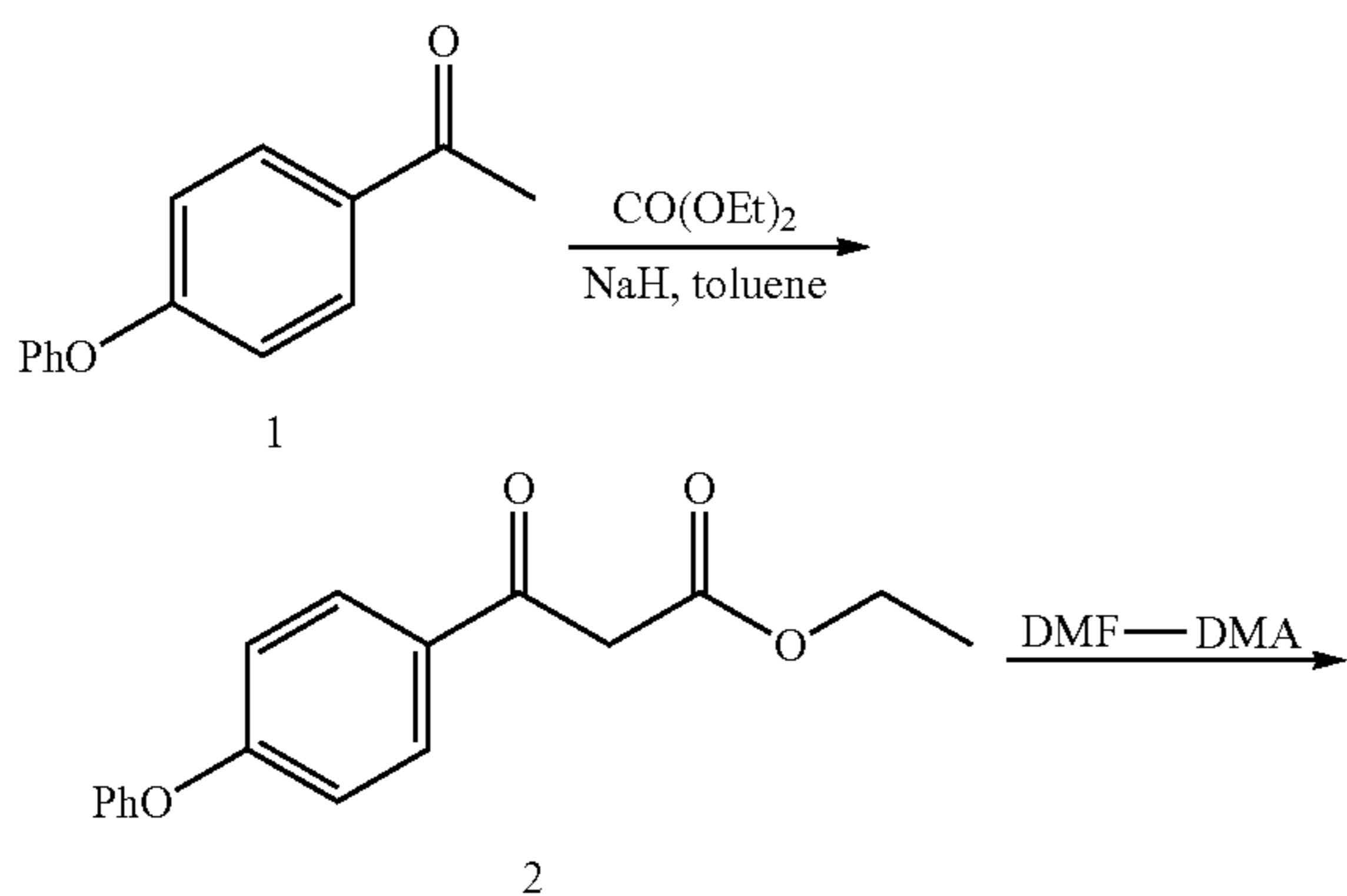
Scheme 23
