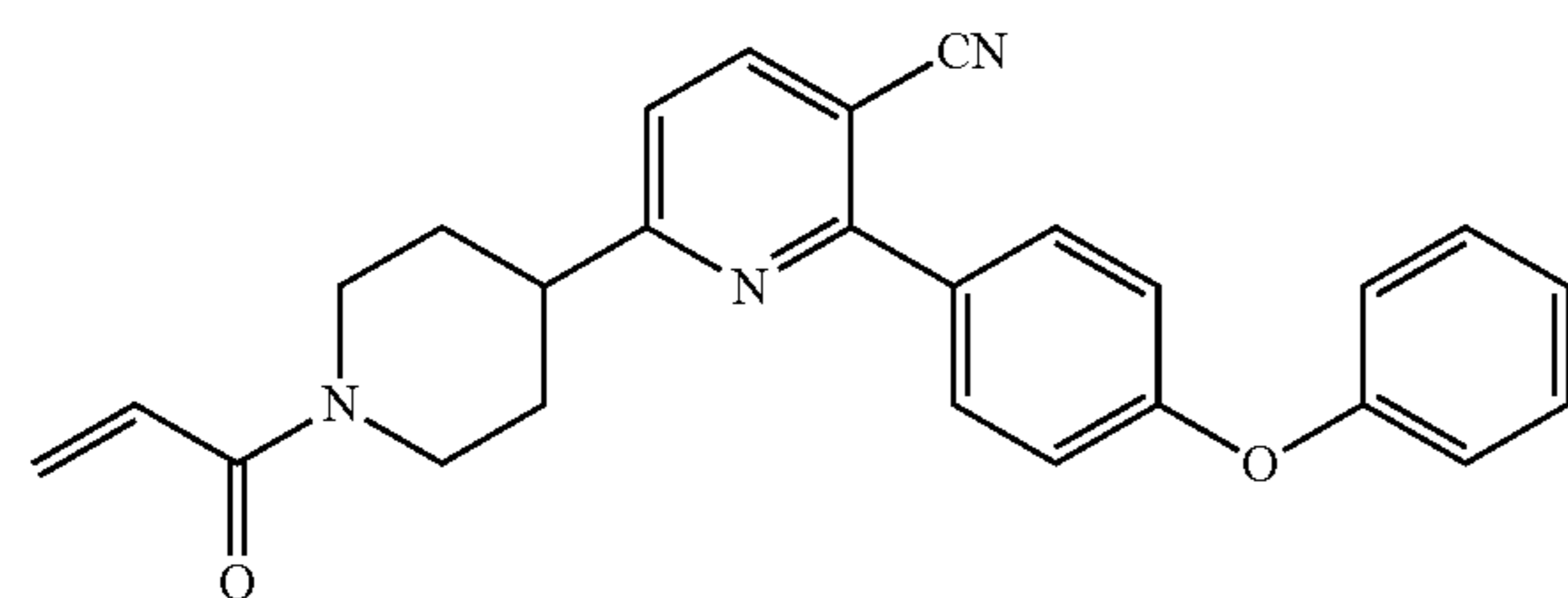
Example 24
