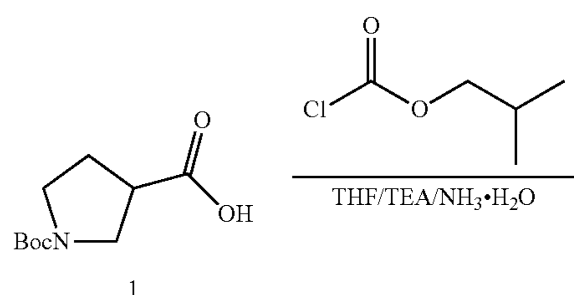
Scheme 31
