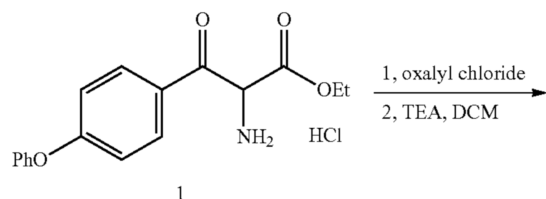
Scheme 34
