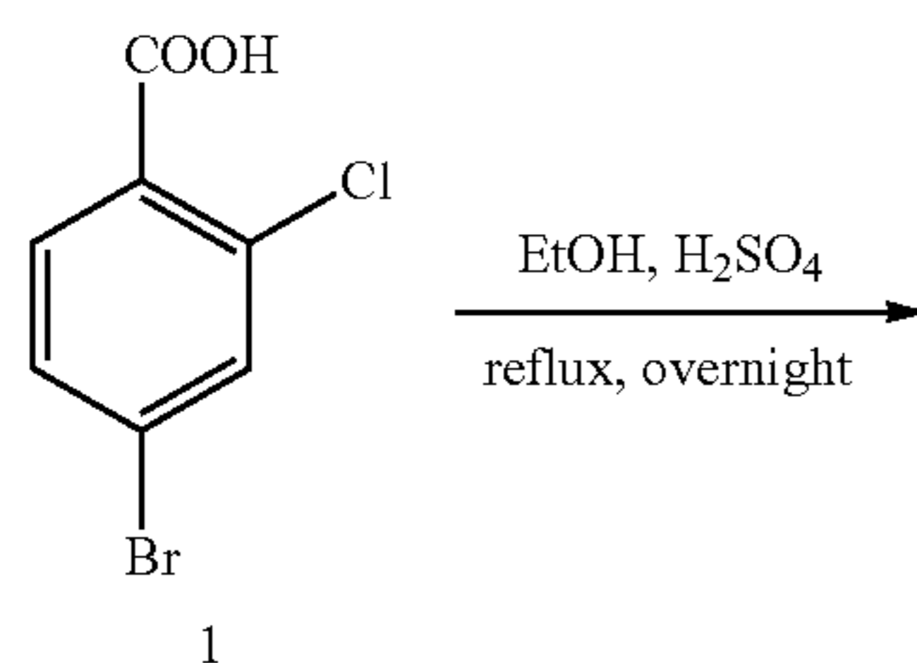
Scheme 45
