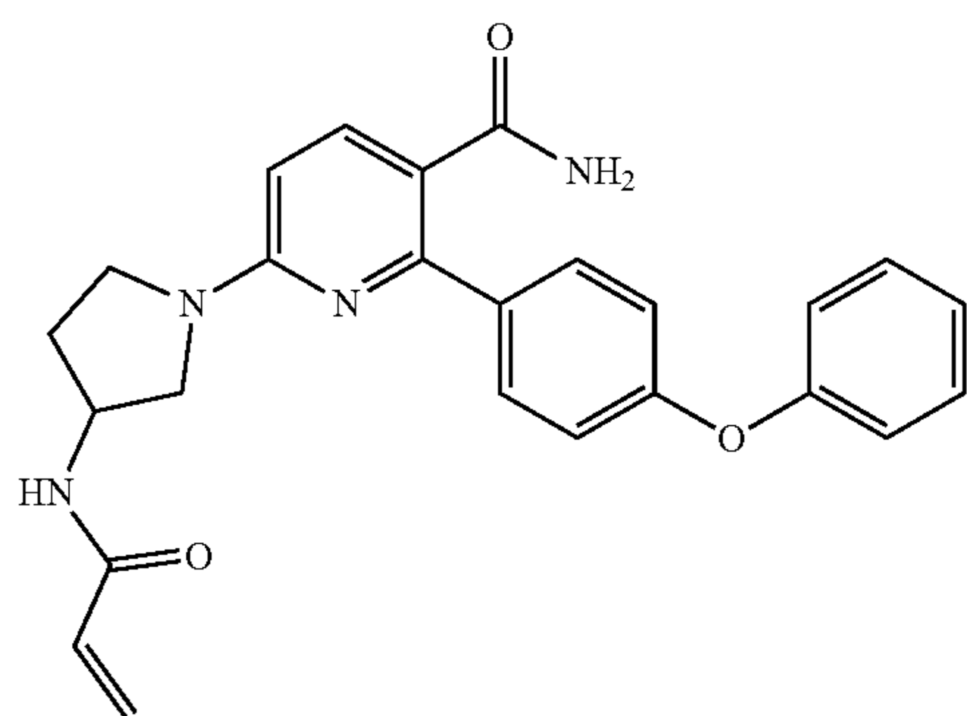
Example 10
