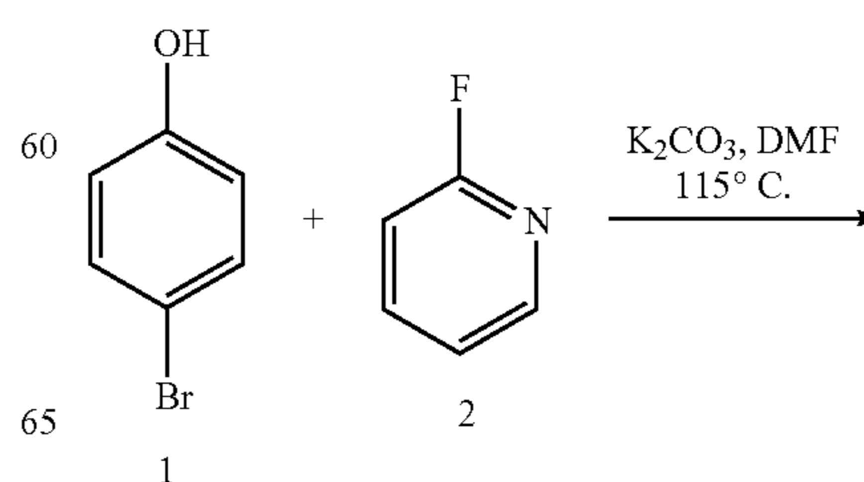
Scheme 21
