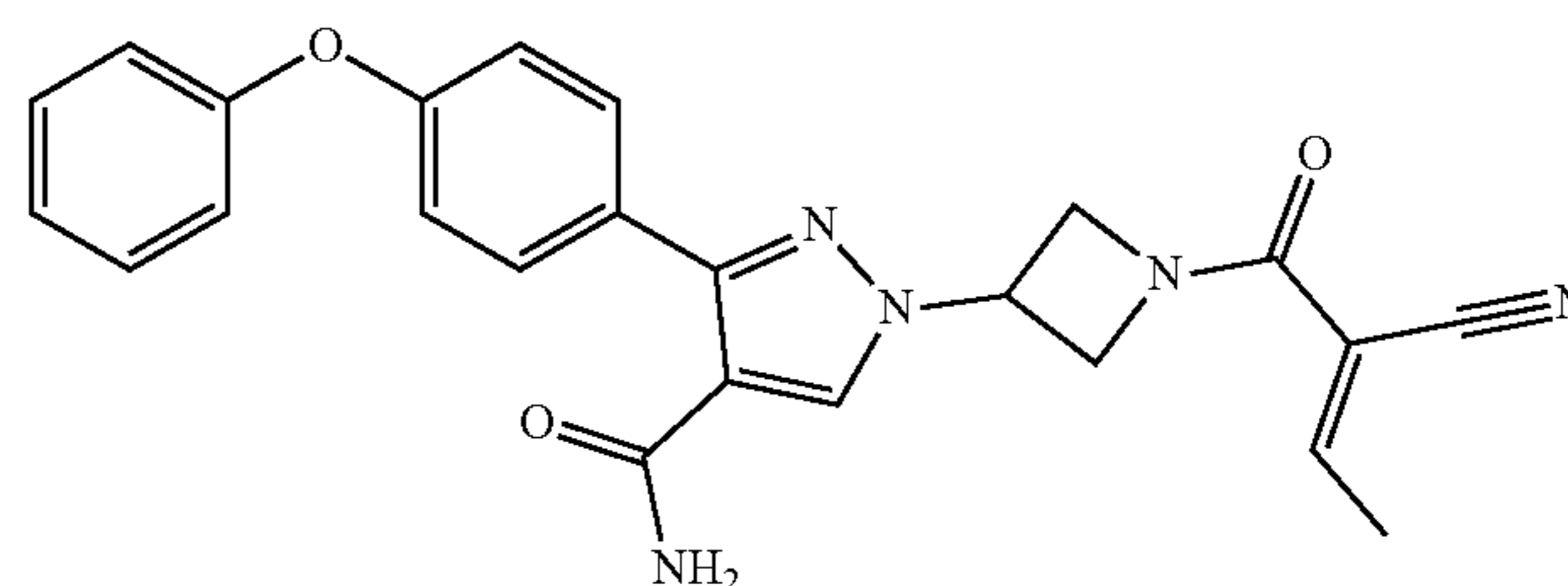
Example 59
