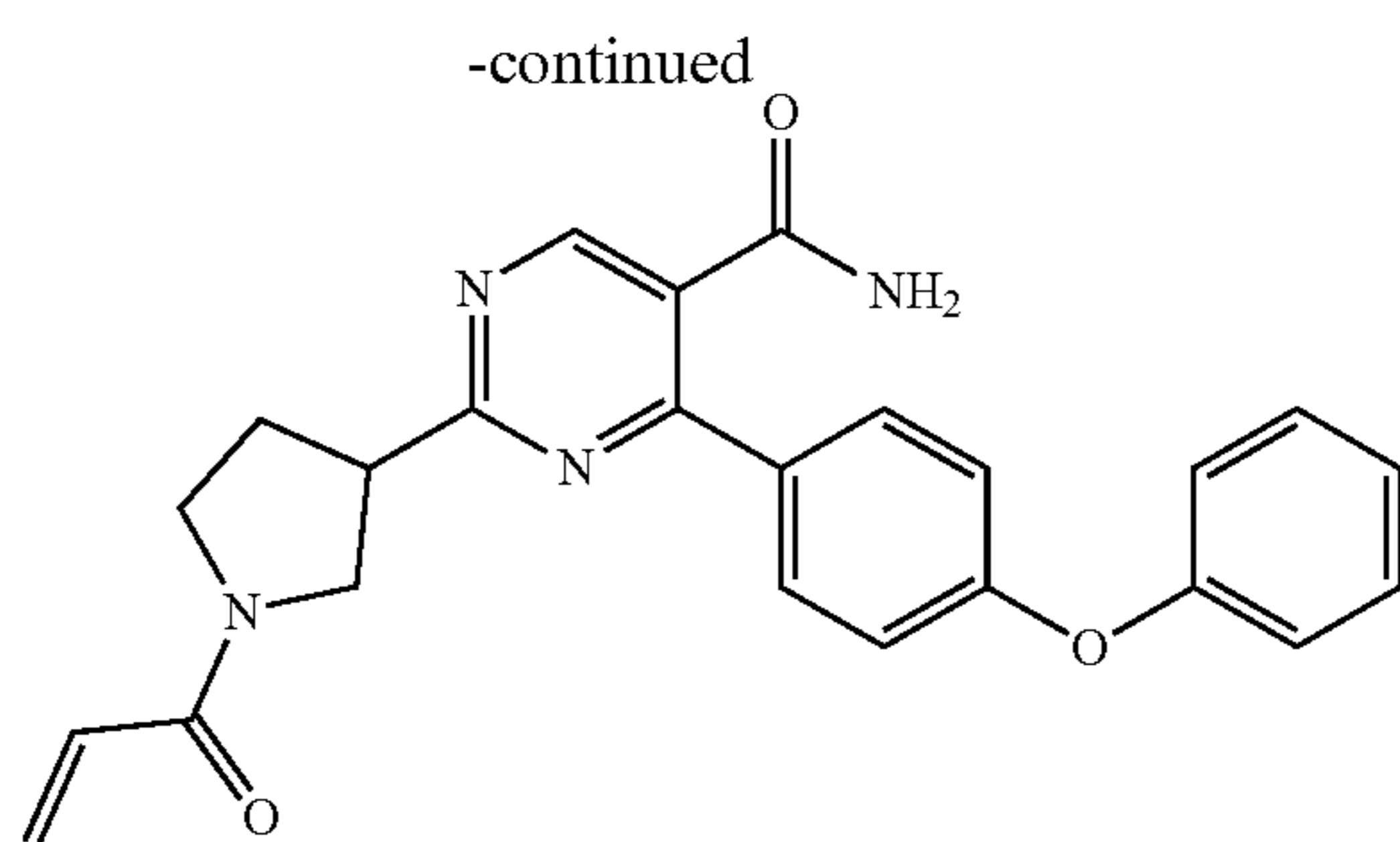
Example 22
