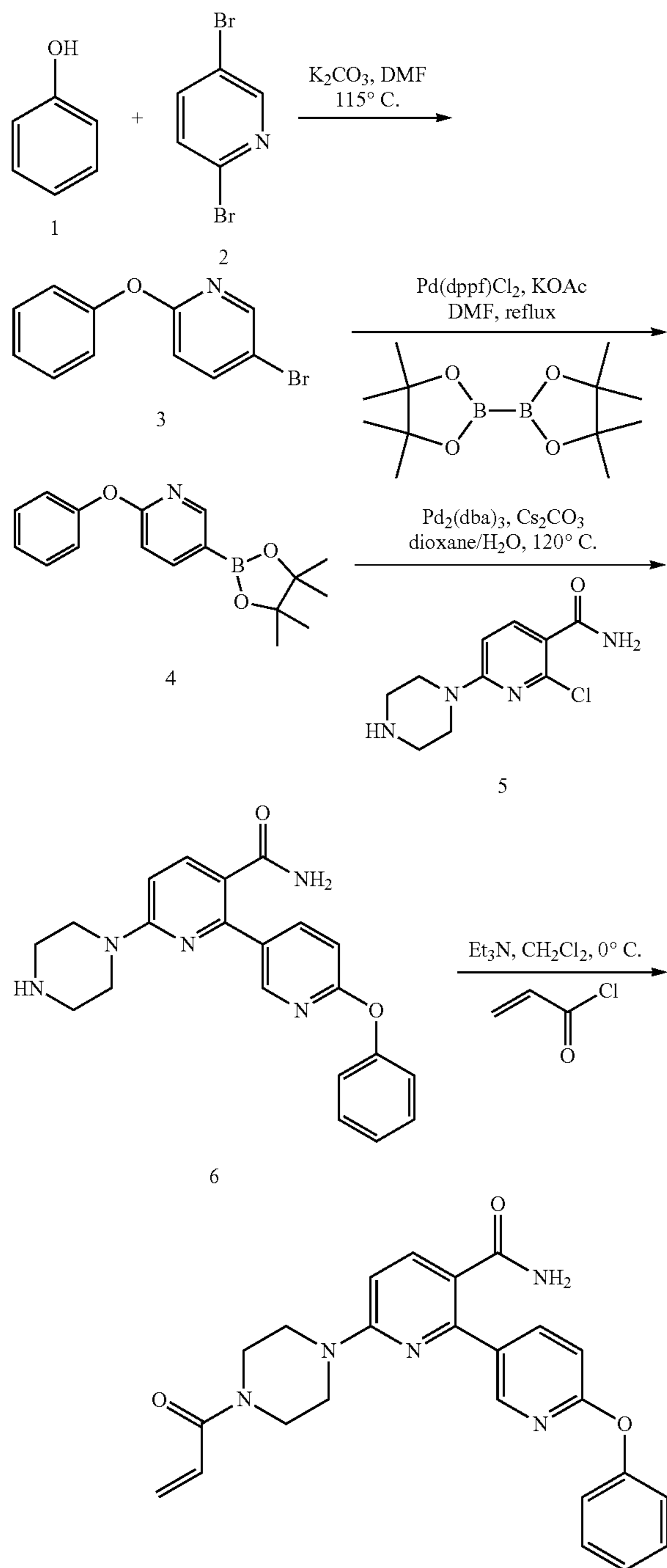
Example 31
