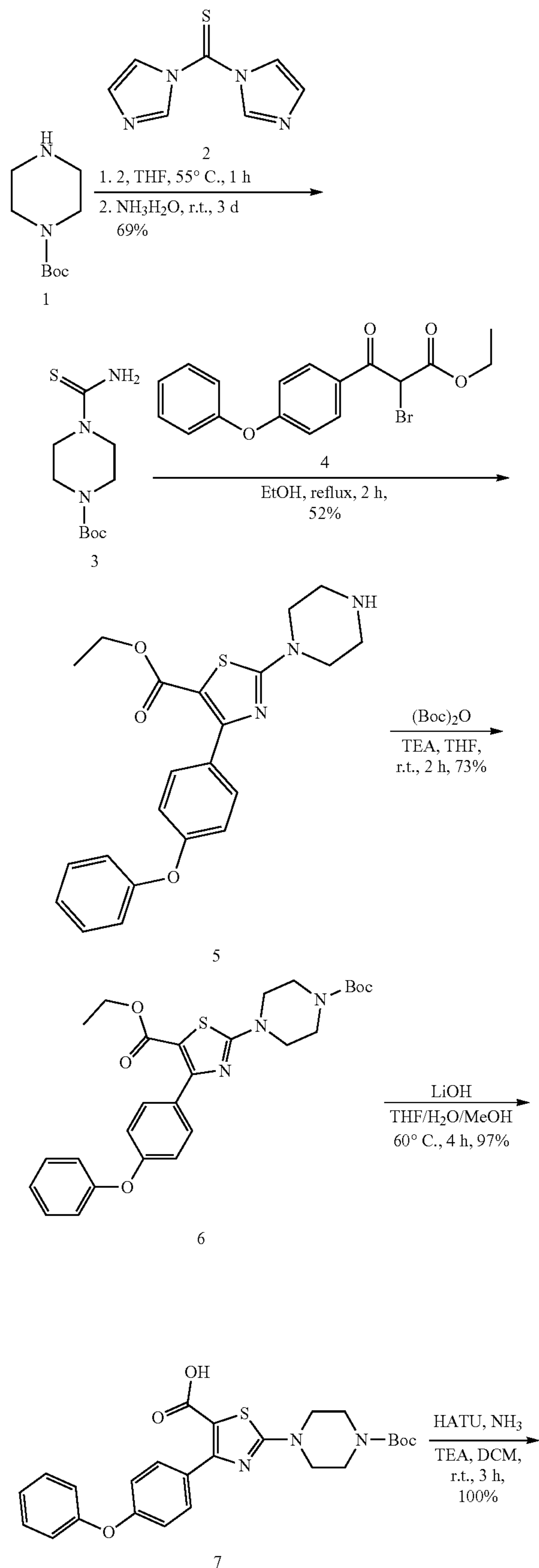
Scheme 41
