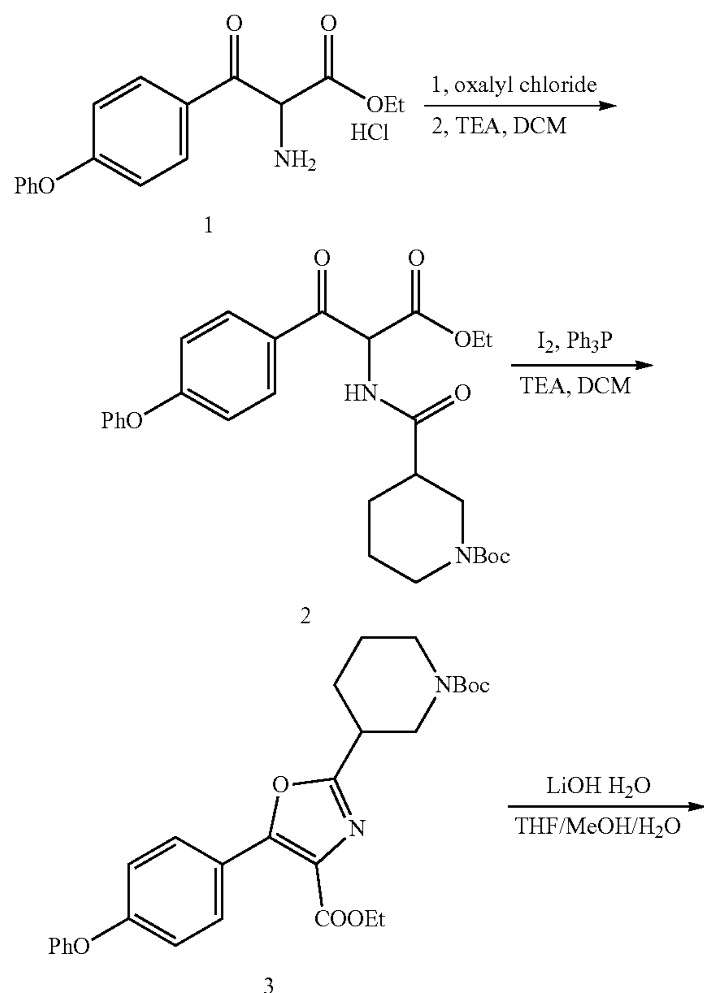
Scheme 44
