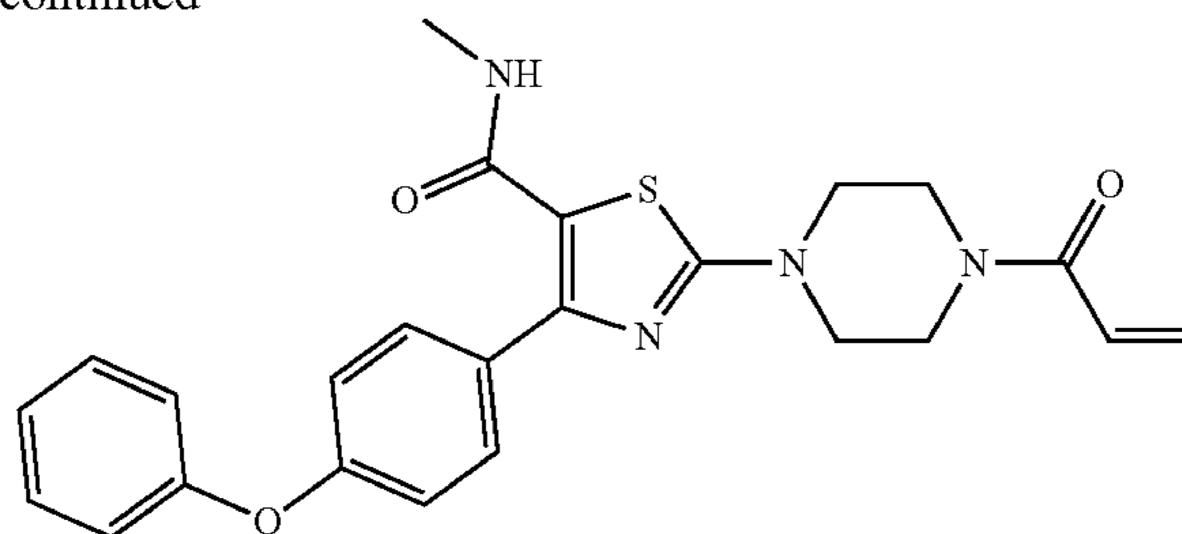
Example 47
