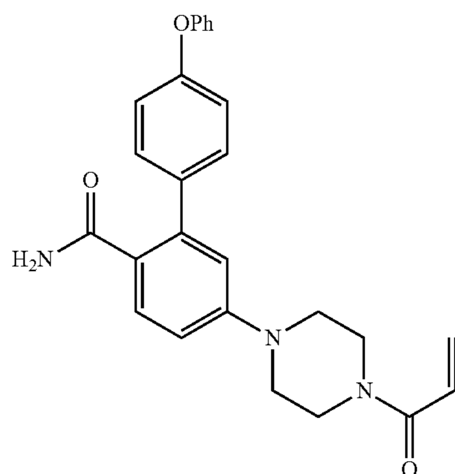
Example 57
