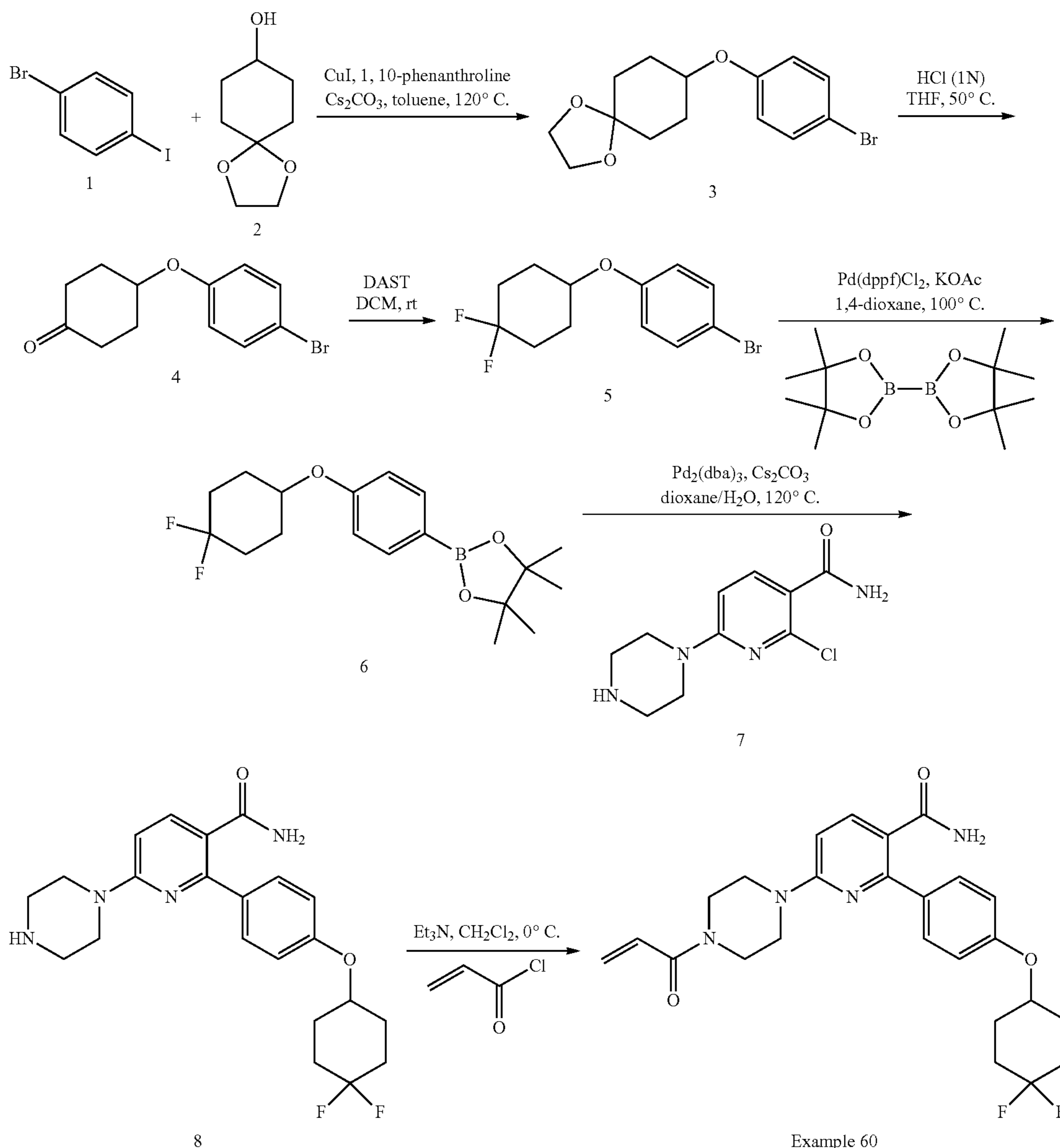
Scheme 50
