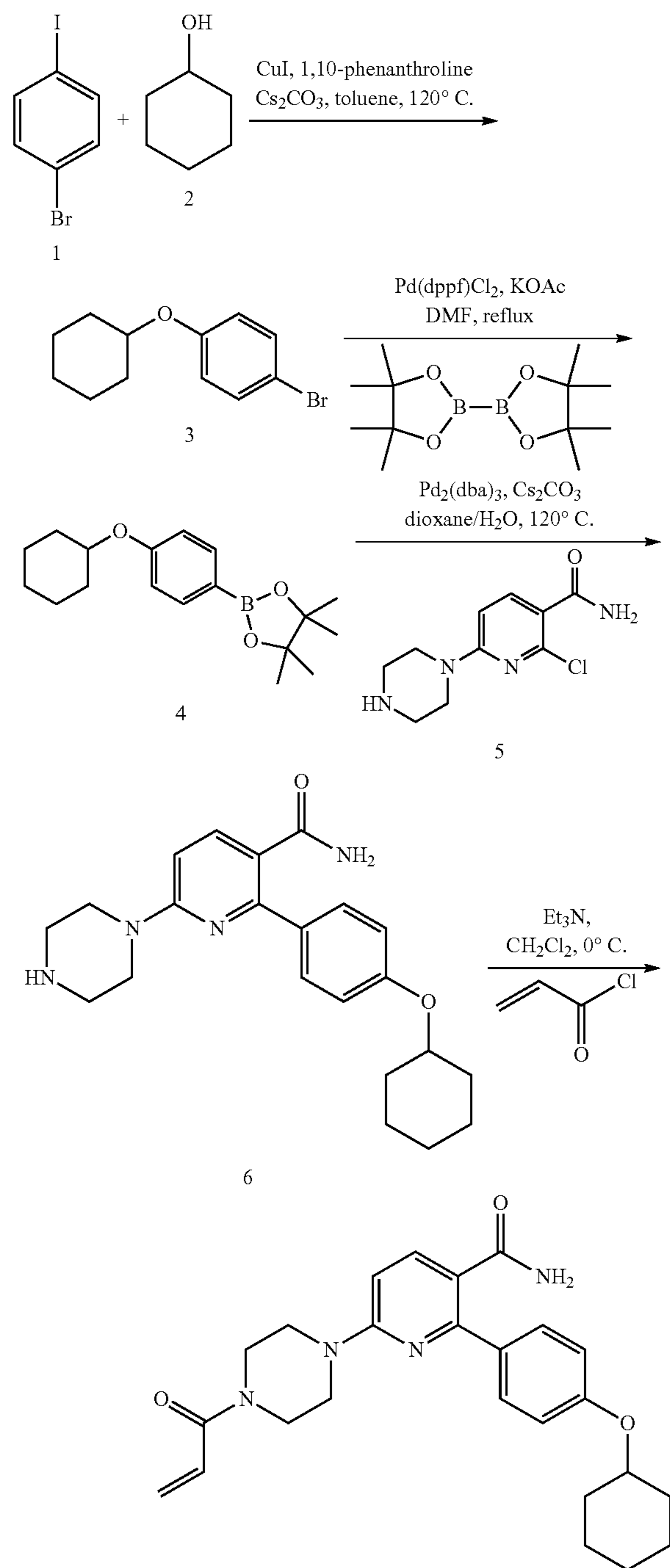
Example 28
