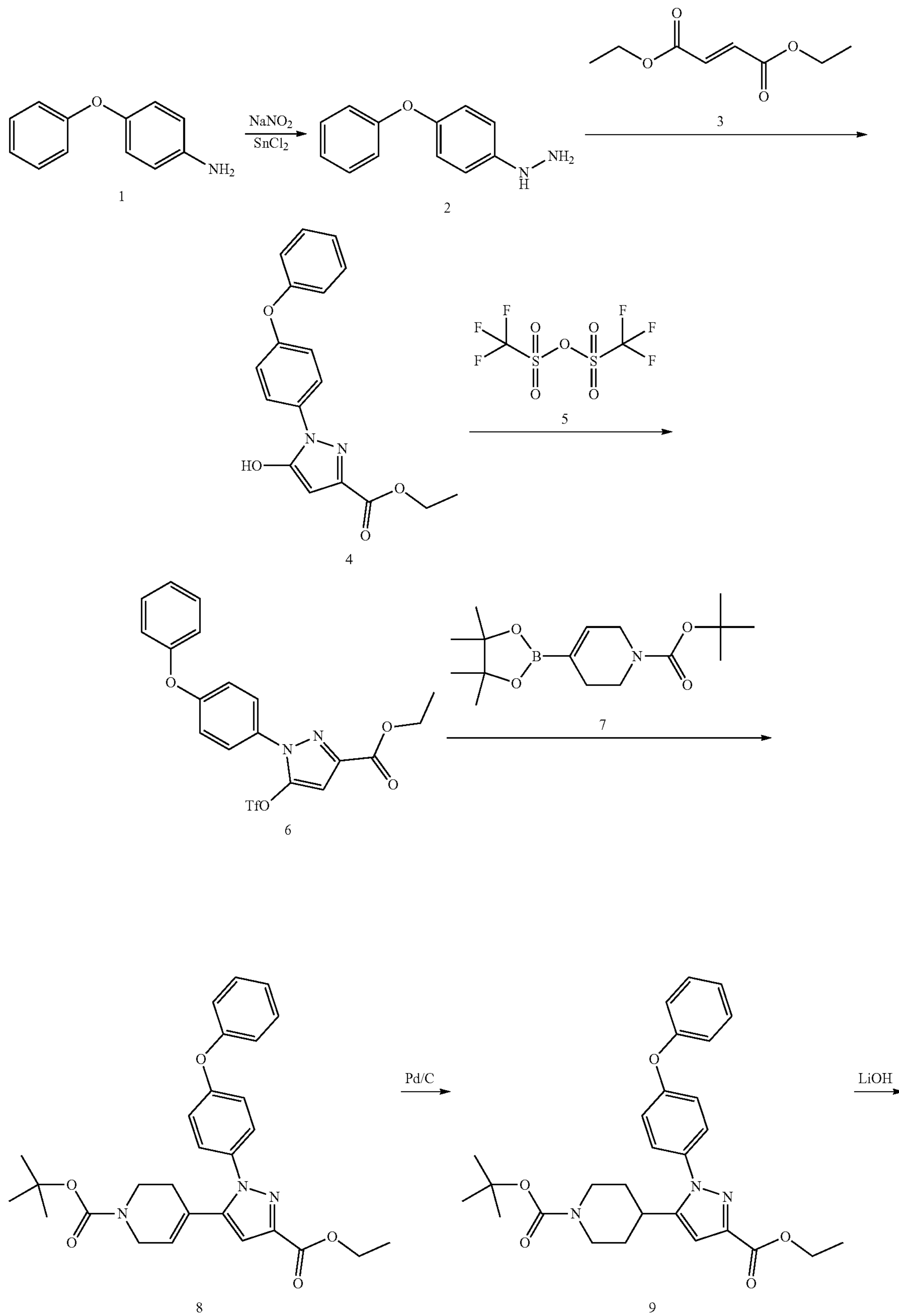
Scheme 46
