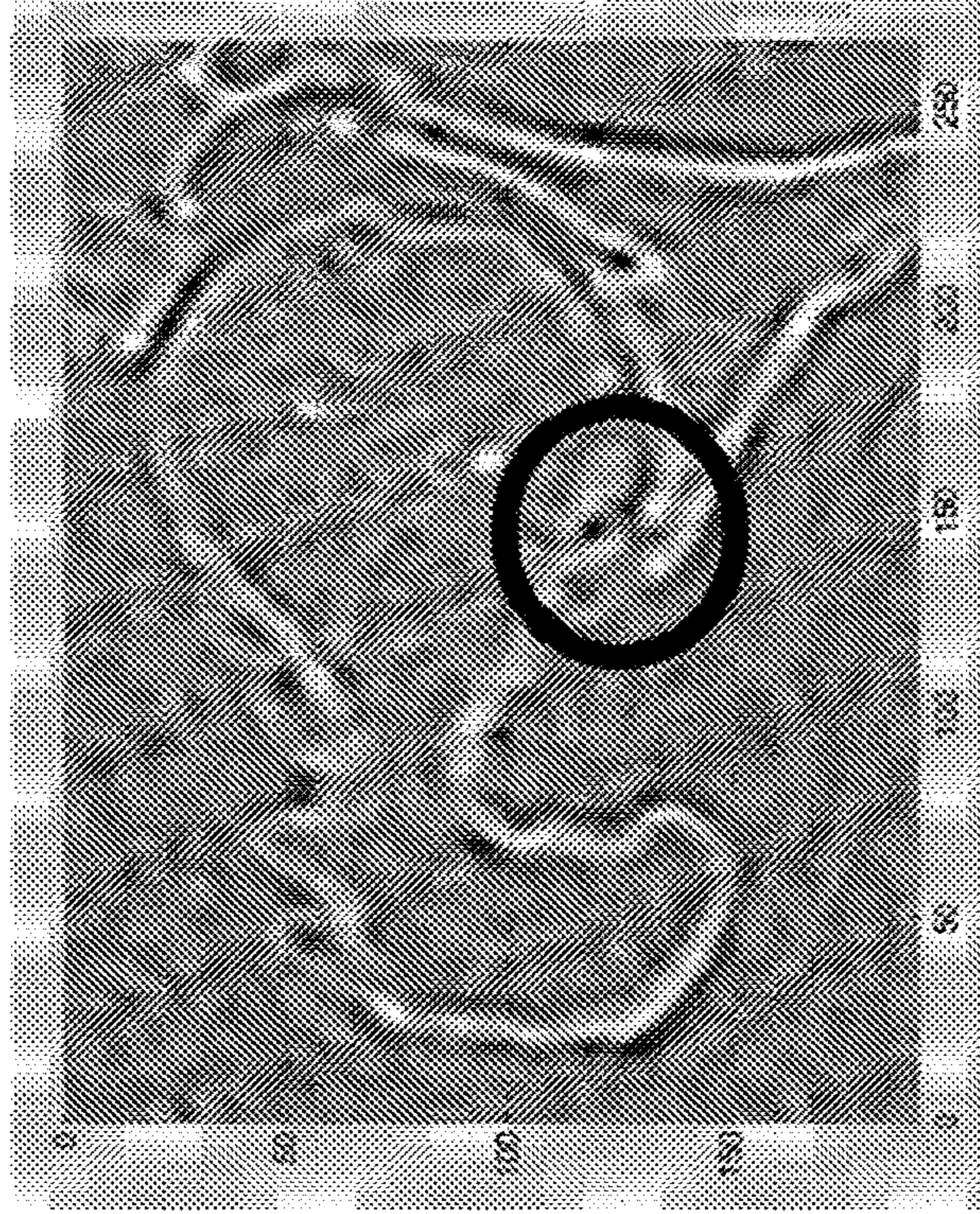
Hessian+ operation
