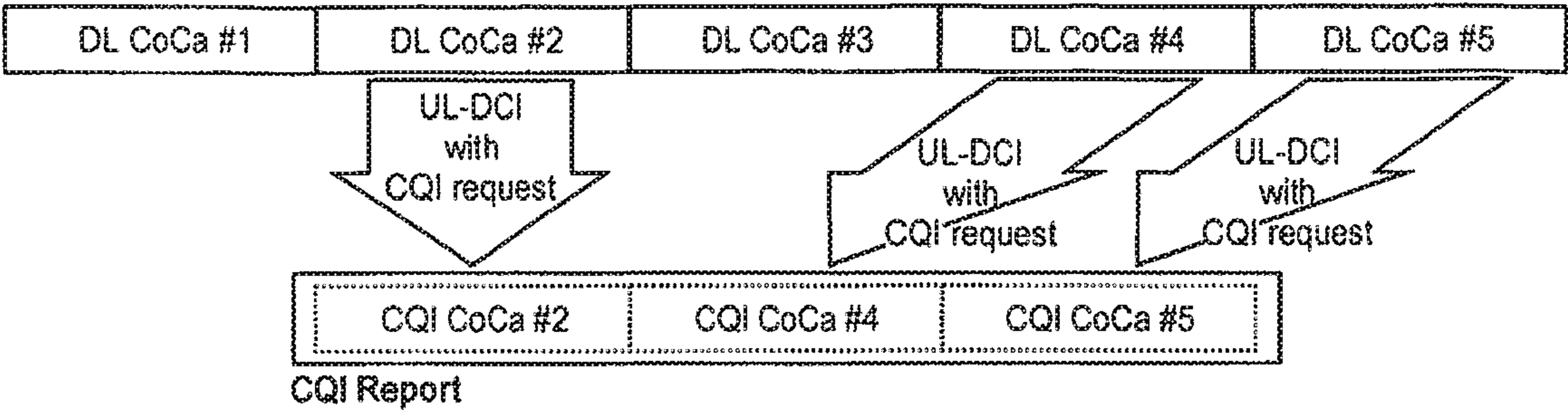
Fig. 5 (PRIOR ART)
