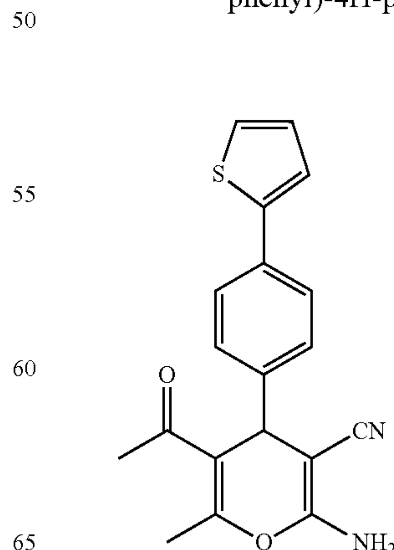
5-Acetyl-2-amino-6-methyl-4-(4-(thiophen-2-yl)phenyl)-4H-pyran-3-carbonitrile
