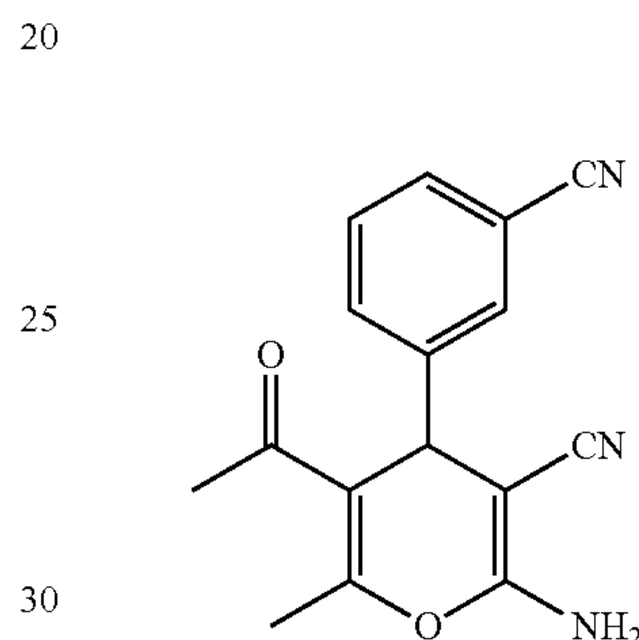
5-Acetyl-2-amino-4-(3-cyanophenyl)-6-methyl-4H-pyran-3-carbonitrile
