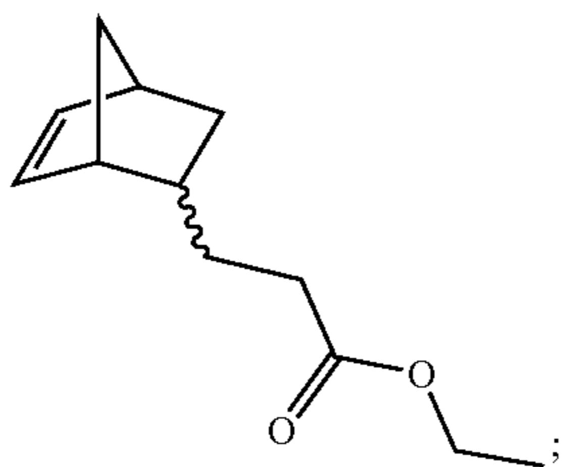
ethyl 3-(bicyclo[2.2.1]hept-5-en-2-yl)propanoate (EPEsNB)
