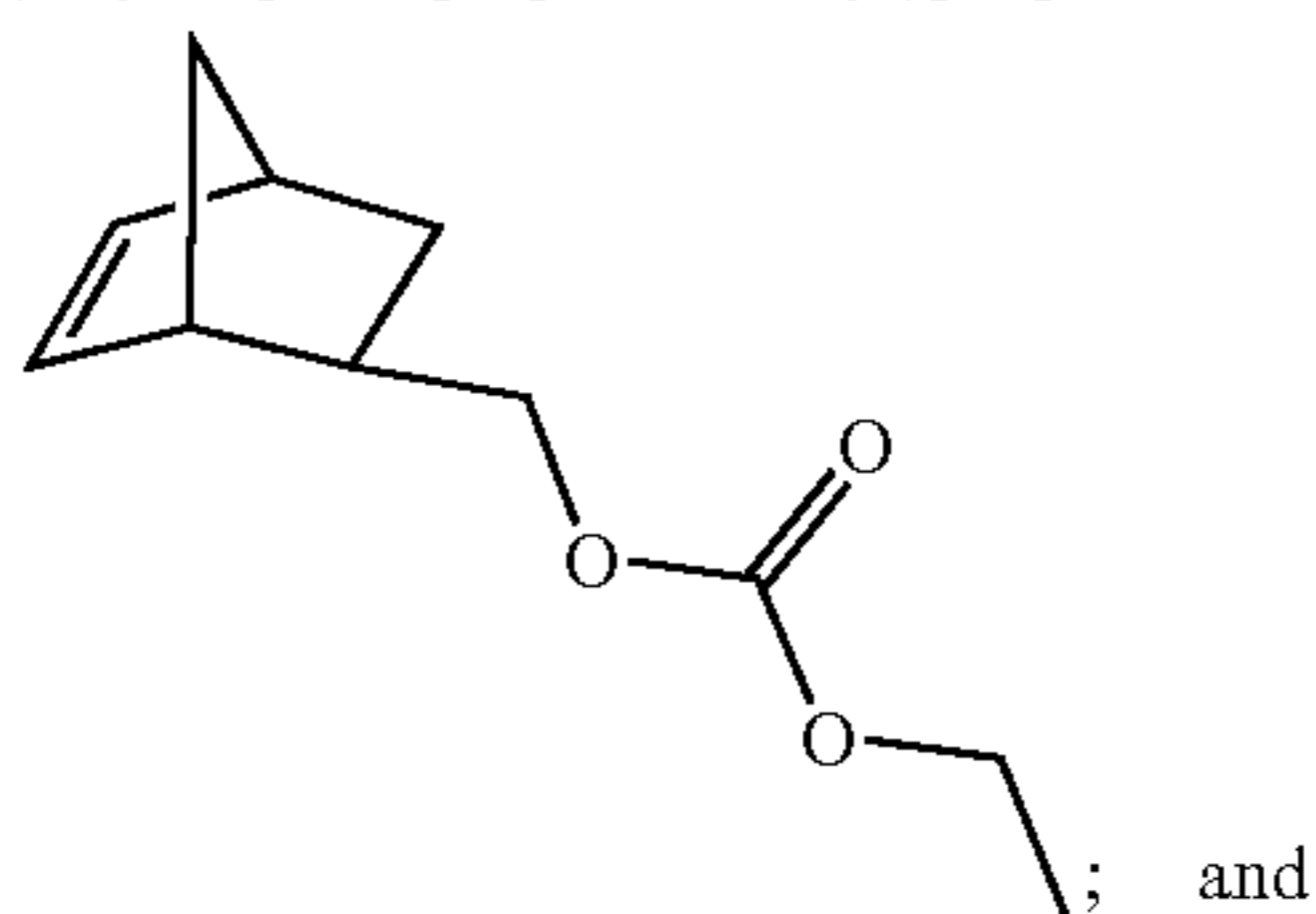
(bicyclo[2.2.1]hept-5-en-2-yl)methyl ethyl carbonate (NBEtCarb)
