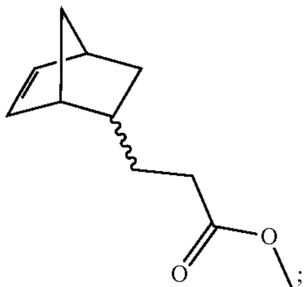
methyl 3-(bicyclo[2.2.1]hept-5-en-2-yl)propanoate (MPEsNB)
