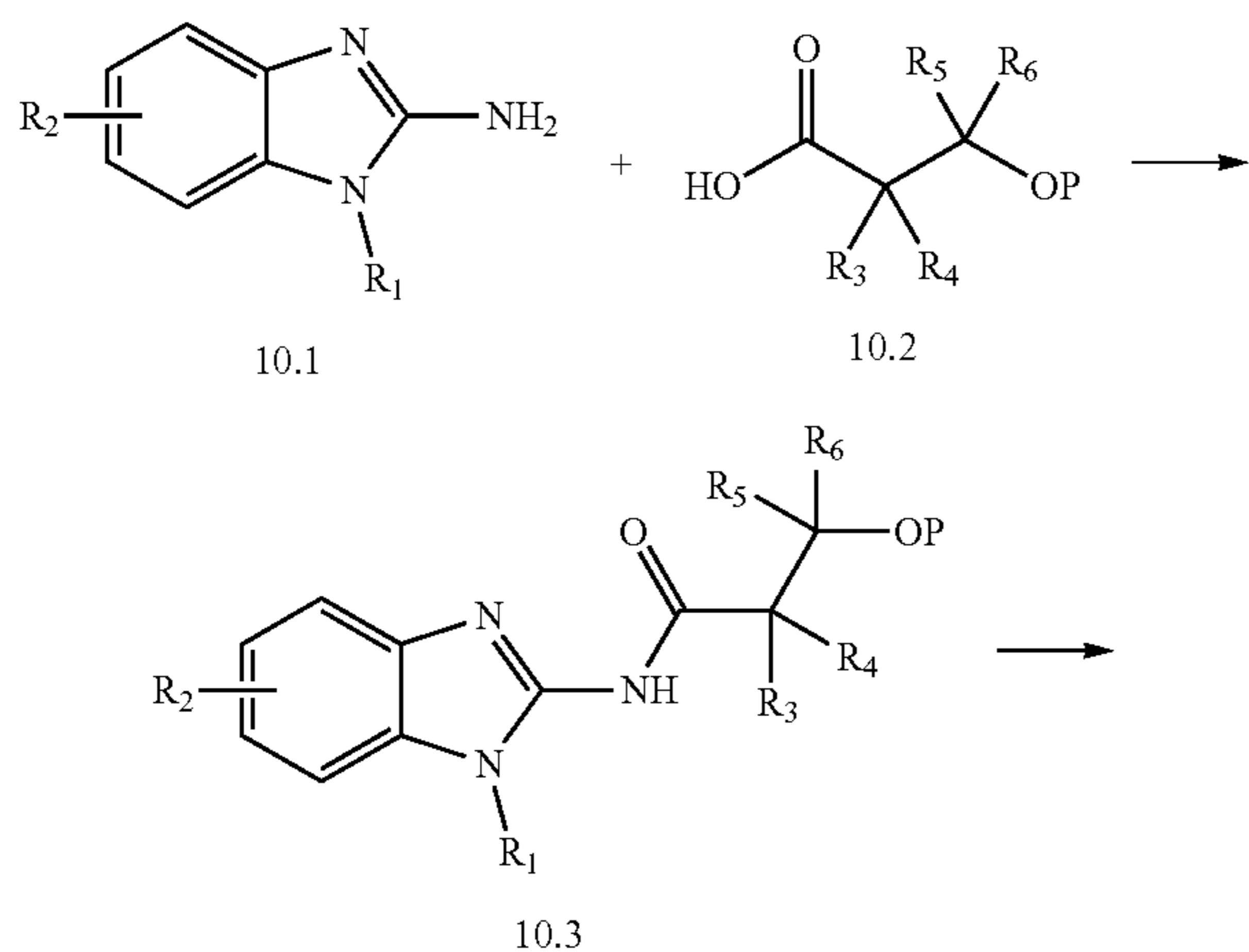
Scheme 10
