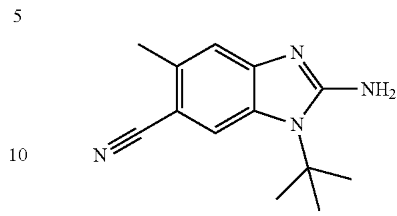
2-amino-1-(tert-butyl)-5-methyl-1H-benzo[d]imidazole-6-carbonitrile
