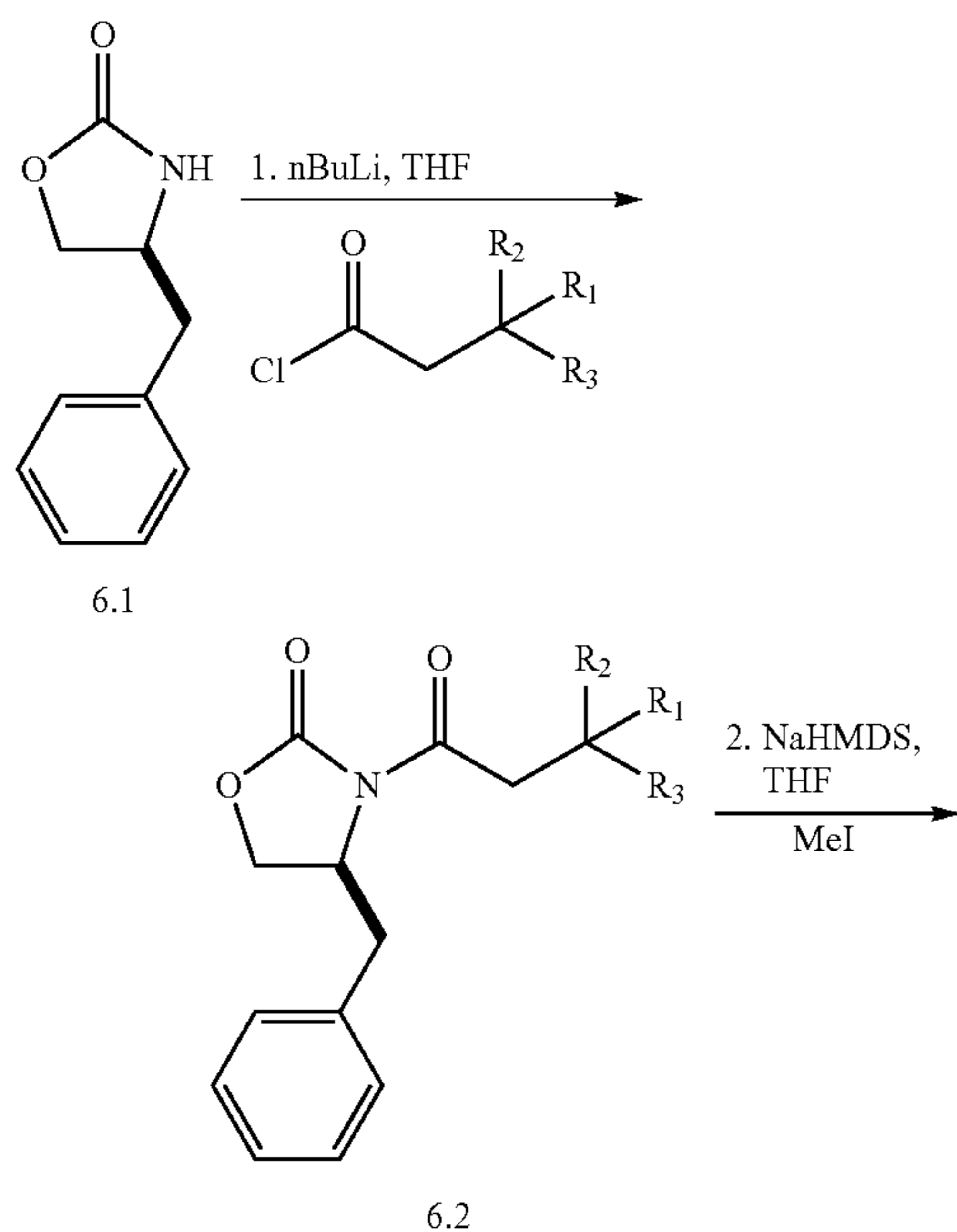
Scheme 6
