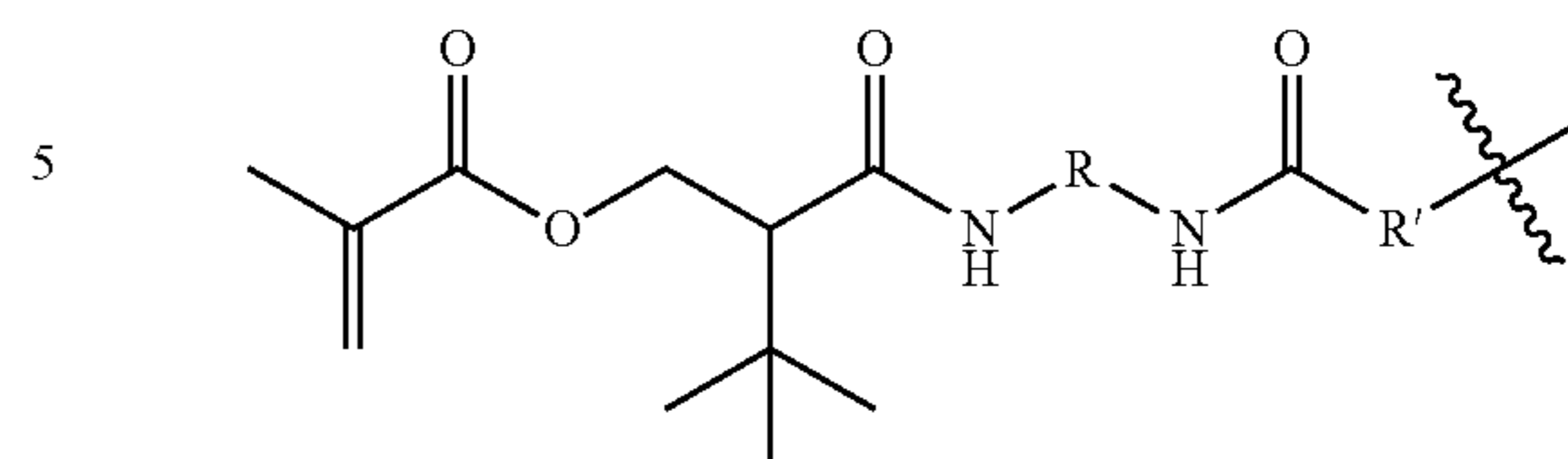
Formula (XI)
