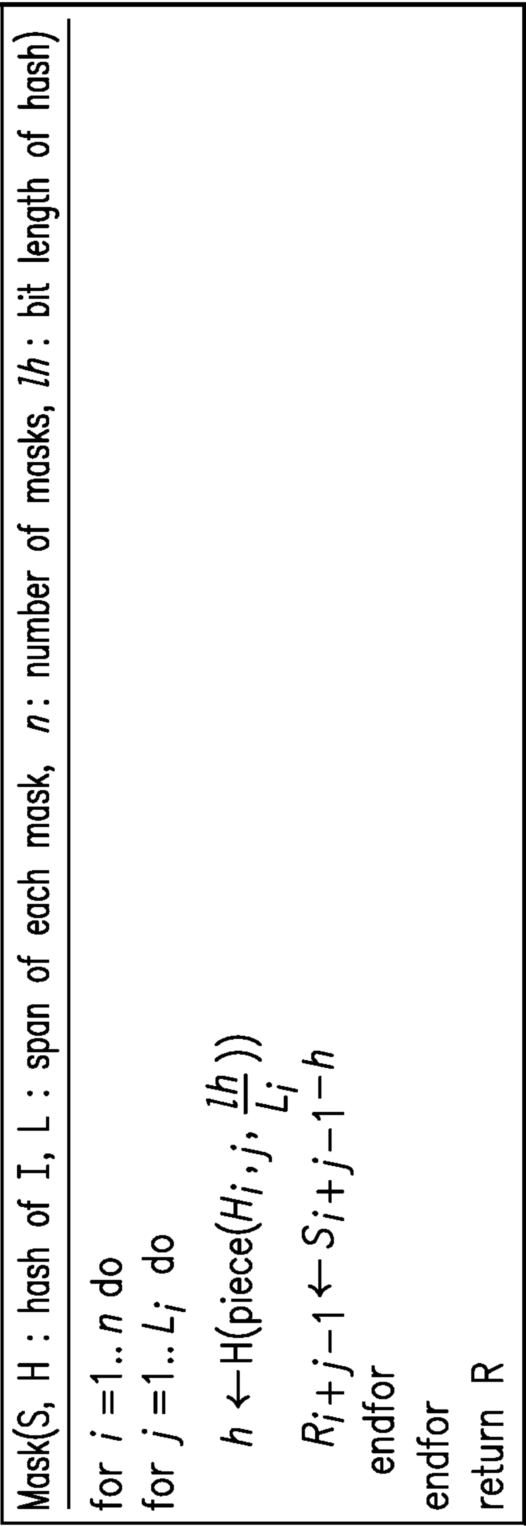
Masking algorithm
