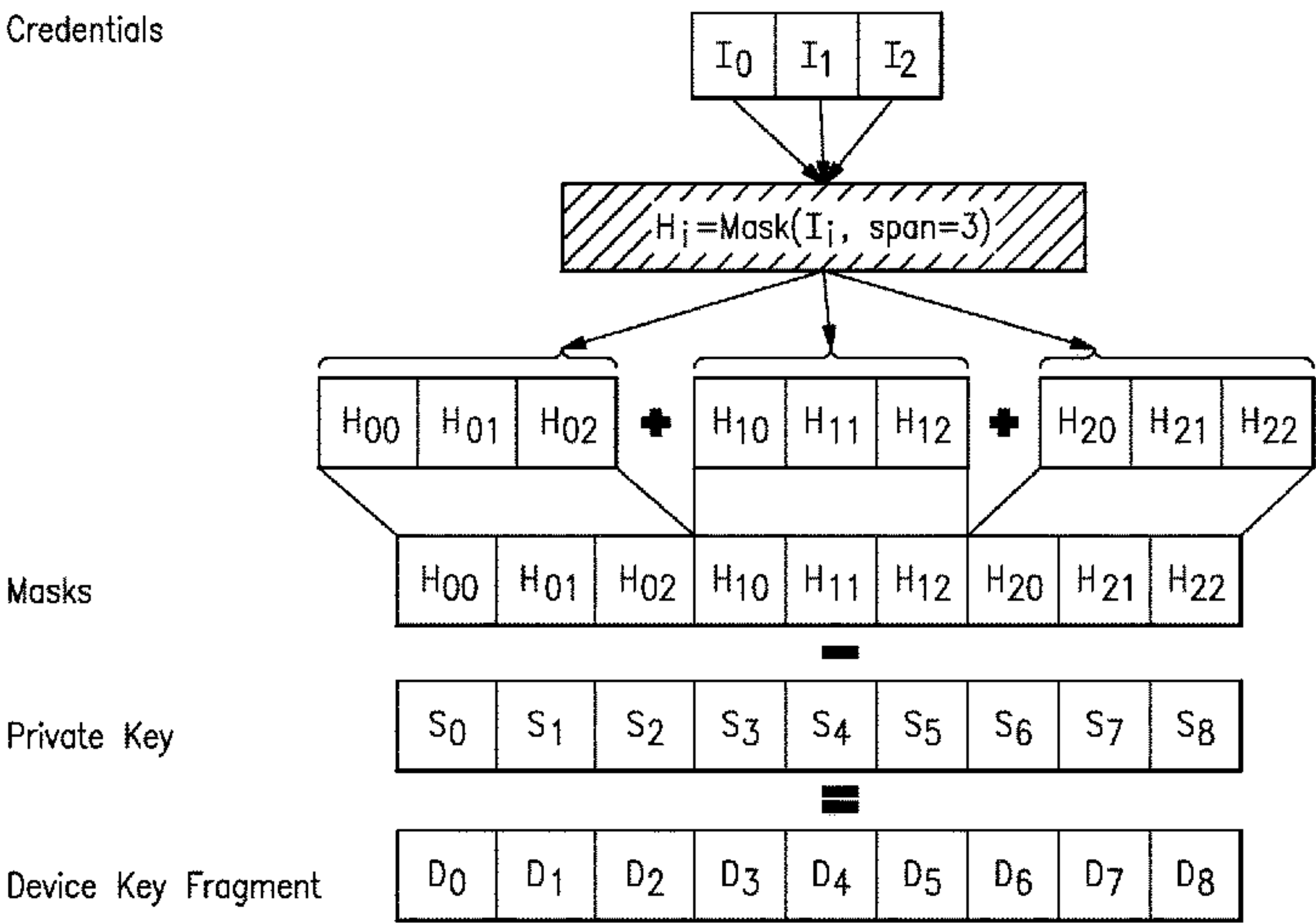
An diagram showing how device key fragments are generated from credentials and ZKP private keys
