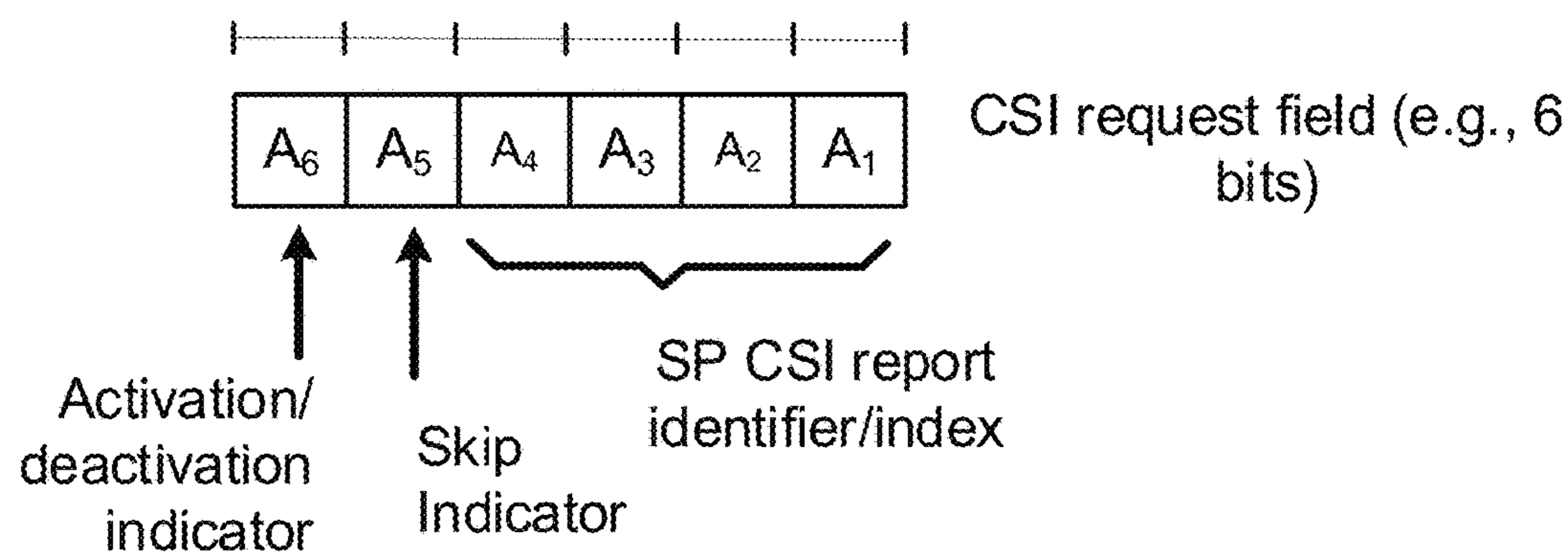
1-bit indicators for SP CSI activation/deactivation and skip indicator
