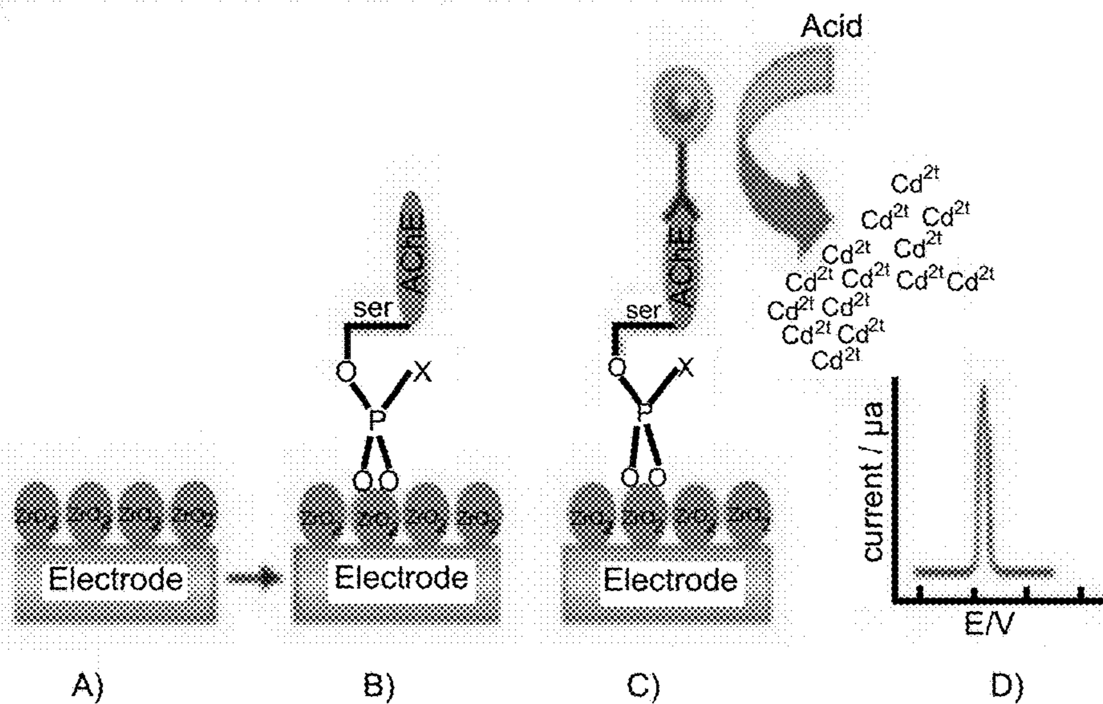
Figure: Example detection using an electrode
