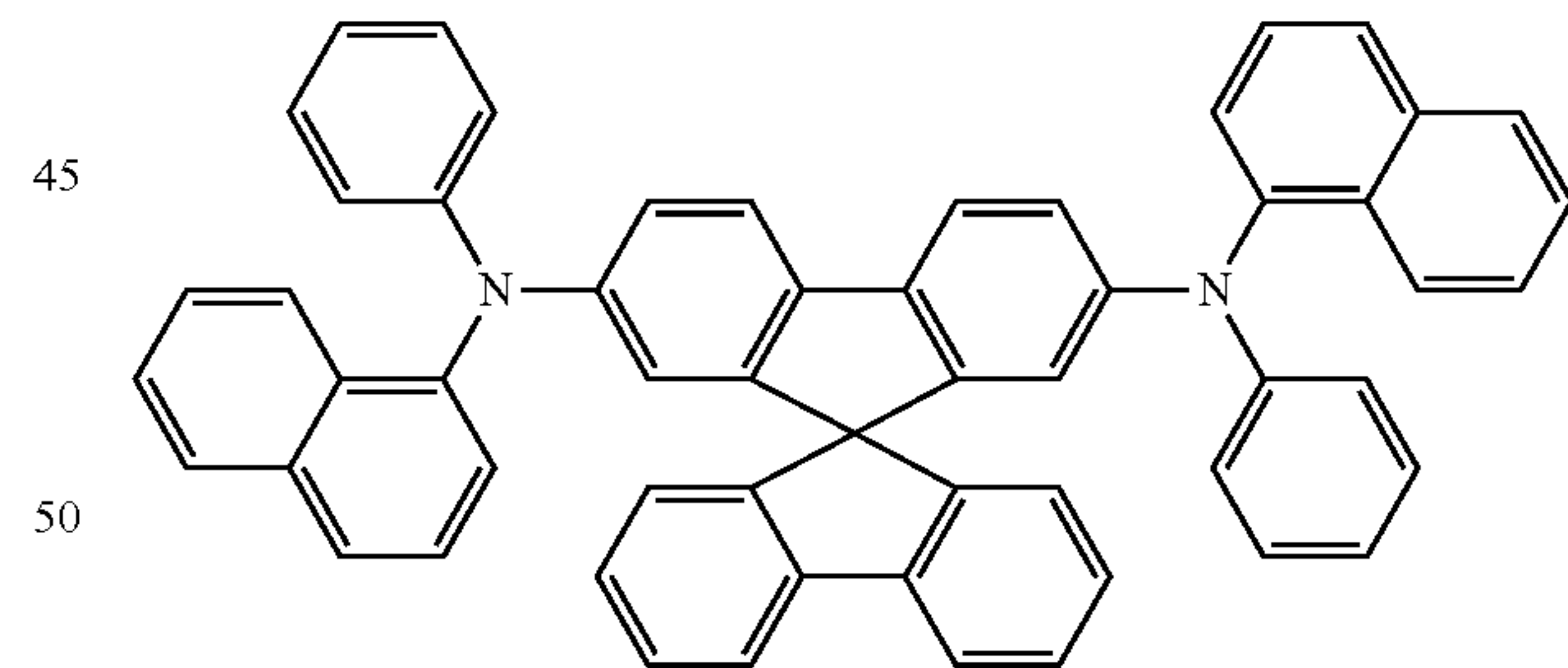
Spiro-NPB
