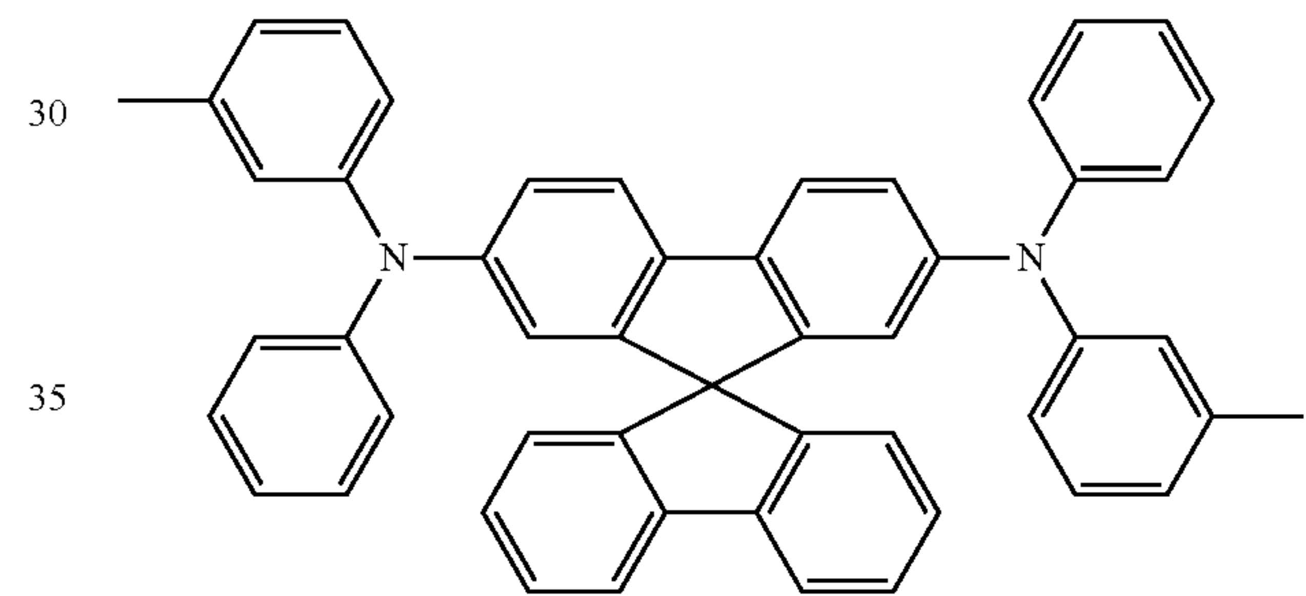
Spiro-TPD
