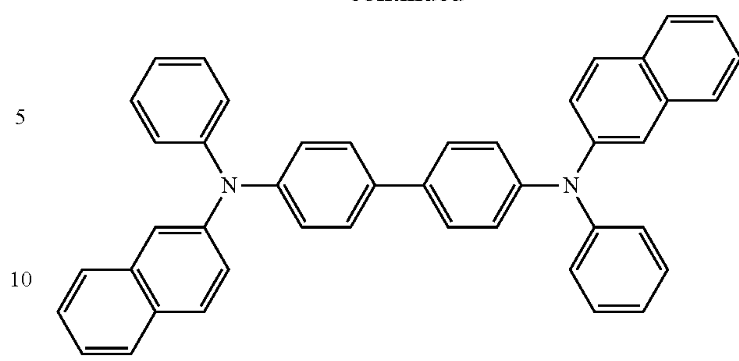
\beta -NPB
