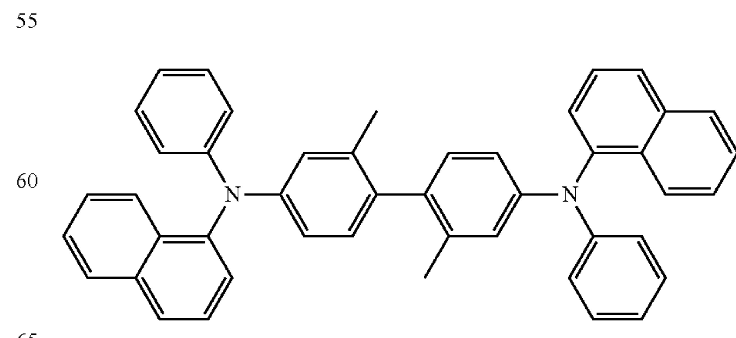
methylated NPB
