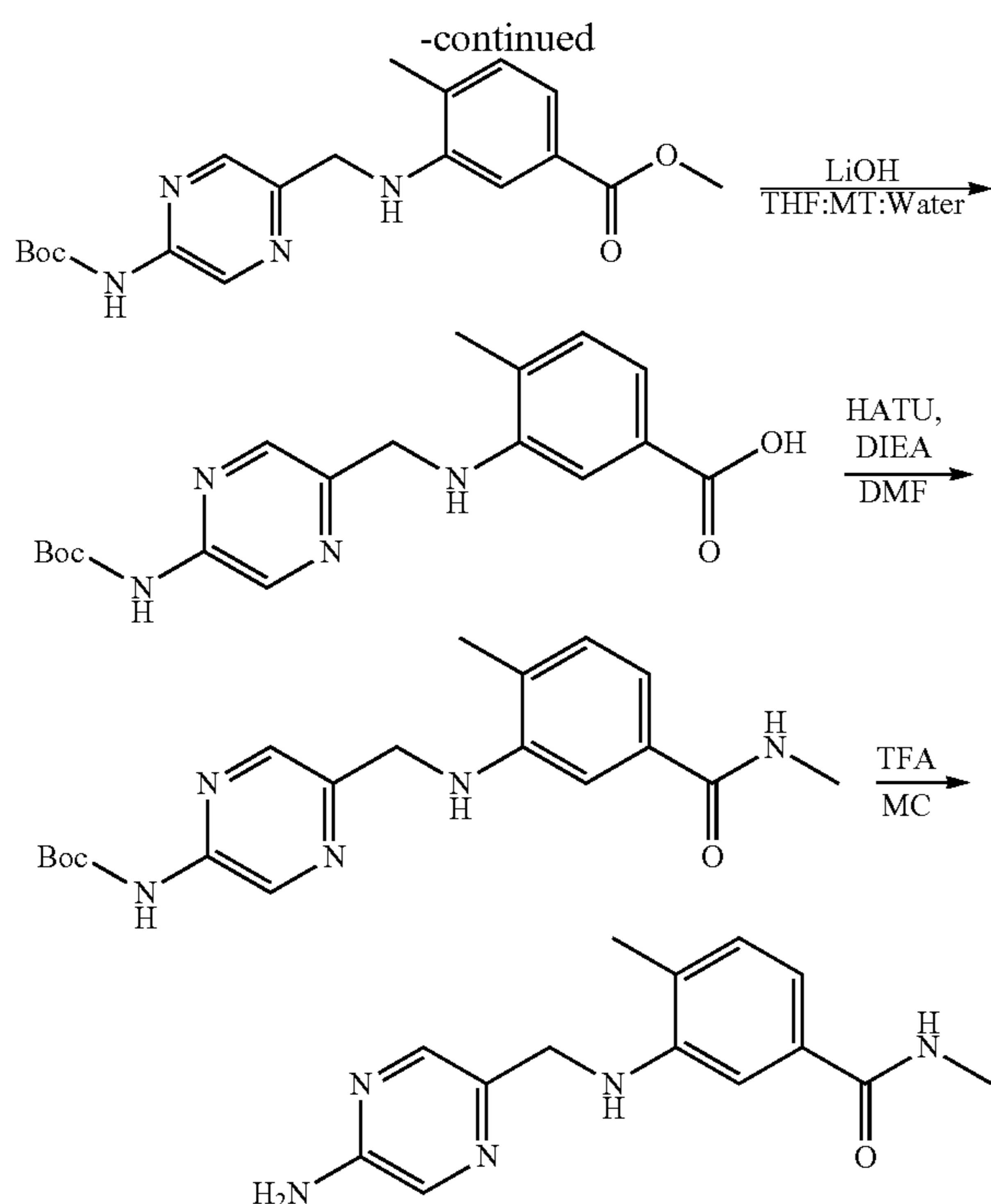
A. Methyl 3-((5-(tert-butoxycarbonylamino)pyrazin-2-yl)methylamino)-4-methylbenzoate
