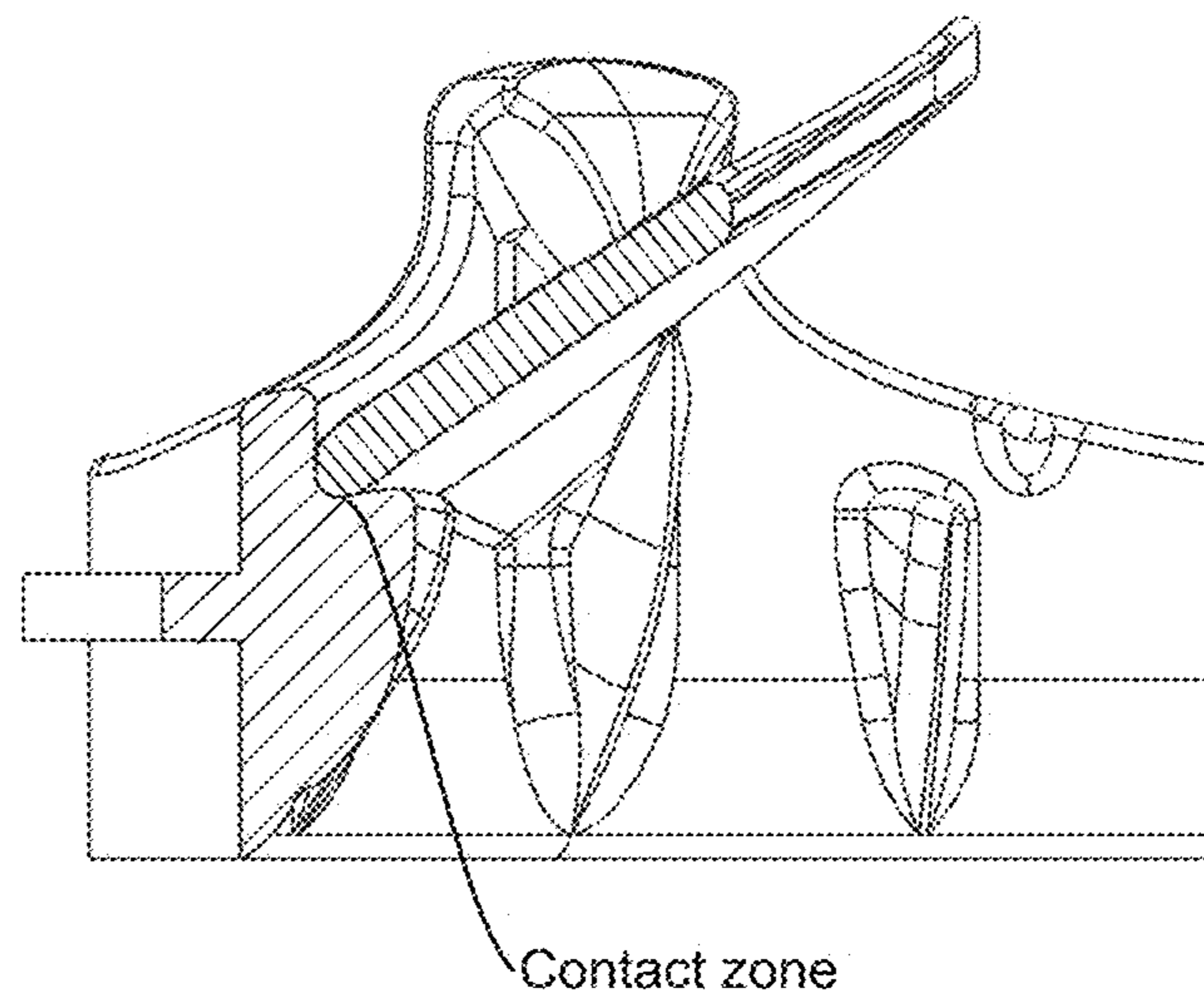
Fig. 14 - prior art
