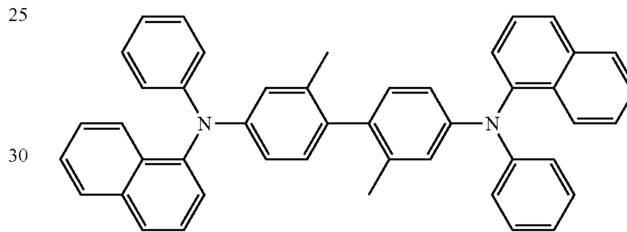
methylated NPD
