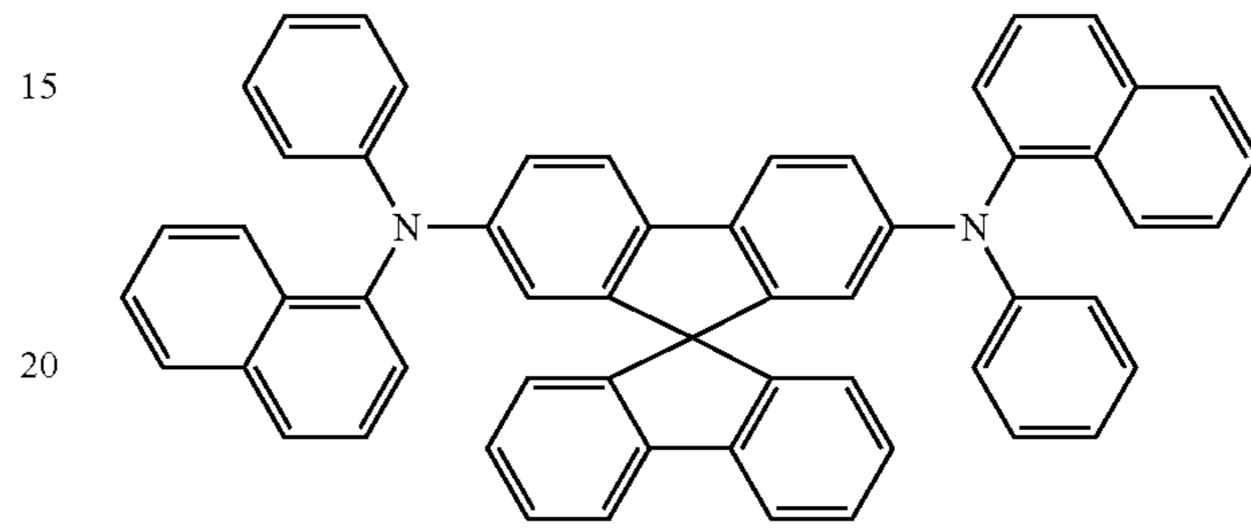
Spiro-NPB
