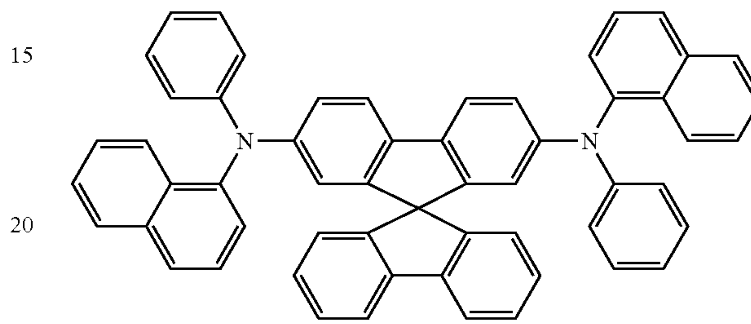
Spiro-NPB
