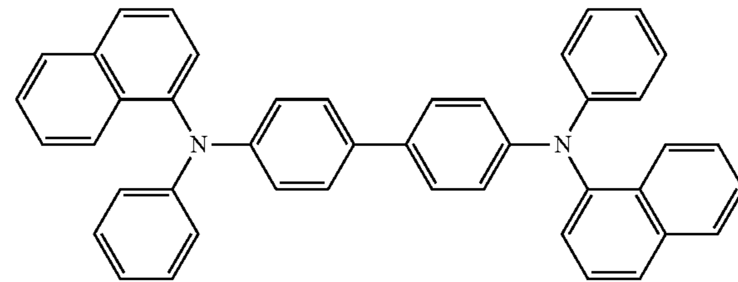
NPB
