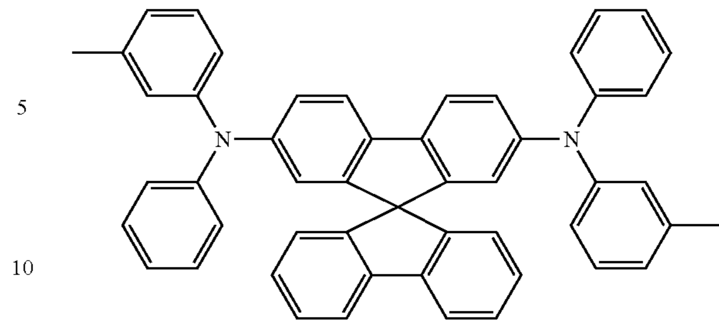
Spiro-TPD
