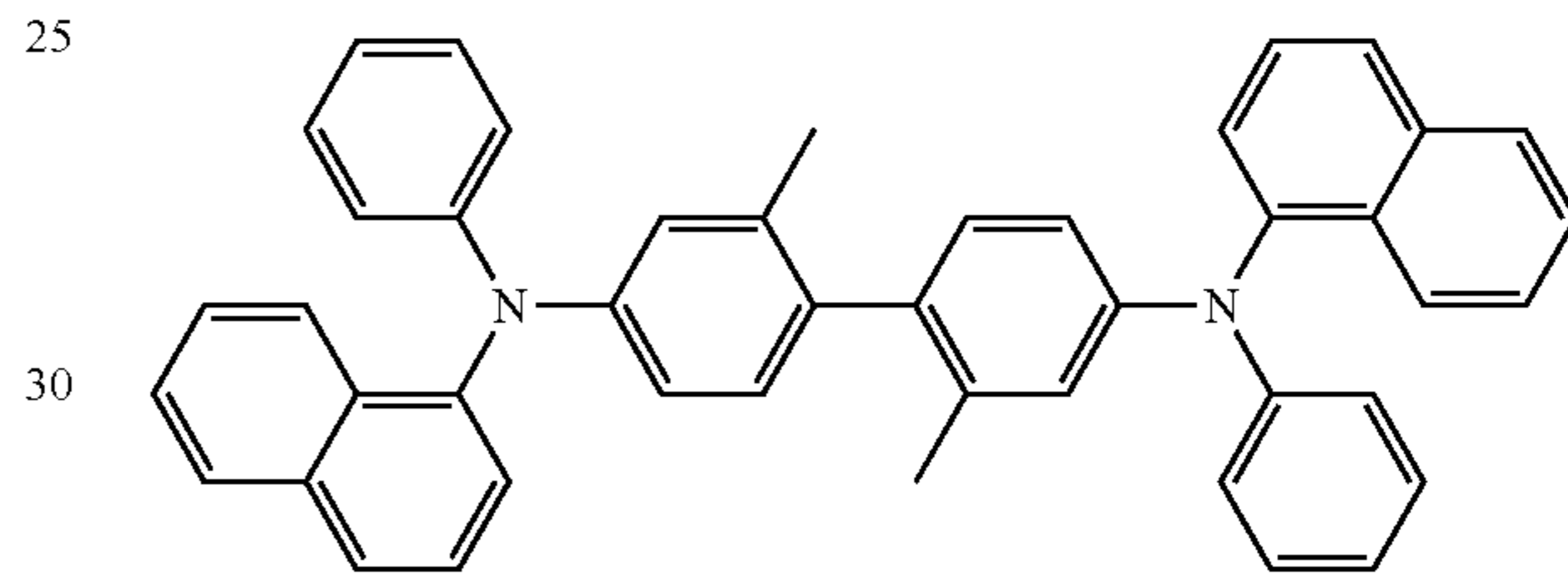
methylated NPD
