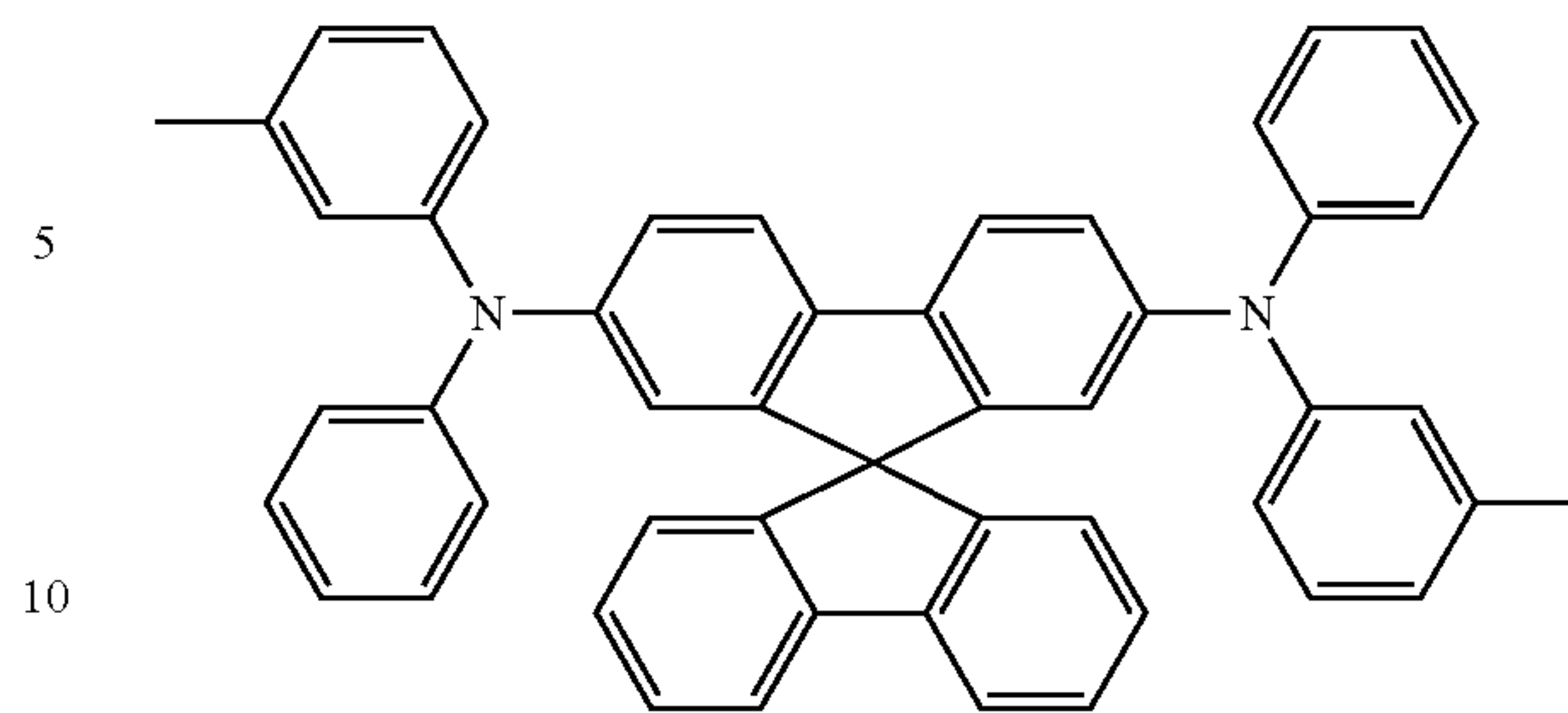
Spiro-TPD
