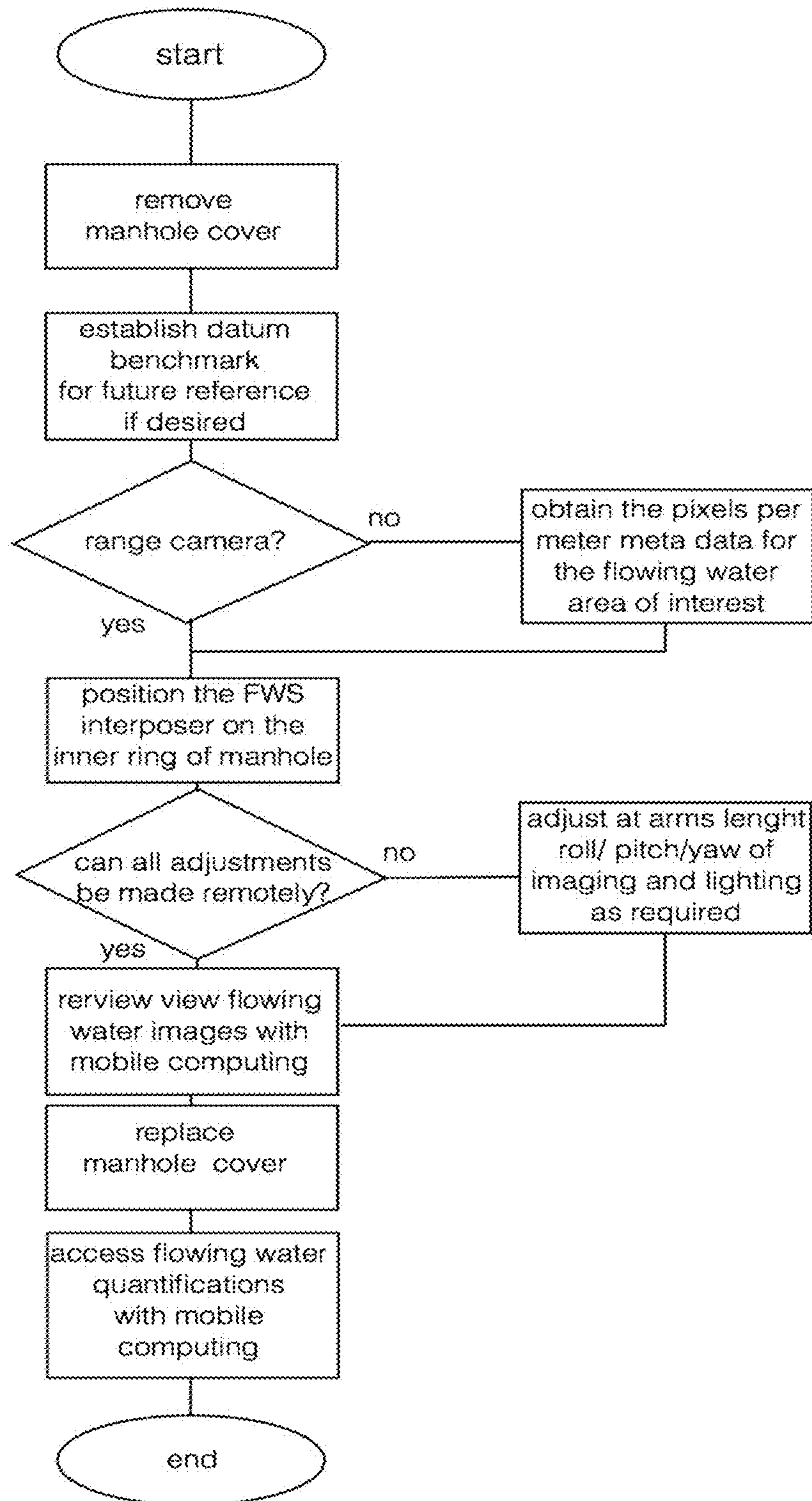
FWS process for manhole installation
