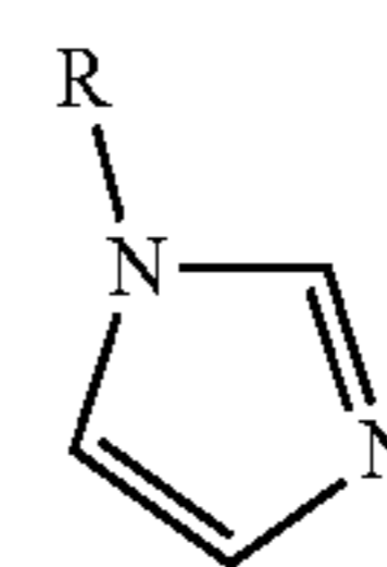
imidazole
