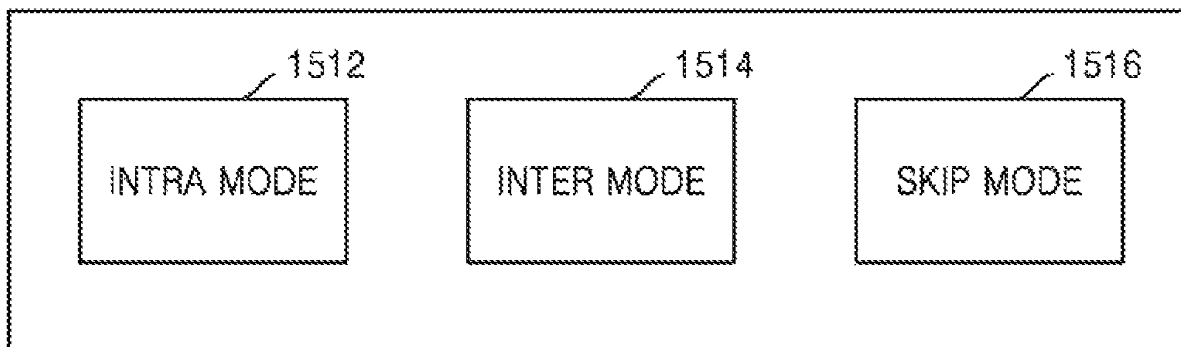
PREDICTION MODE (1510)
