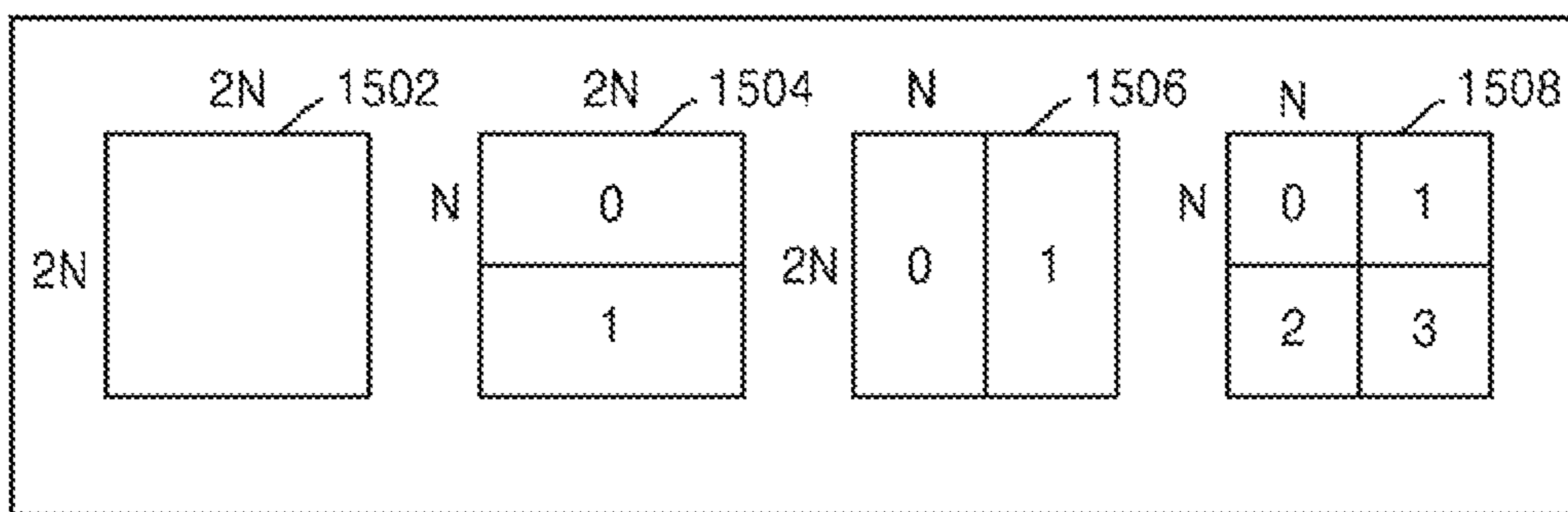
PARTITION MODE (1500)
