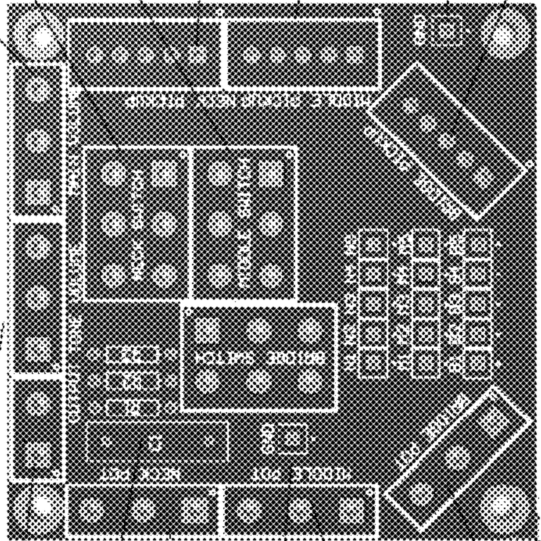
Series / Parallel Printed PCB
