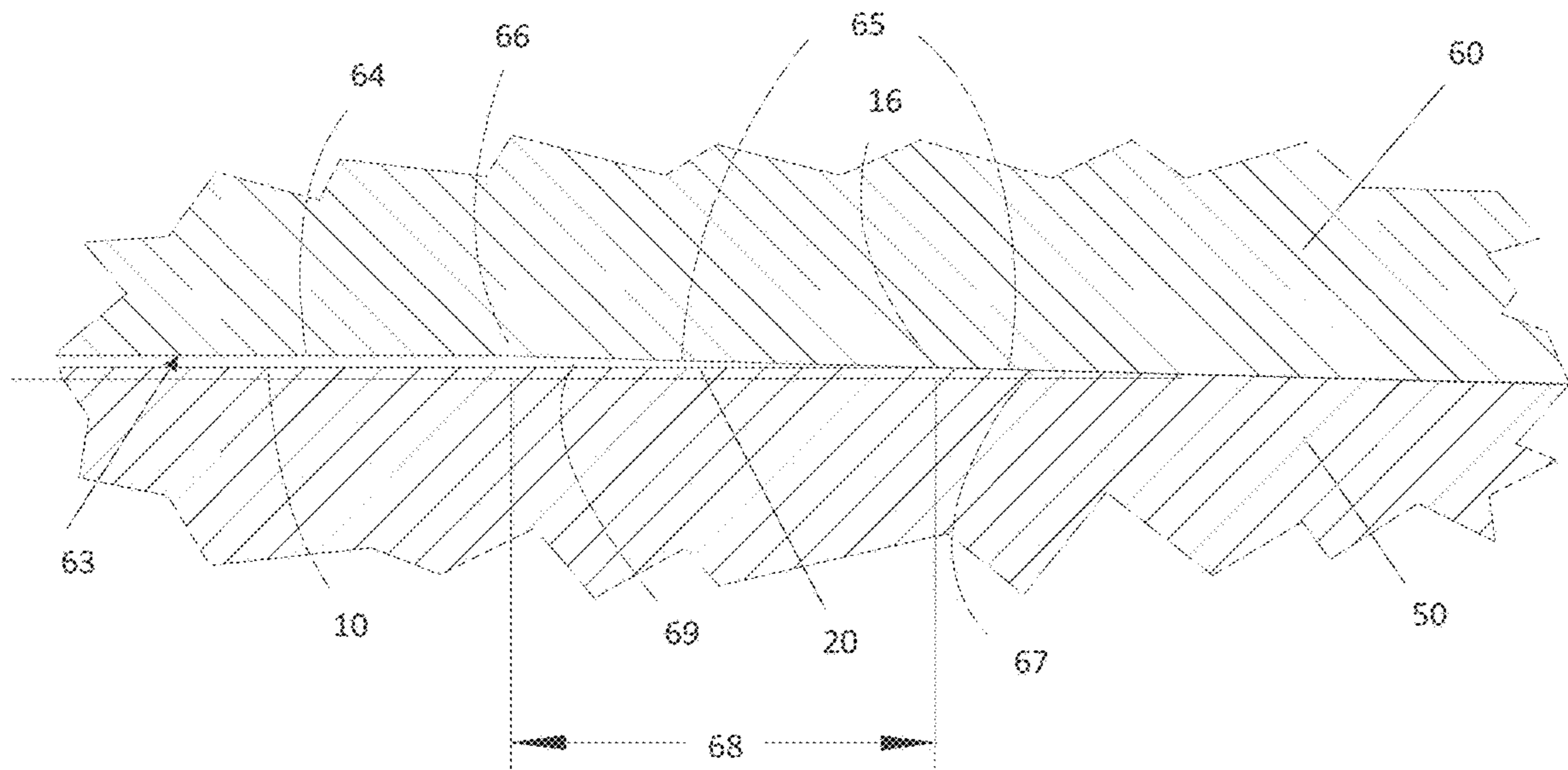
FIGURE 5 (PRIOR ART)
