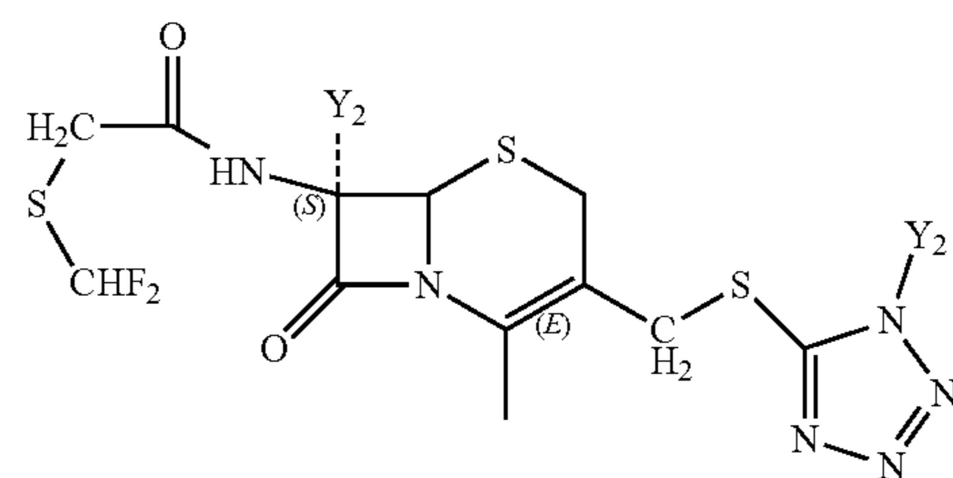
Structure FP-56
