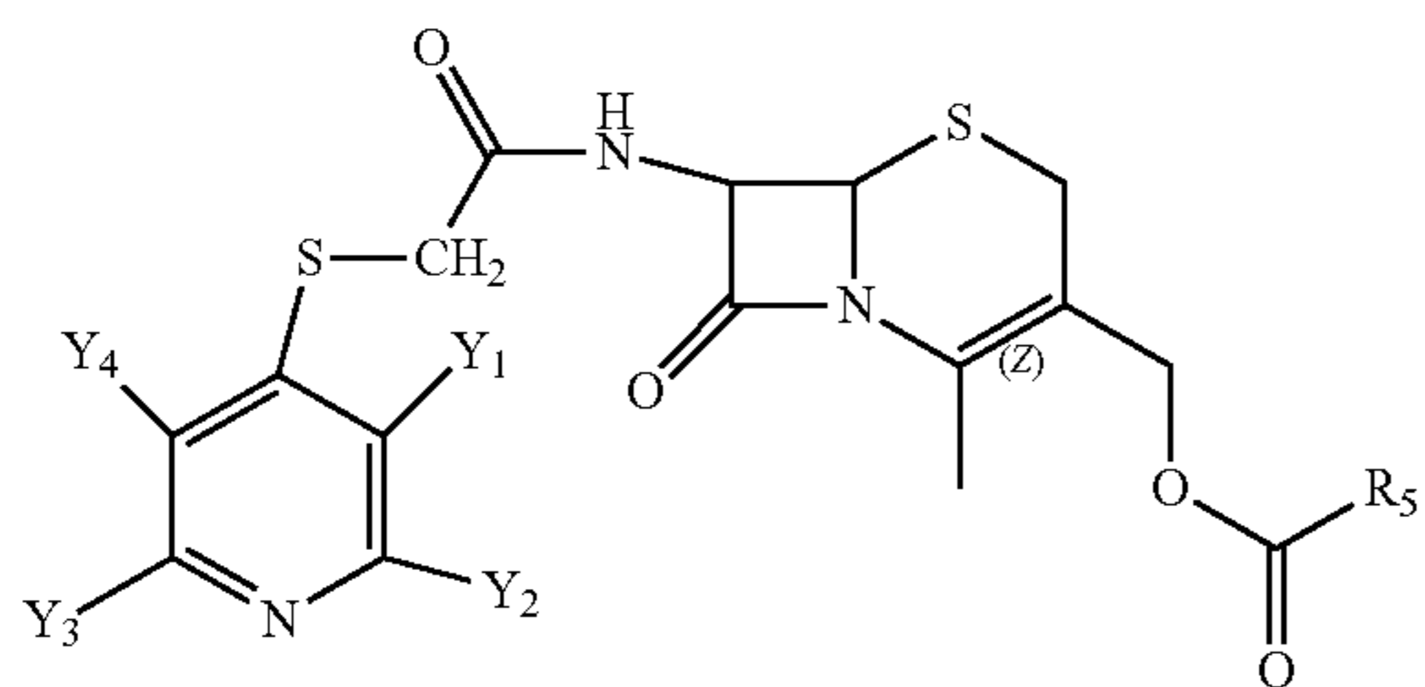
Structure FP-59
