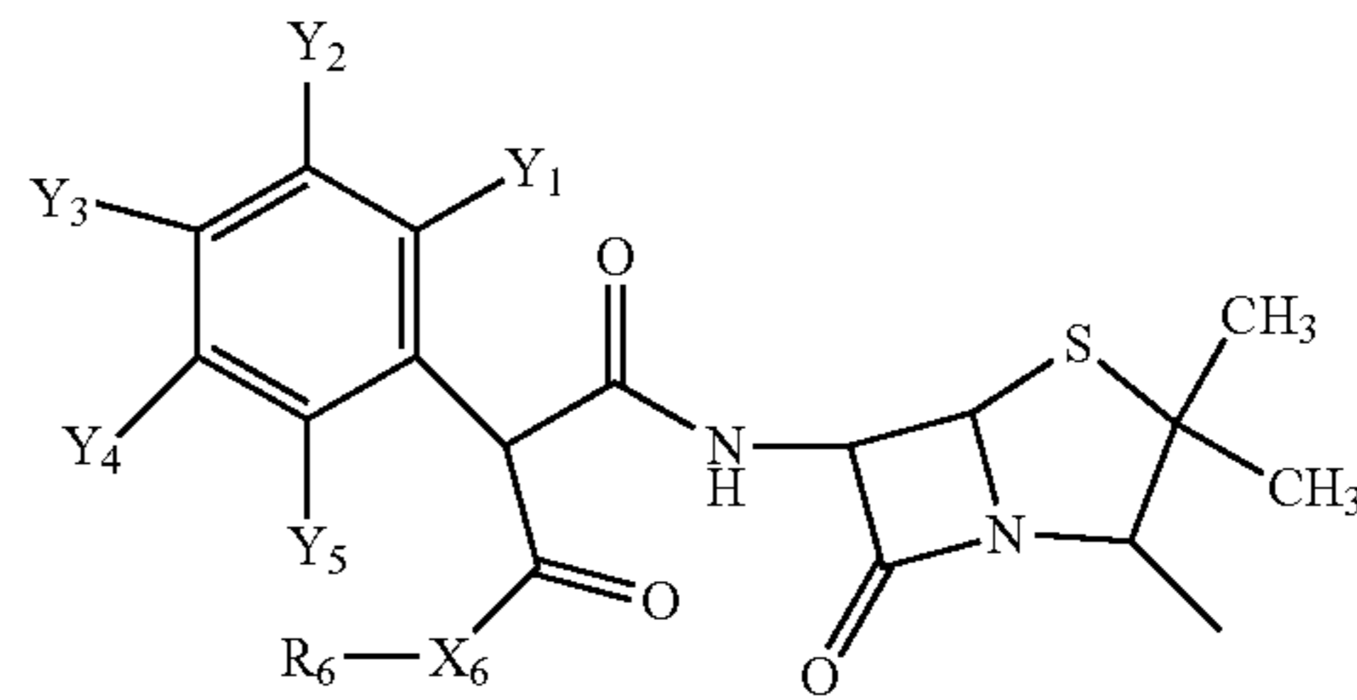
Structure FP-12
