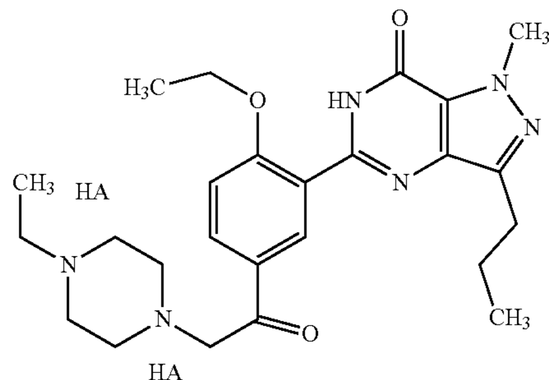
Structure PDE5-I-4
