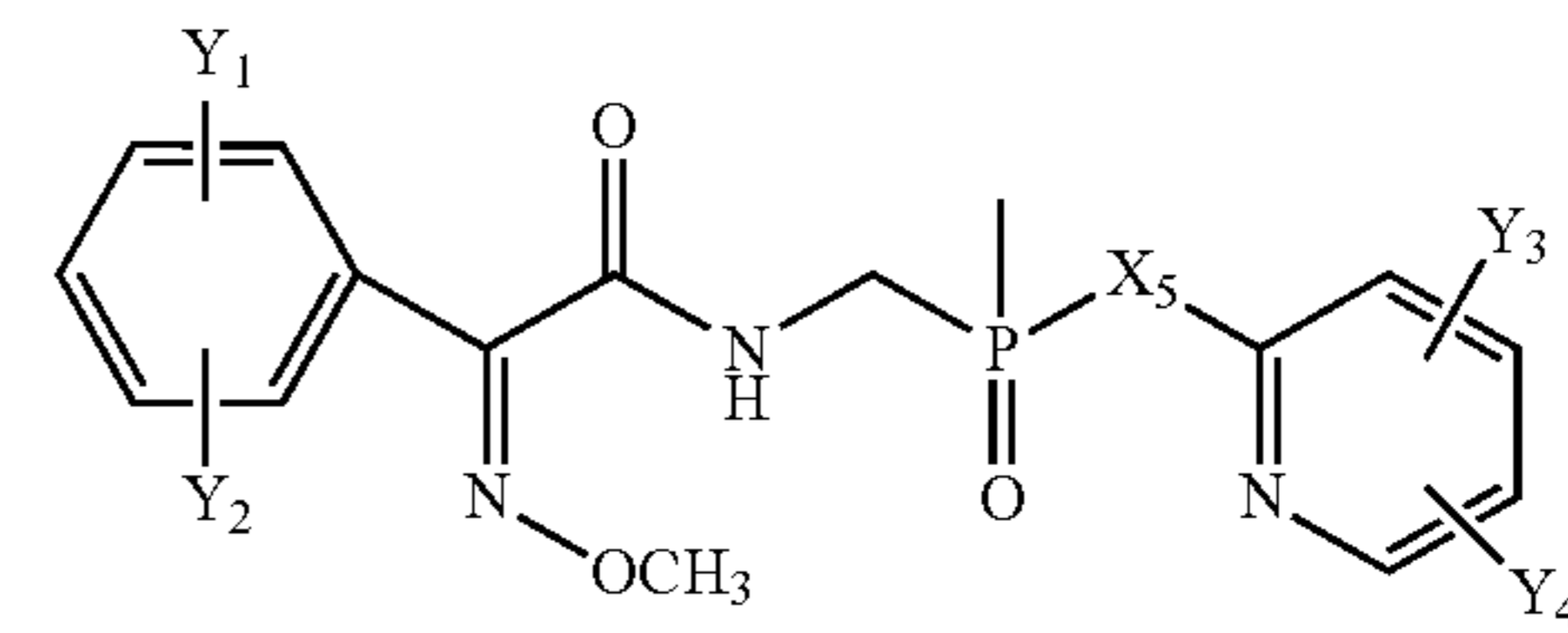
Structure FI-29
