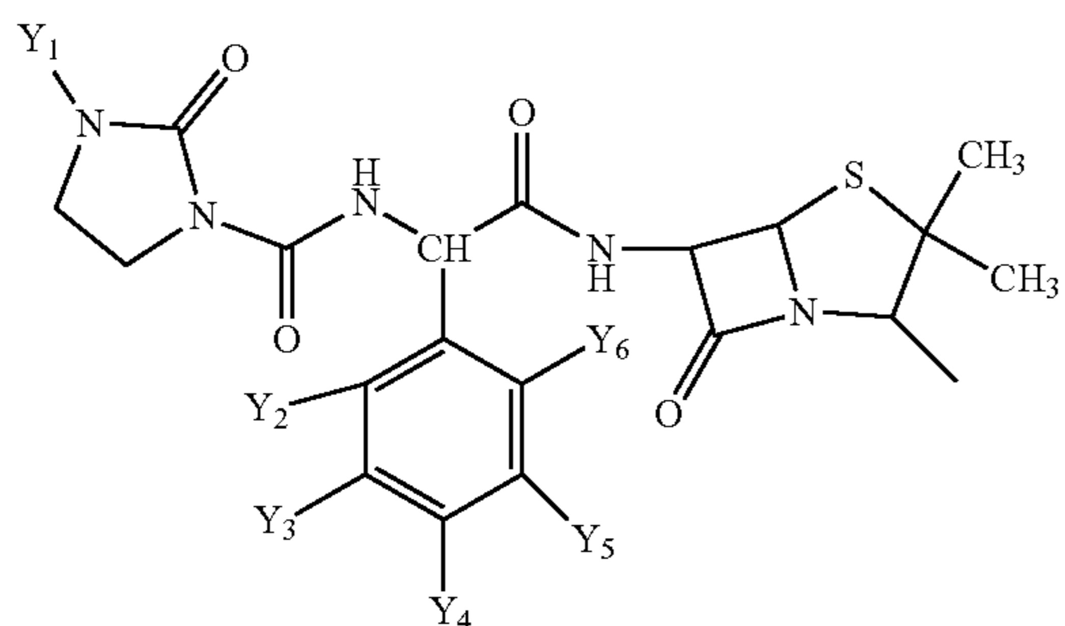
Structure FP-8
