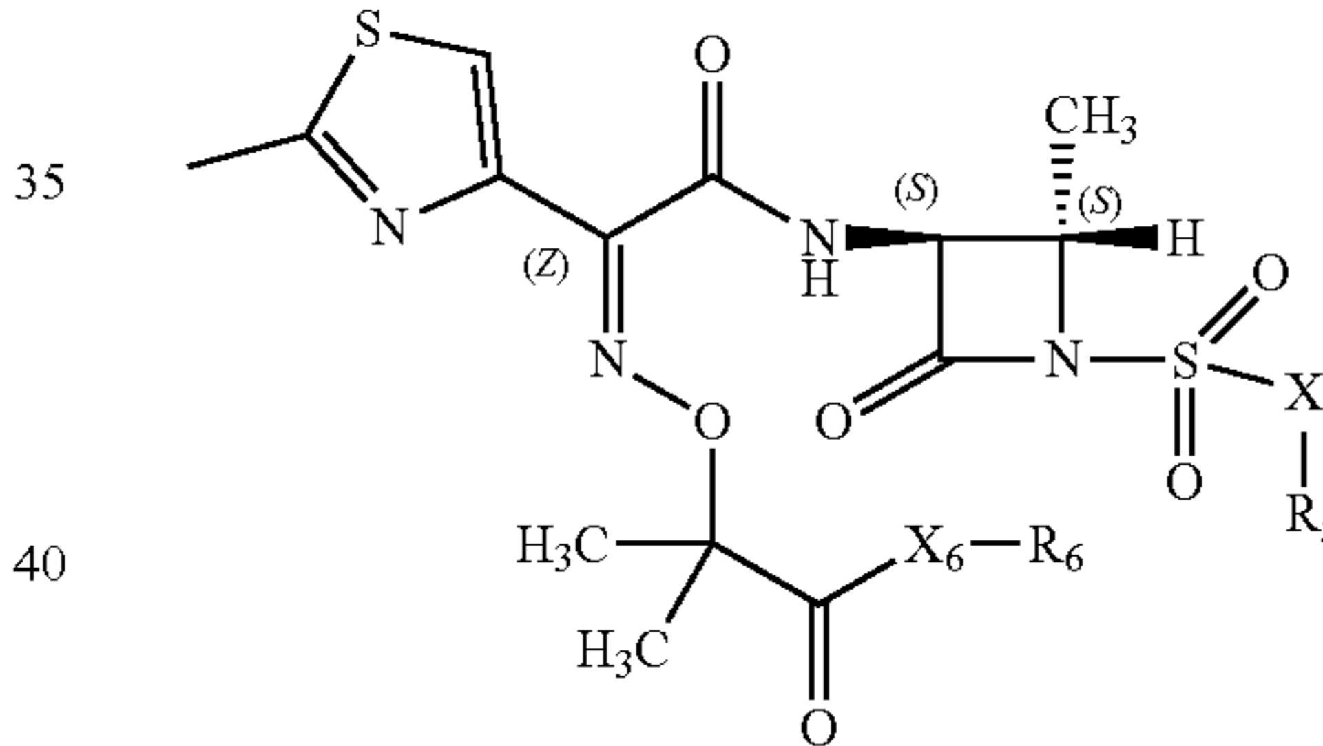
Structure FP-71
