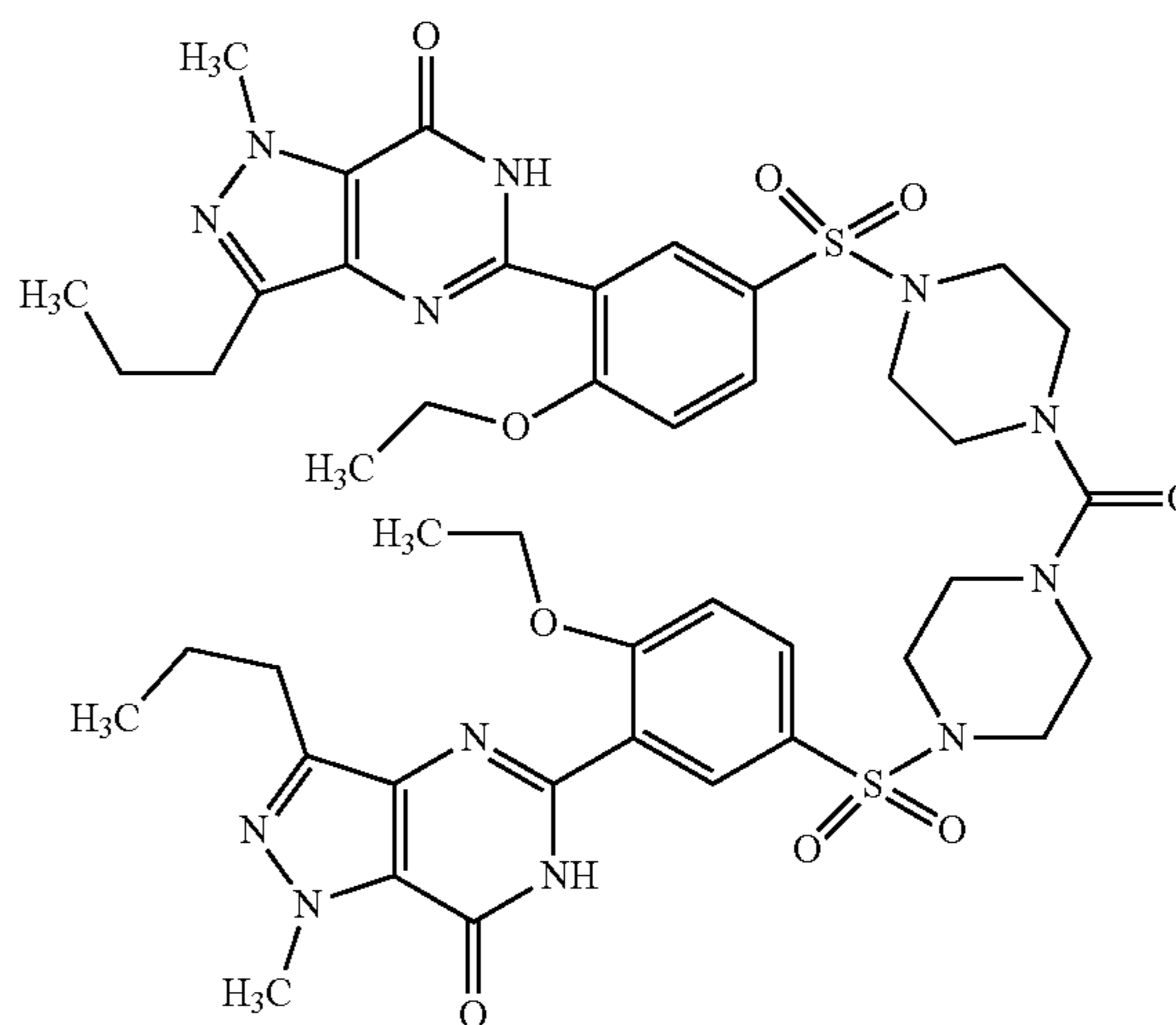
Structure PDE5-I-6
