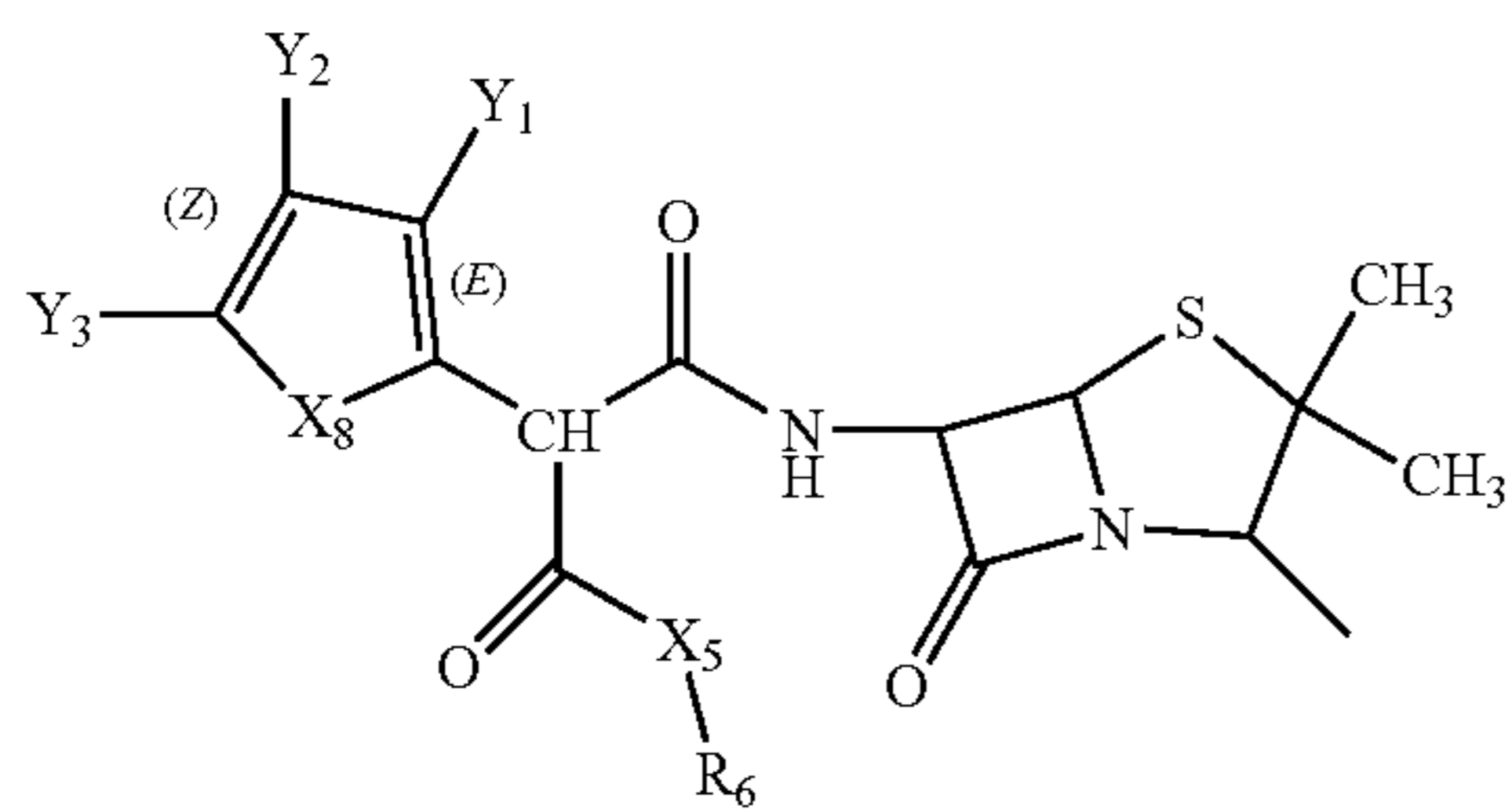
Structure FP-9
