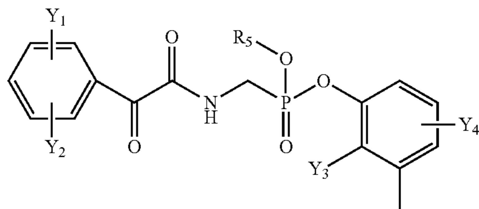
Structure FI-22
