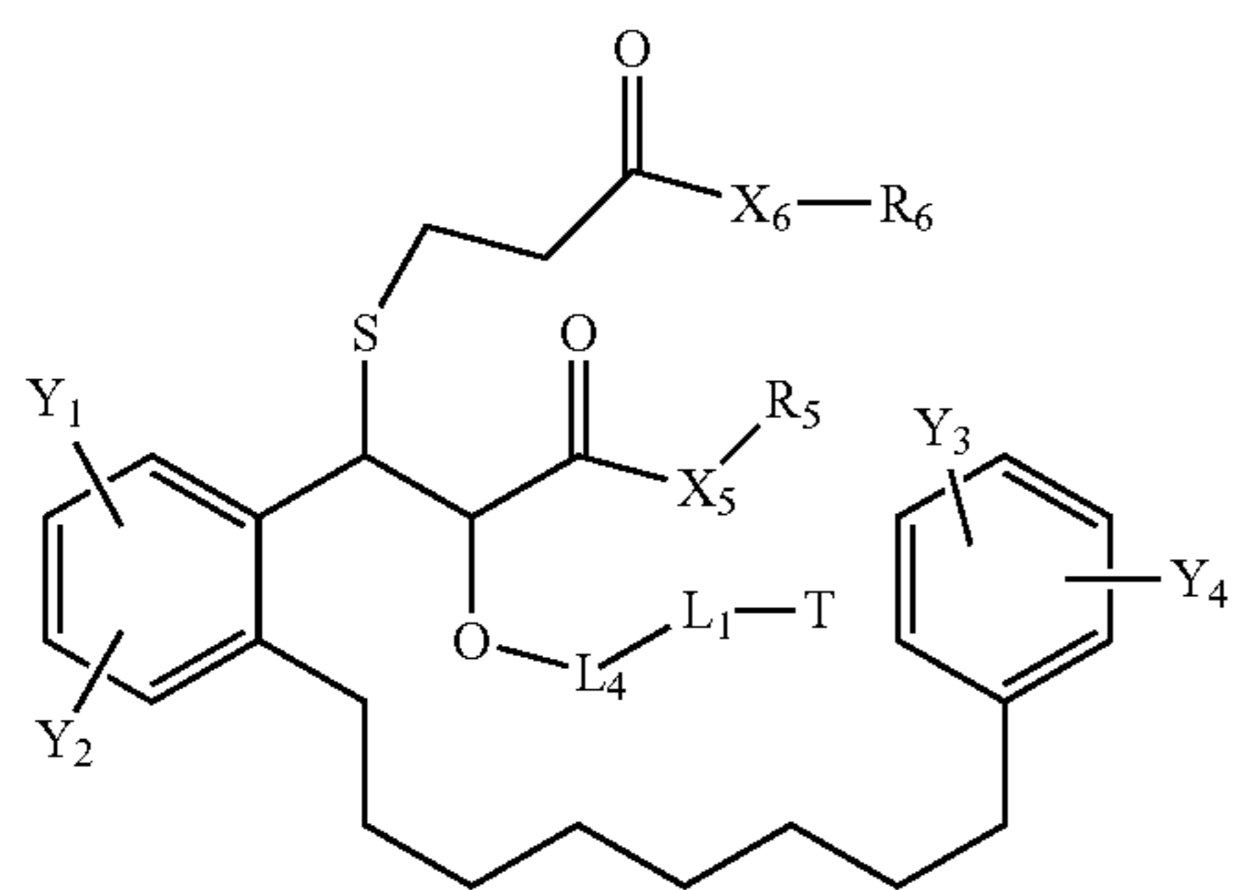
Structure LRA-2
