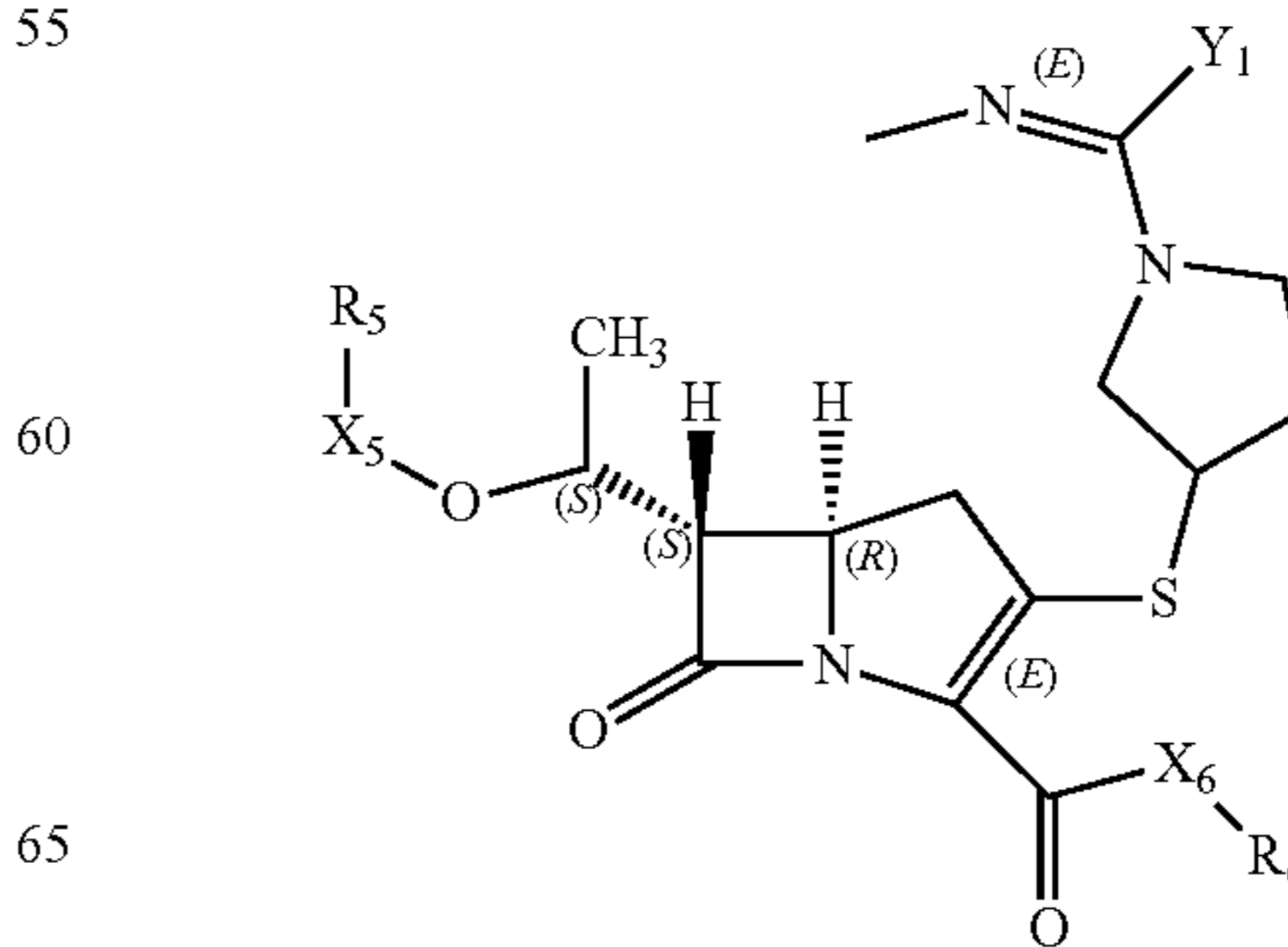
Structure FP-73
