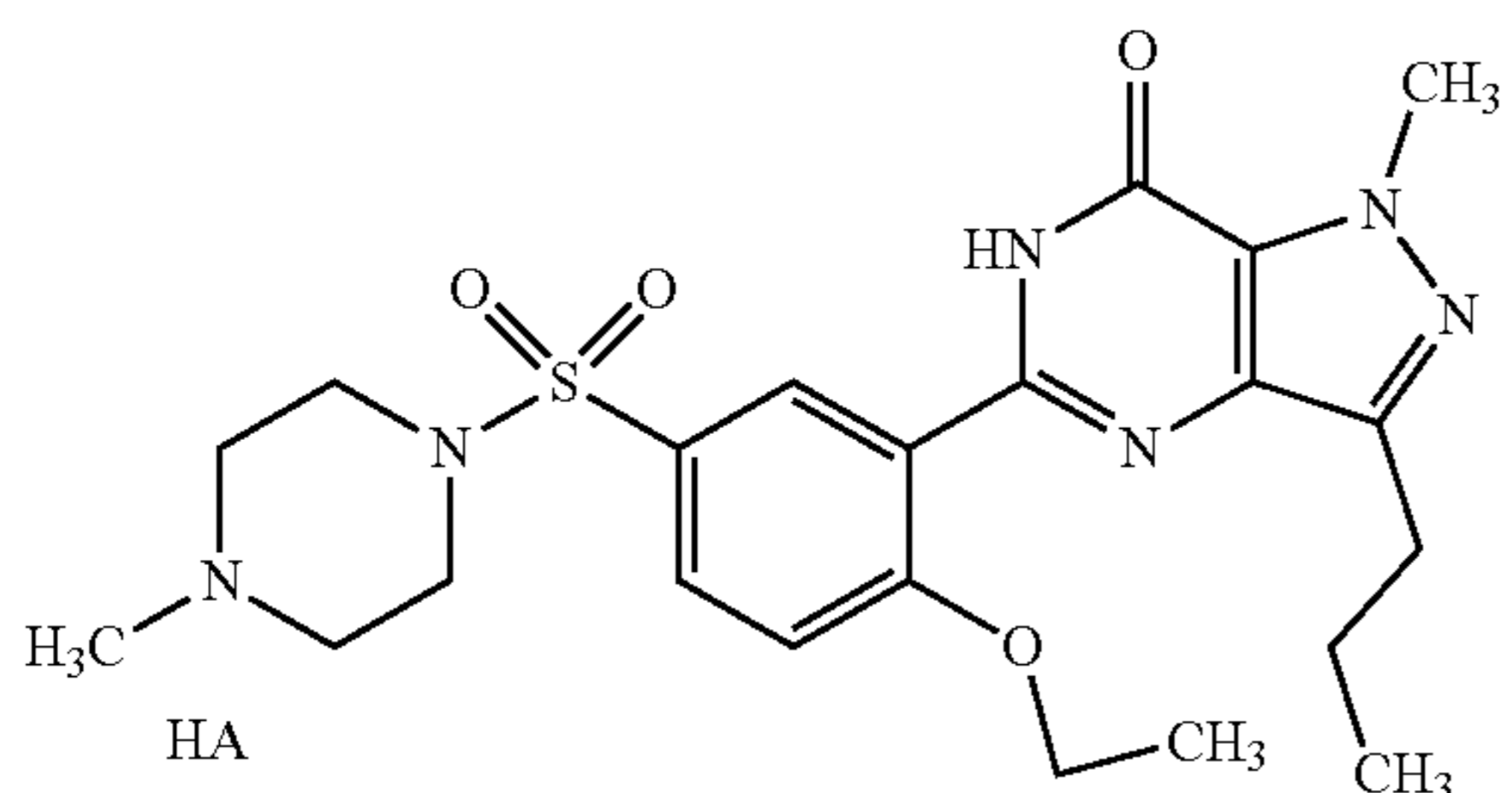
Structure PDE5-I-2
