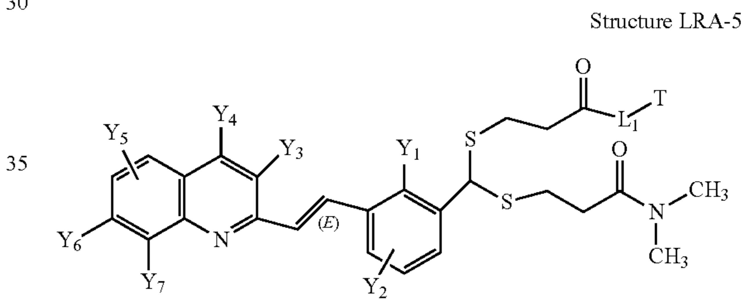
Structure 5-LI-8
