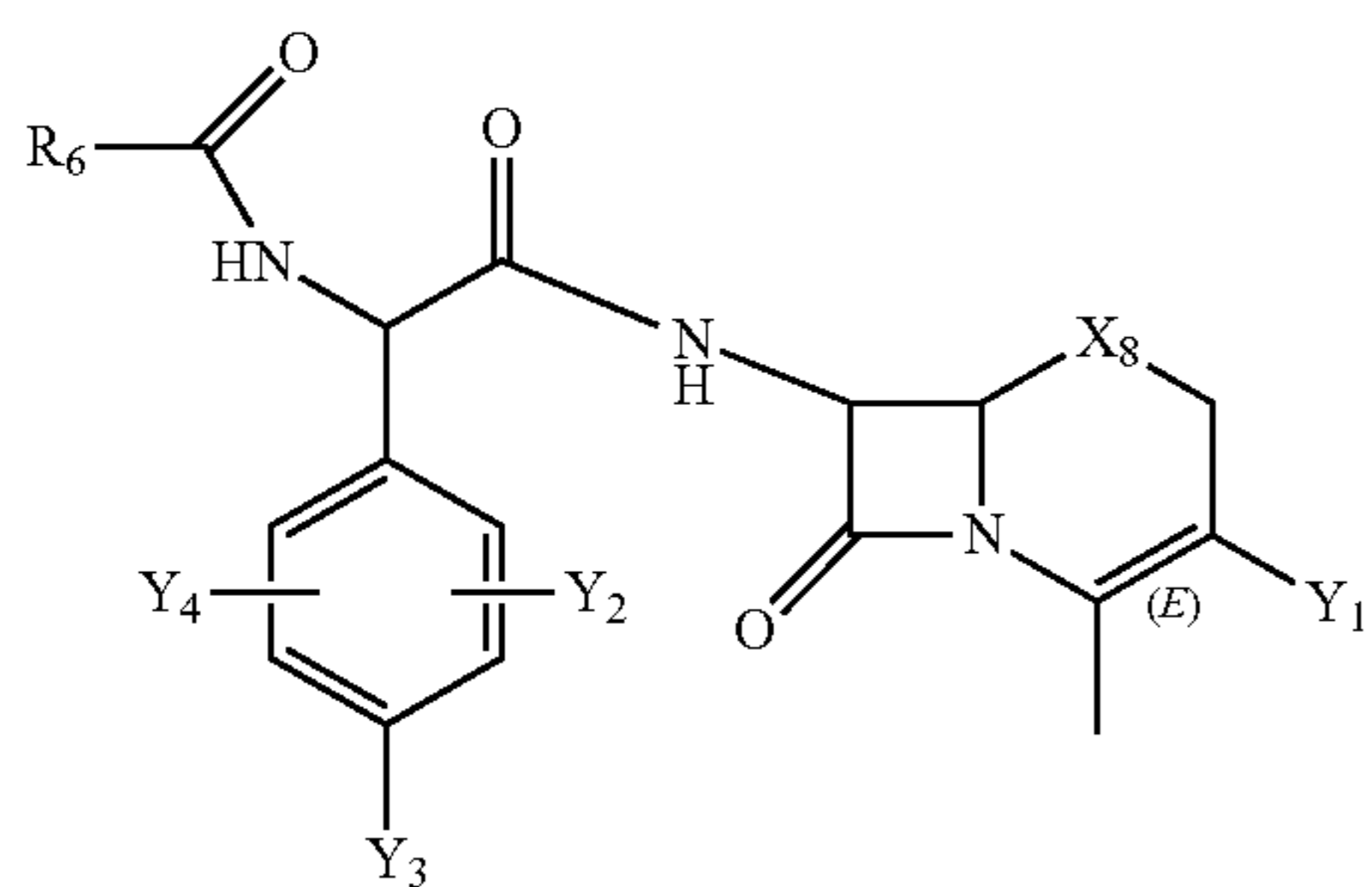
Structure FP-69
