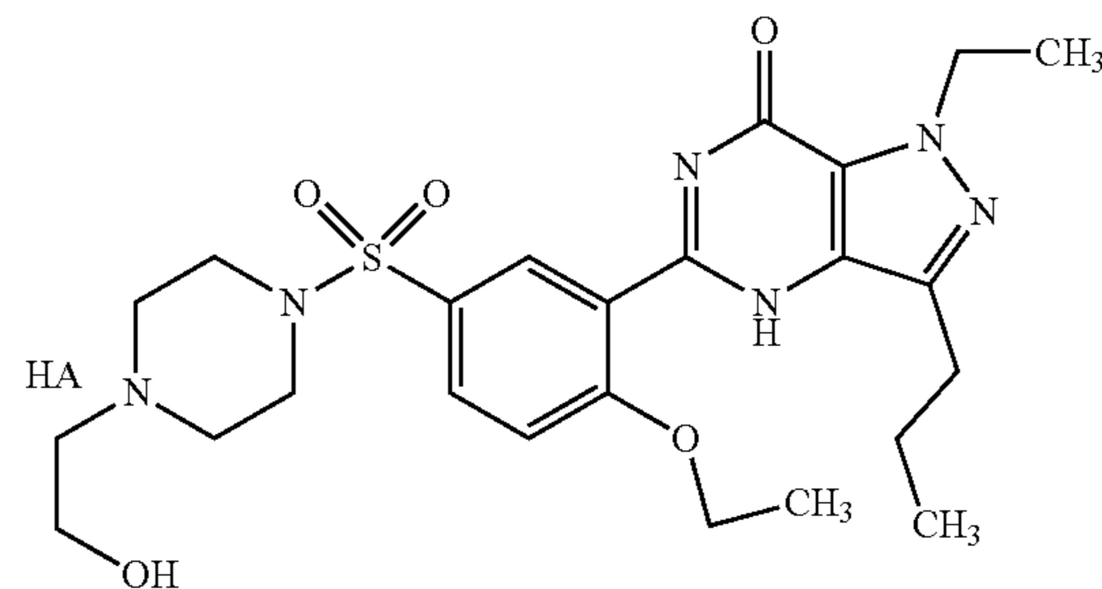
Structure PDE5-I-7
