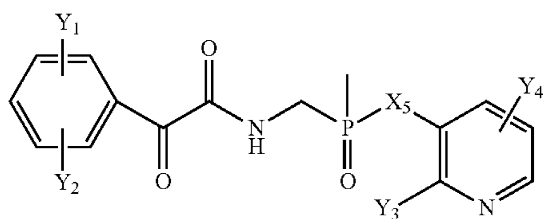
Structure FI-31
