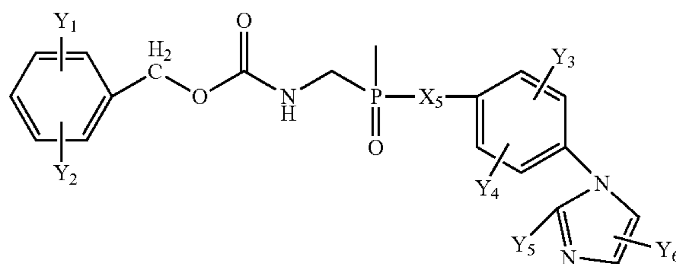
Structure FI-13
