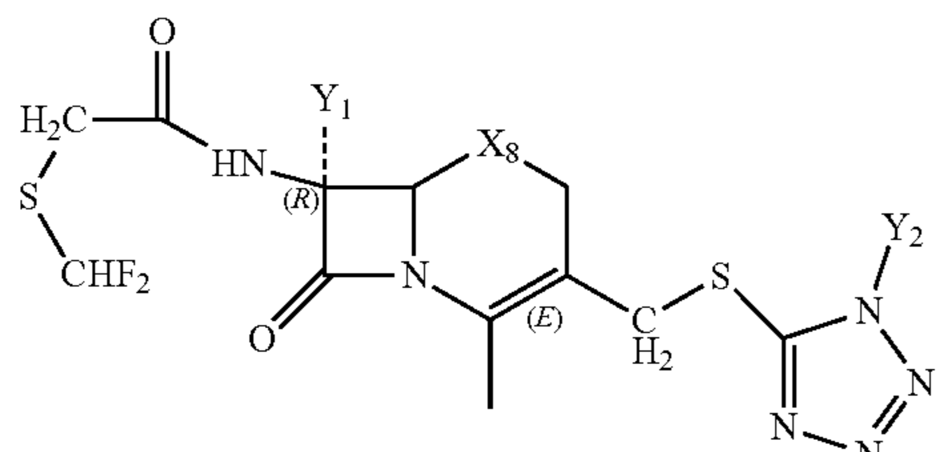
Structure FP-71
