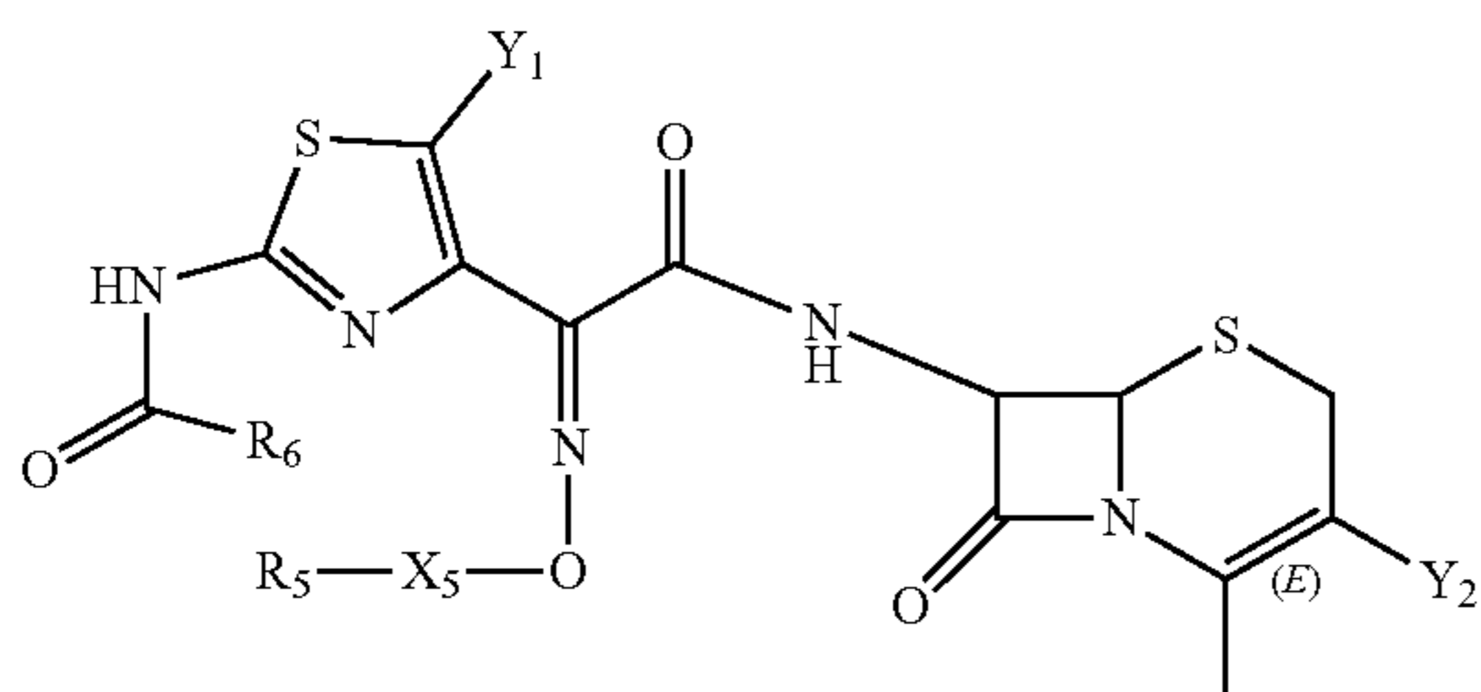
Structure FP-28
