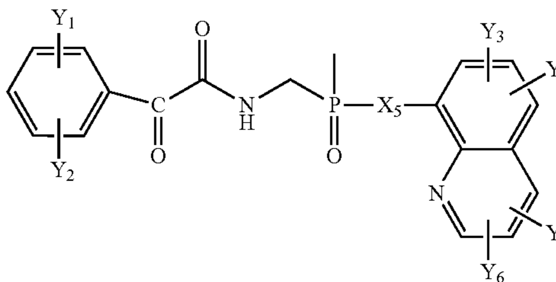
Structure FI-14
