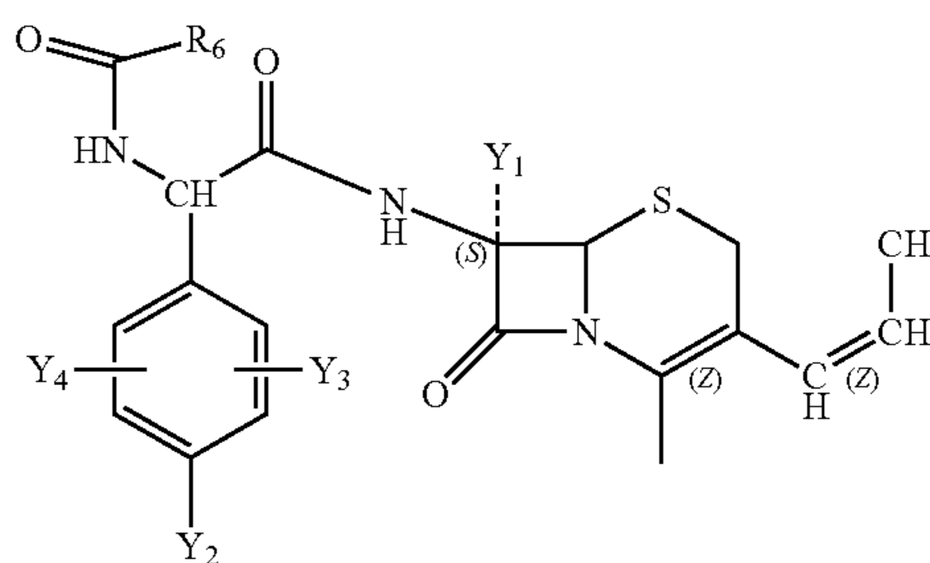
Structure FP-57
