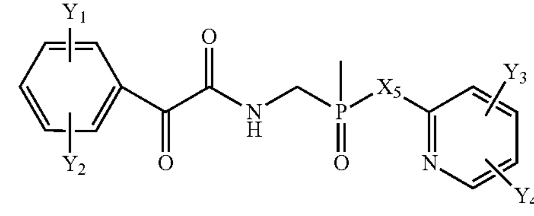
Structure FI-30
