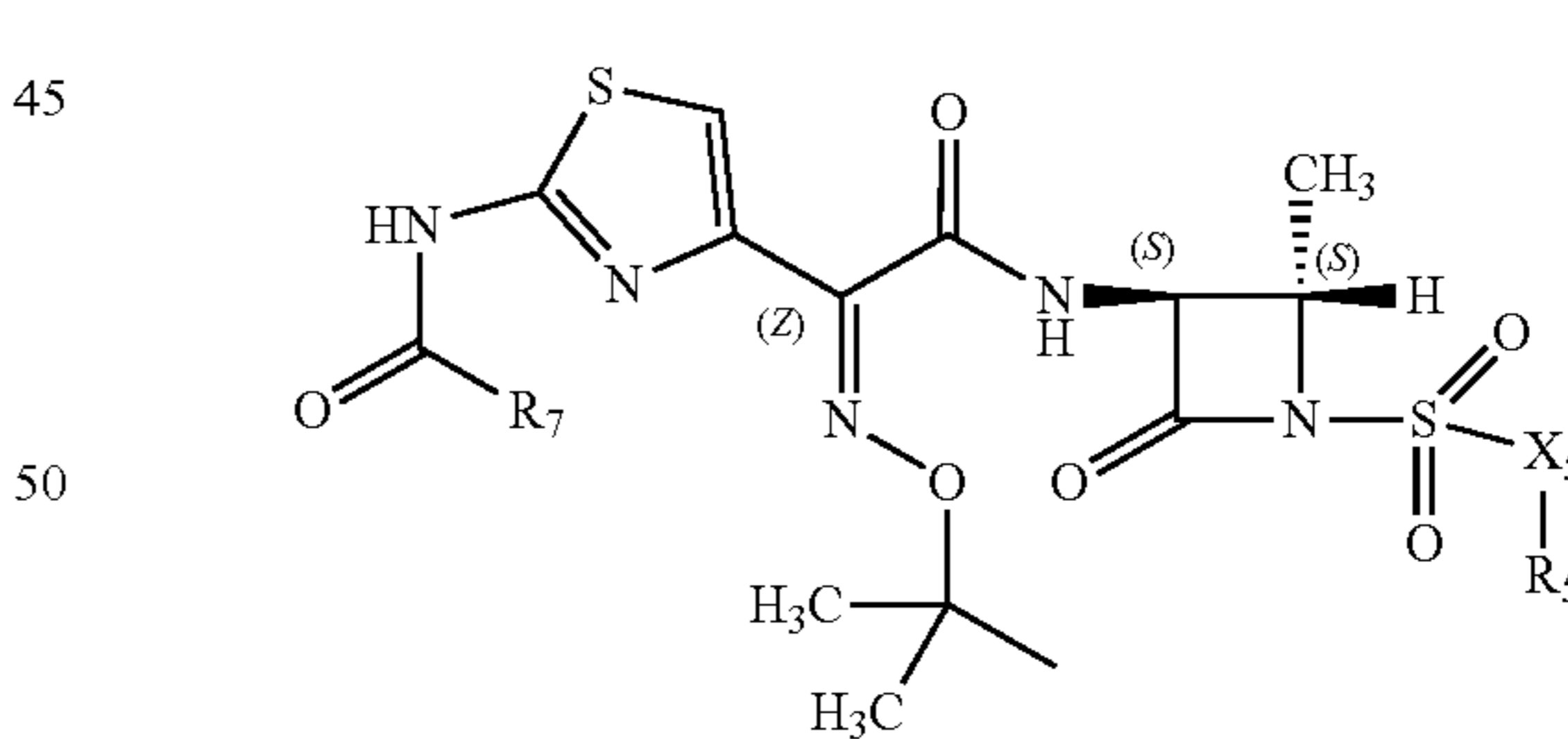
Structure FP-79
