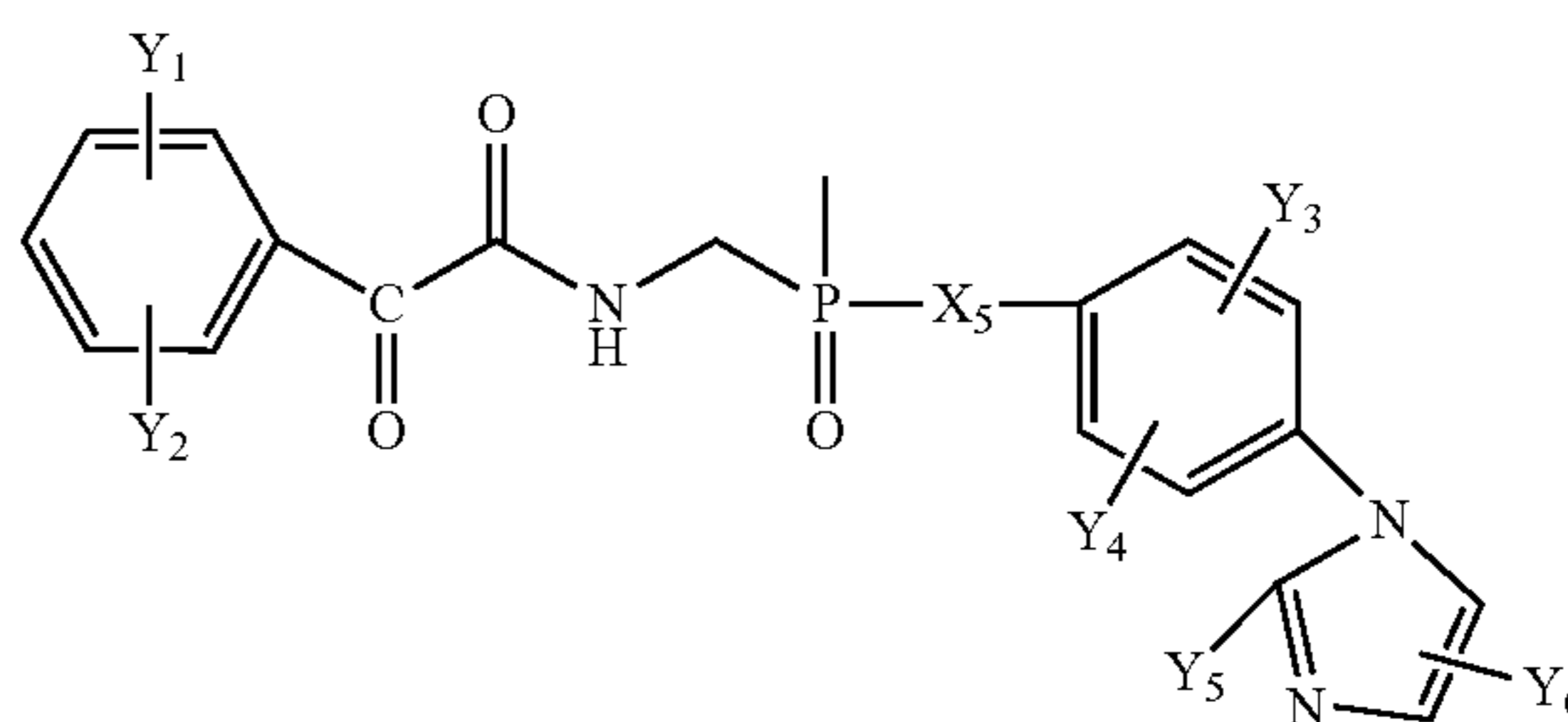
Structure FI-15
