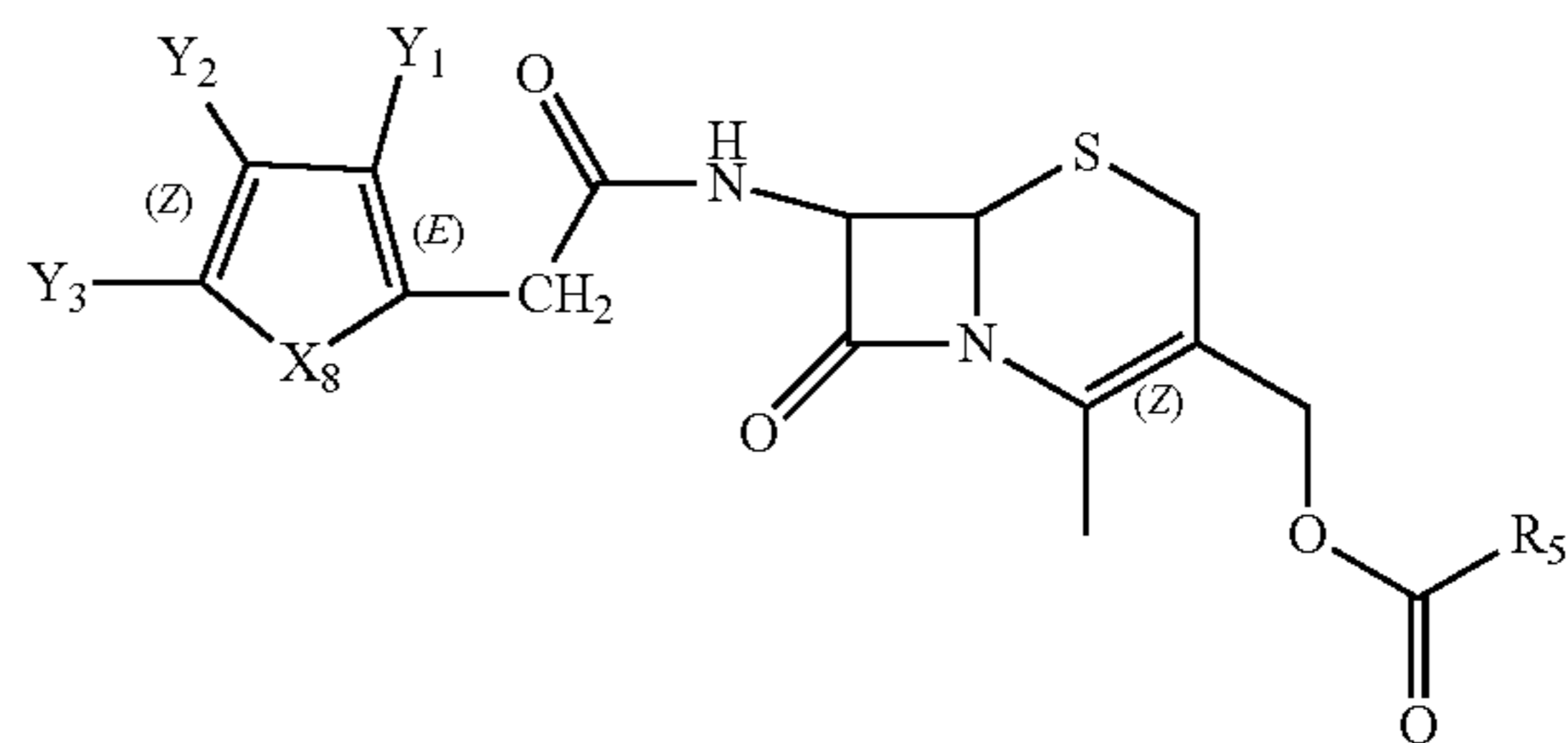
Structure FP-14
