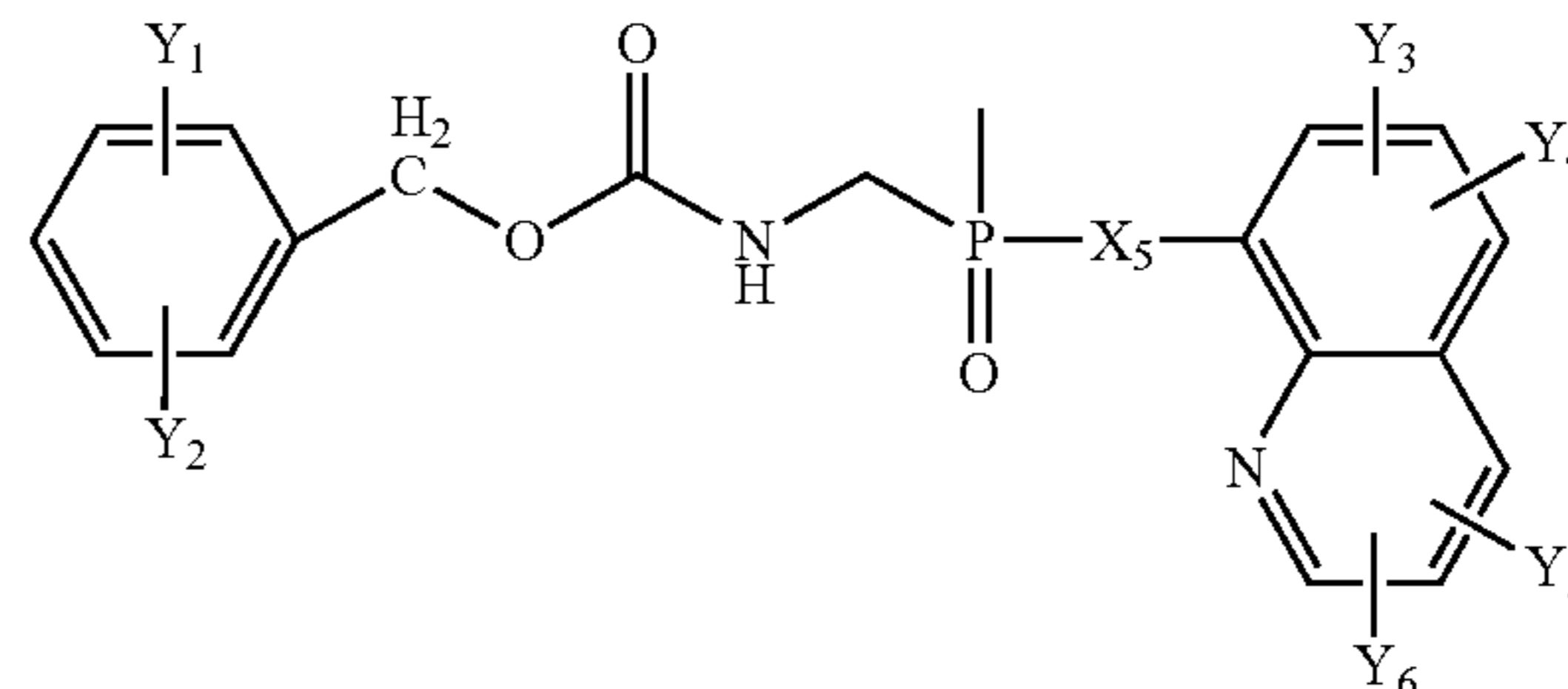
Structure FI-12
