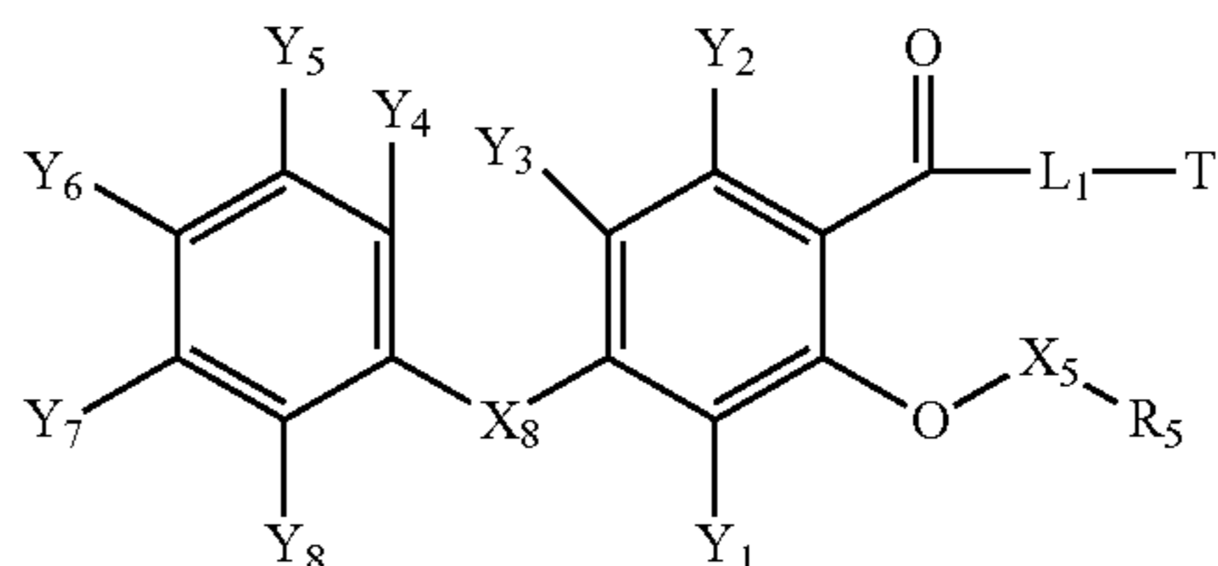
Structure NSAID-11
