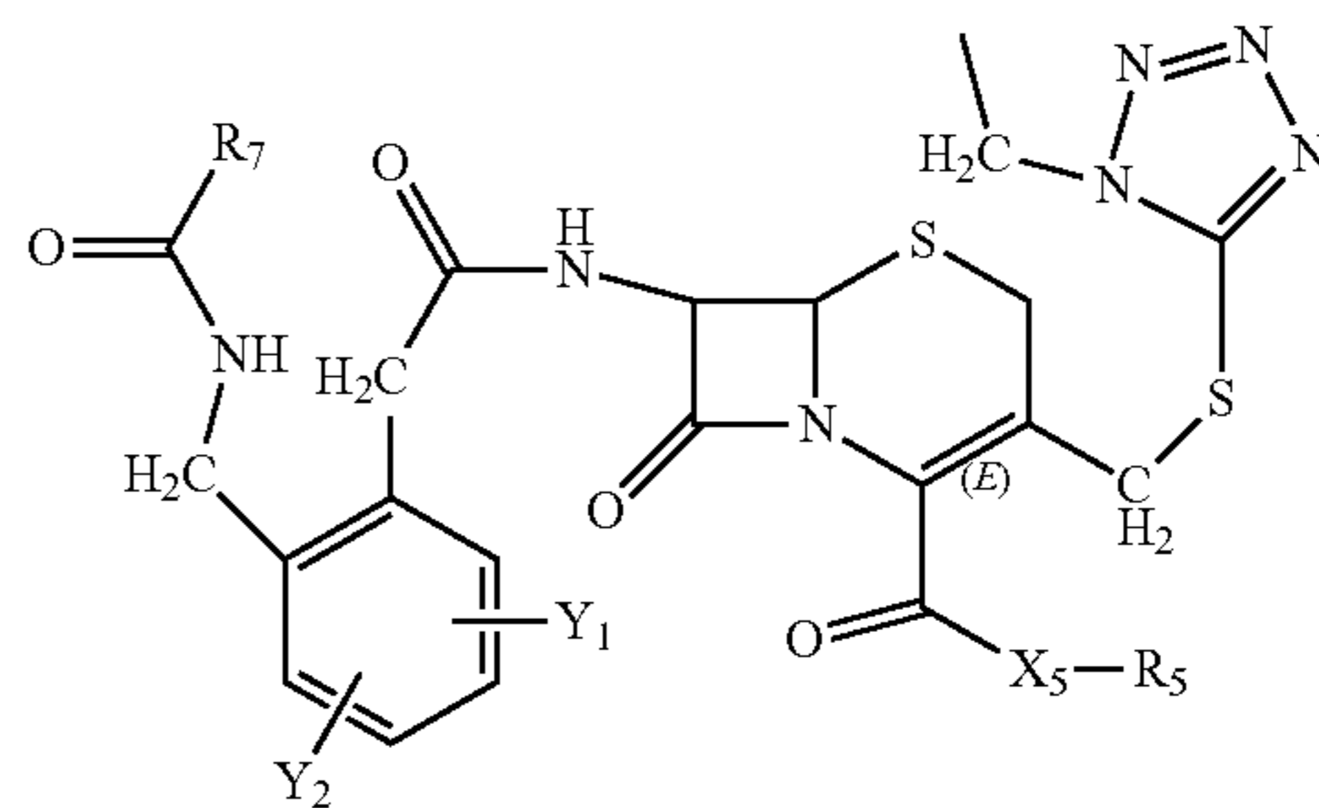
Structure FP-63
