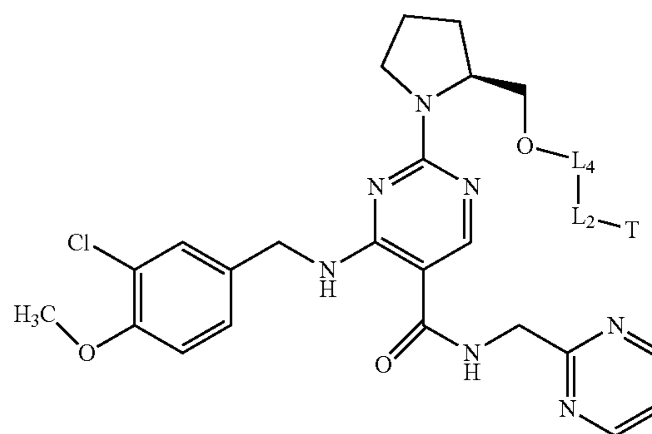
Structure PDE5-I-5
