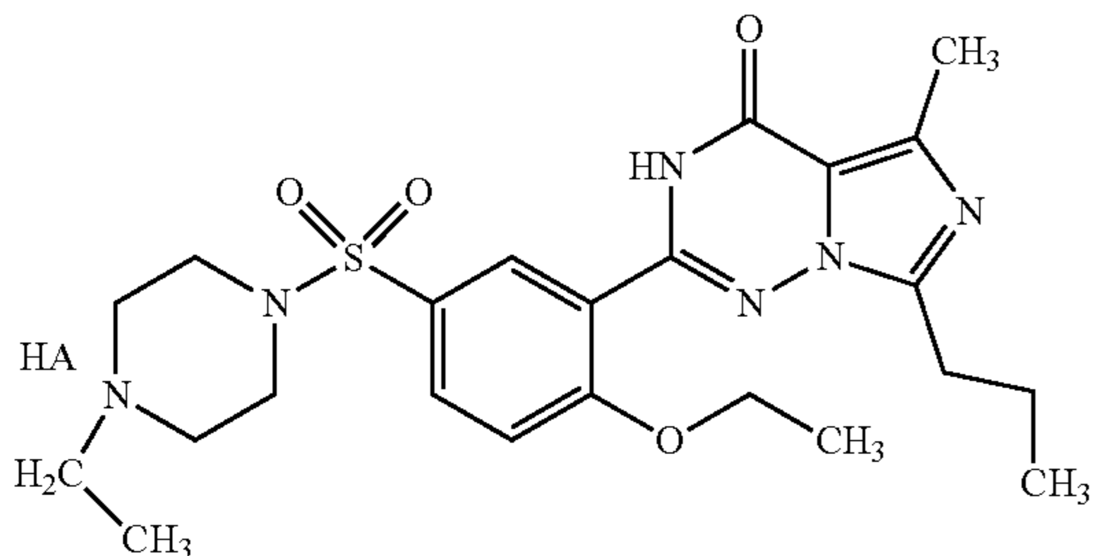
Structure PDE5-I-3
