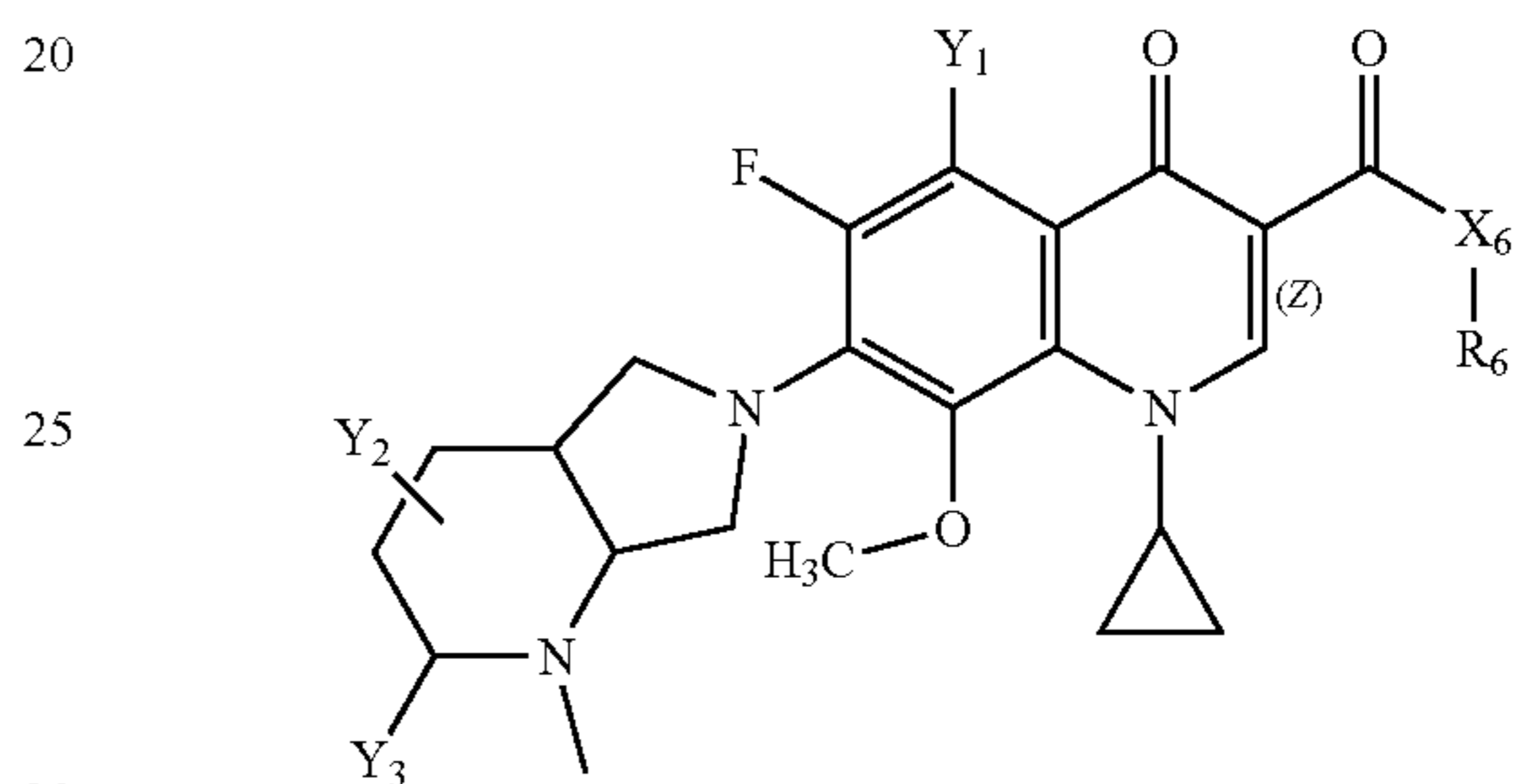
Structure FT-18
