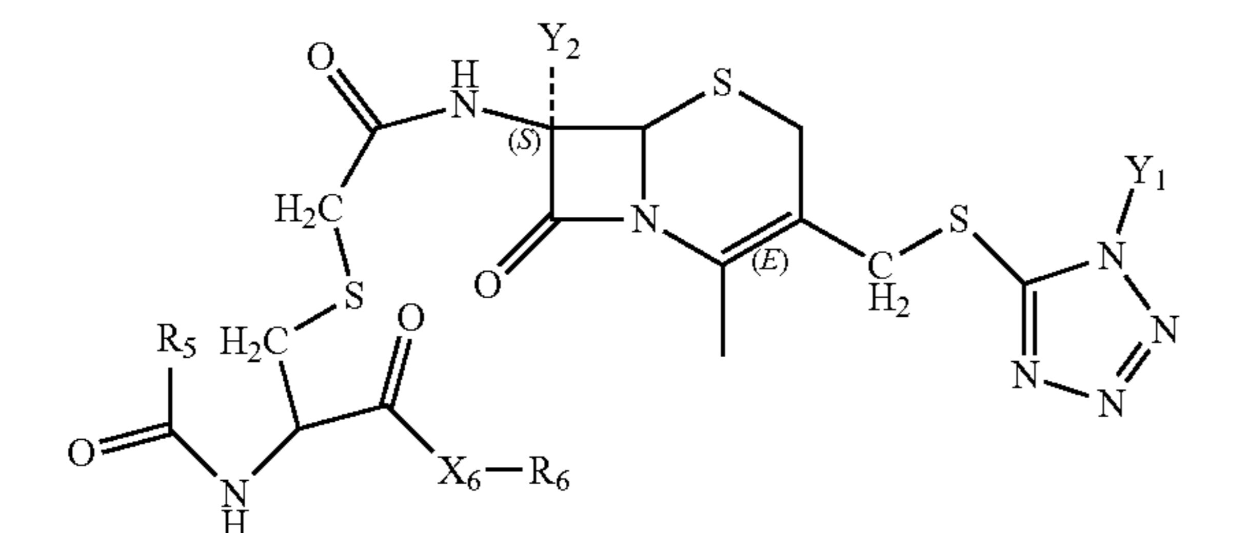
Structure FP-52
