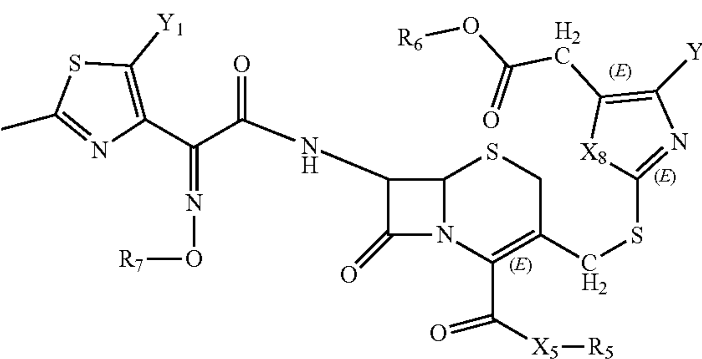
Structure FP-36
