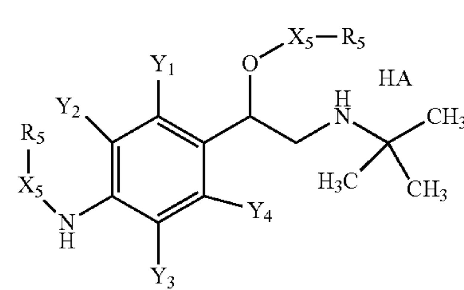
Structure ARA-13
