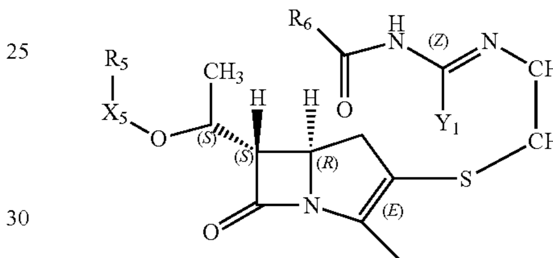
Structure FP-70
