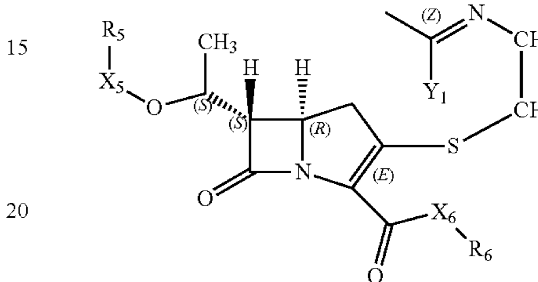
Structure FP-69
