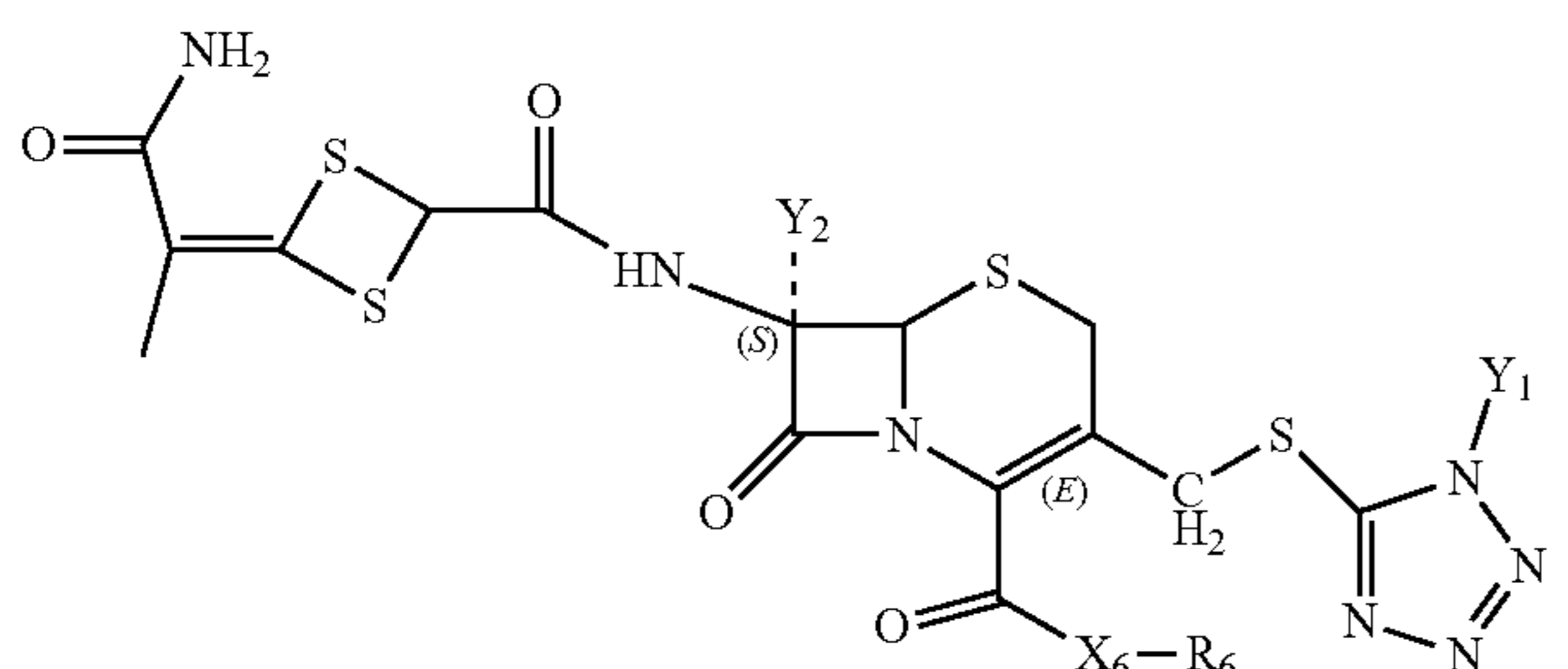
Structure FP-50
