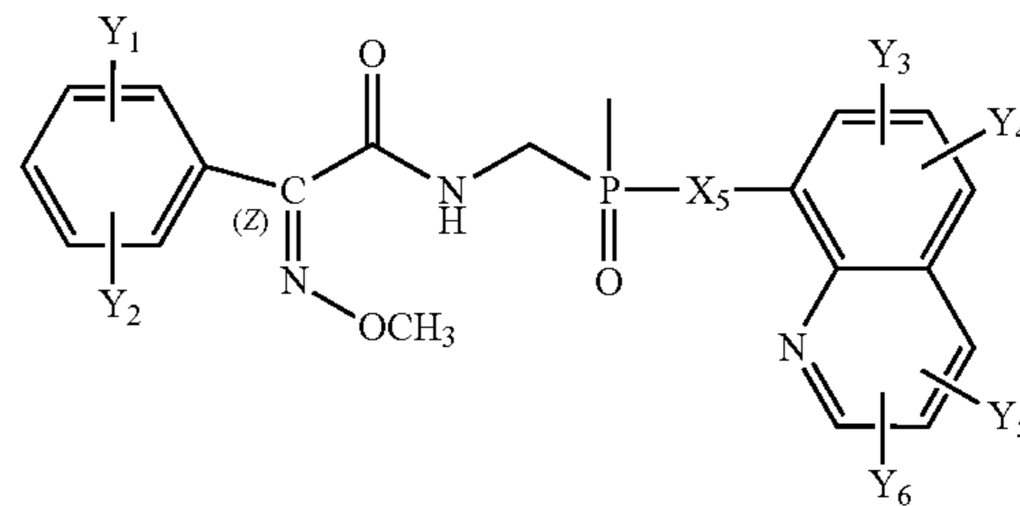
Structure FI-27
