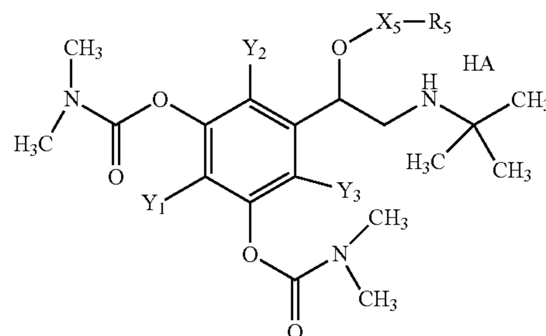
Structure ARA-12
