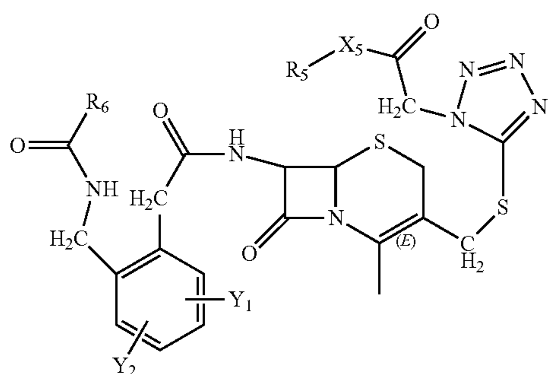
Structure FP-62
