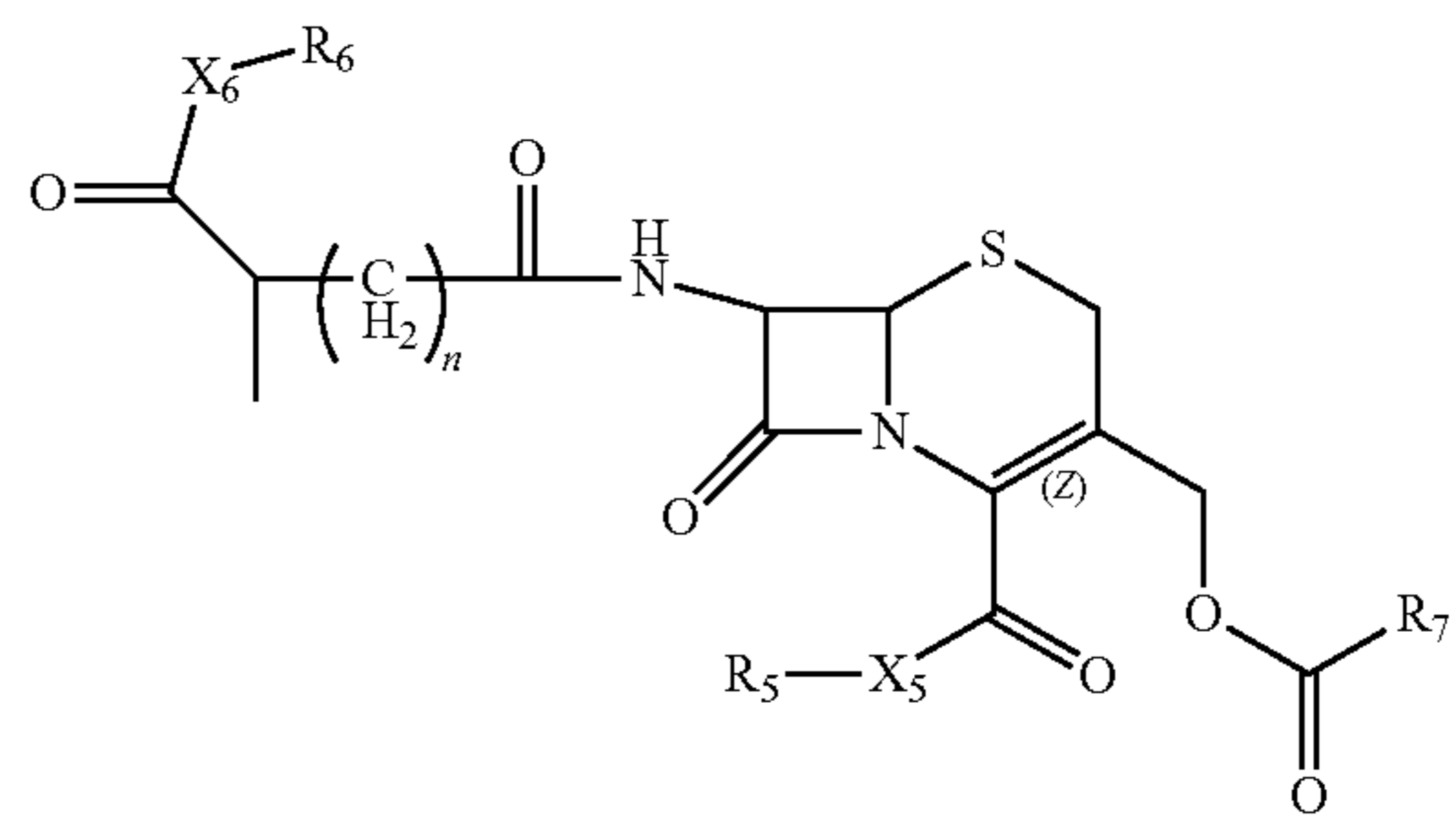
Structure FP-16
