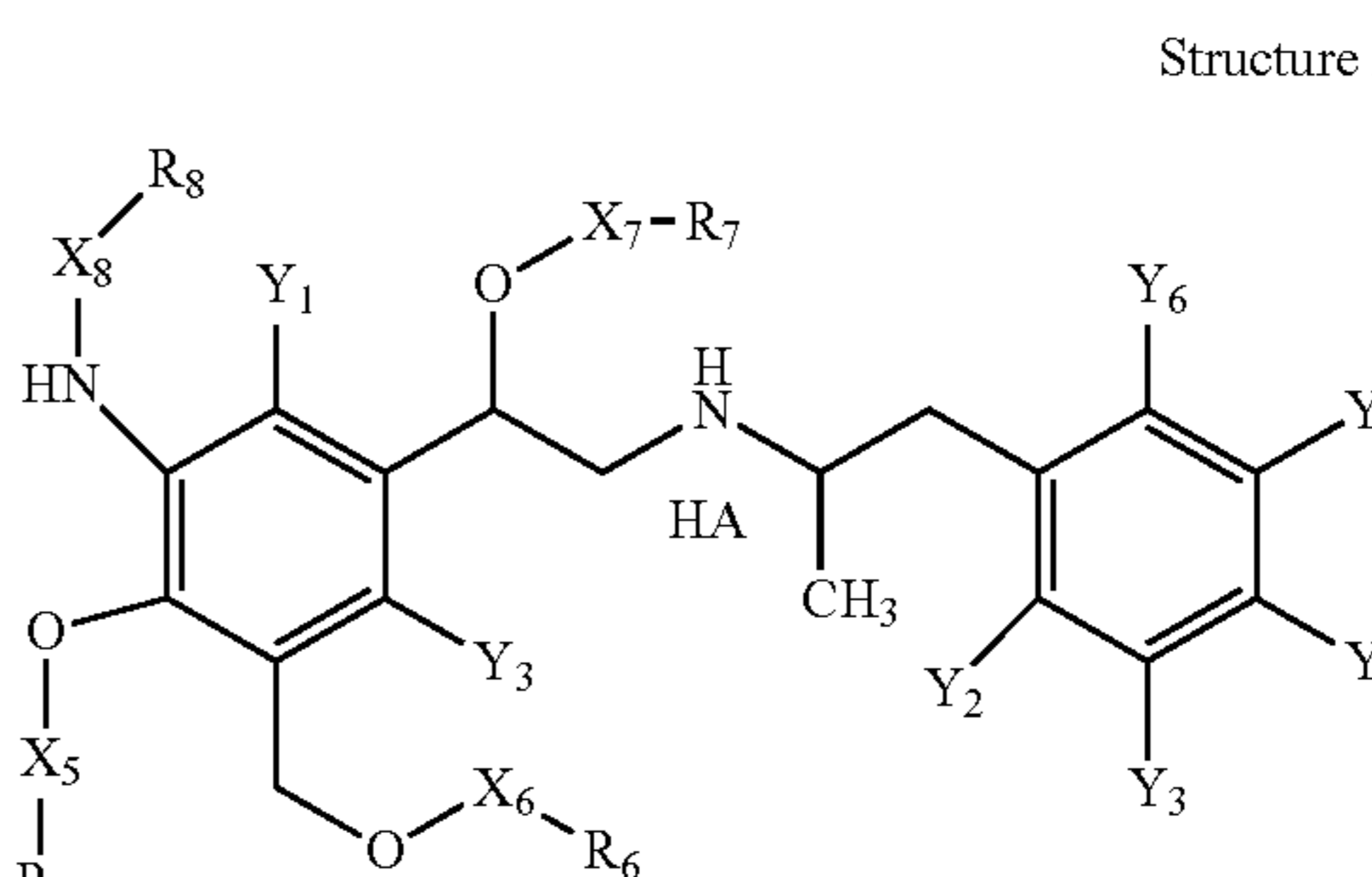
Structure ARA-12
