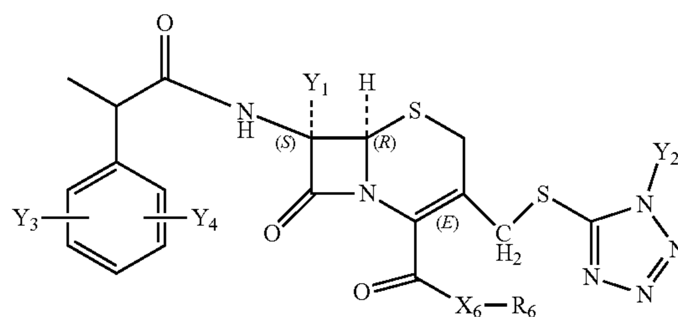
Structure FP-65
