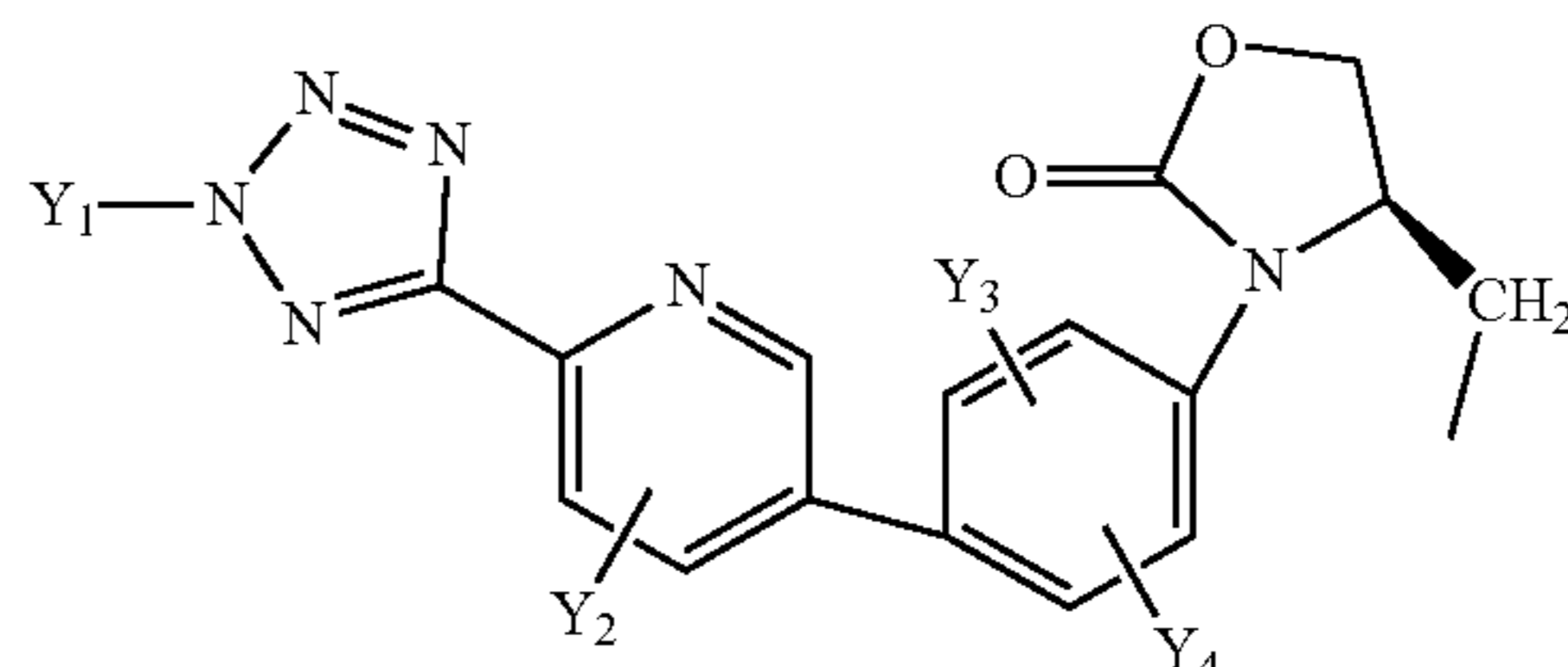
Structure FT-1
