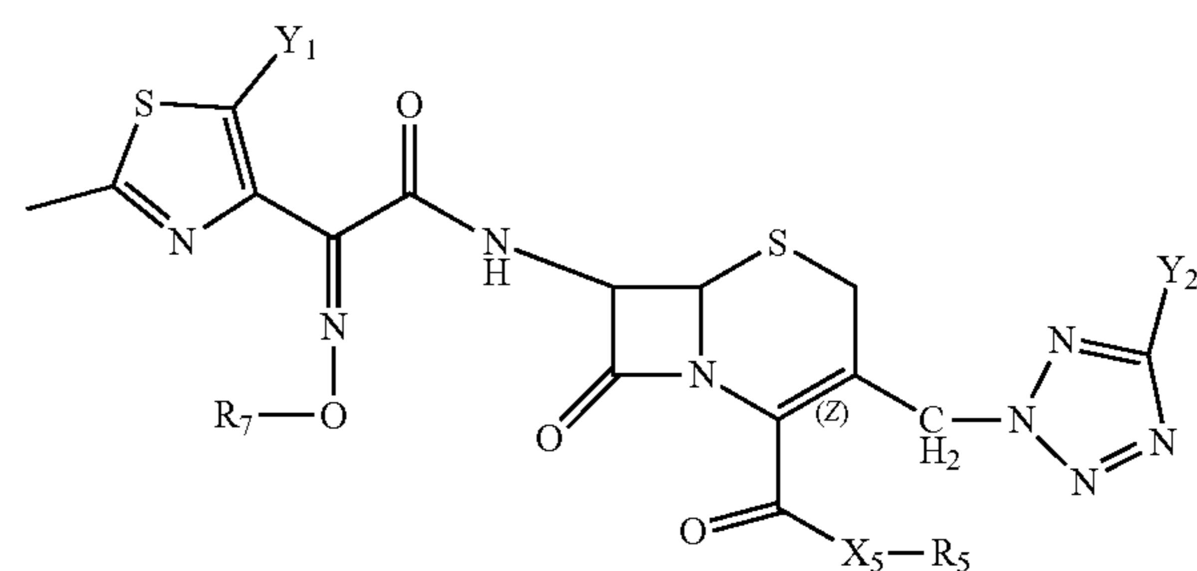
Structure FP-44
