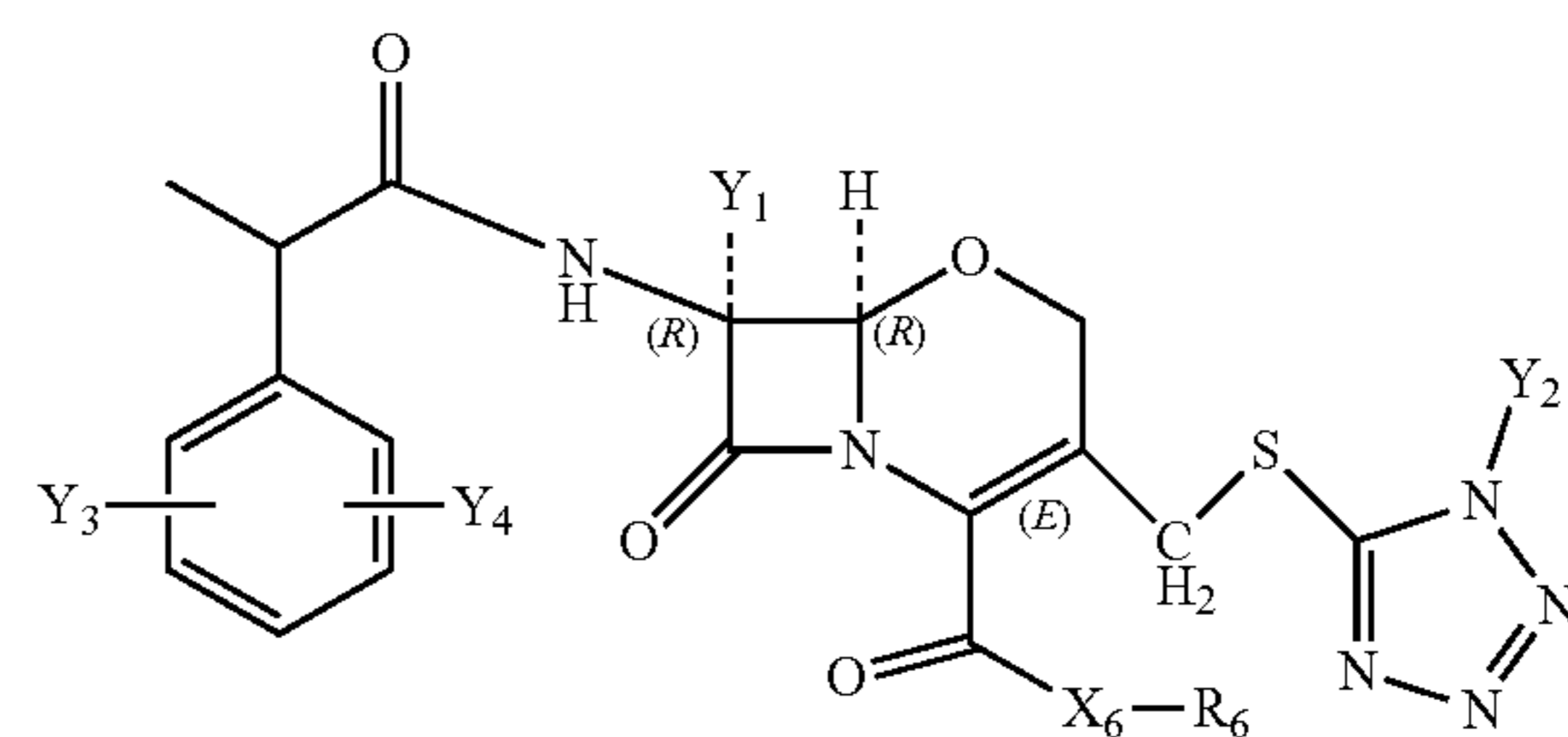
Structure FP-66
