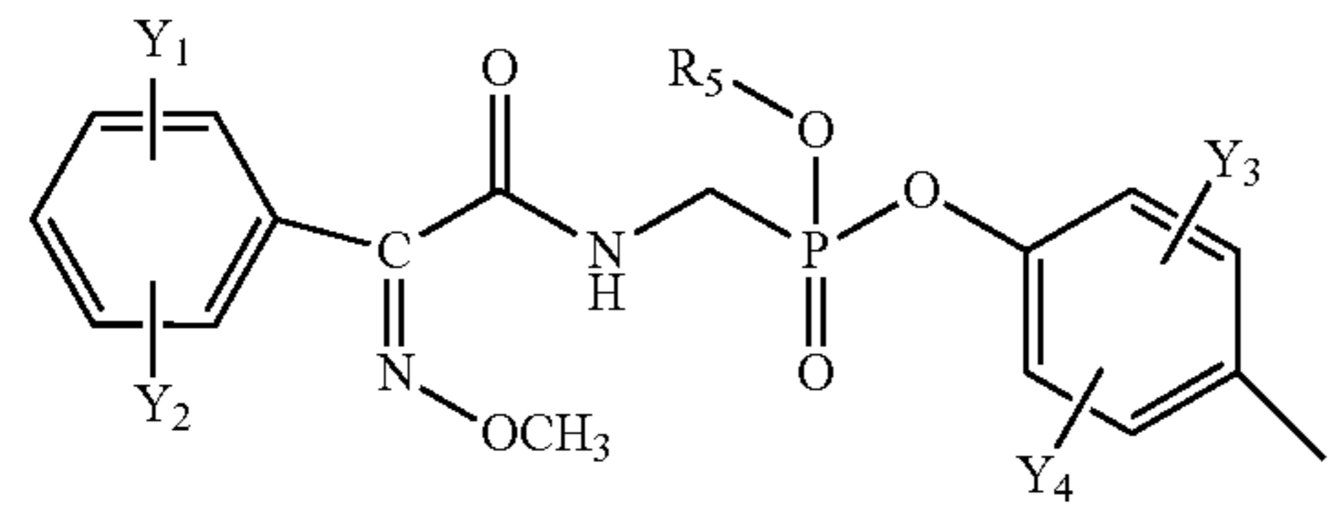
Structure FI-23
