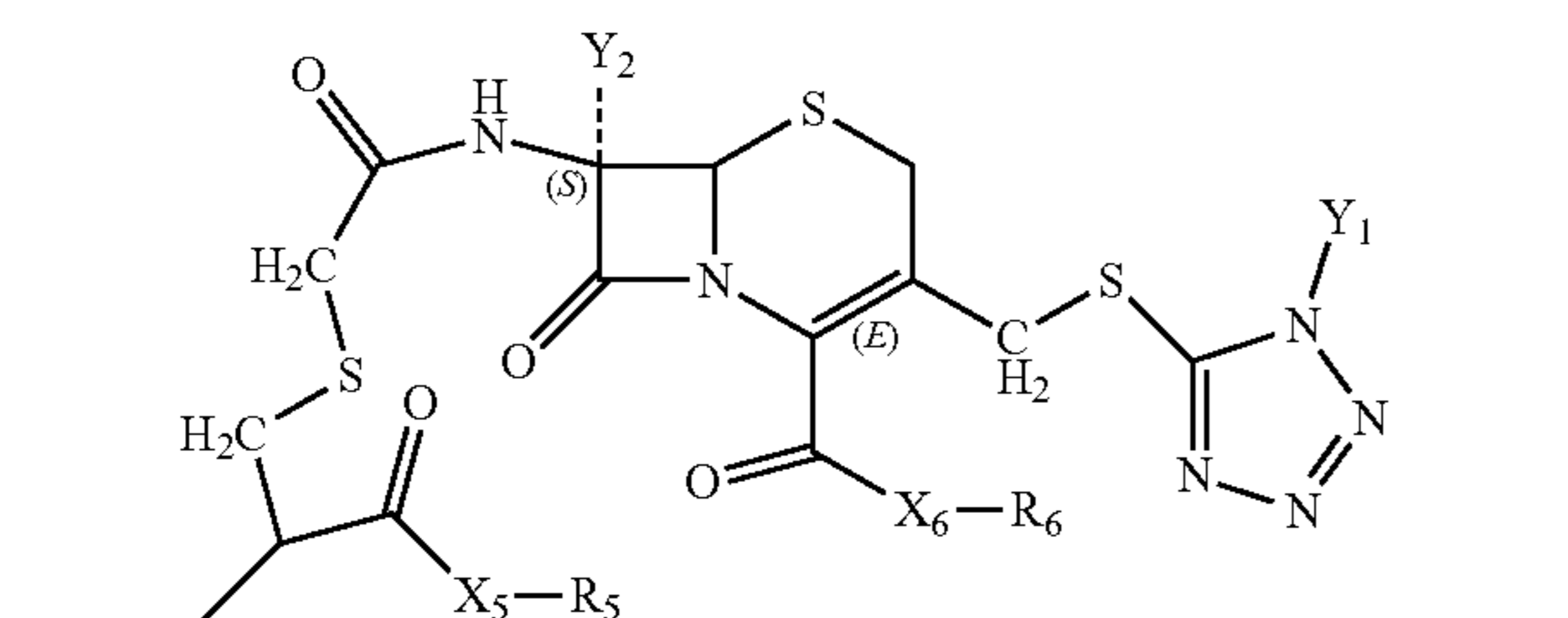
Structure FP-51
