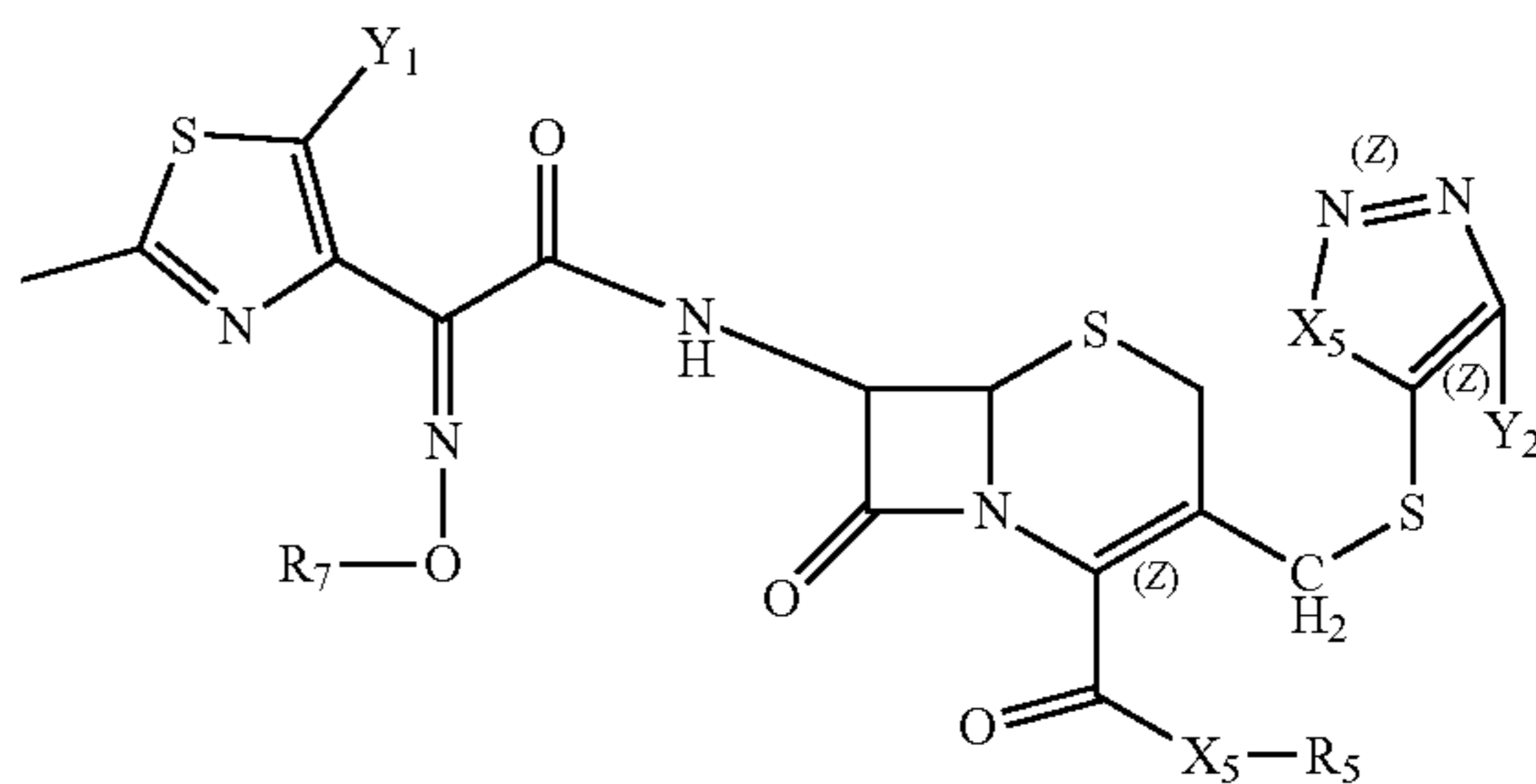
Structure FP-36
