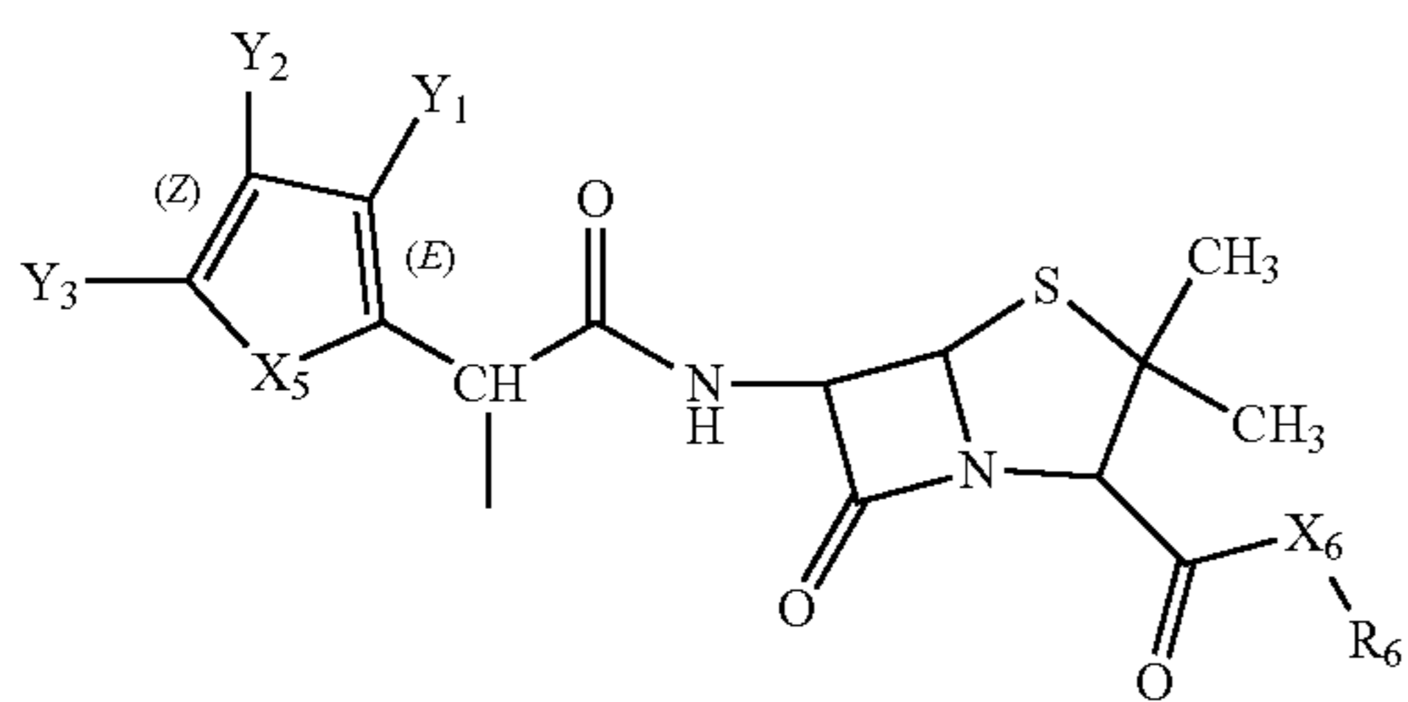
Structure FP-10
