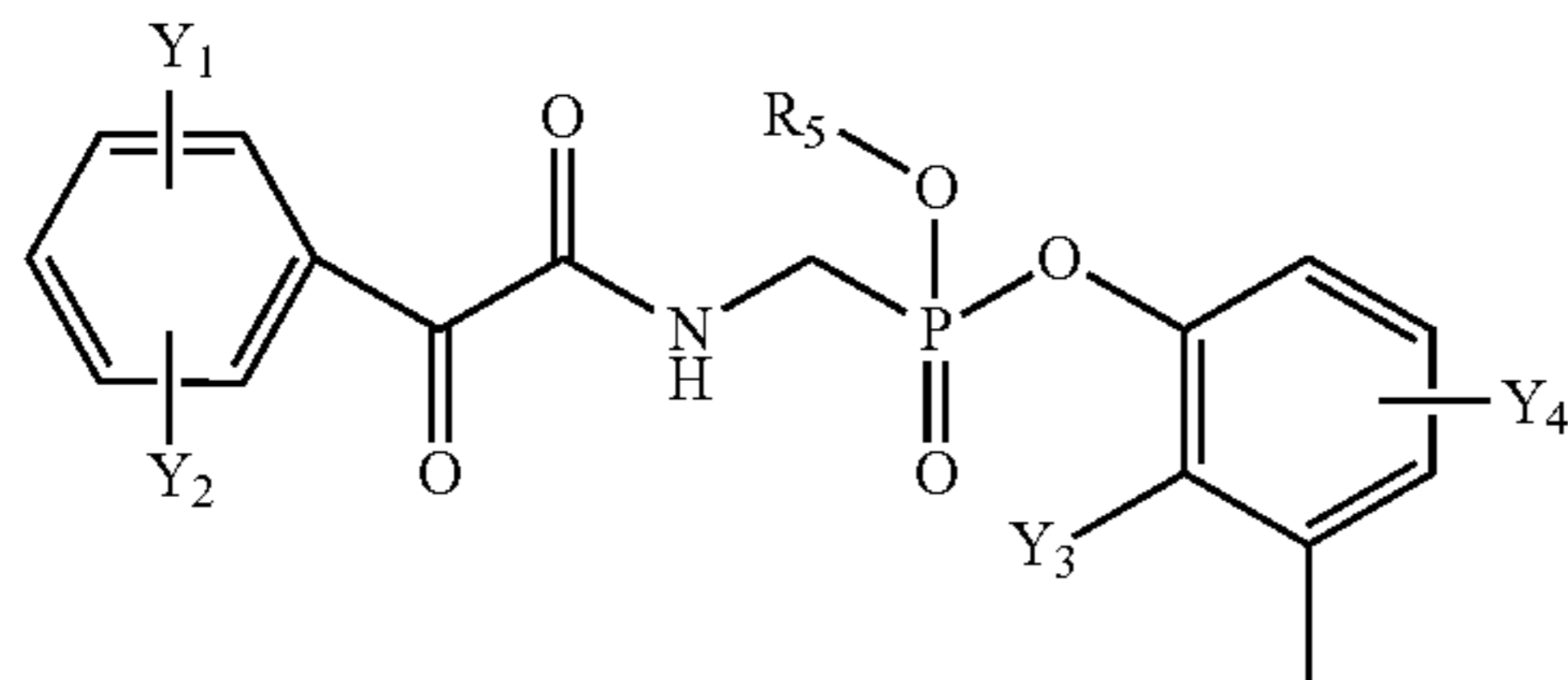
Structure FI-21
