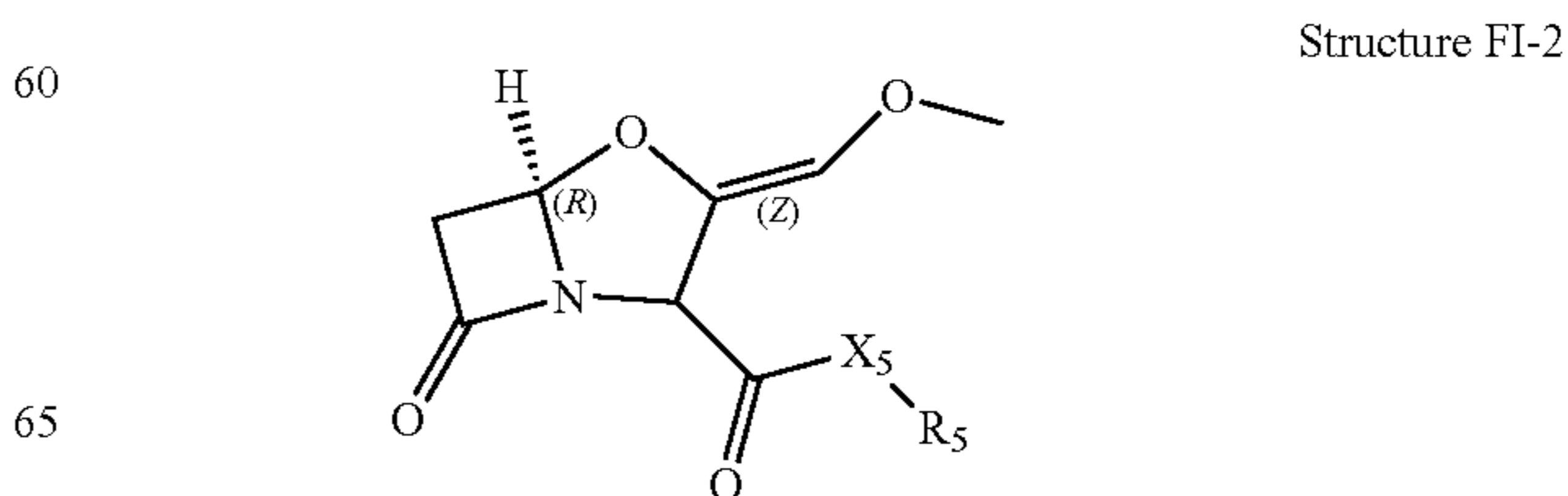
Structure FI-2
