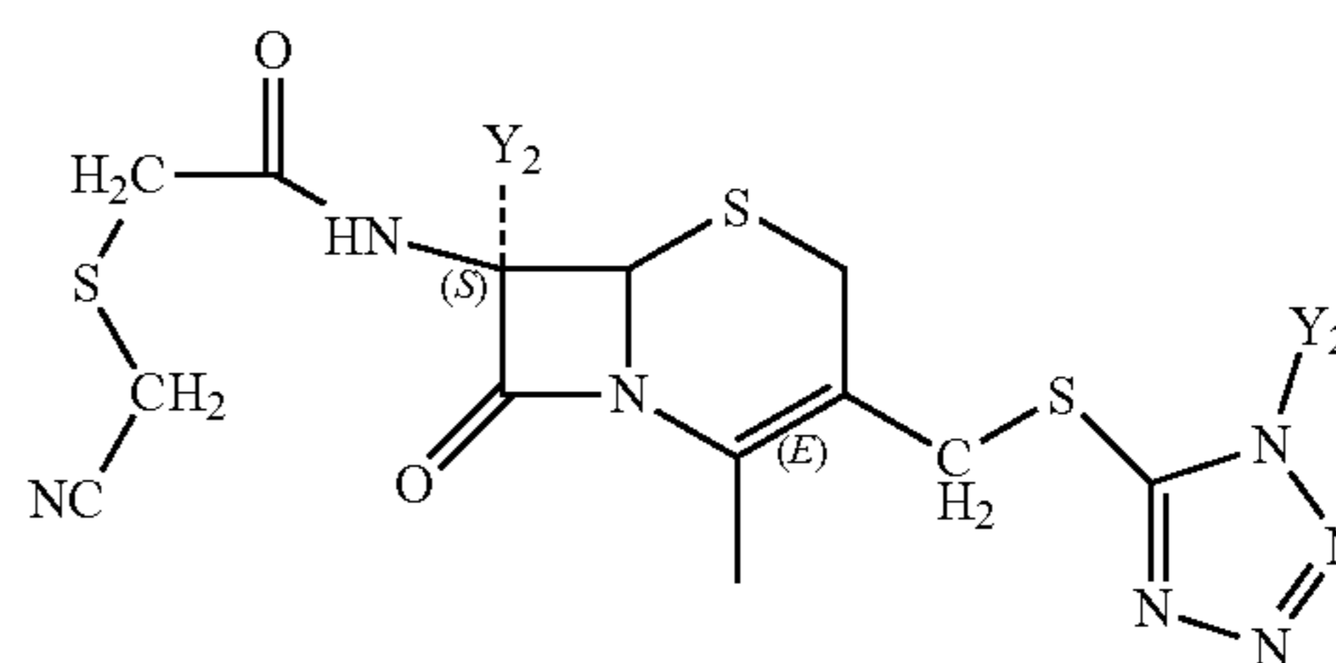
Structure FP-54
