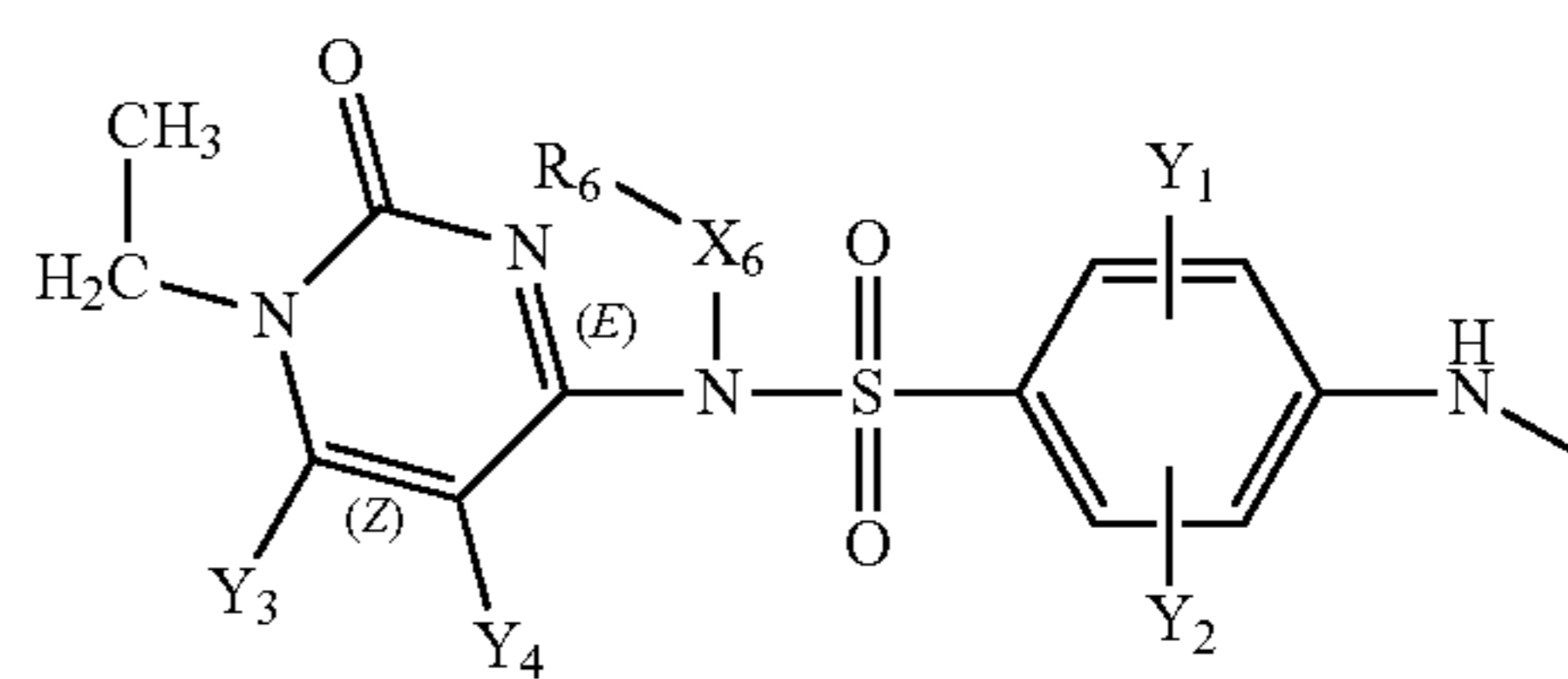
Structure FS-6
