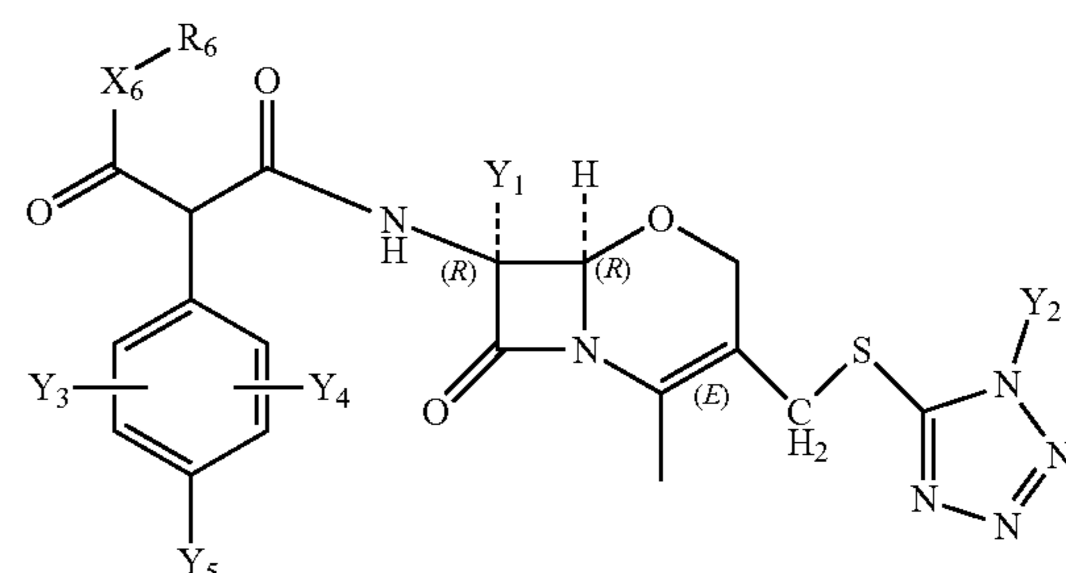
Structure FP-67
