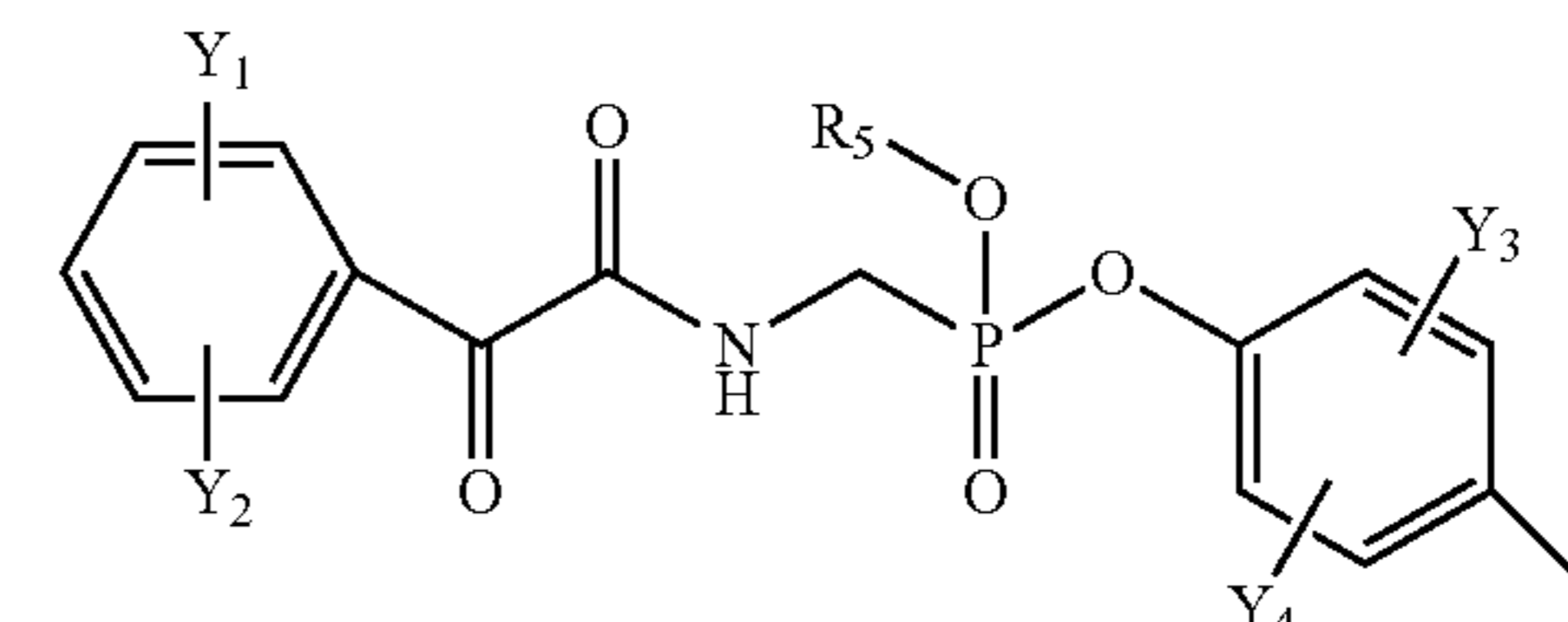
Structure FI-16
