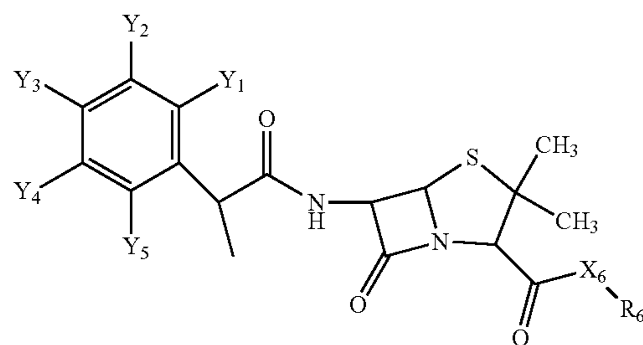
Structure FP-13
