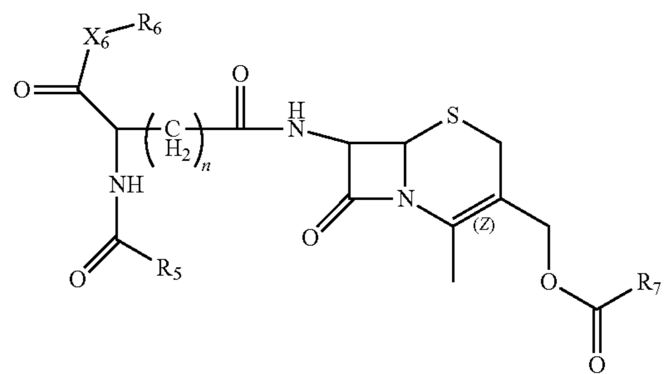
Structure FP-15
