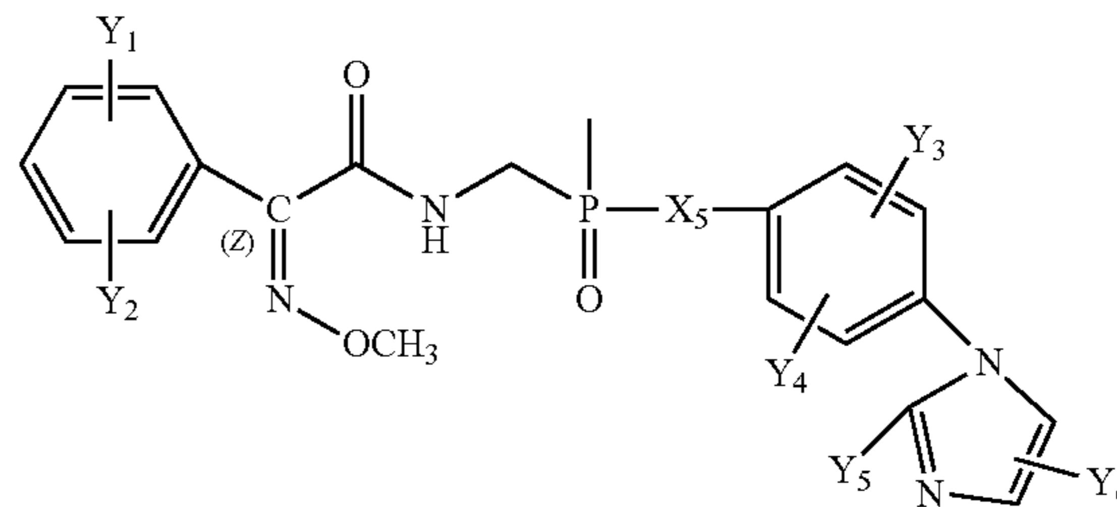
Structure FI-28
