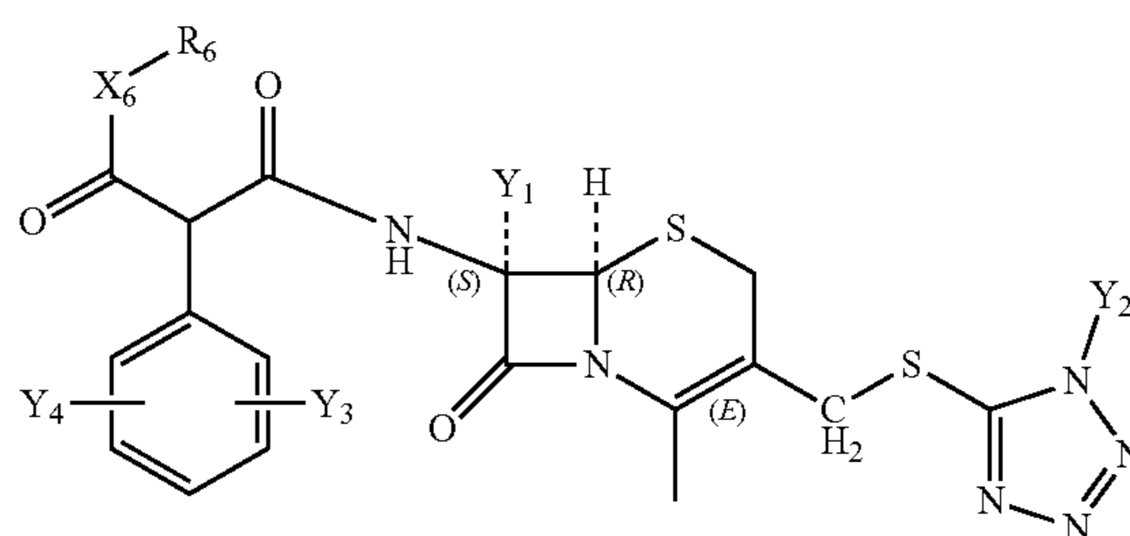
Structure FP-64
