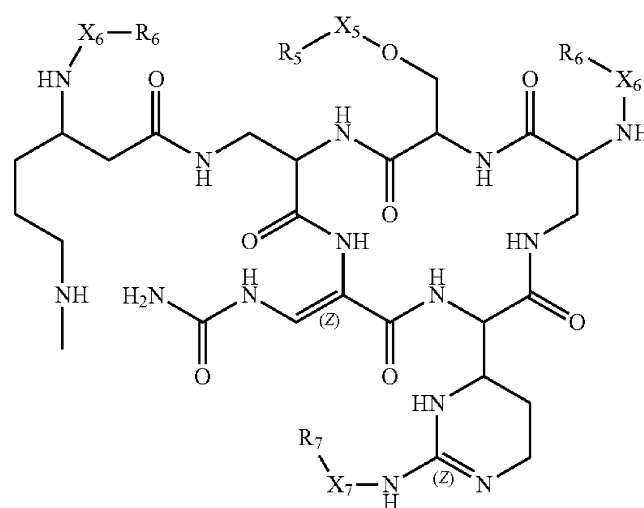
Structure FT-11
