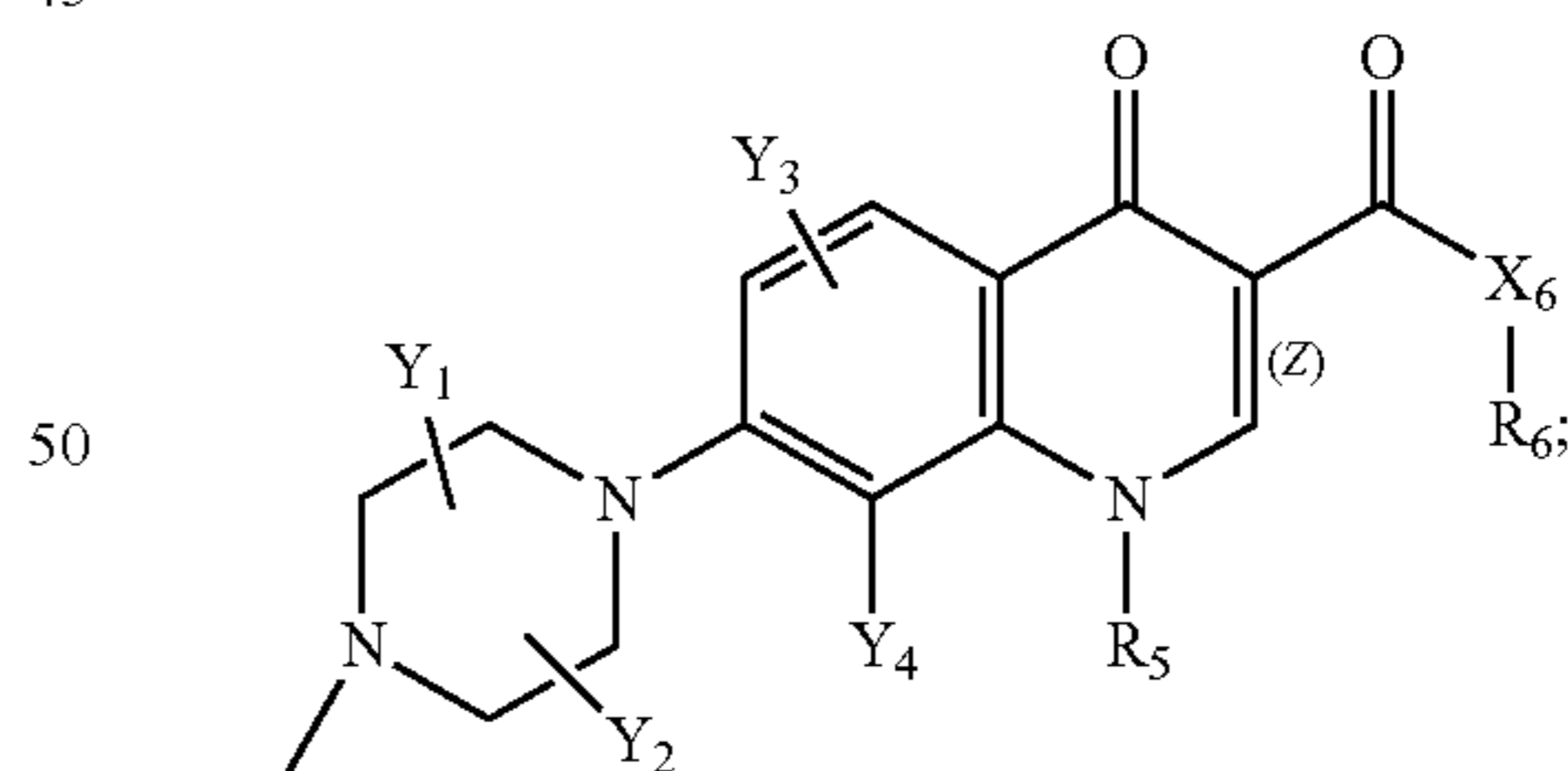
Structure FT-16
