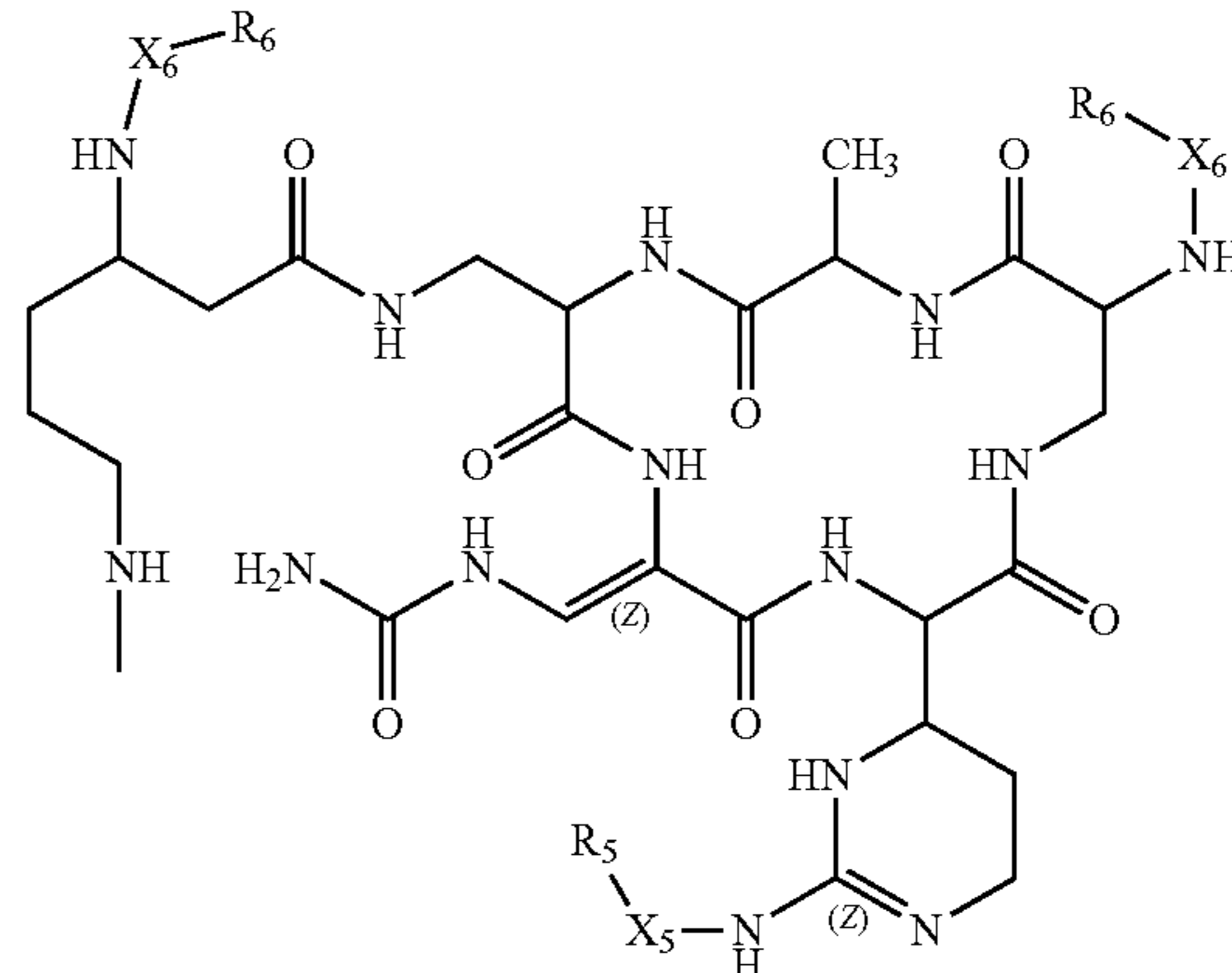
Structure FT-10
