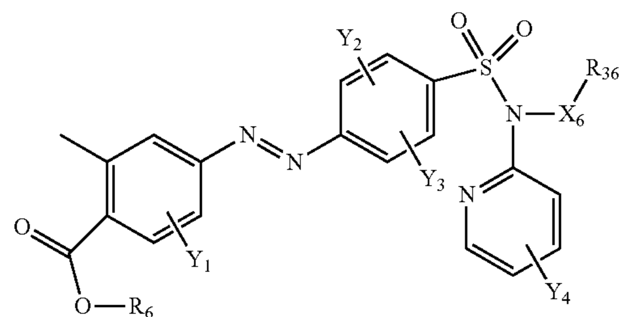
Structure FS-10
