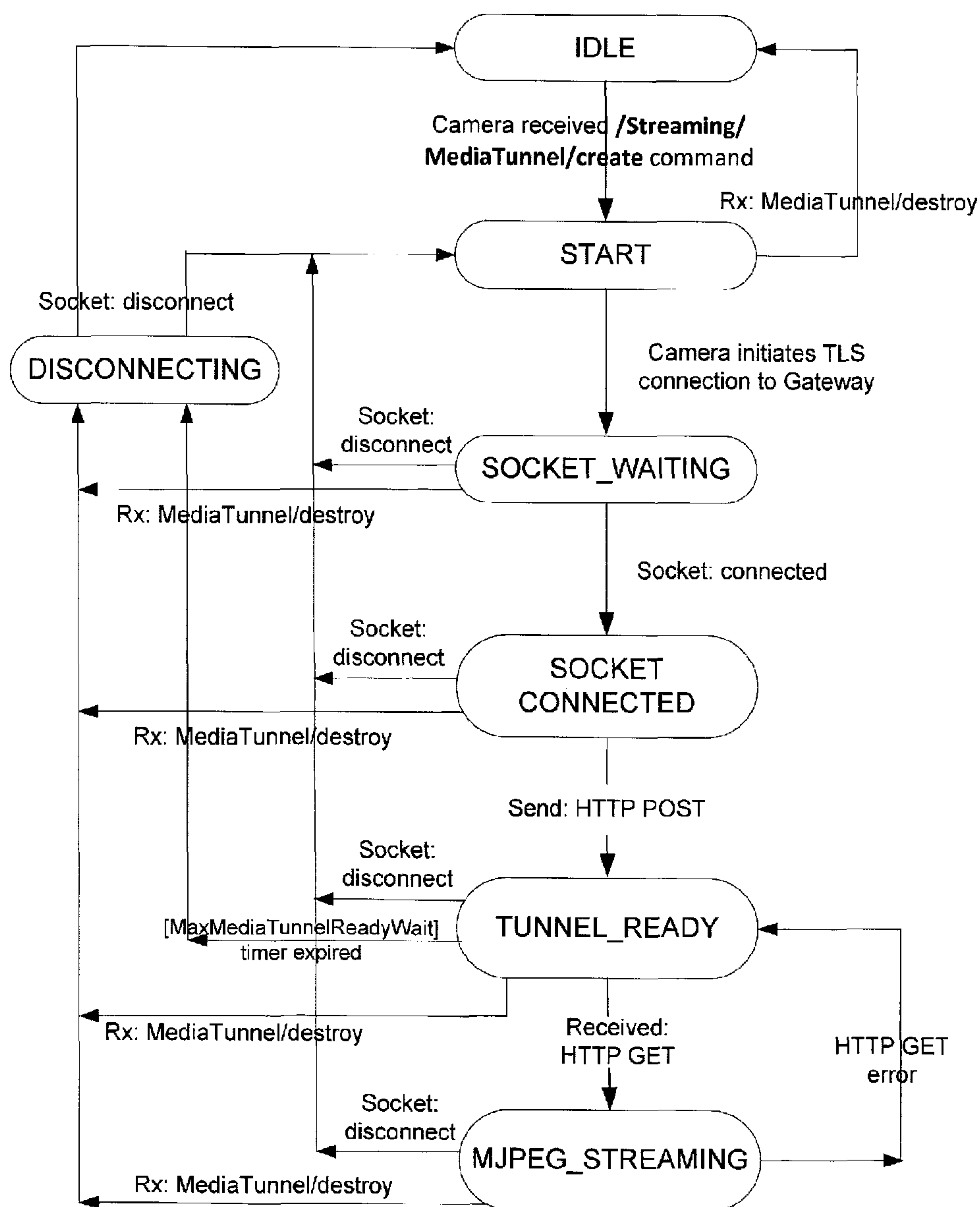
MJPEG Media Channel State Transition Diagram
