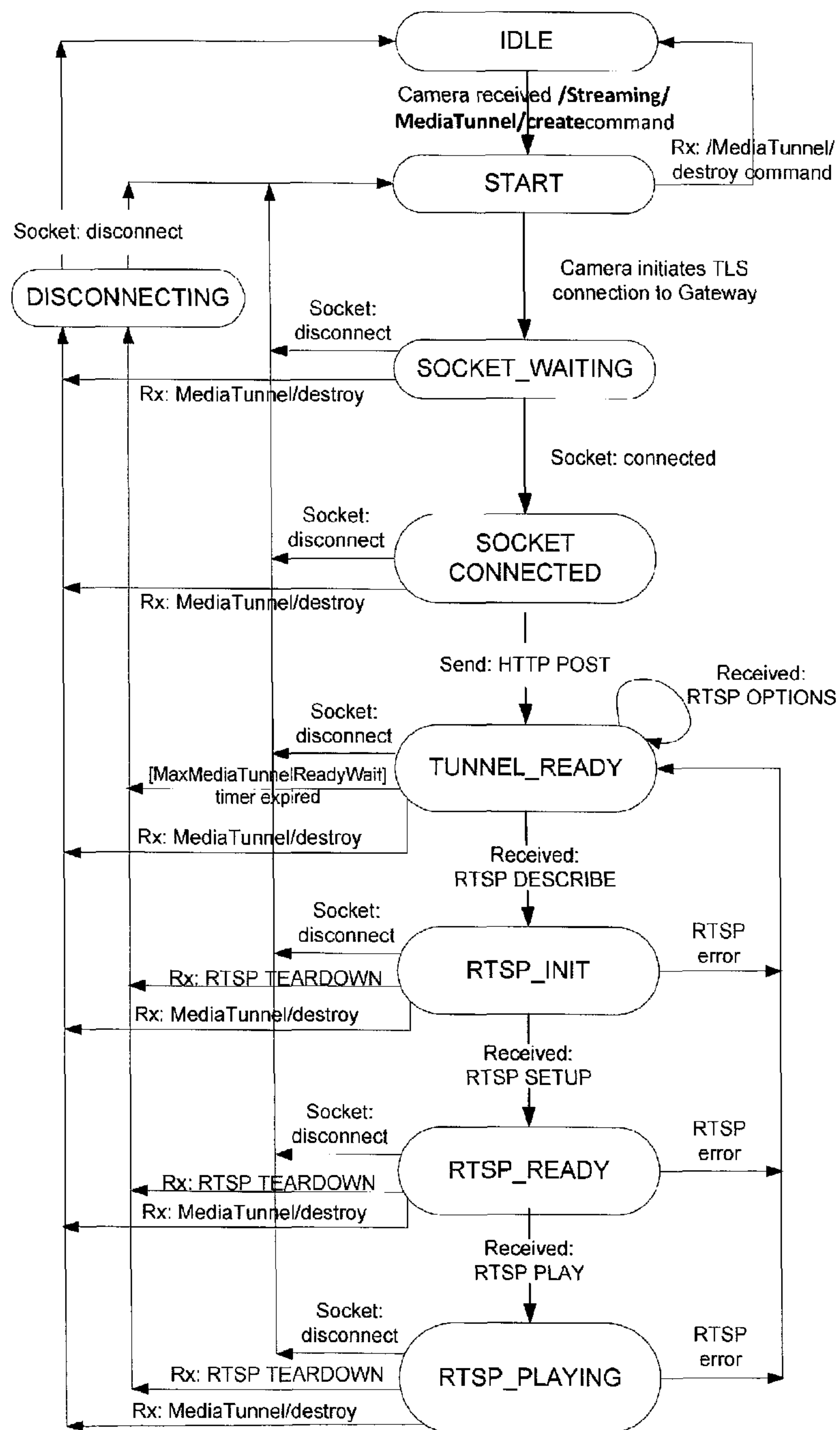
RTSP Tunnel State Transition Diagram
