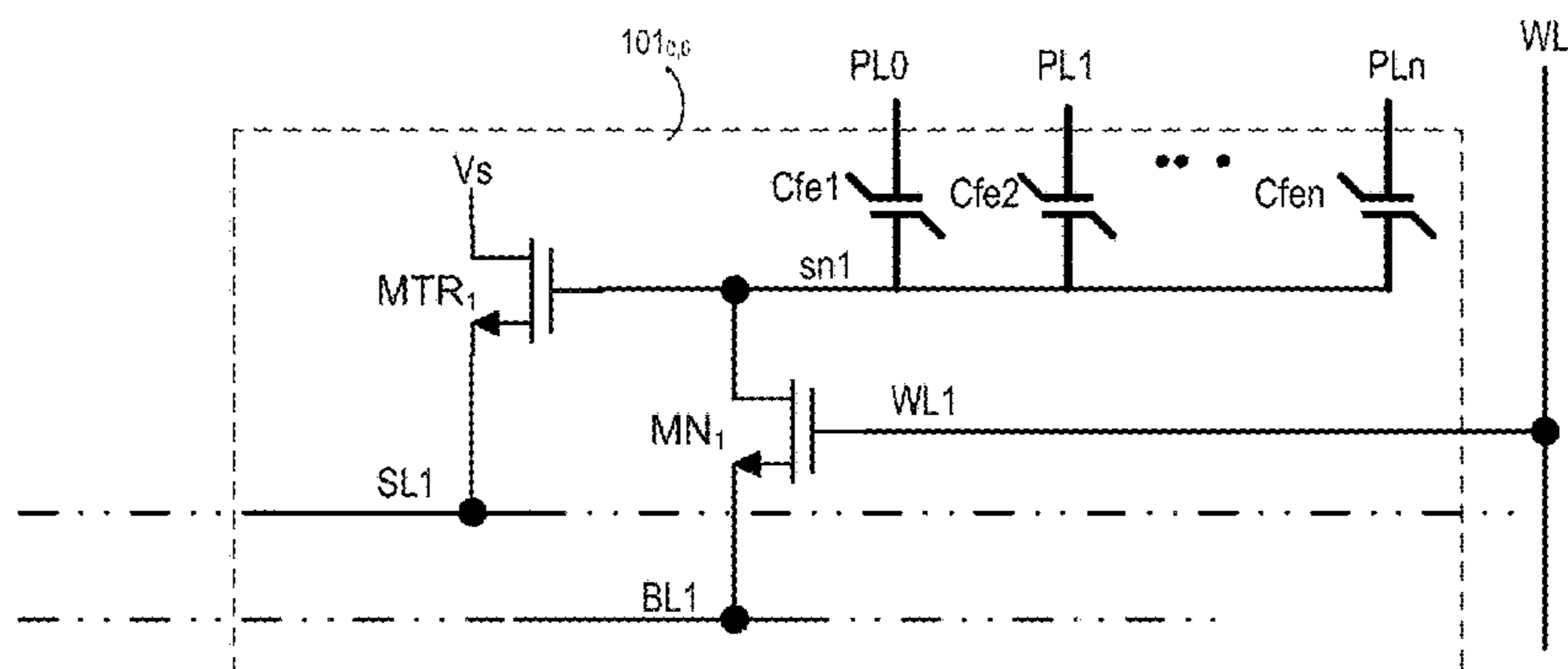
Multi-element FE gain bit-cell
