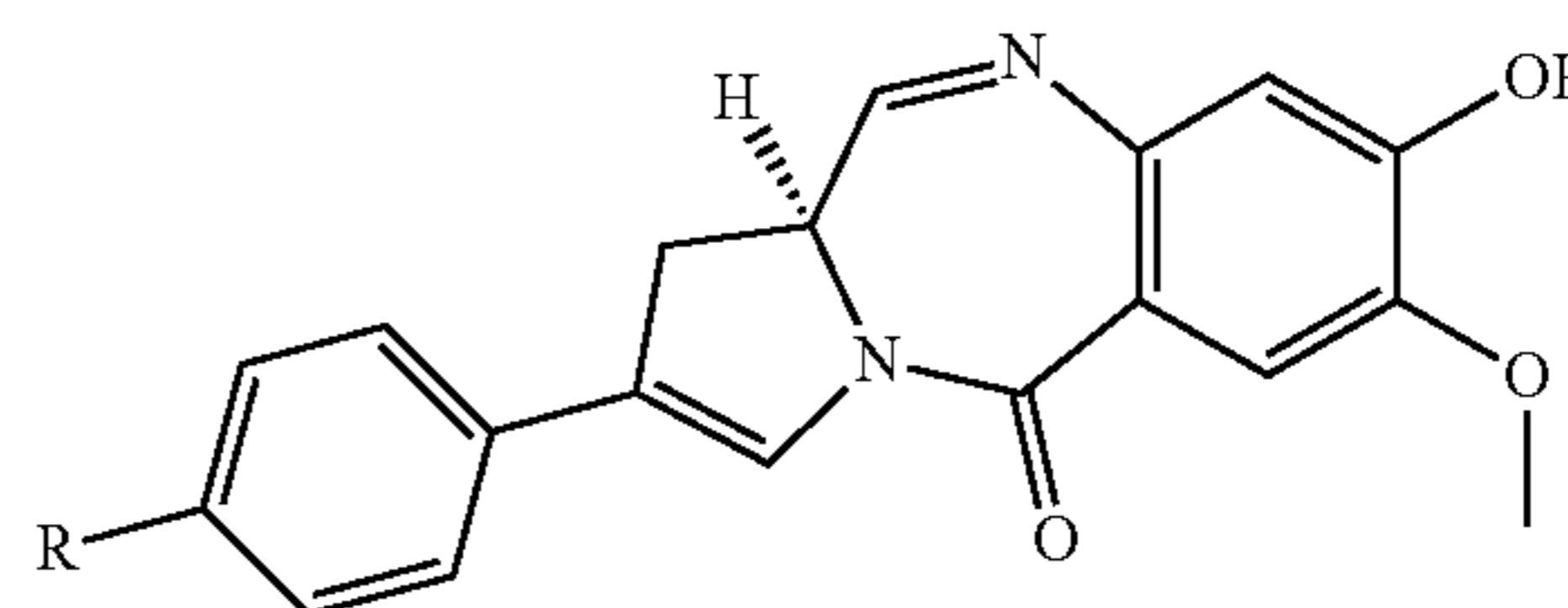
C2-aryl substituted PBD monomer
