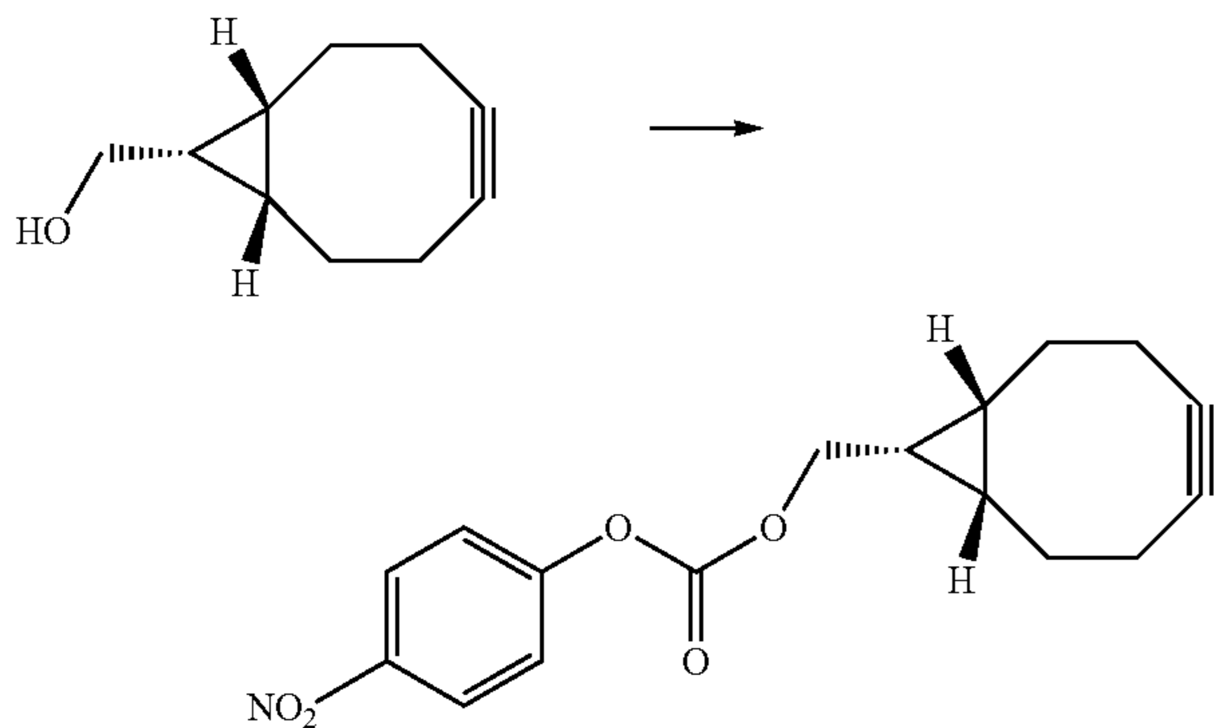
BCN-PNP
