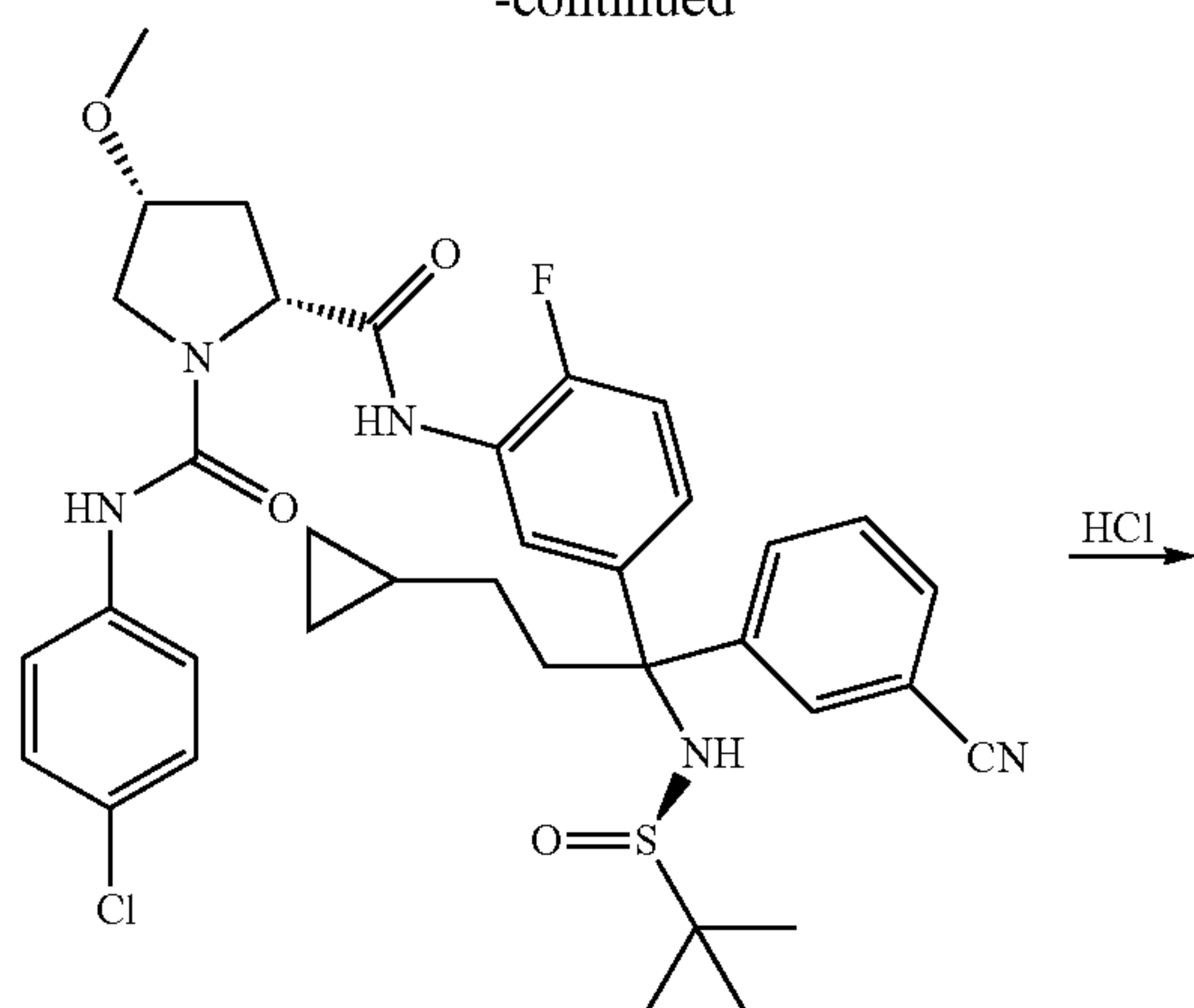
17a (-)-isomer
