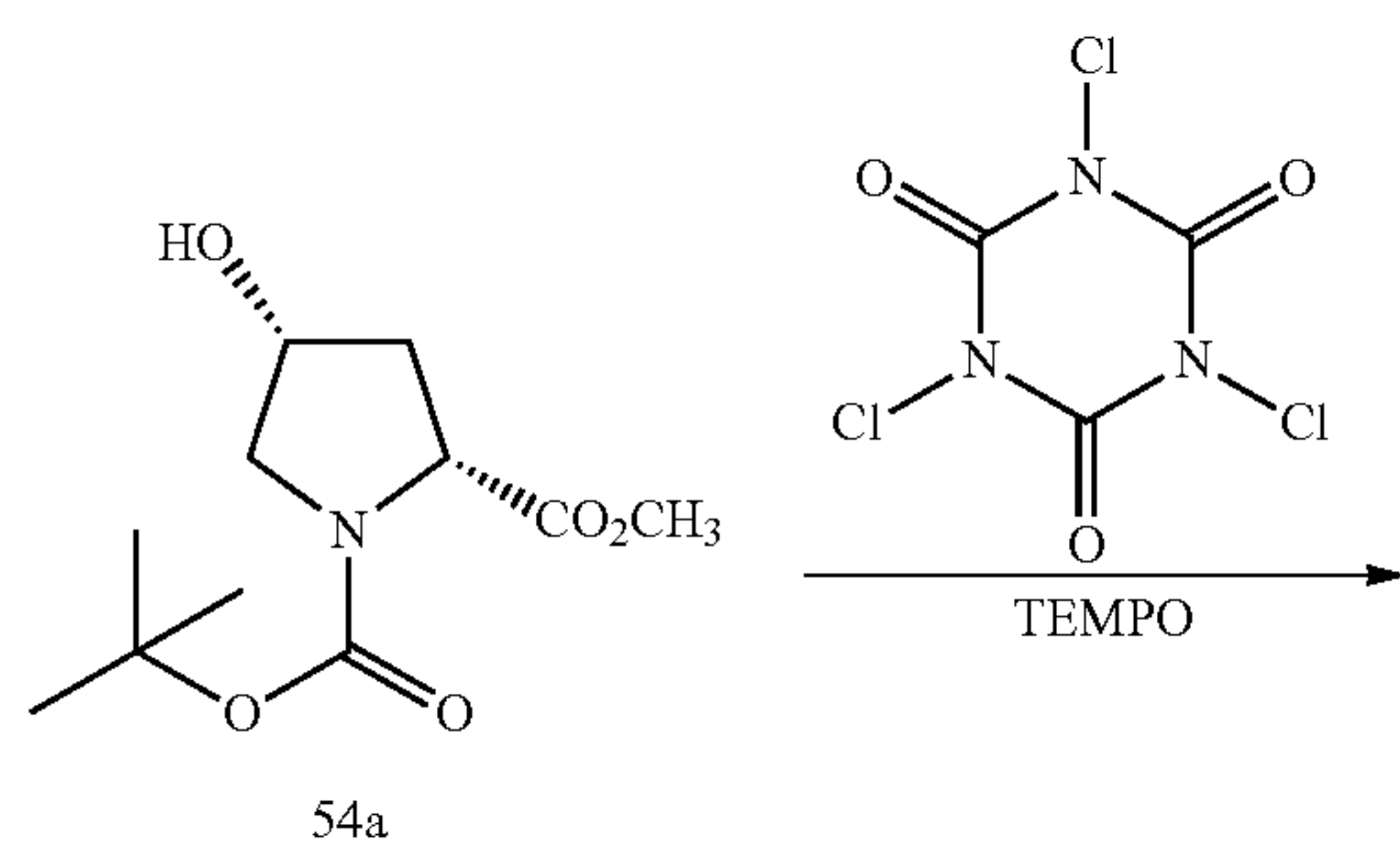
Scheme 54
