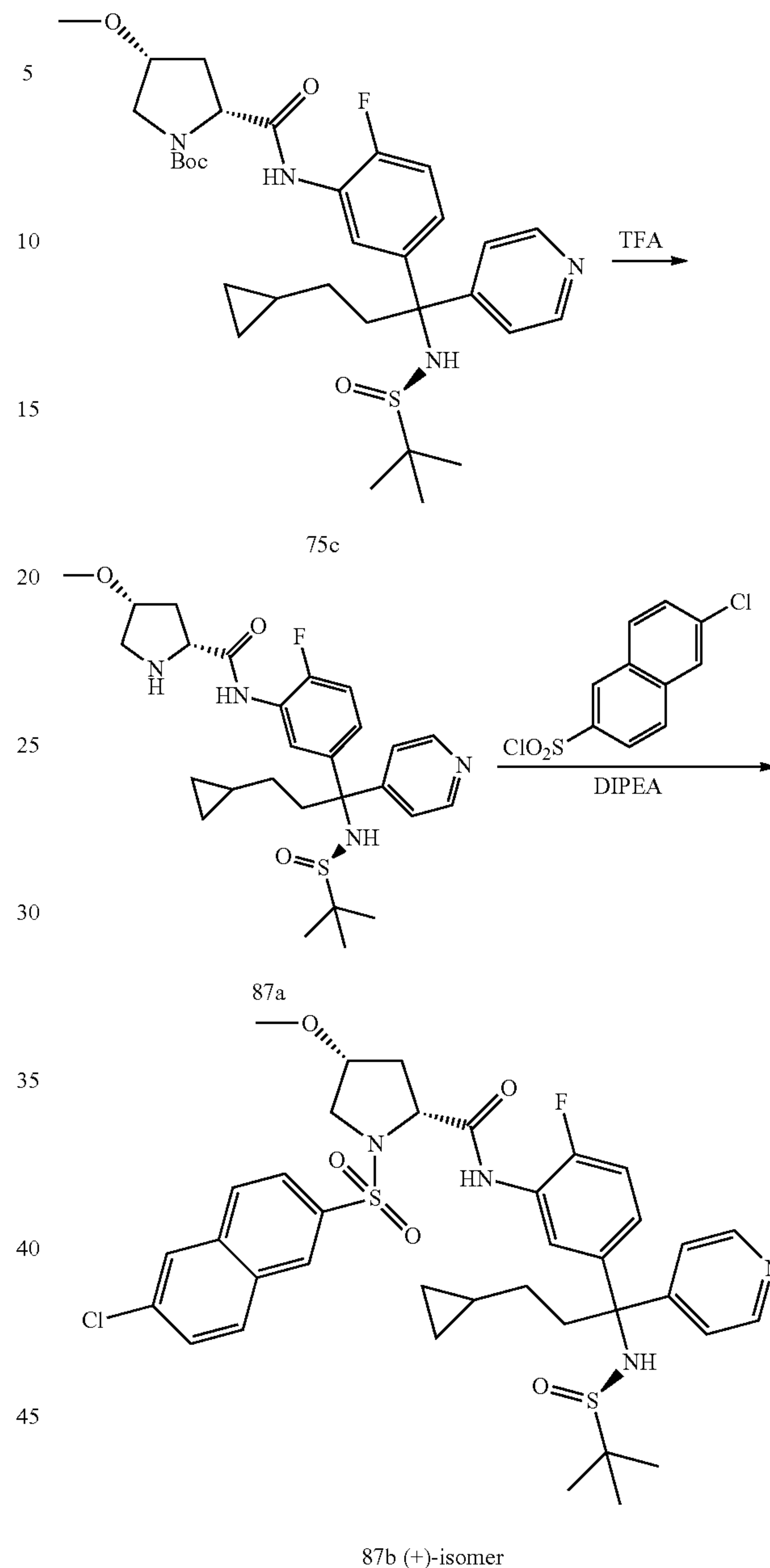
Scheme 87
