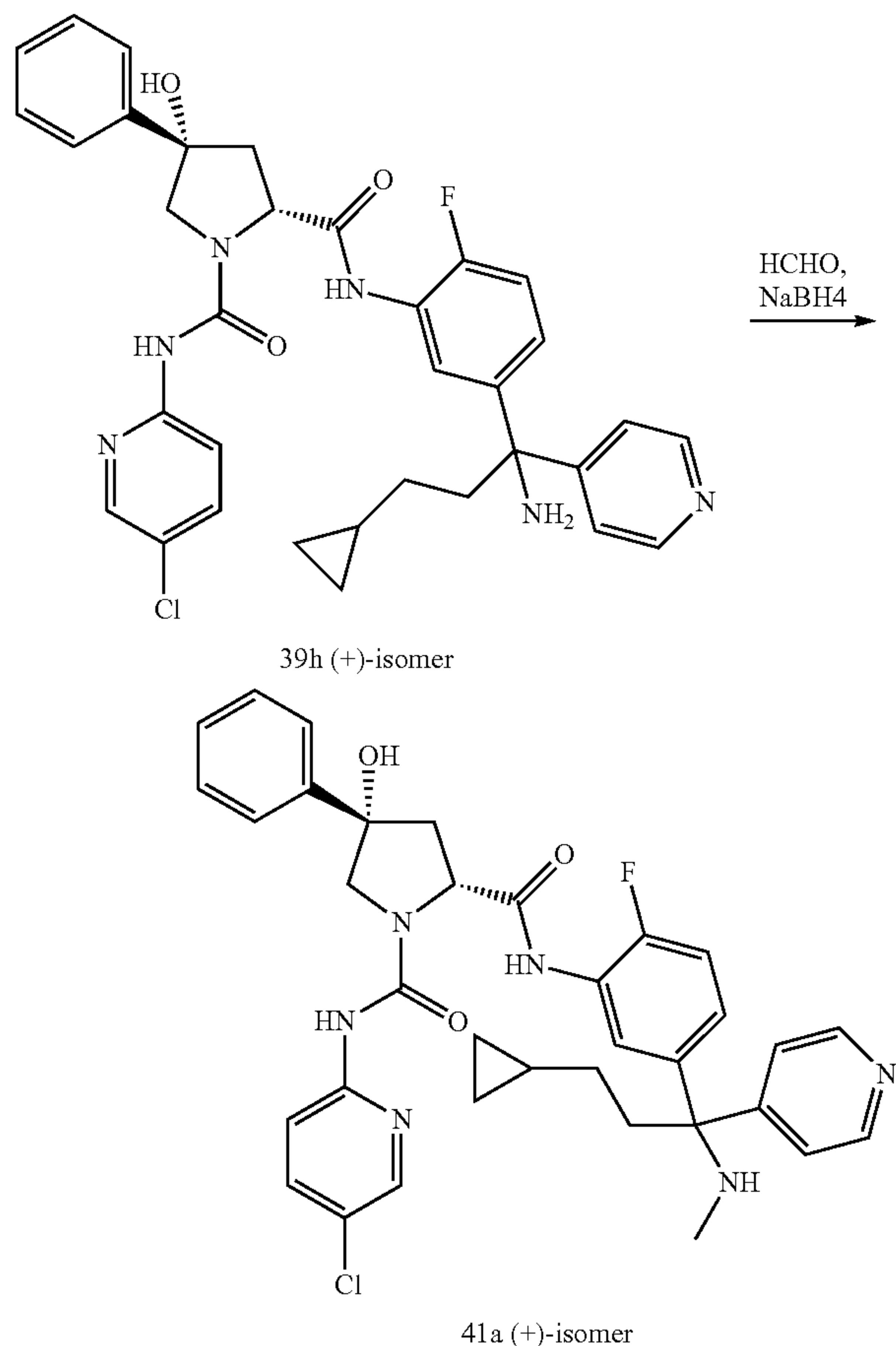
Scheme 41
