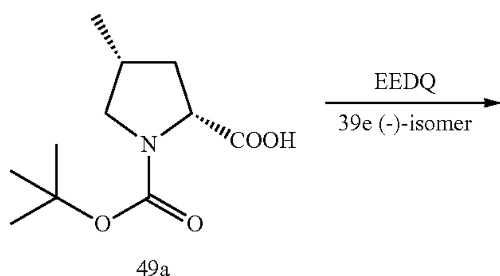
Scheme 49
