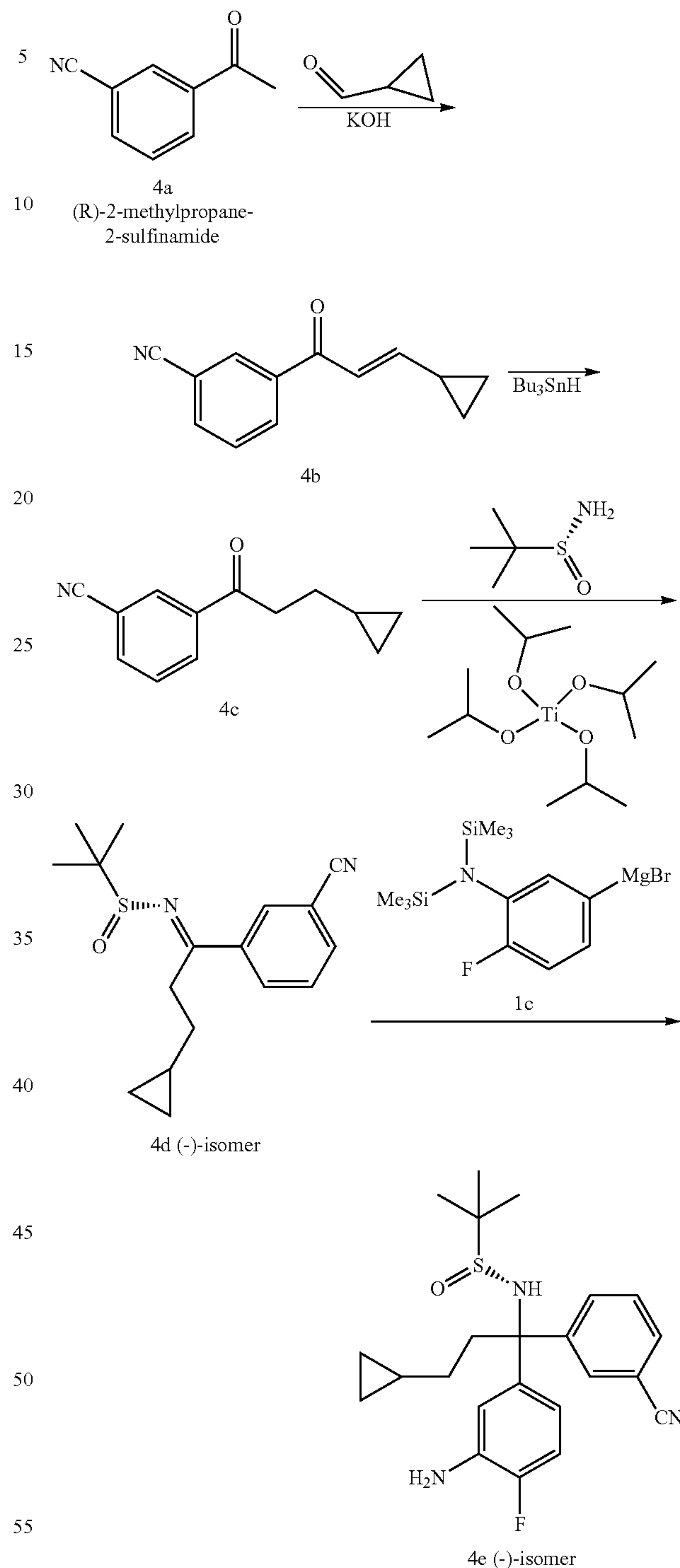
Scheme 4
