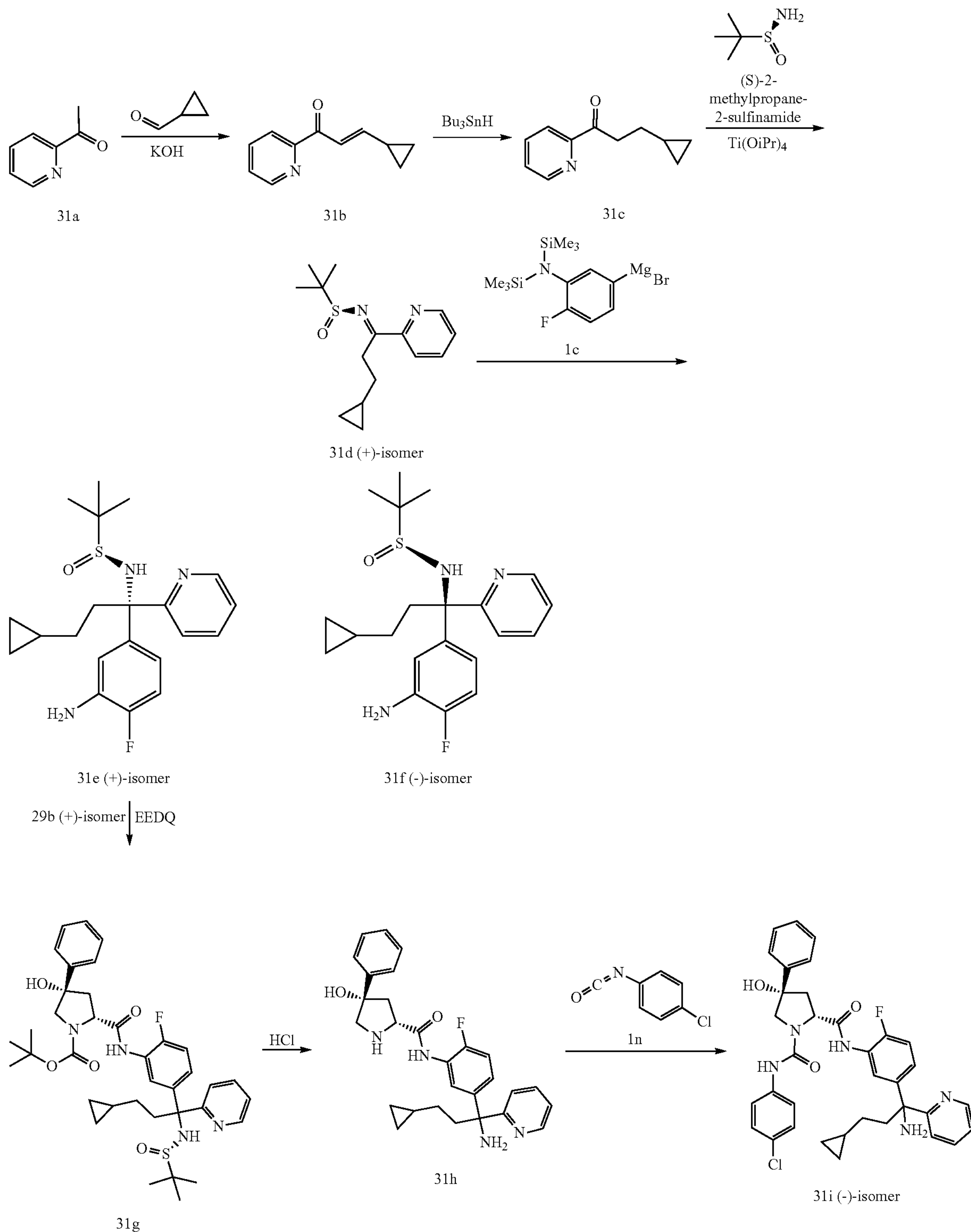
Scheme 31
