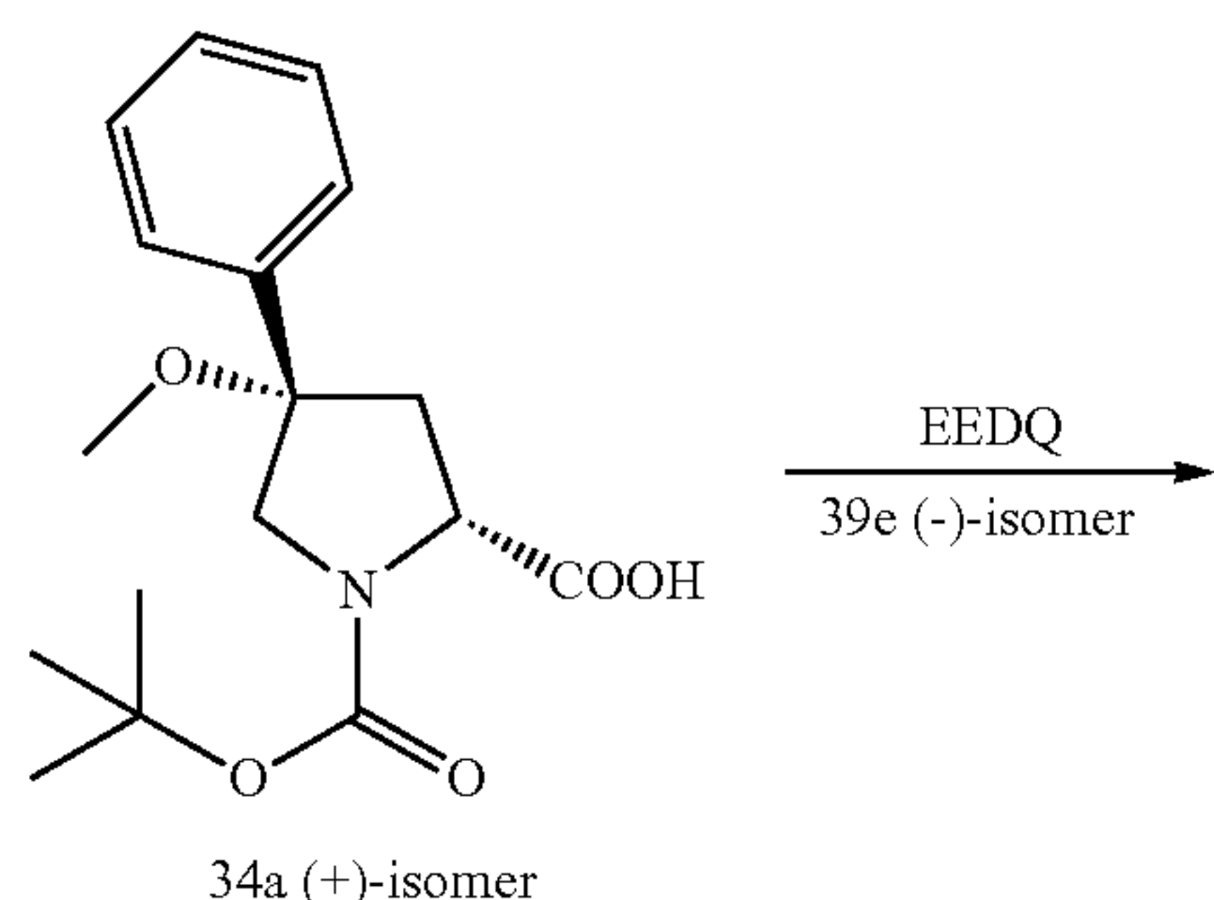
Scheme 45
