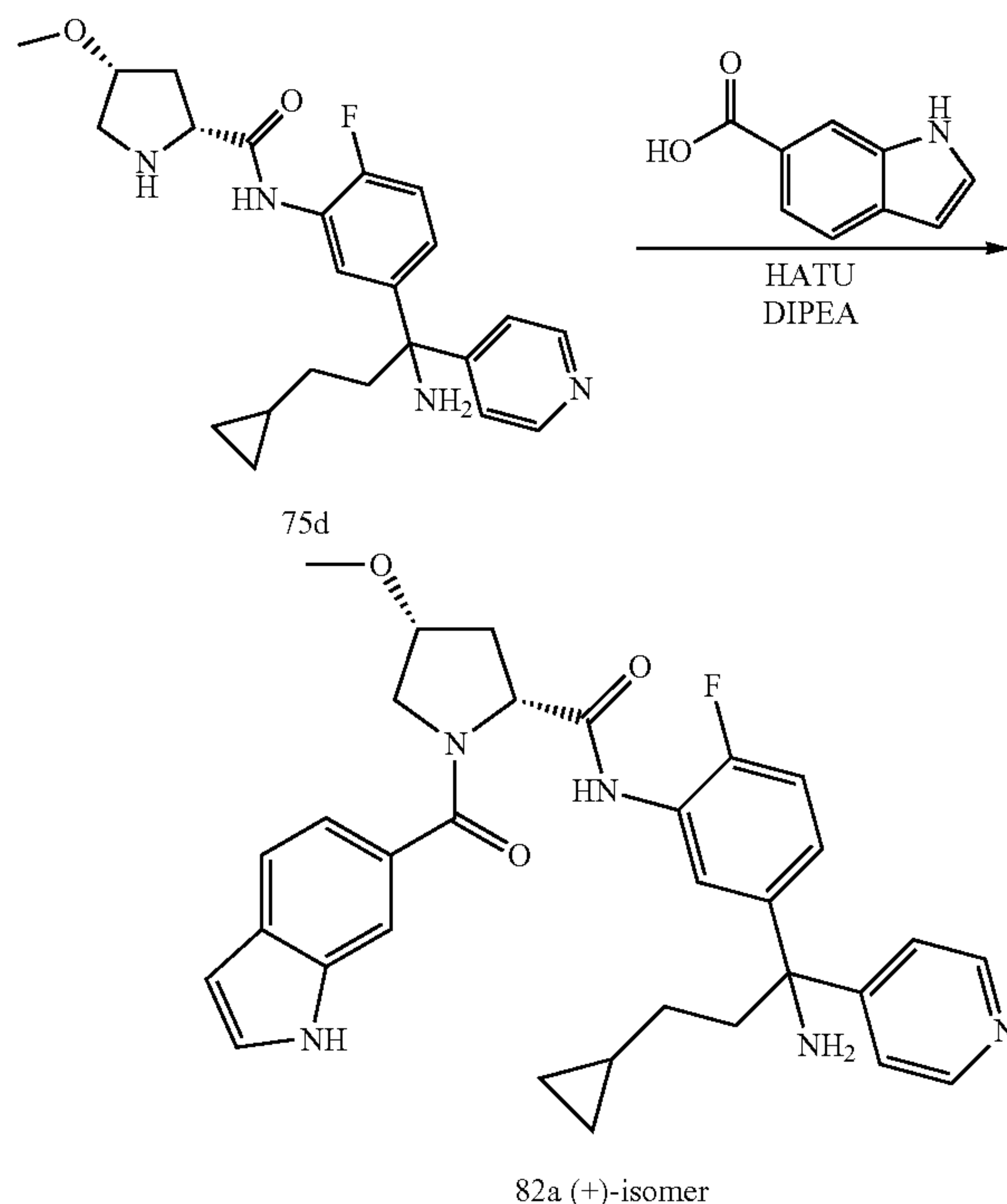
Scheme 82
