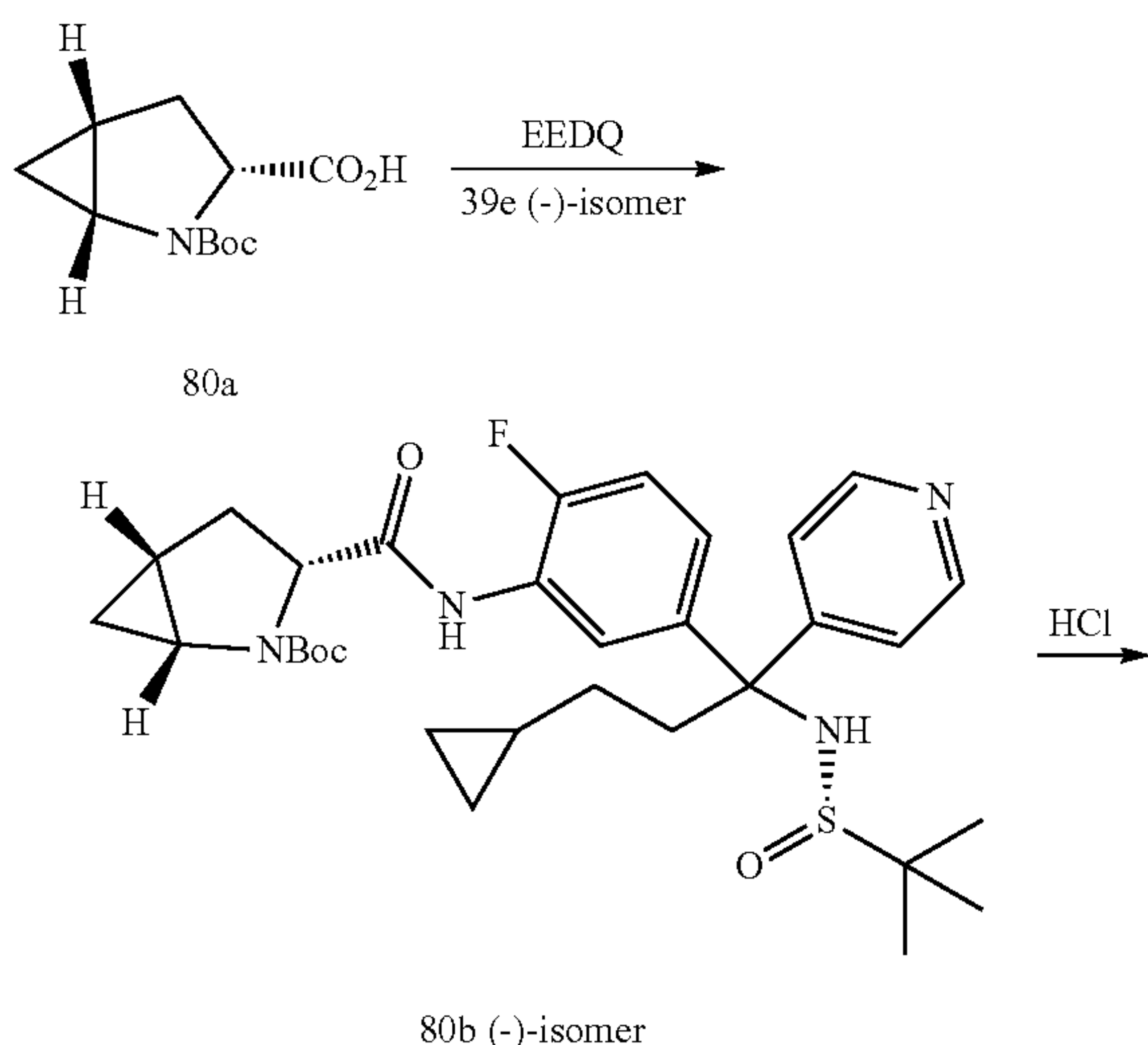
Scheme 80
