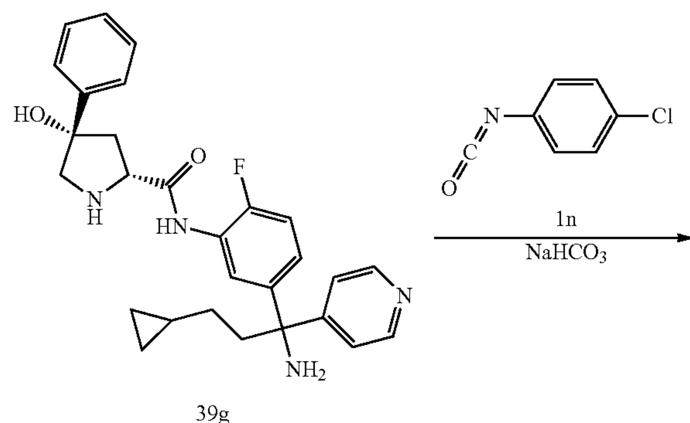
Scheme 40
