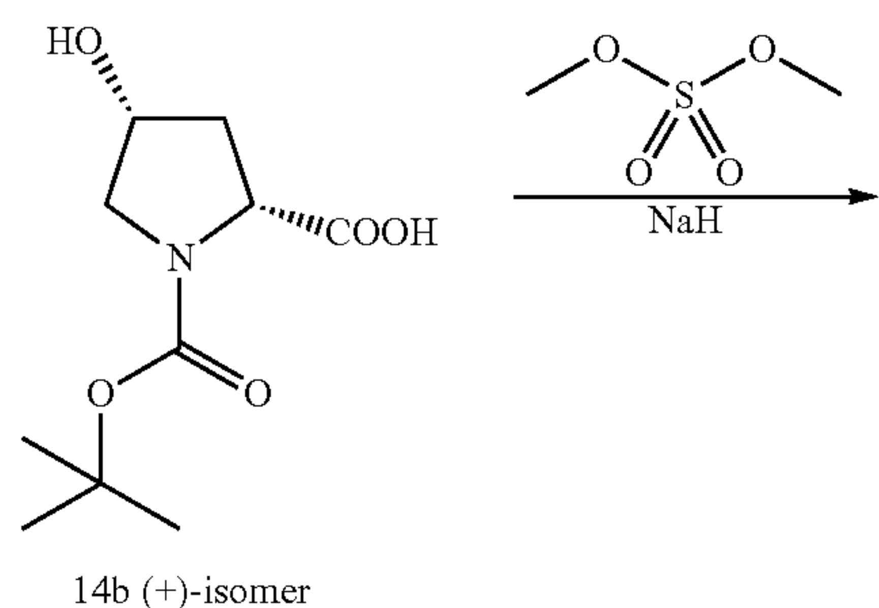
Scheme 36
