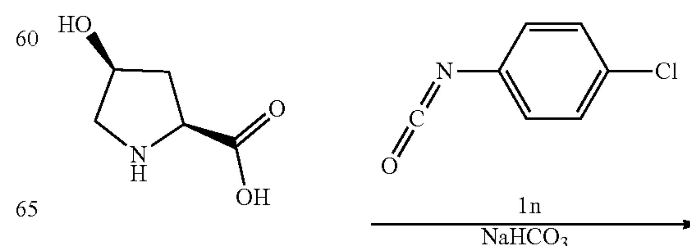
Scheme 10
