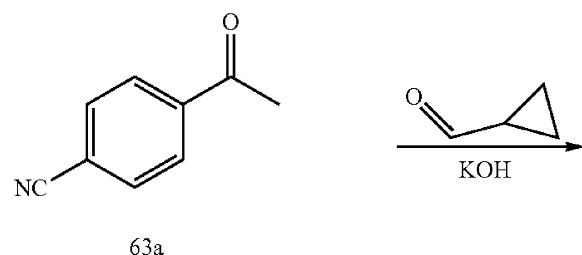
Scheme 63
