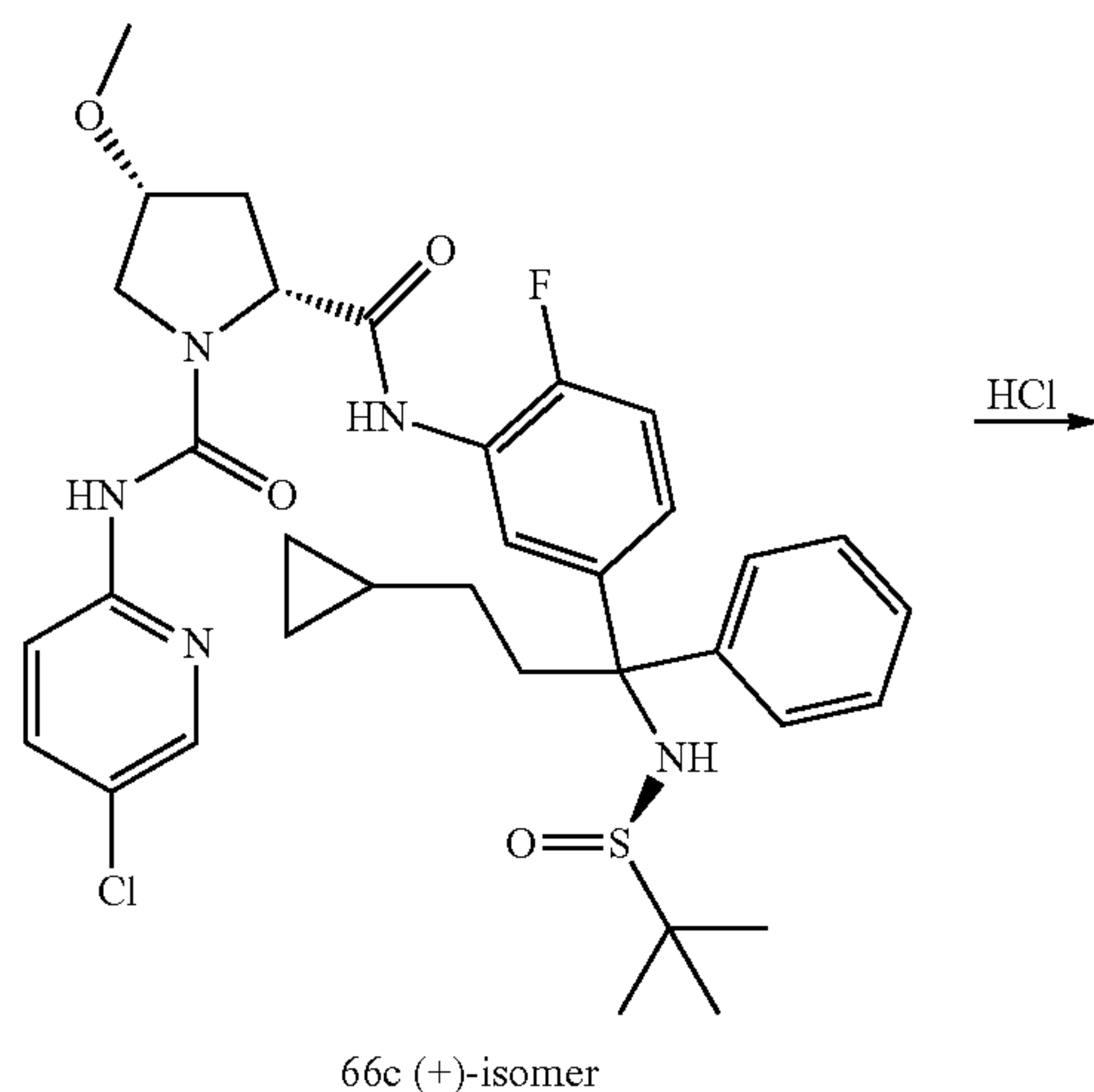
Scheme 67
