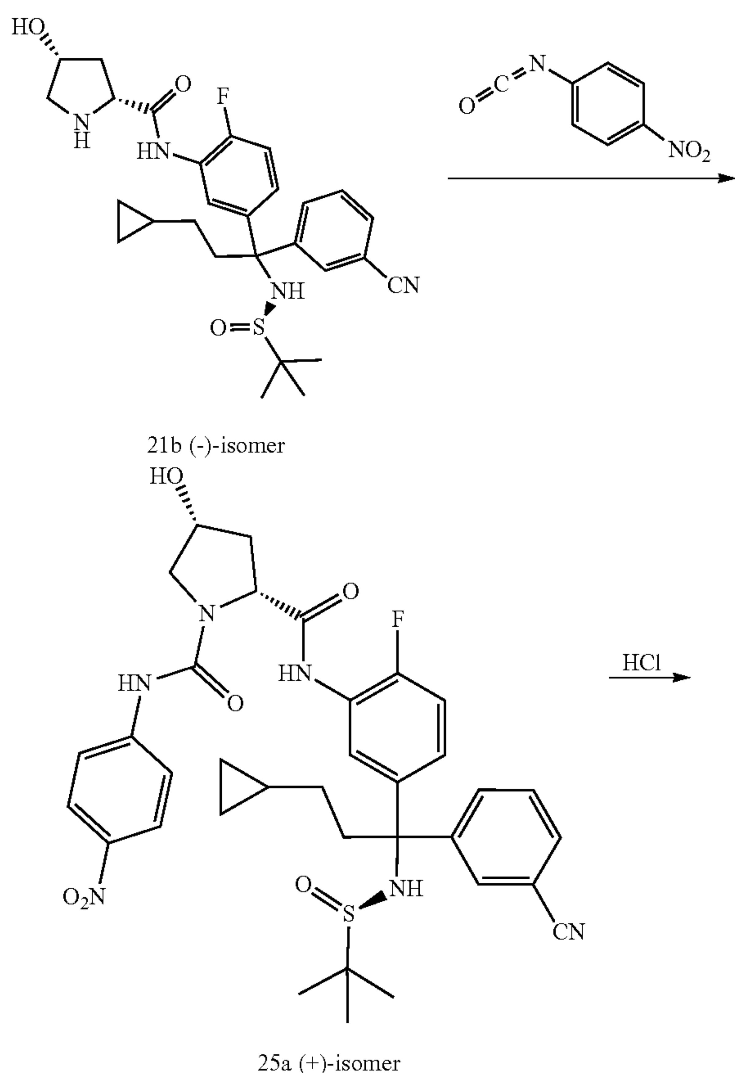
Scheme 25
