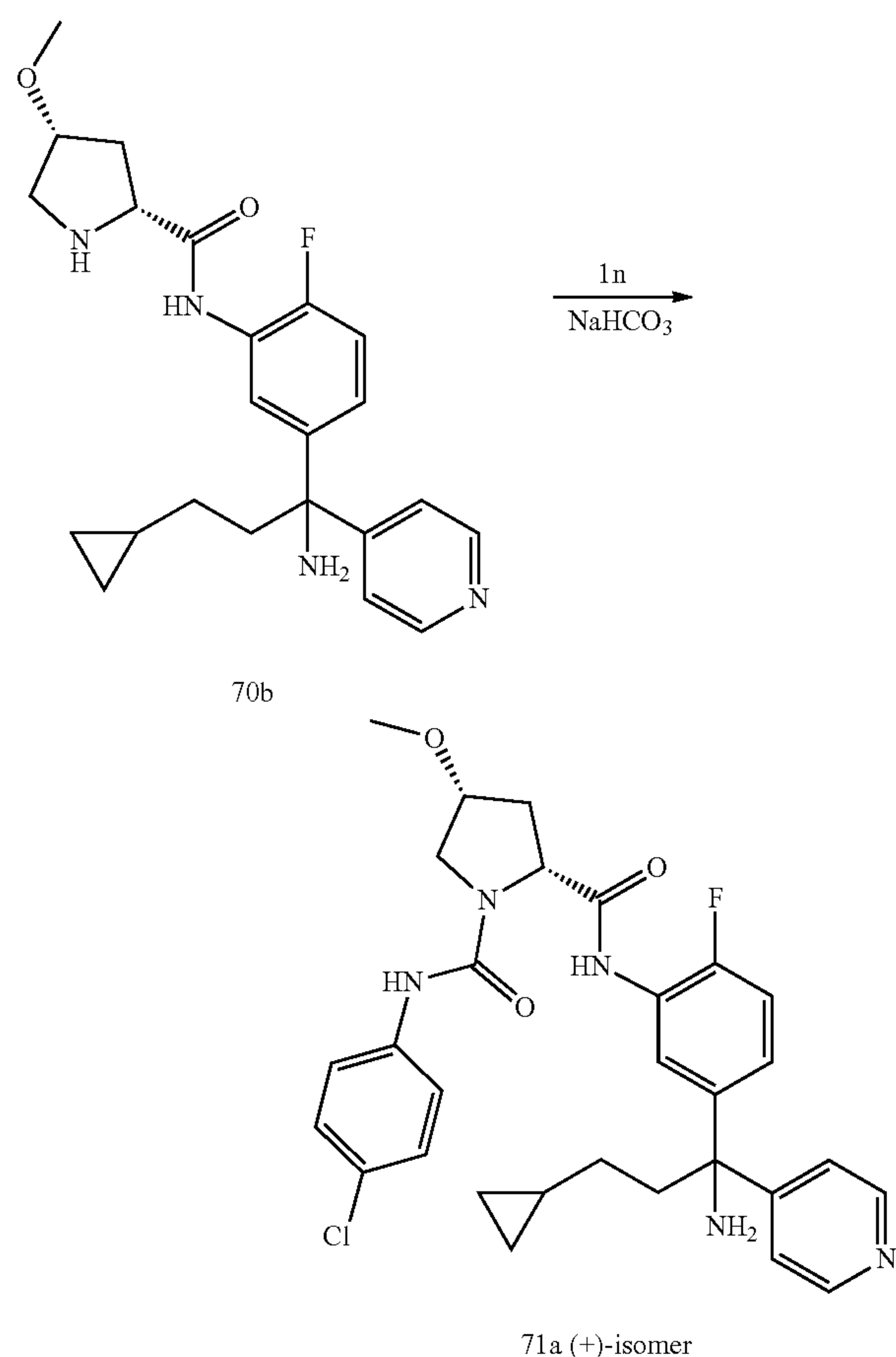
Scheme 71
