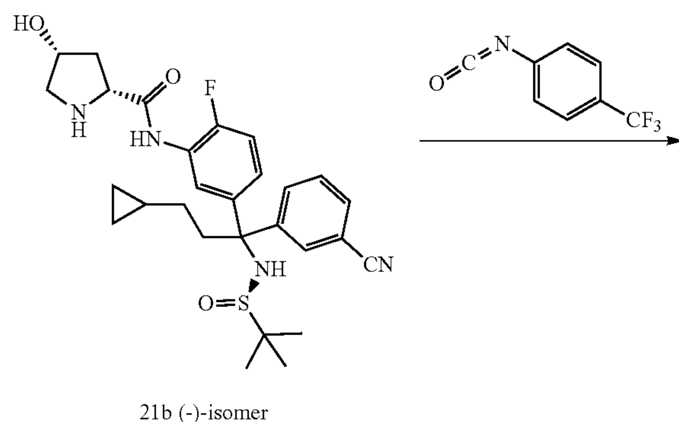
Scheme 27
