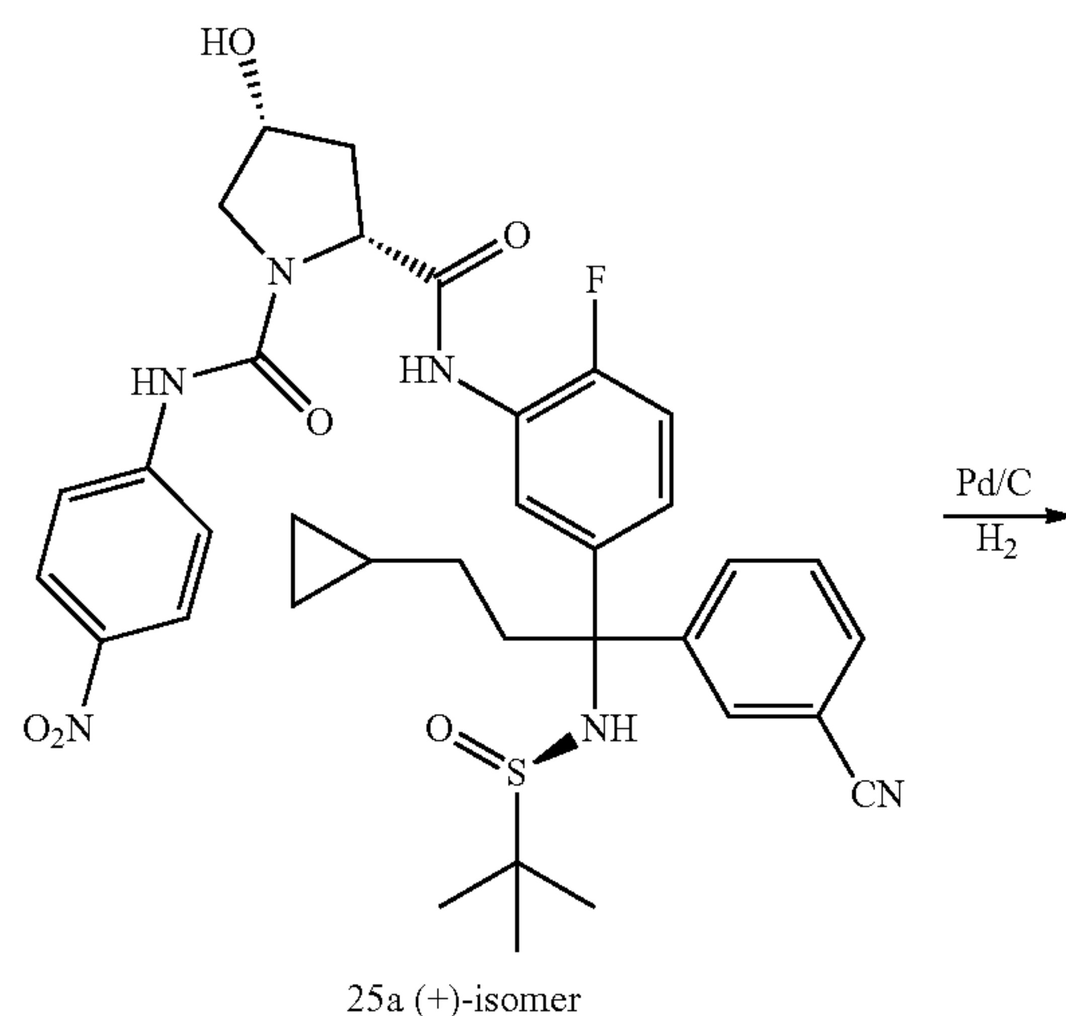
Scheme 28
