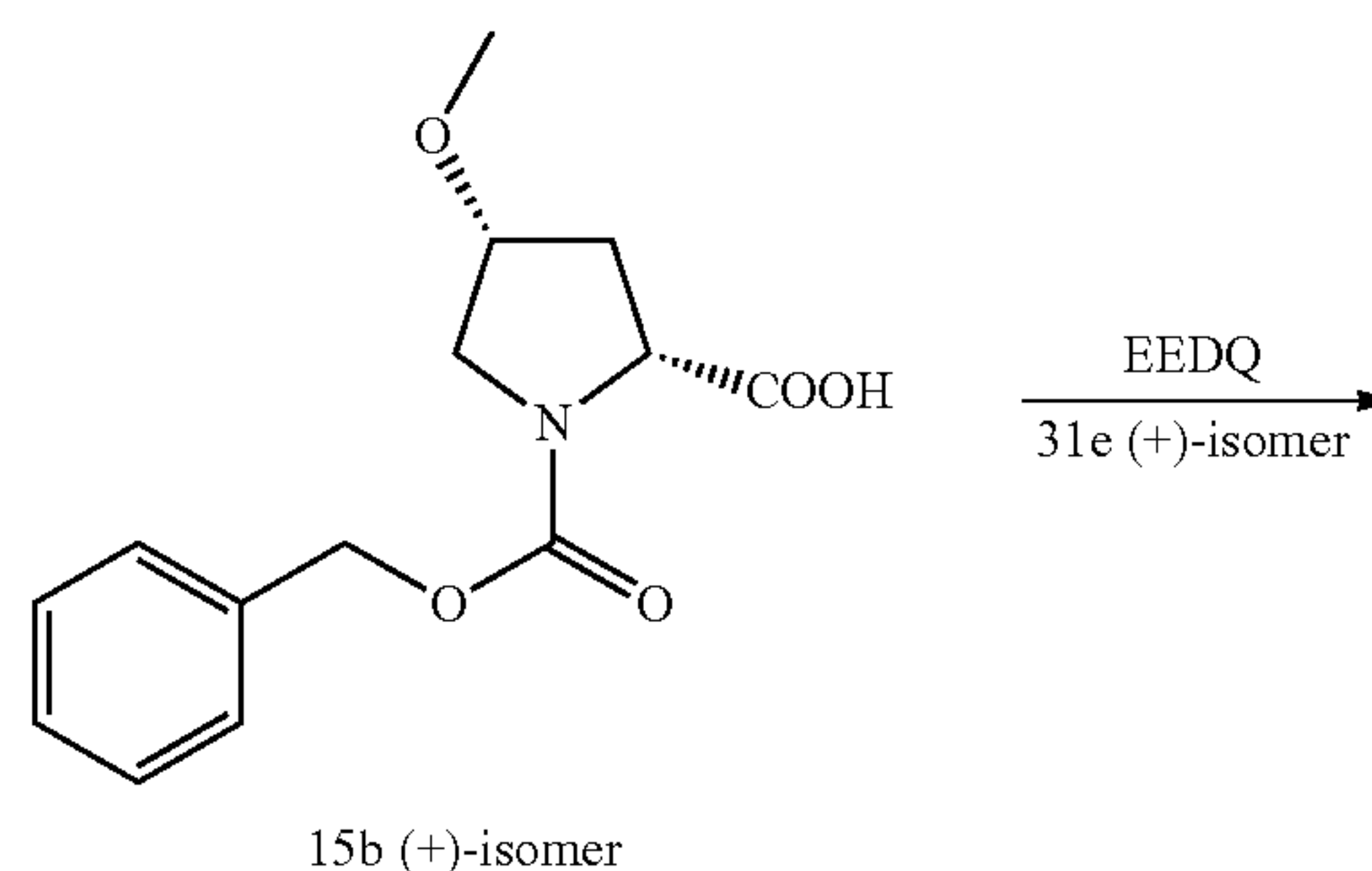
Scheme 37
