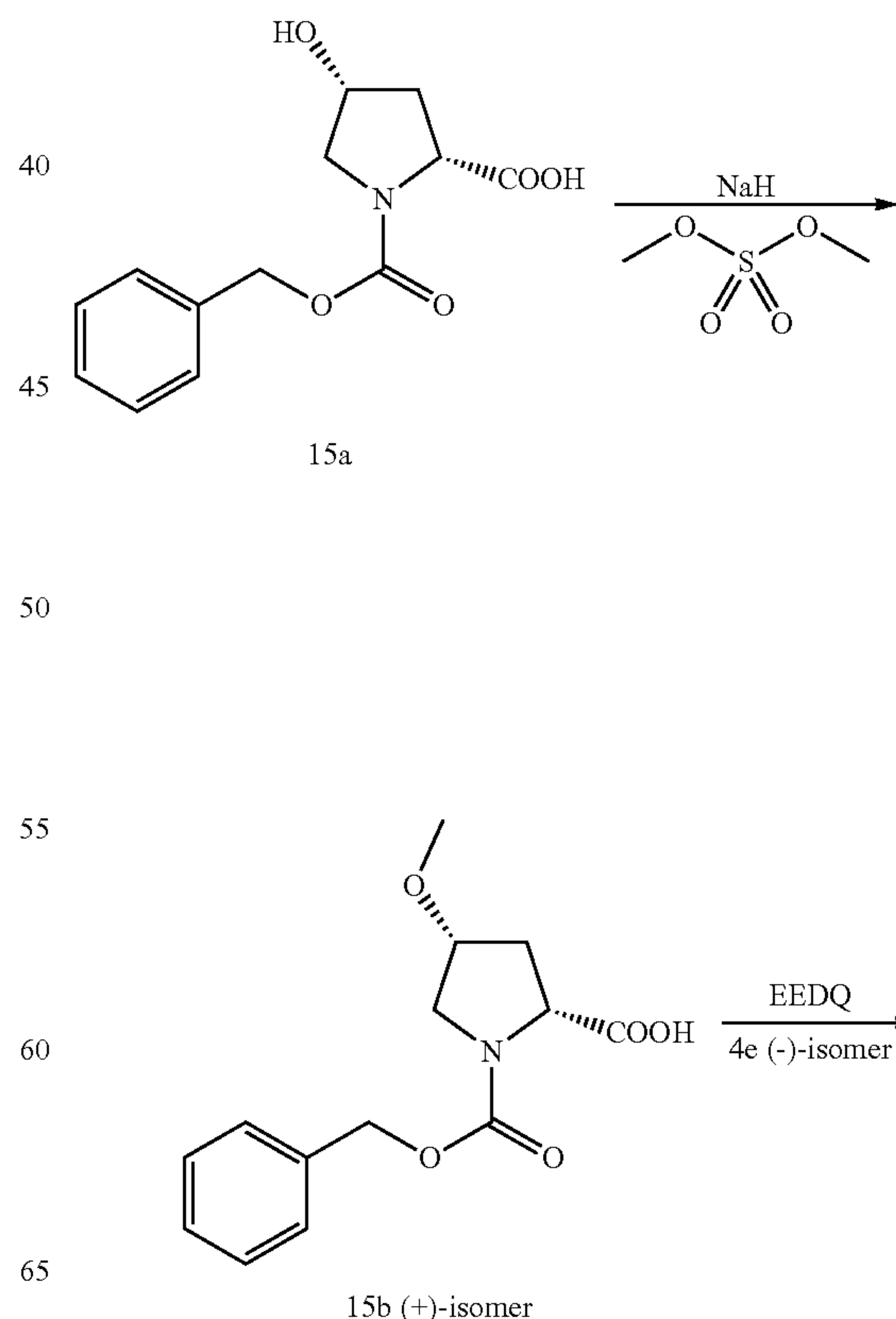
Scheme 15
