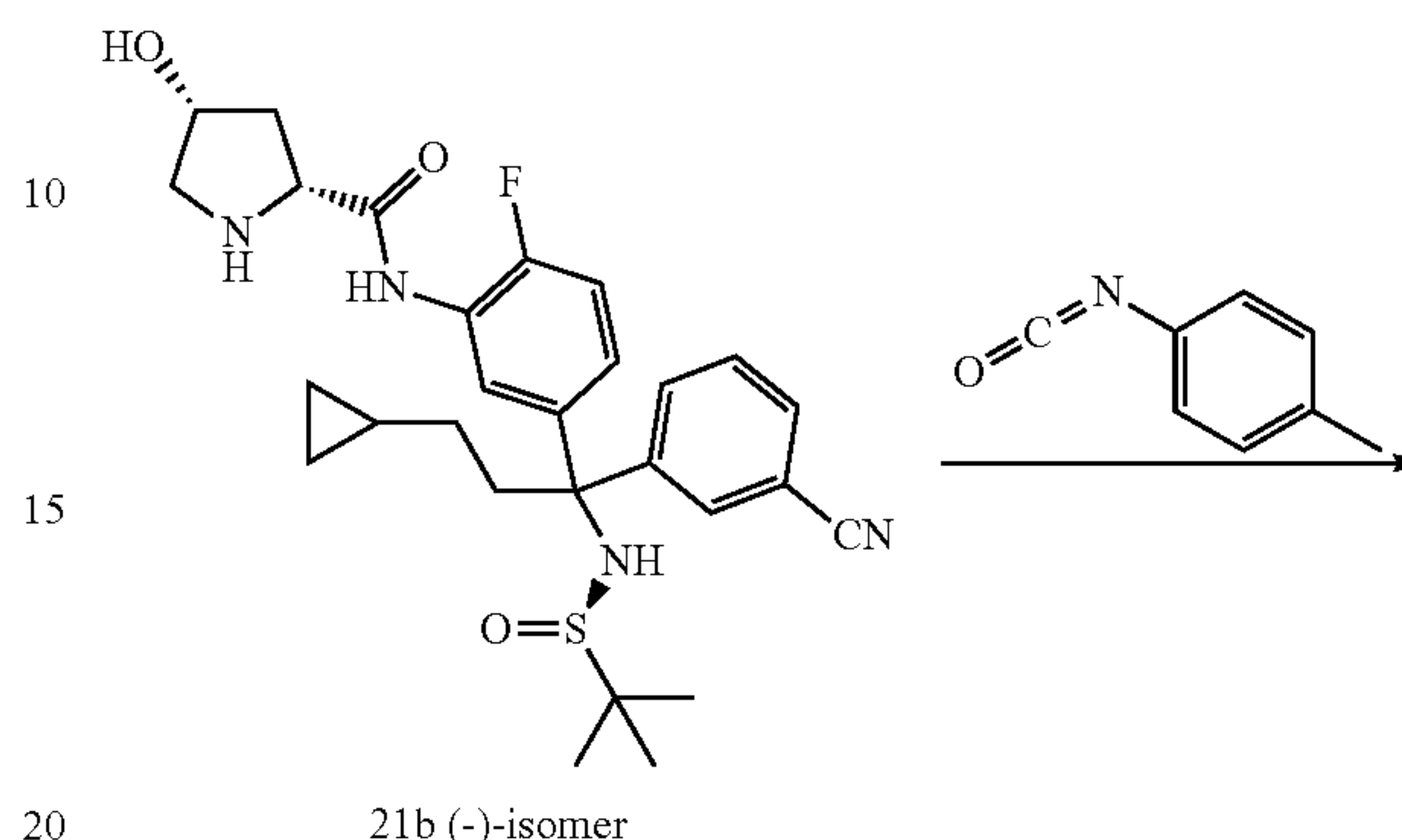
Scheme 22
