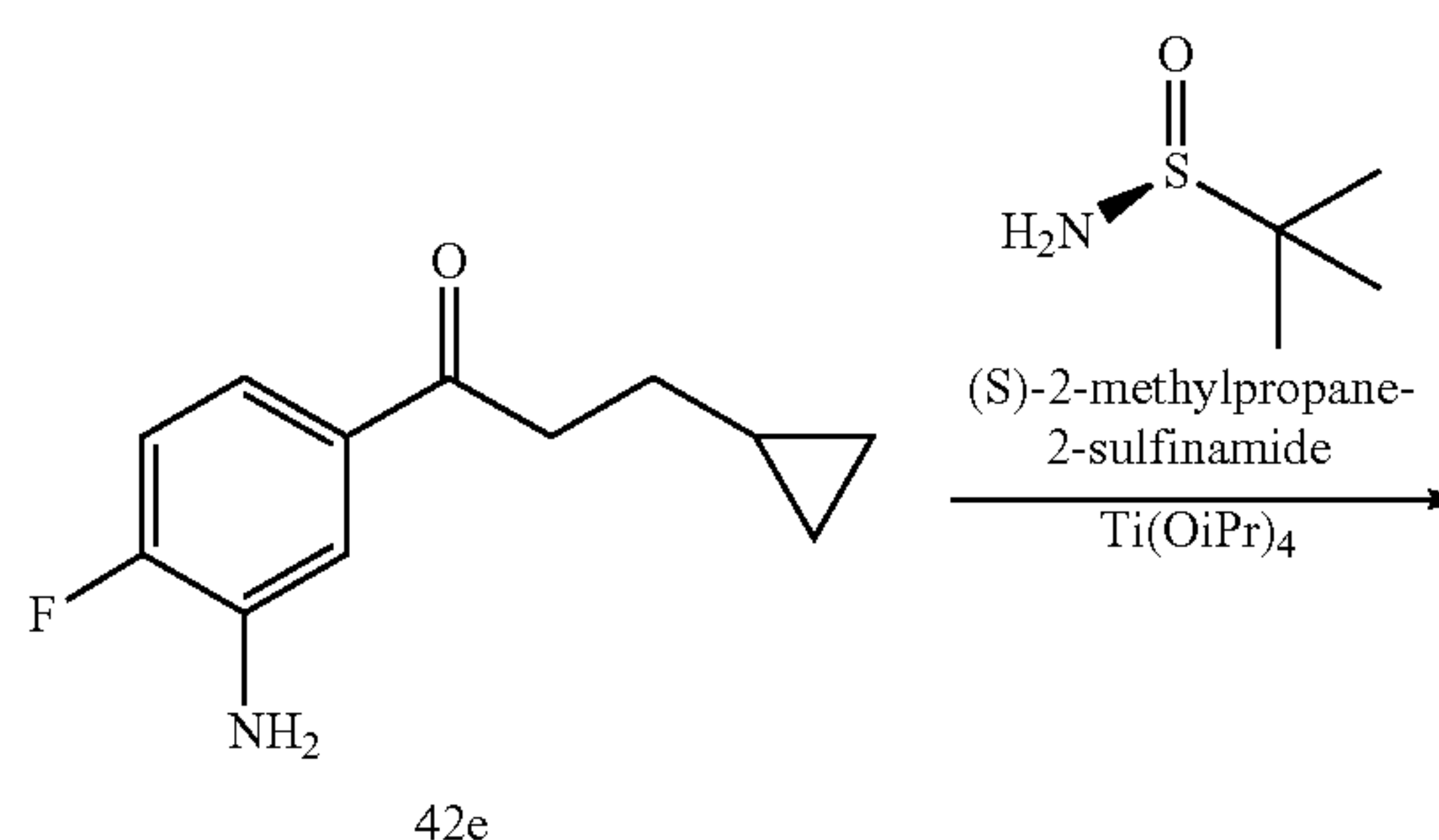
Scheme 43
