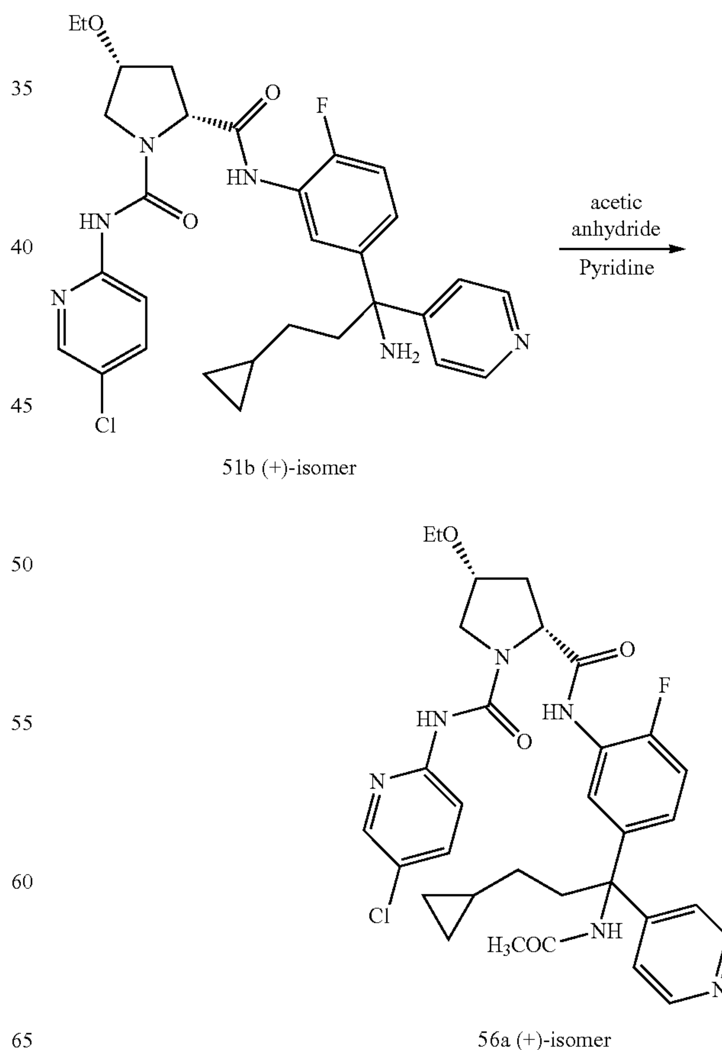
Scheme 56
