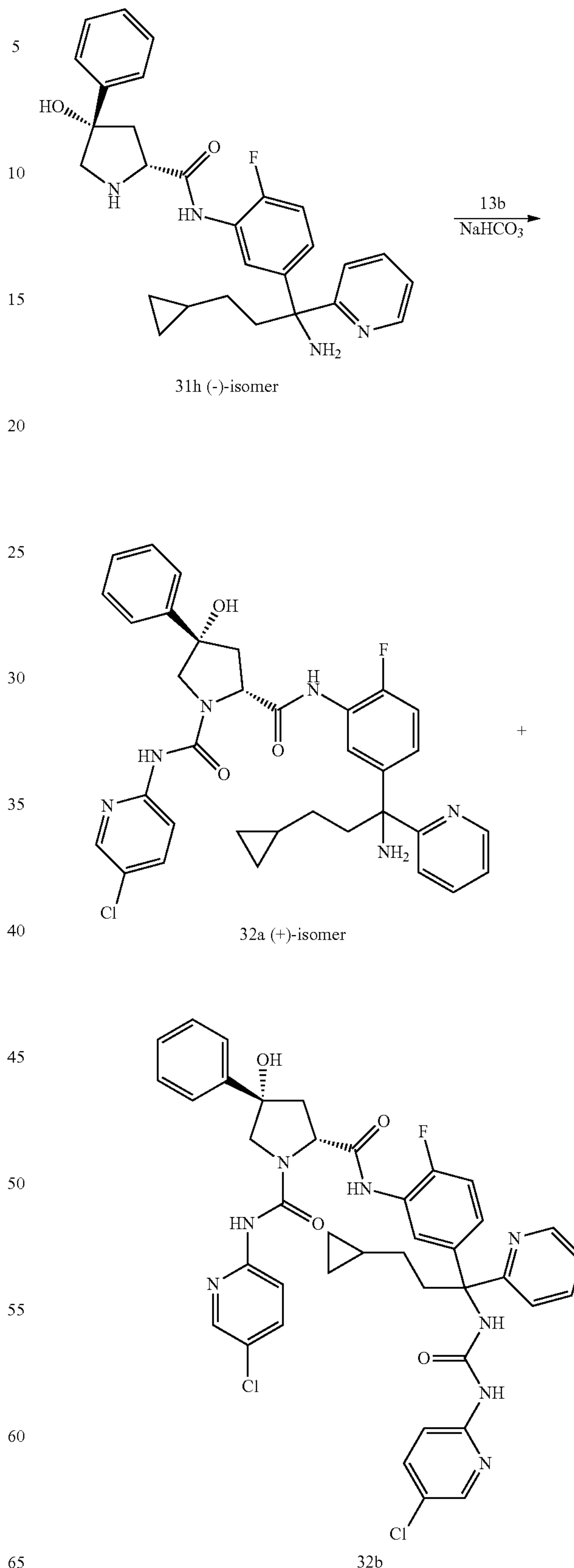
Scheme 32
