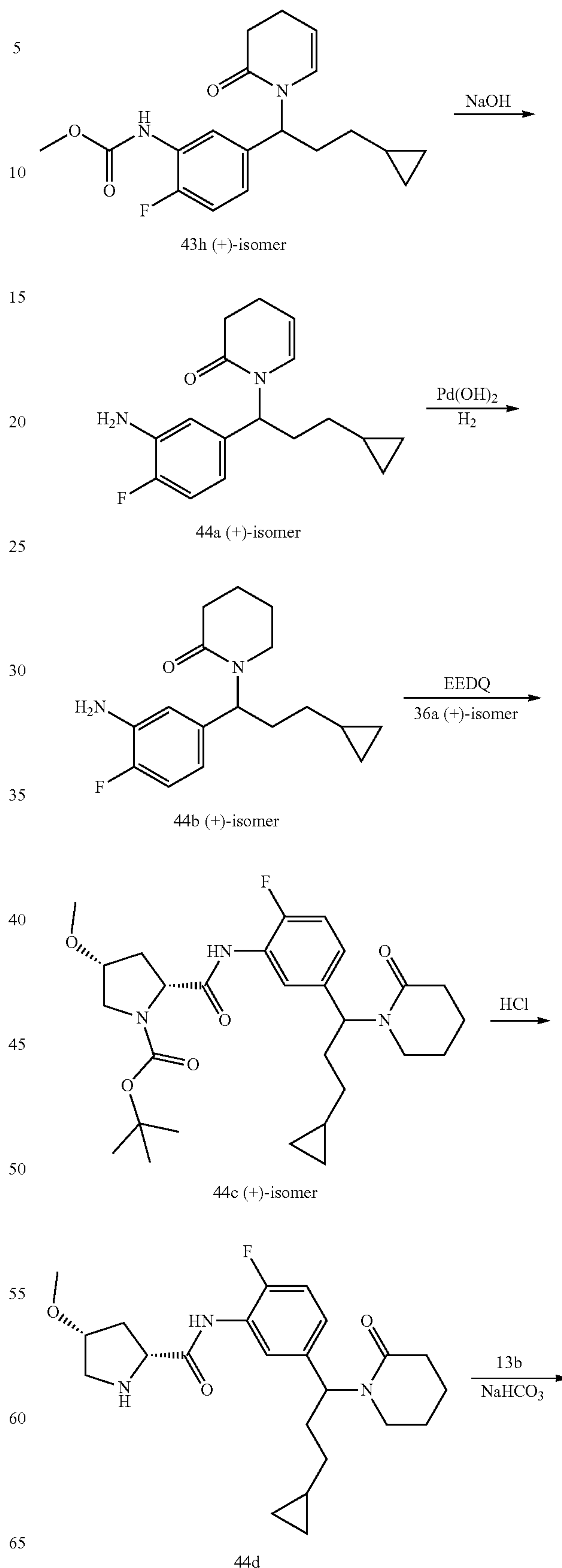
Scheme 44
