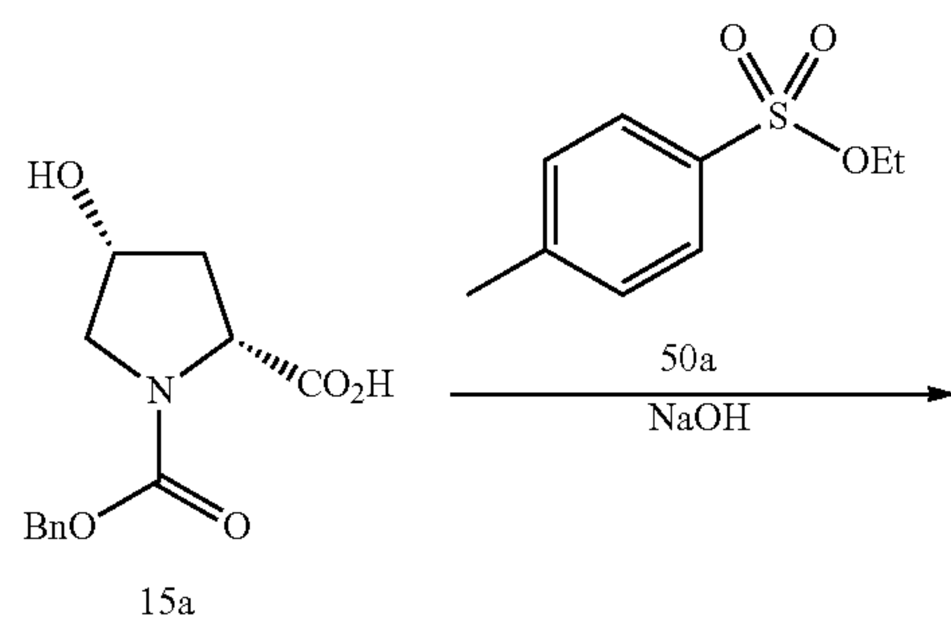
Scheme 50
