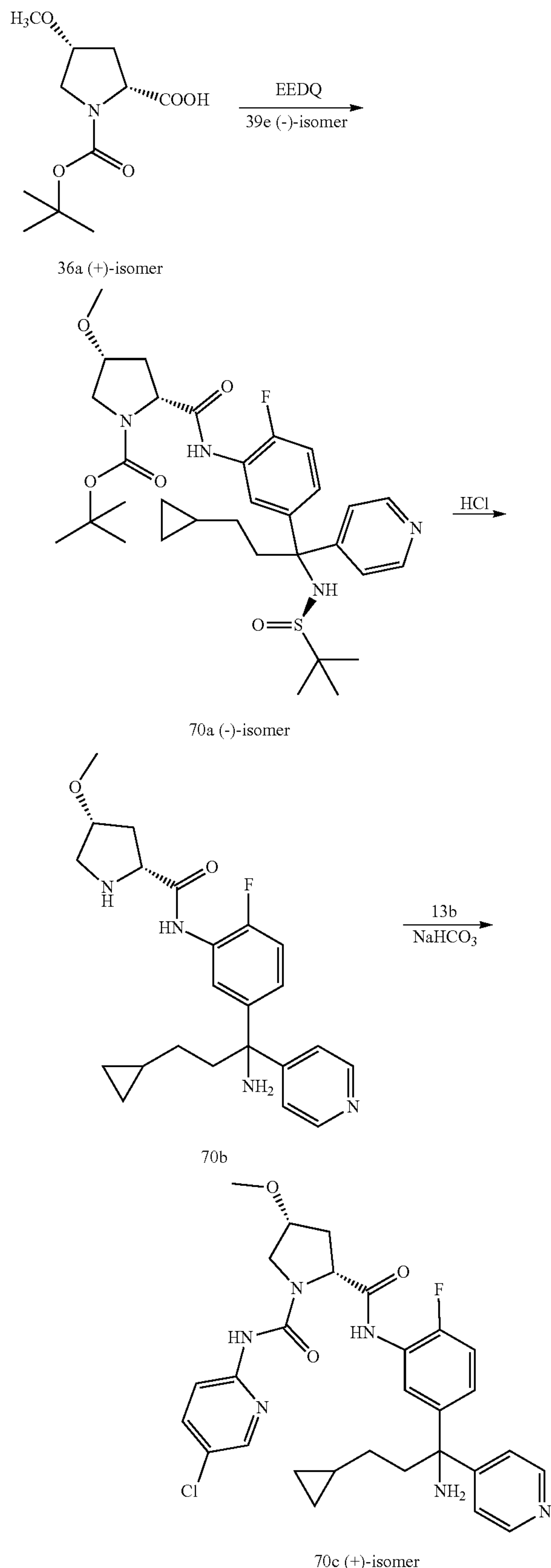
Scheme 70
