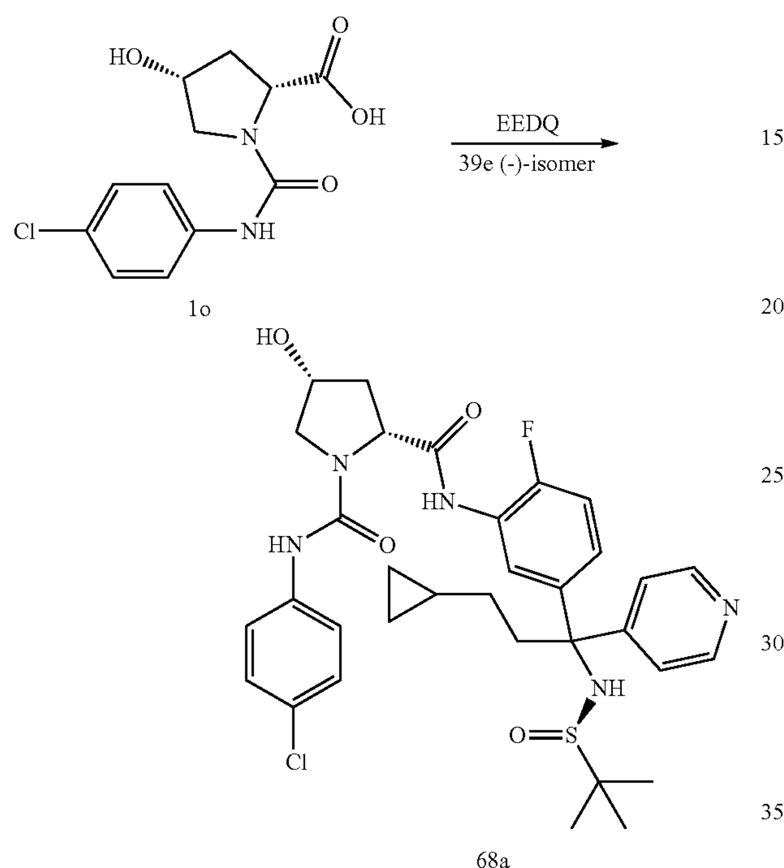
Scheme 68
