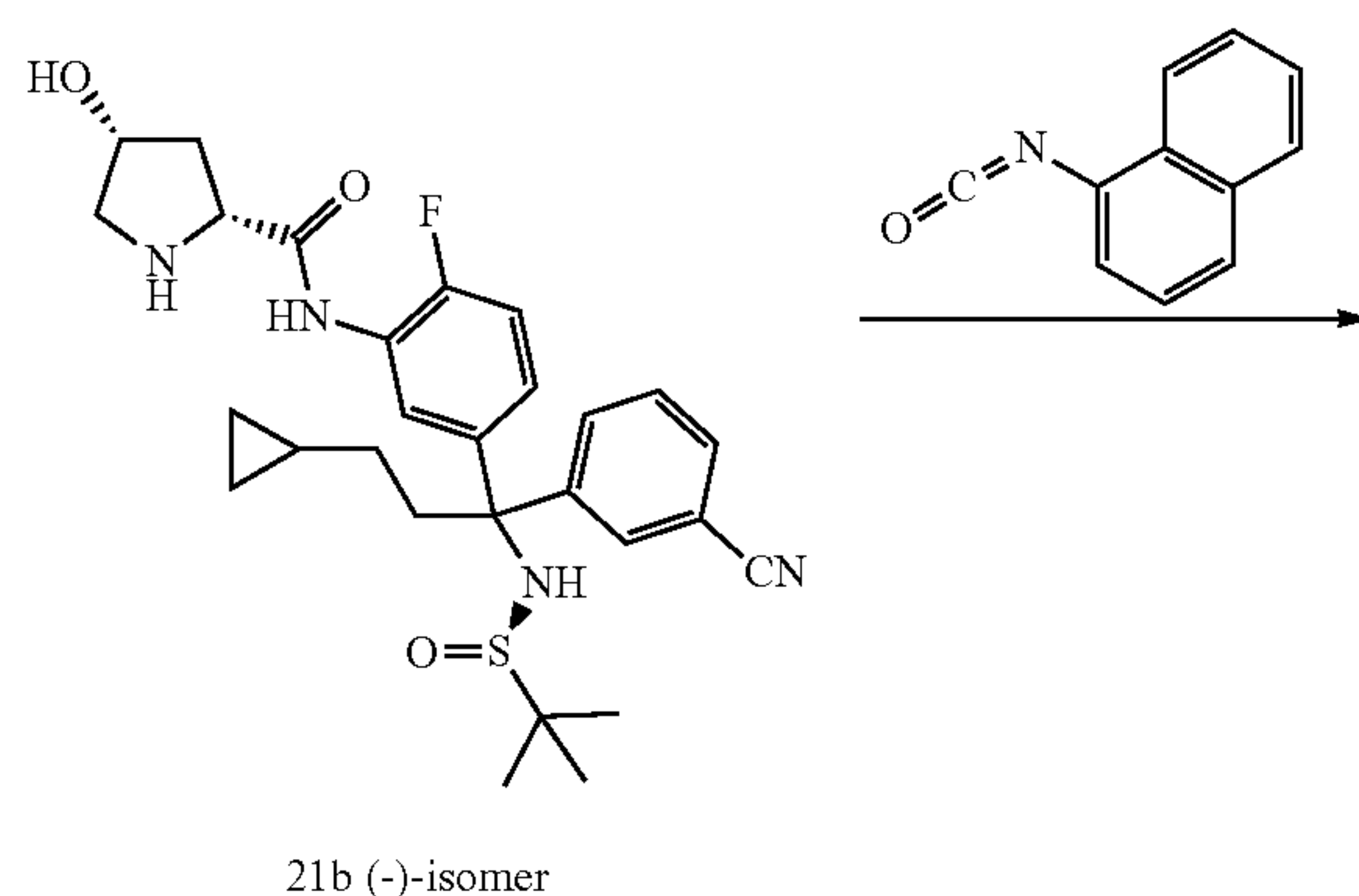
Scheme 26
