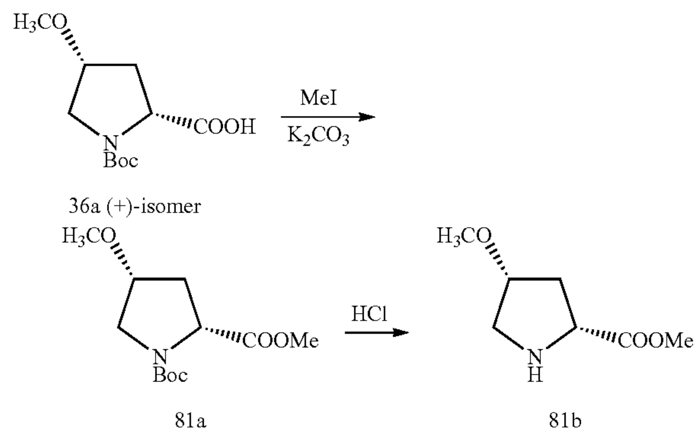
Scheme 81
