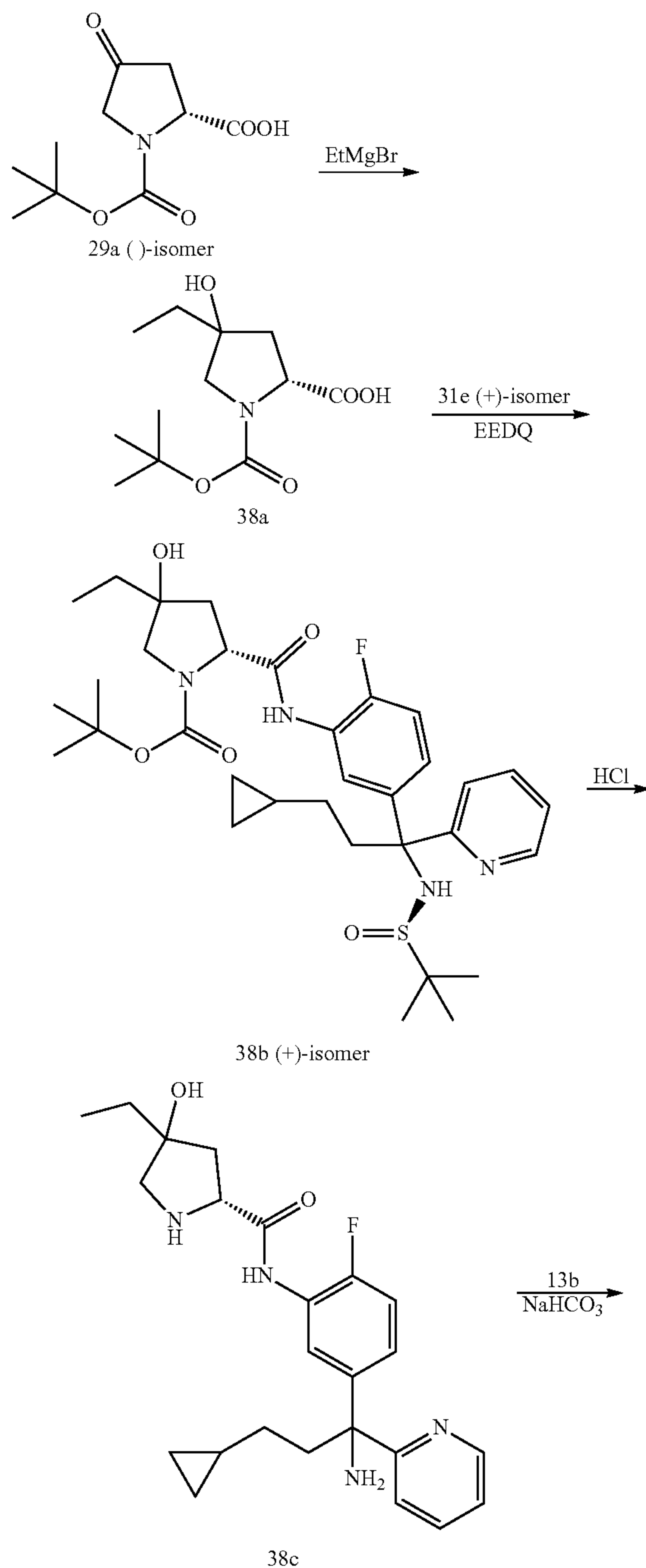
Scheme 38
