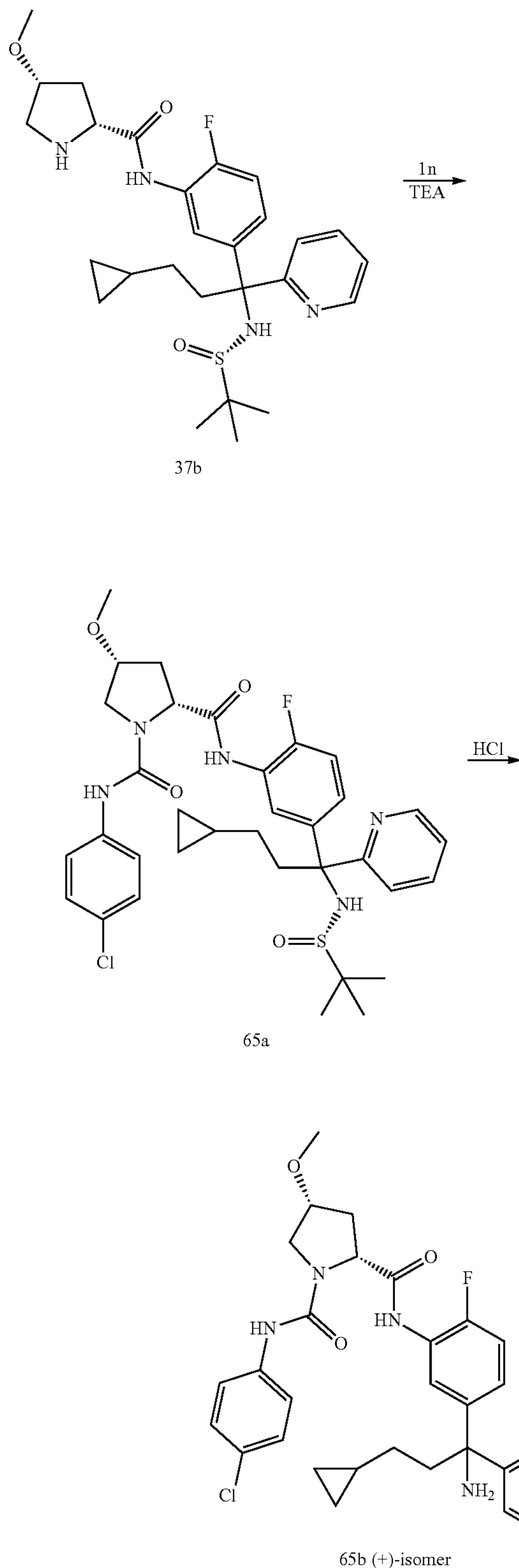
Scheme 65
