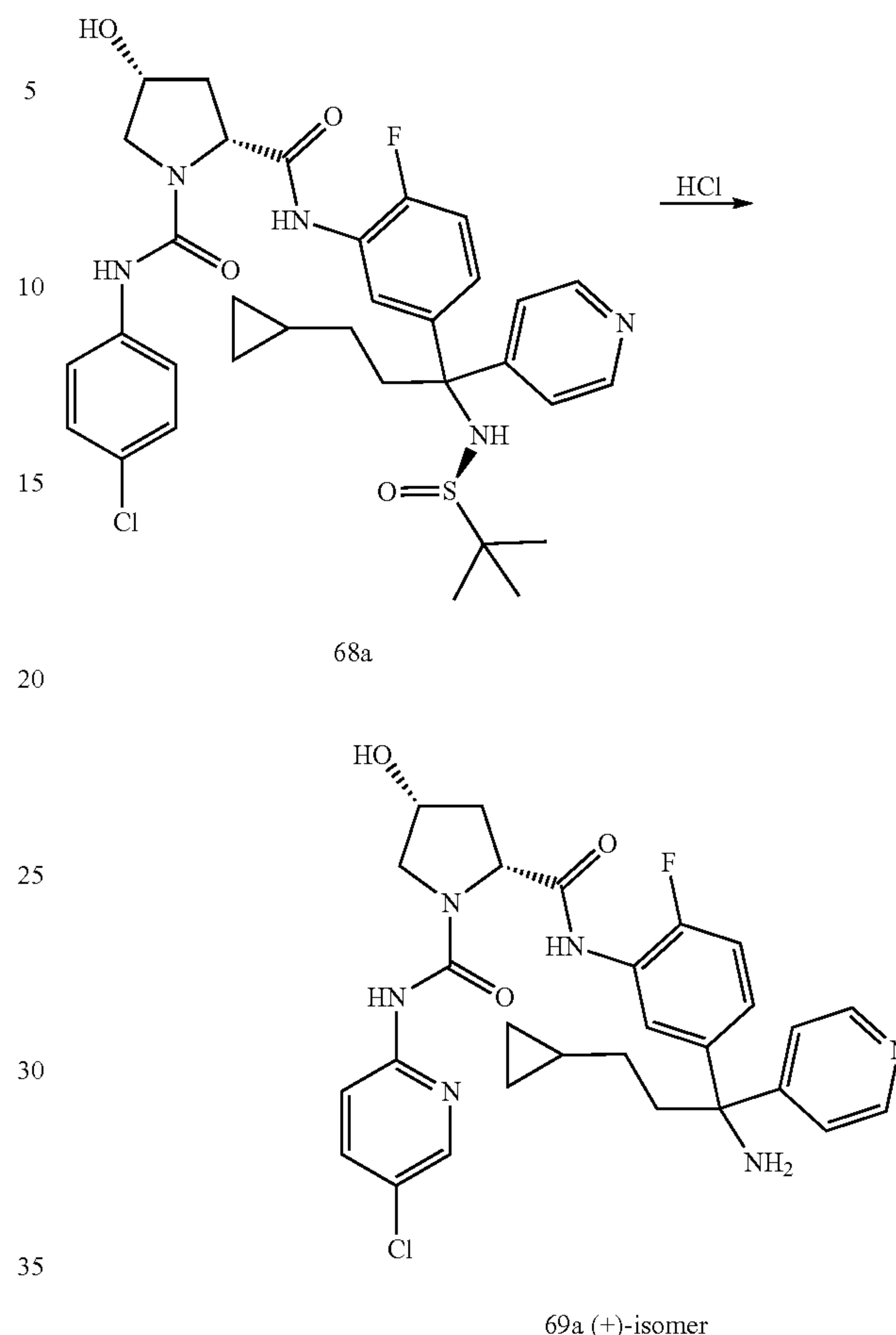
Scheme 69
