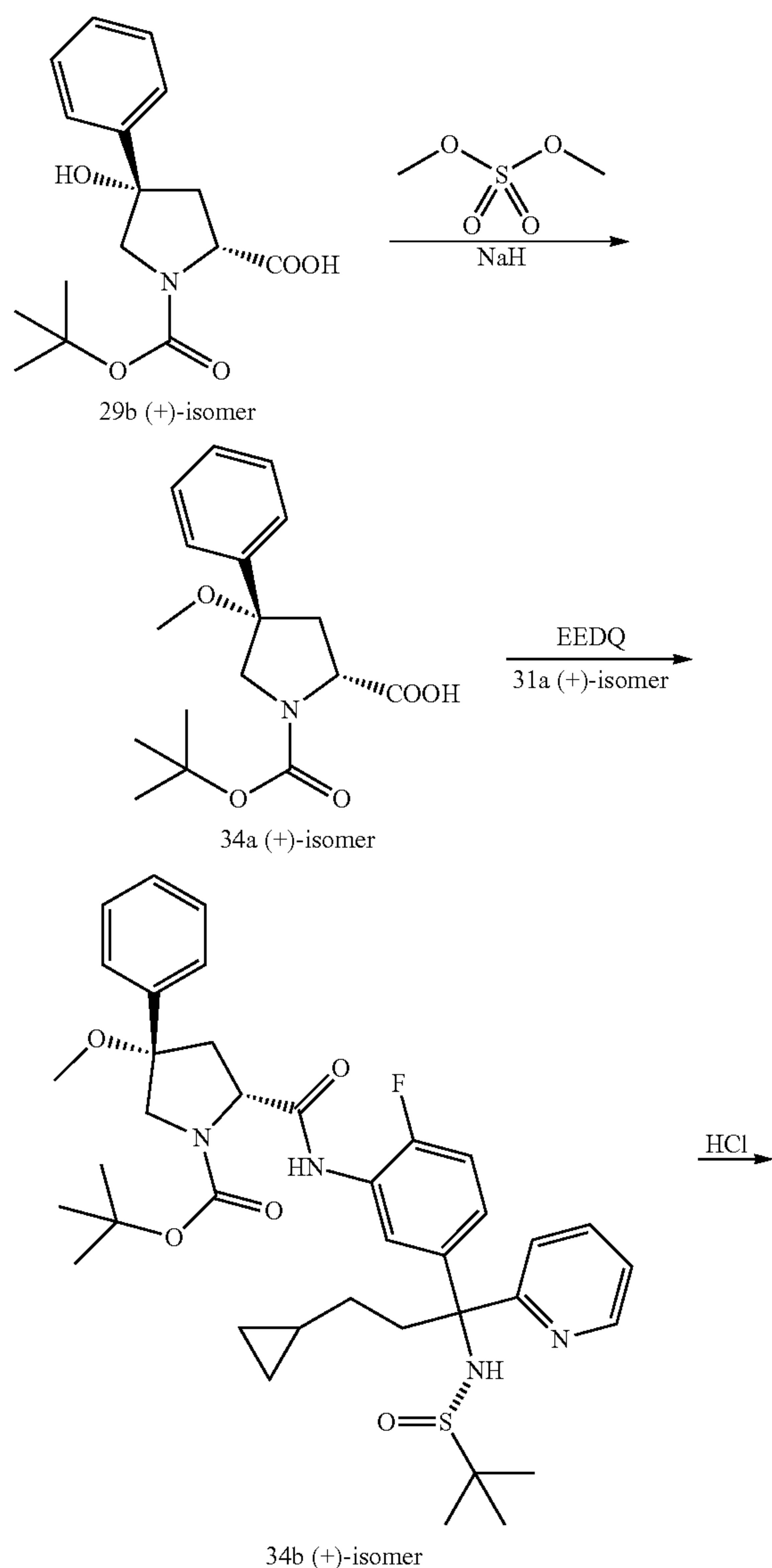
Scheme 34
