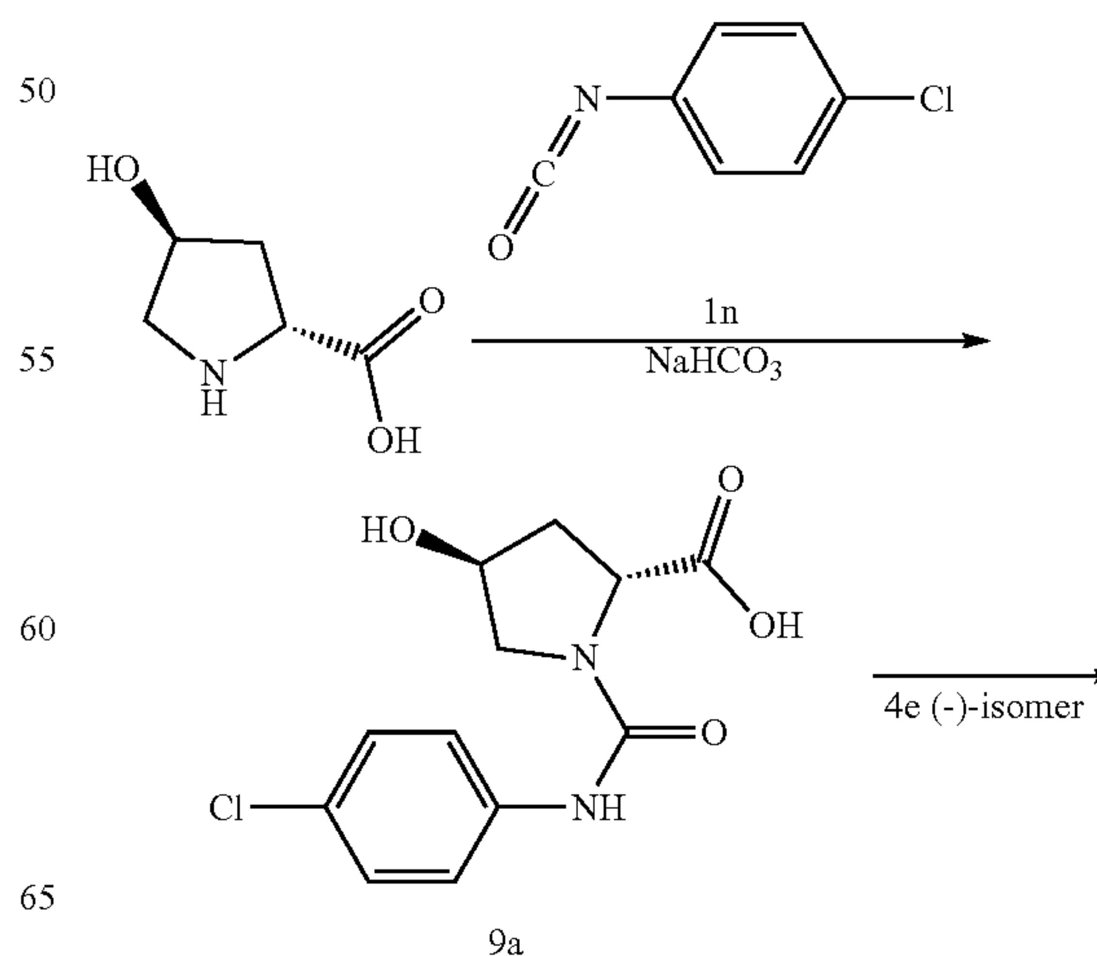
Scheme 9
