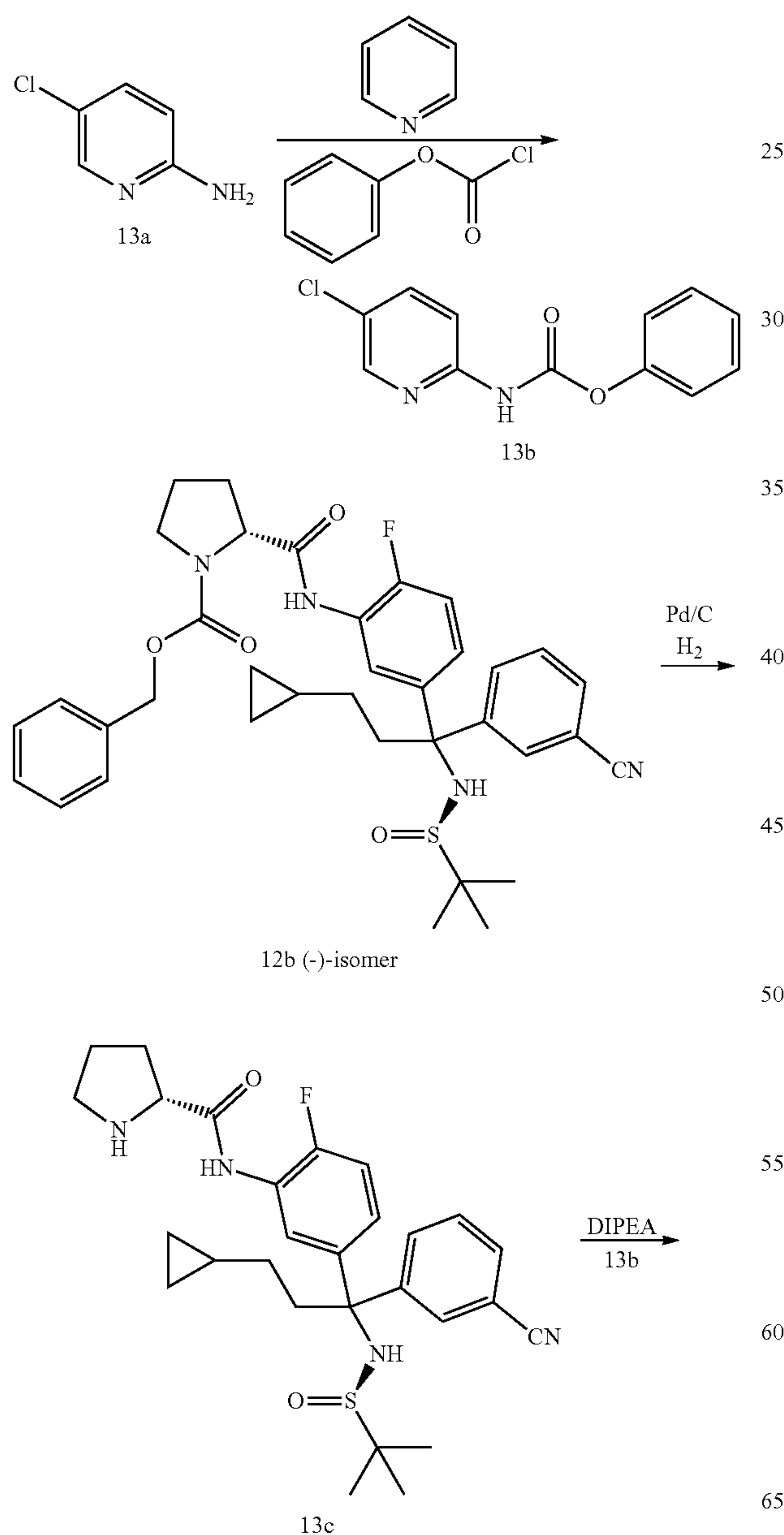
Scheme 13
