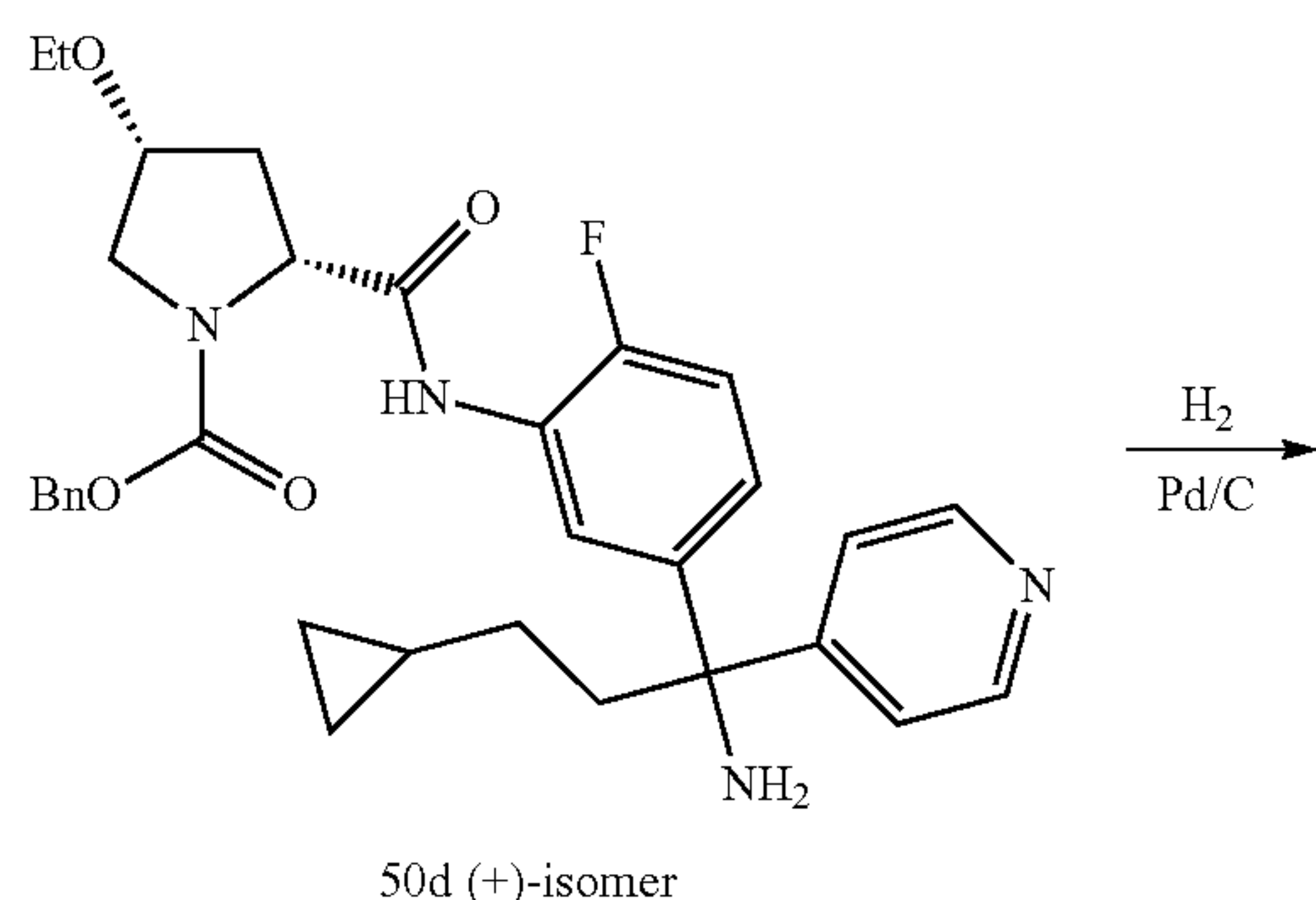
Scheme 51
