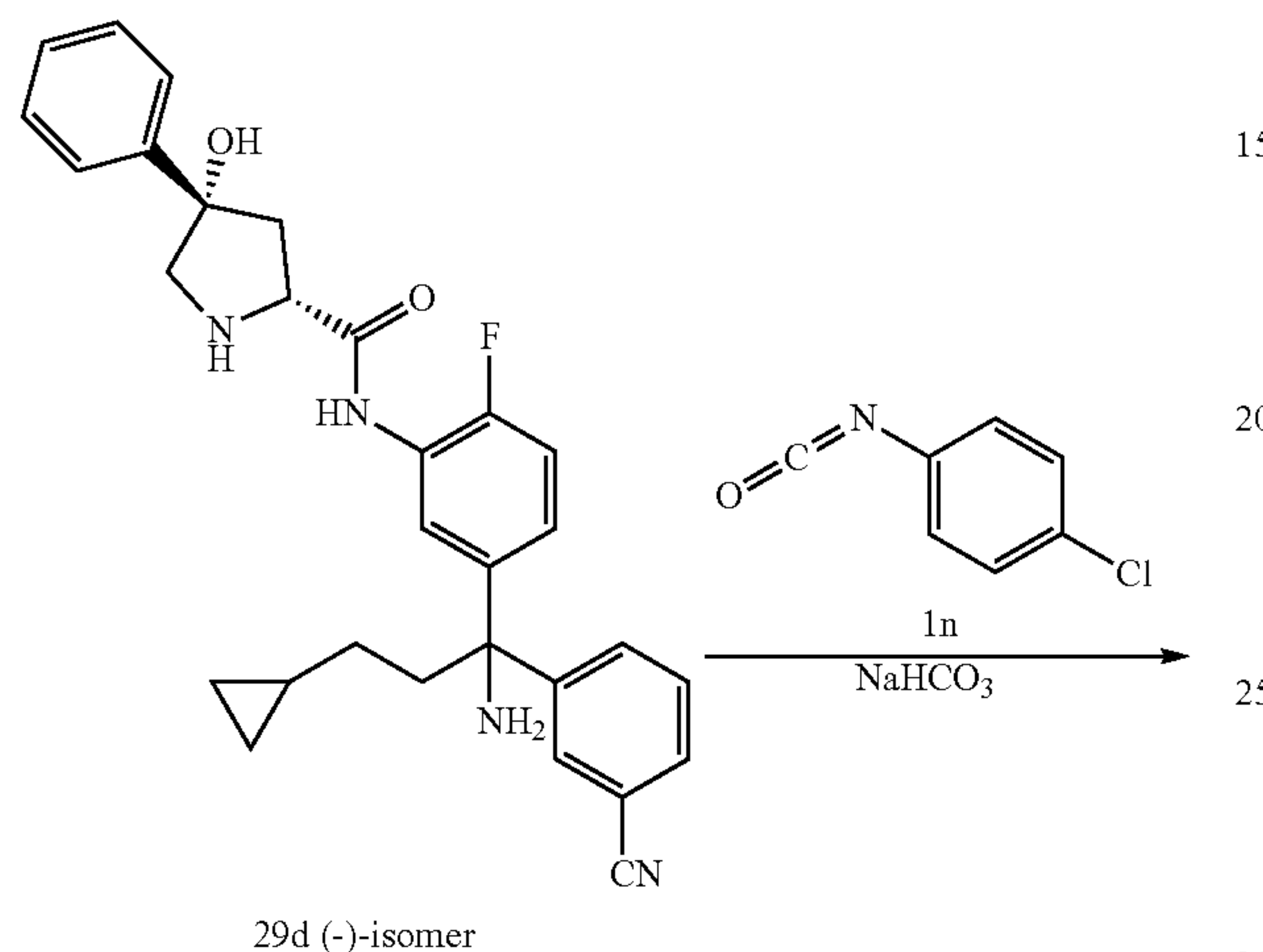
Scheme 30
