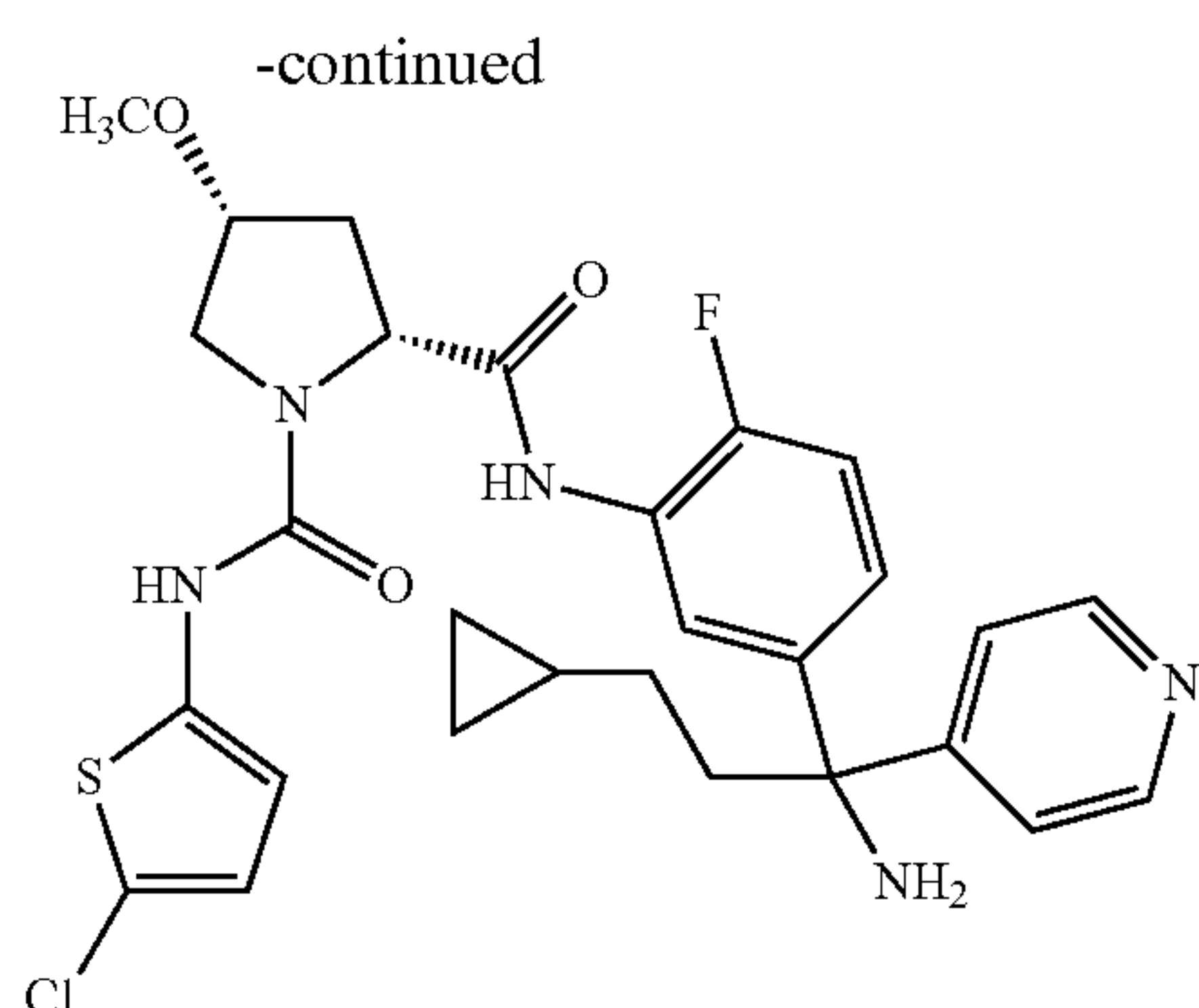
81h (-)-isomer
