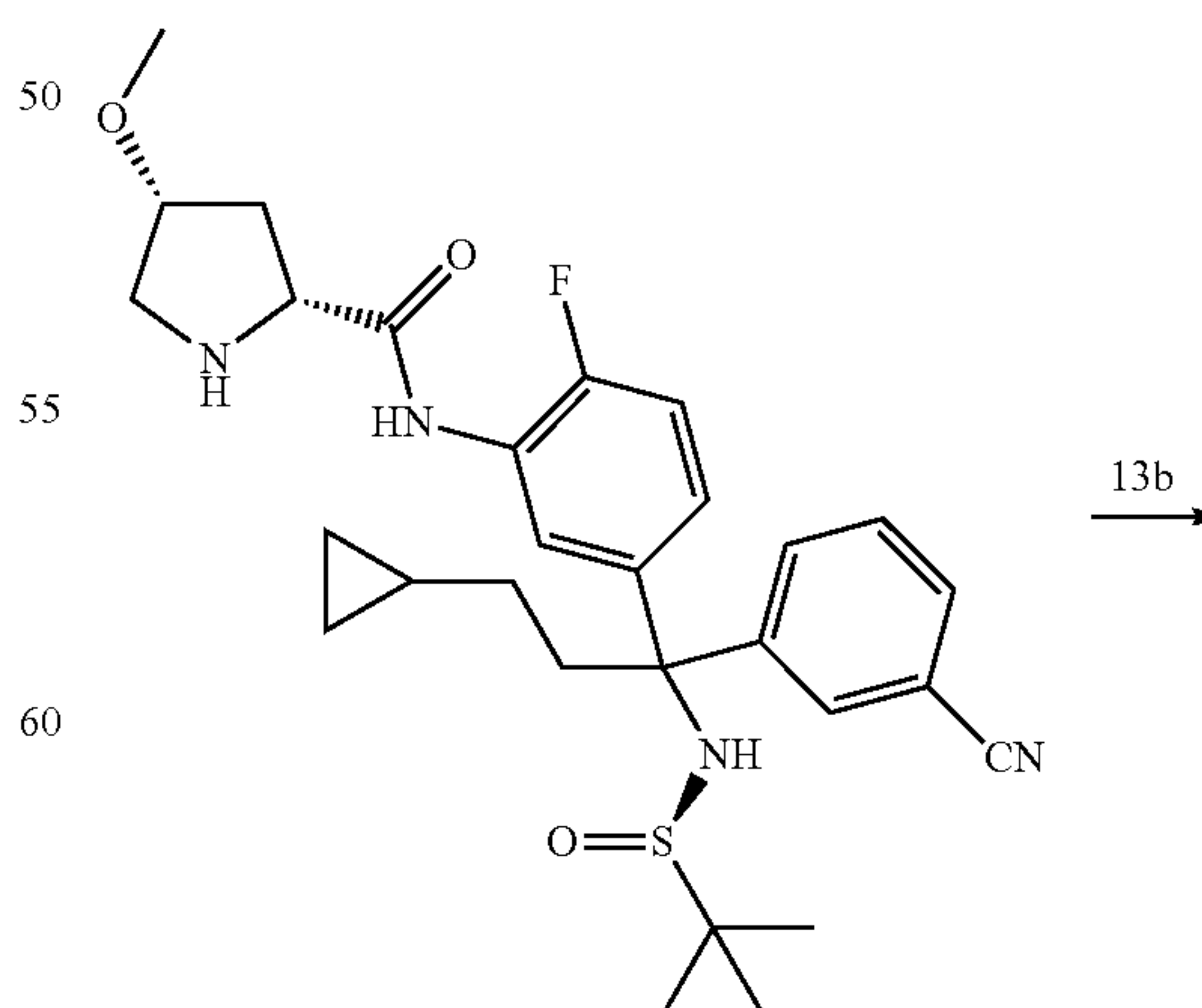
15d (-)-isomer
