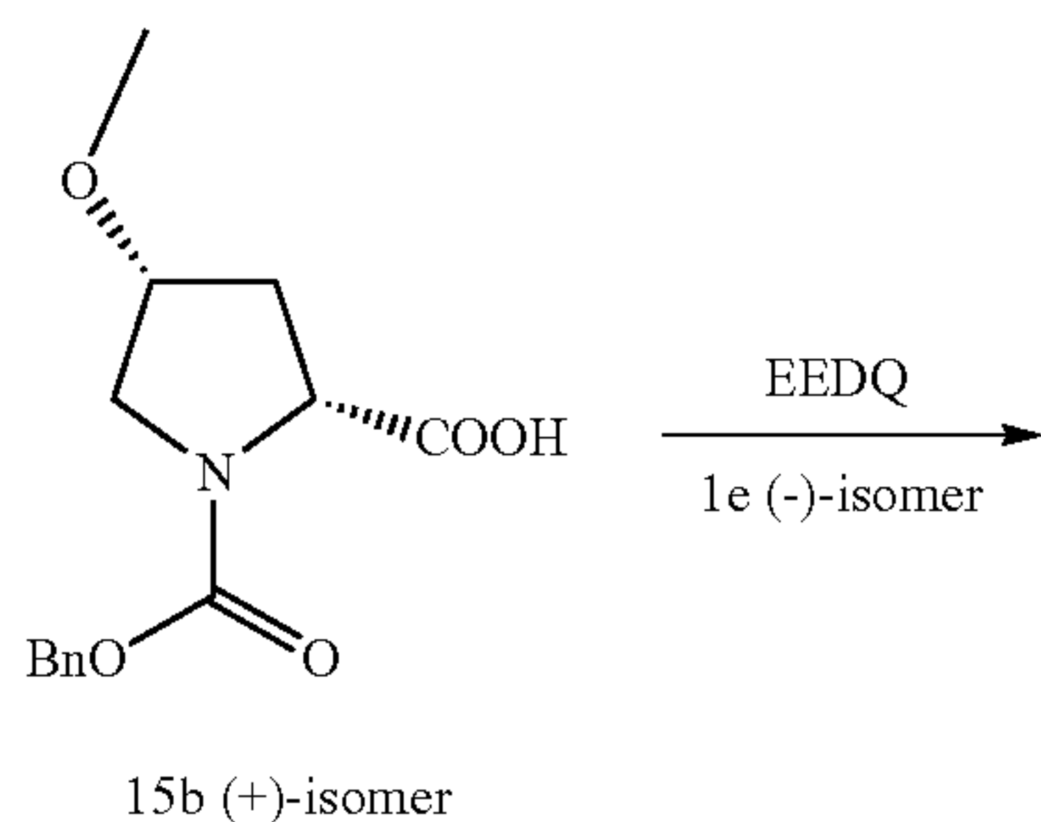
Scheme 66
