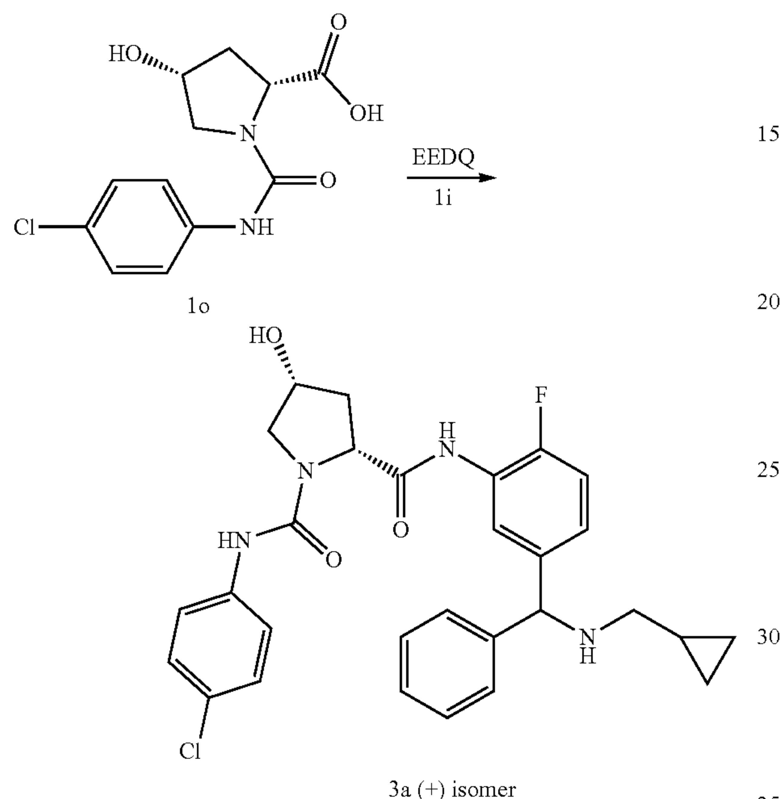
Scheme 3
