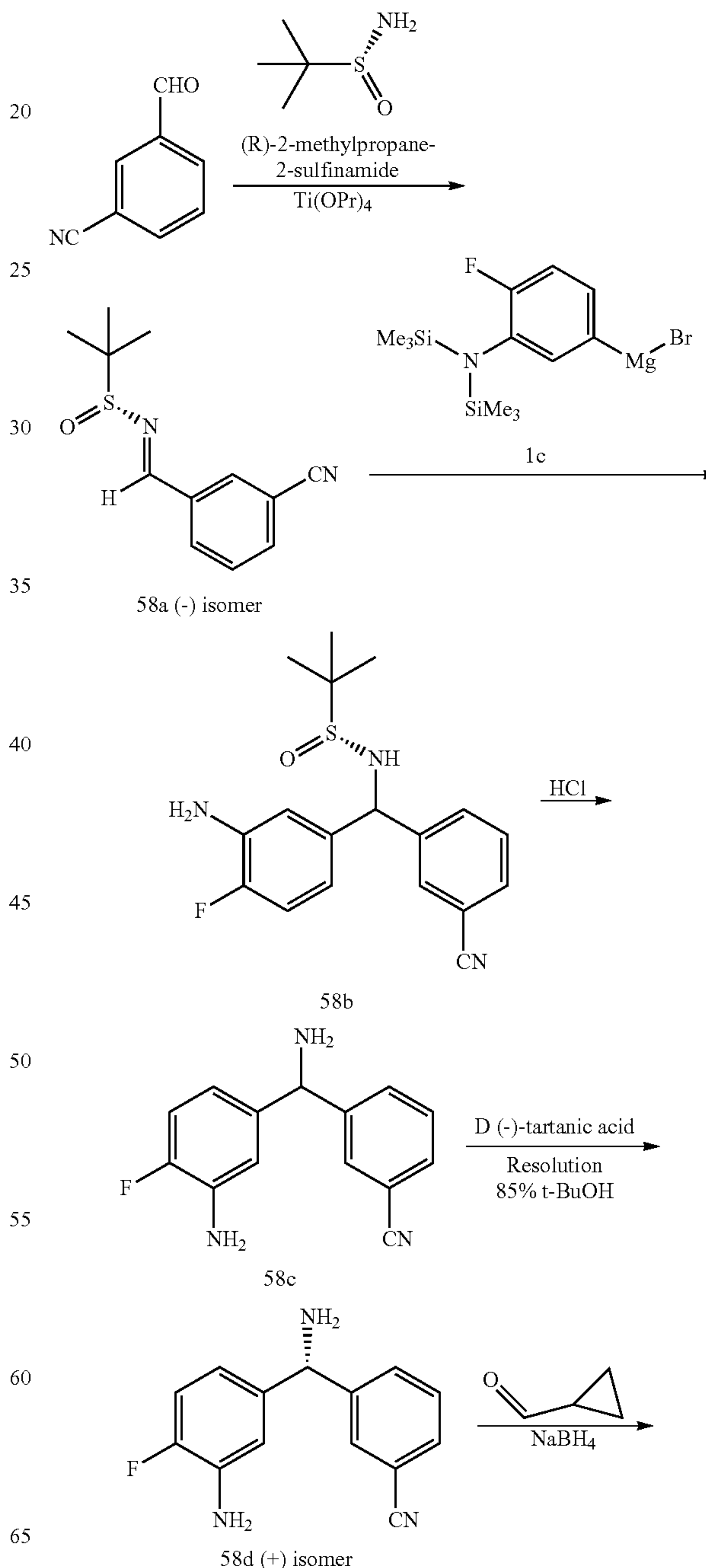
Scheme 58
