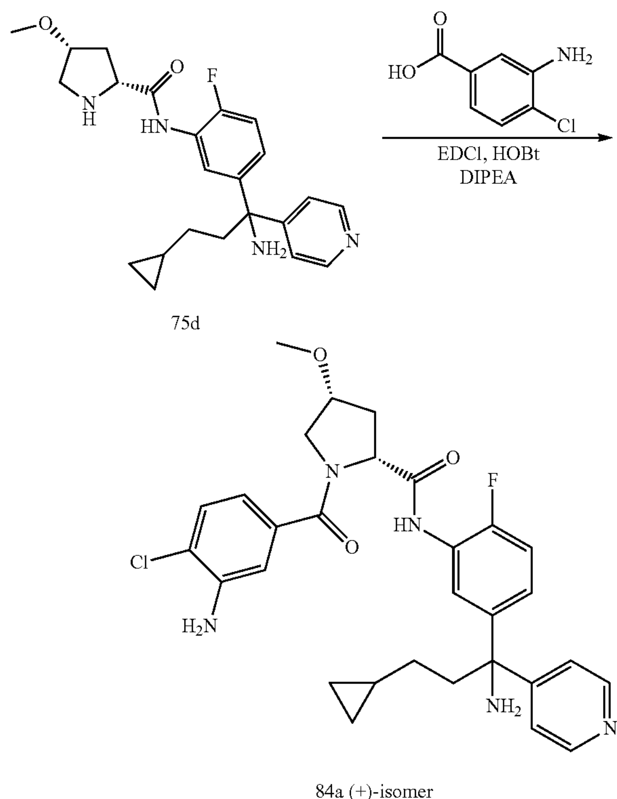
Scheme 84
