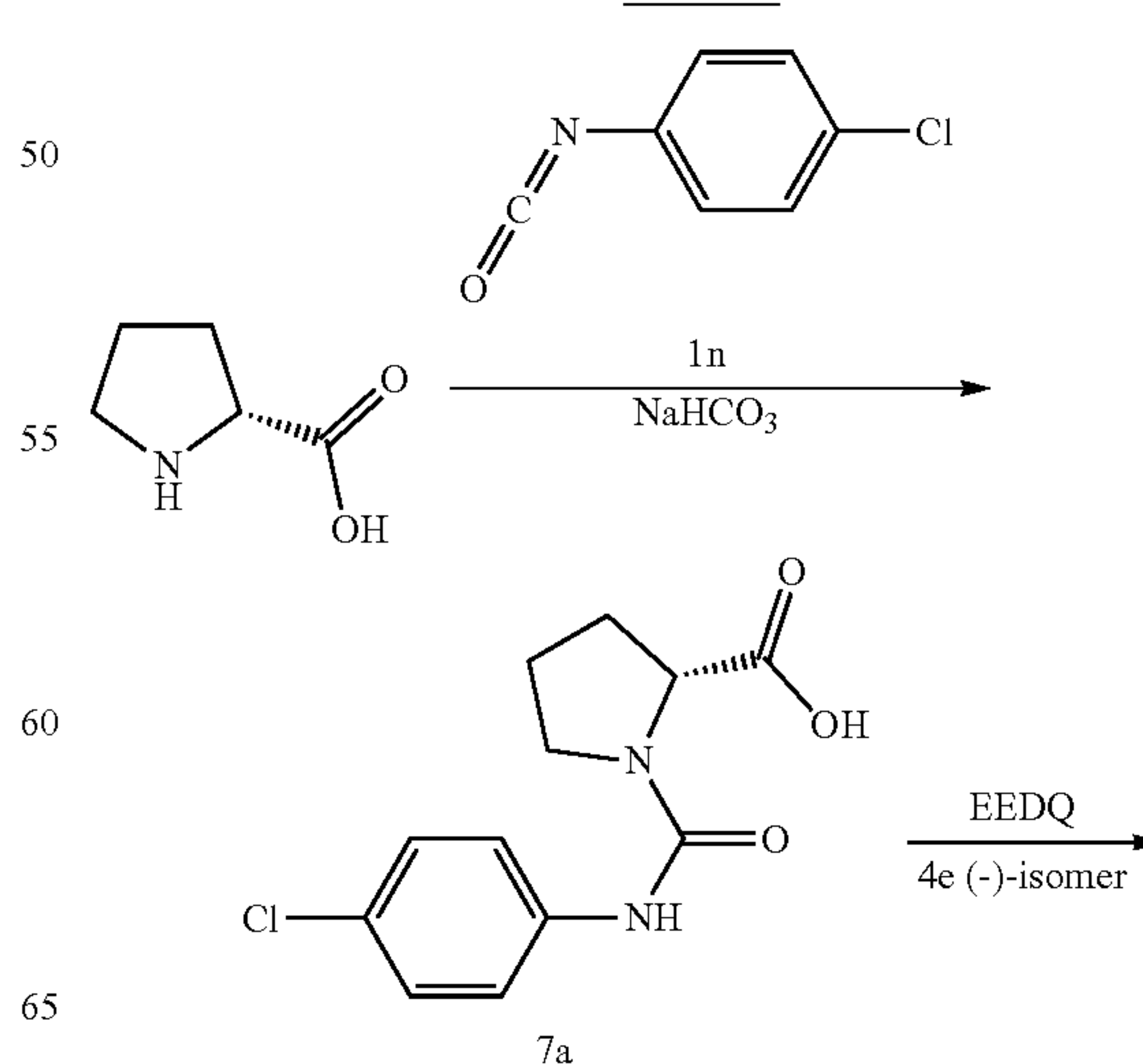
Scheme 7
