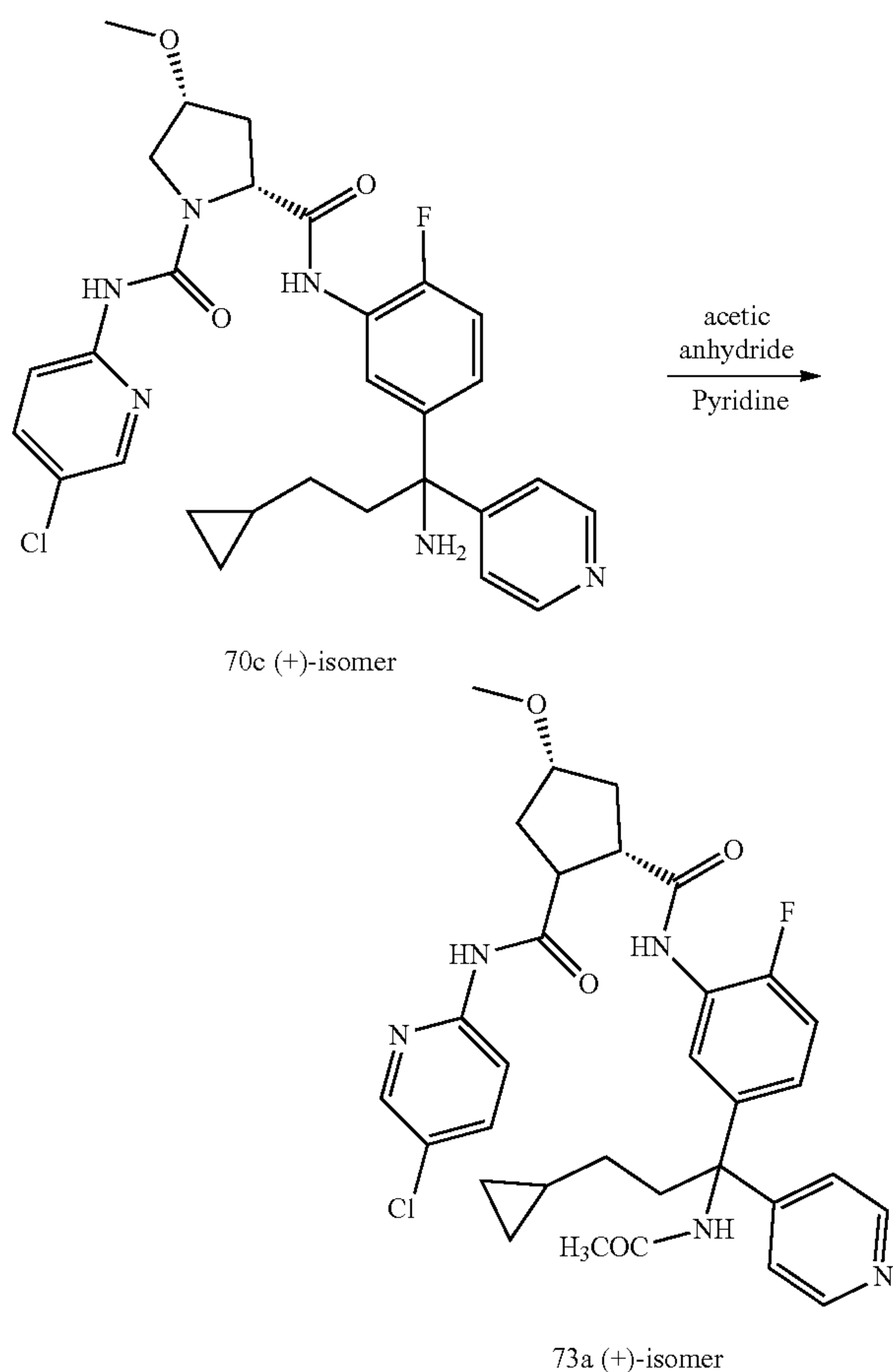
Scheme 73
