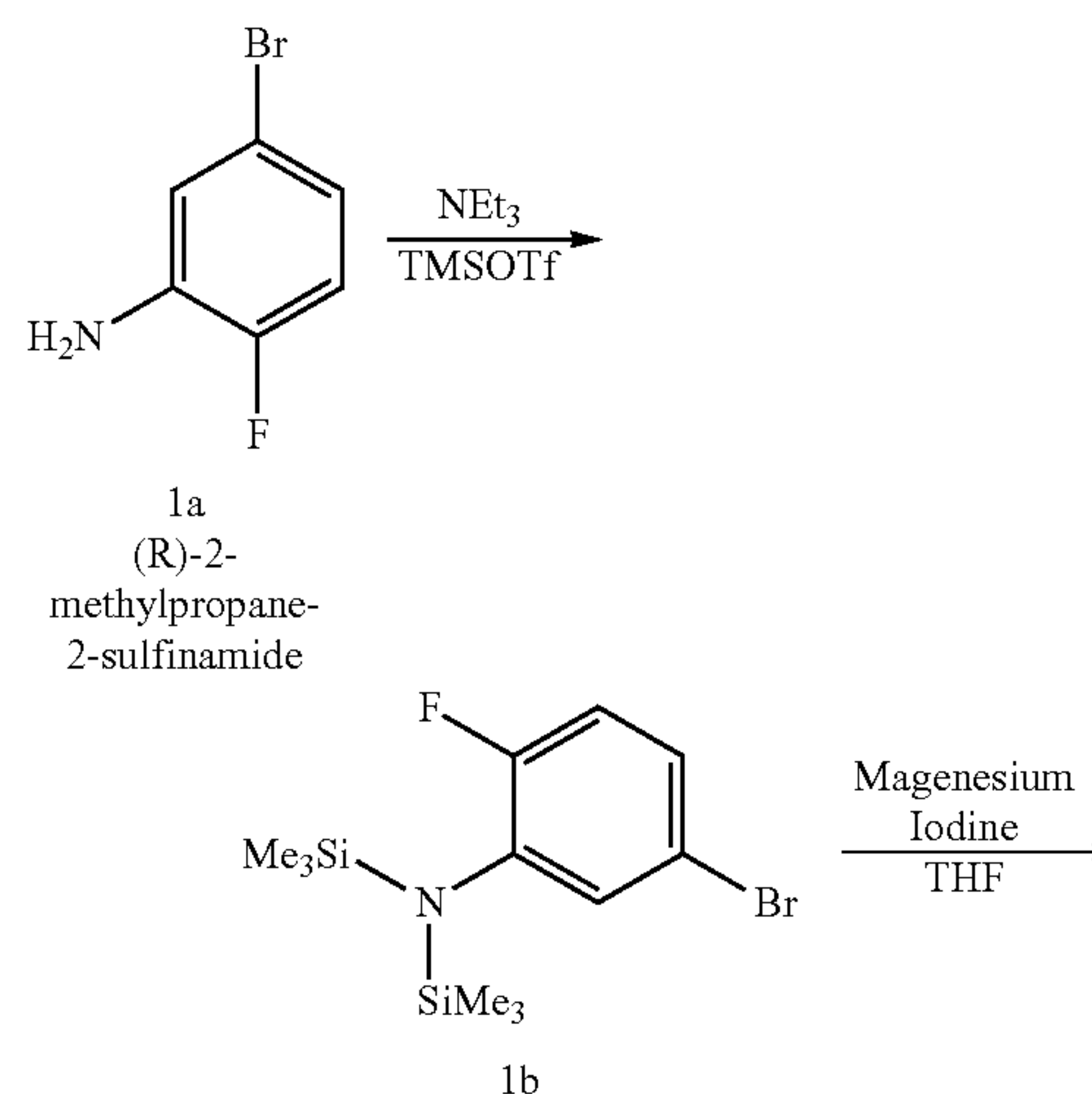
Scheme 1
