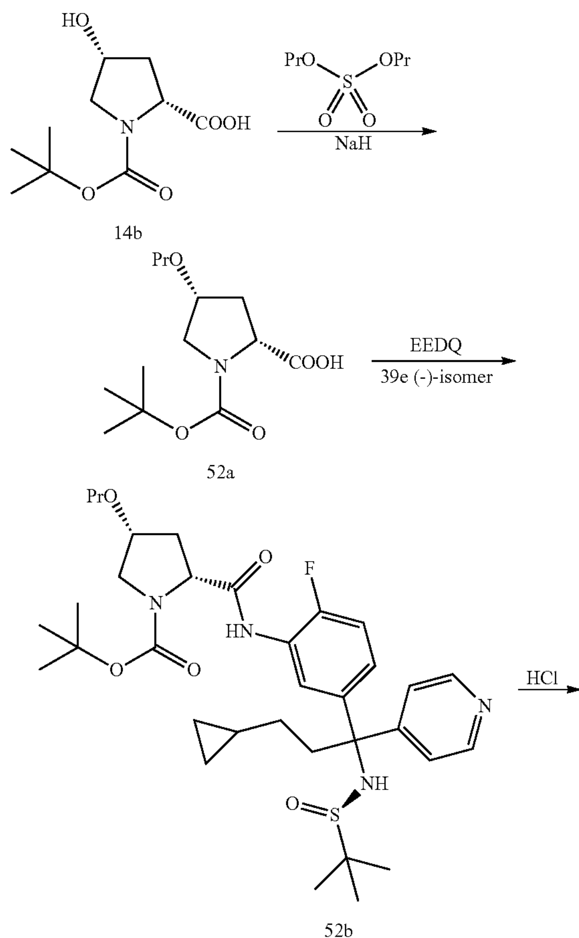
Scheme 52
