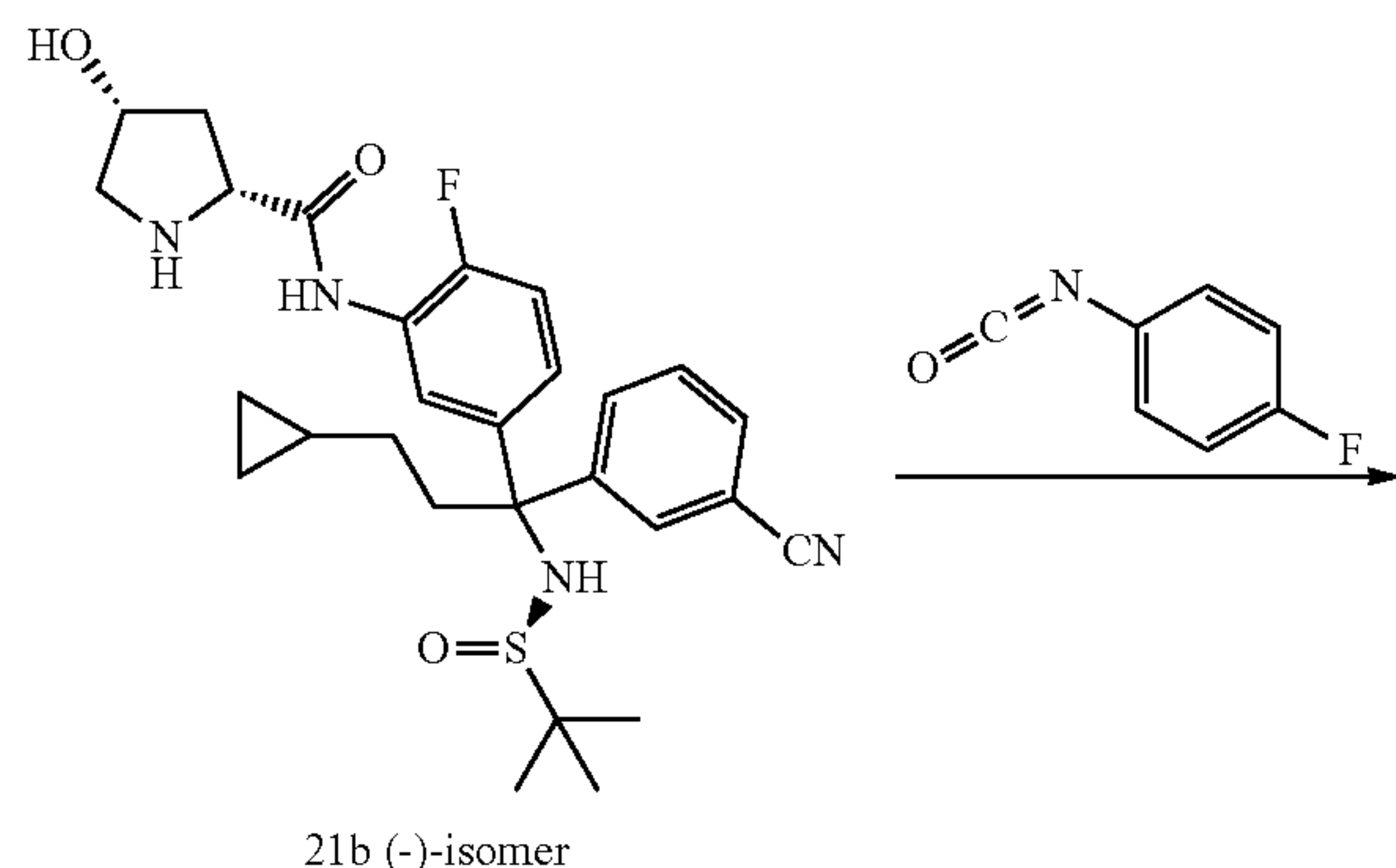
Scheme 24
