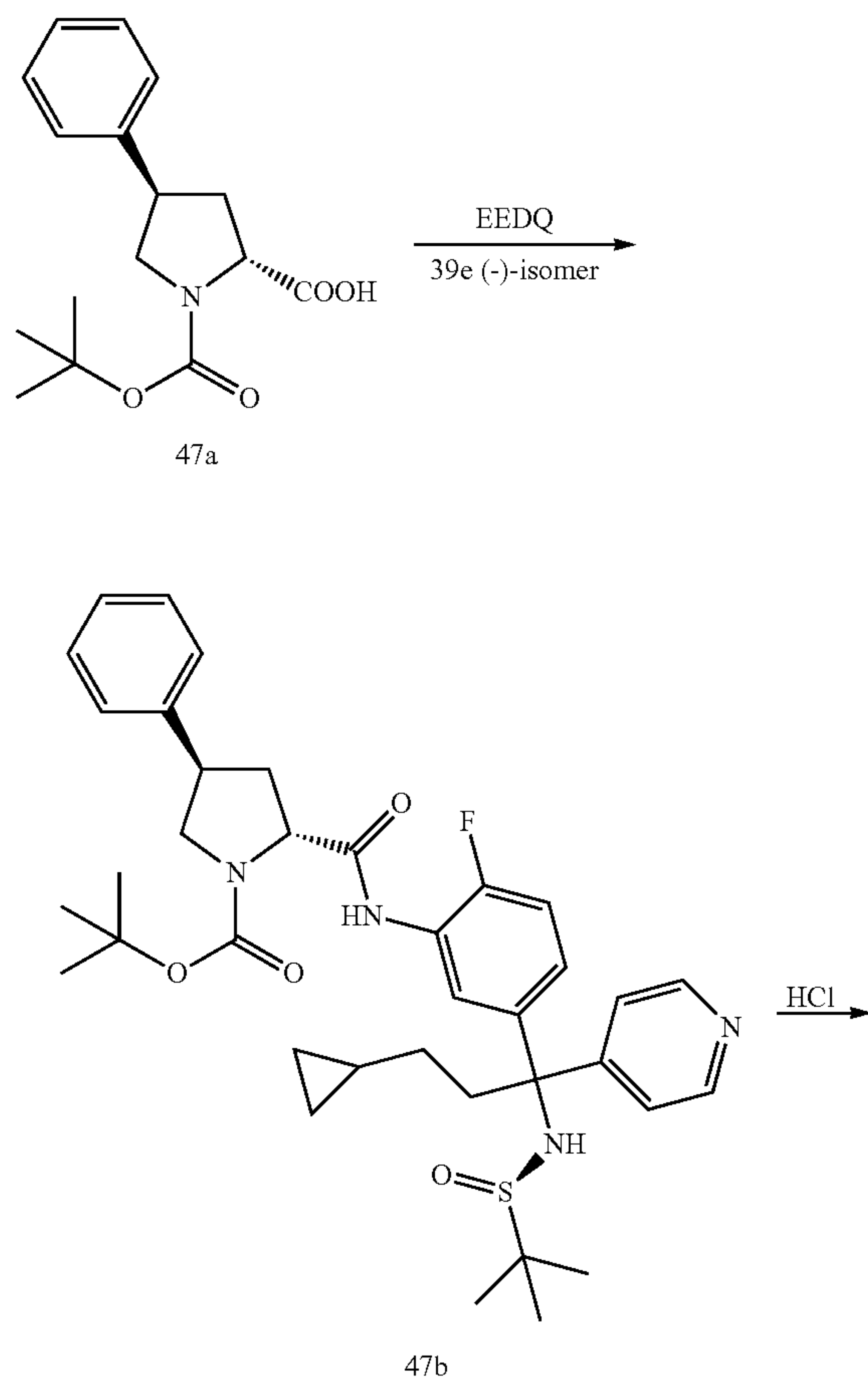
Scheme 47
