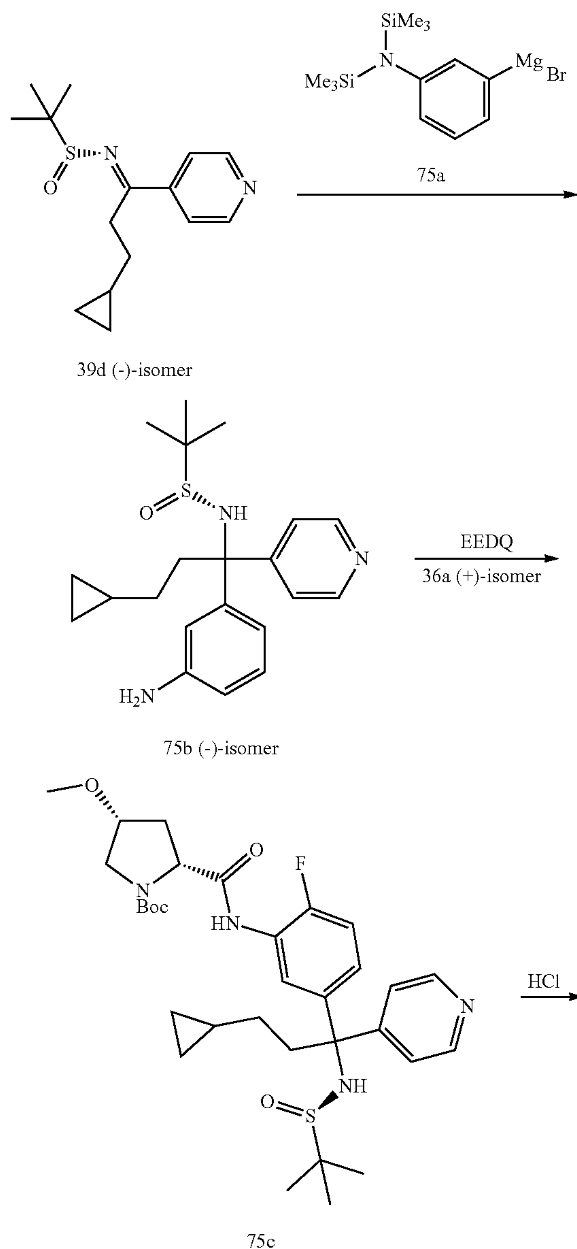
Scheme 75
