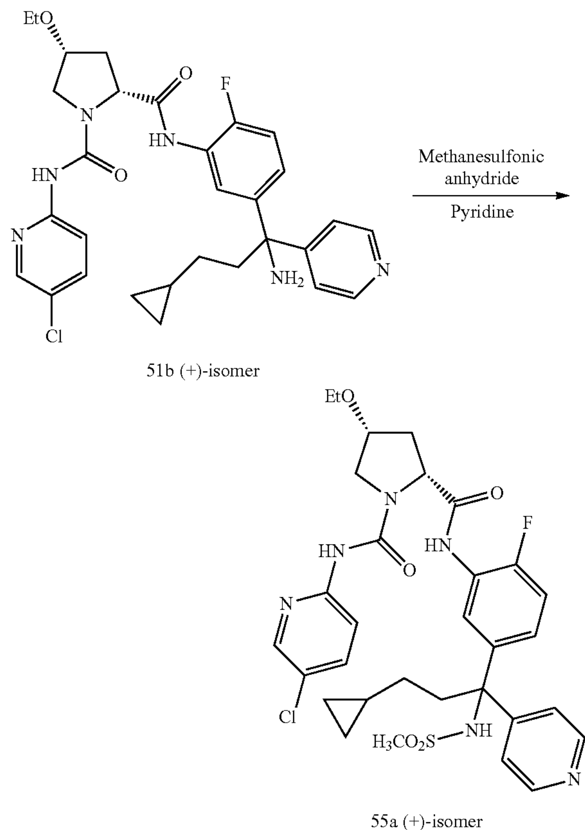
Scheme 55
