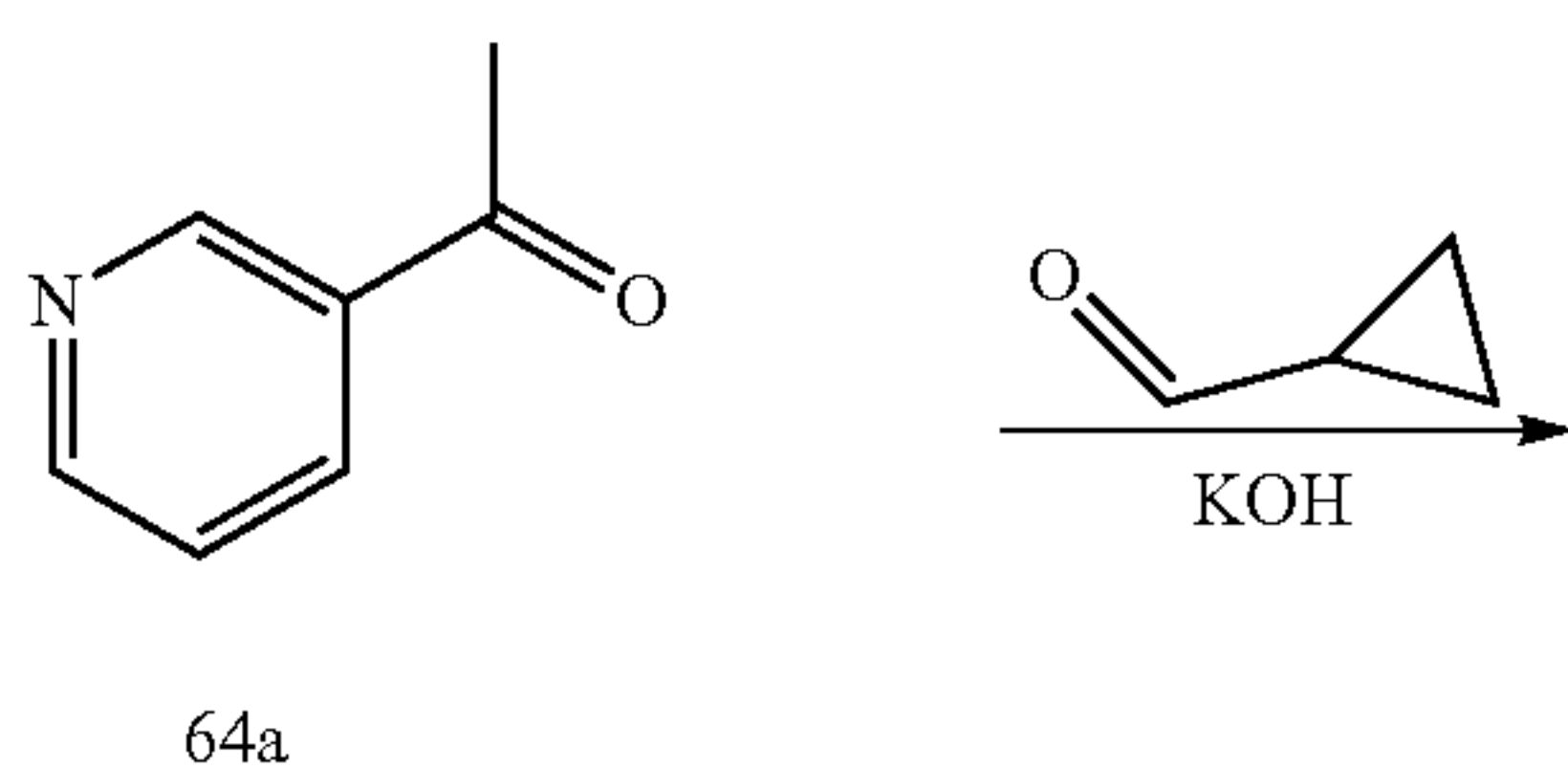
Scheme 64
