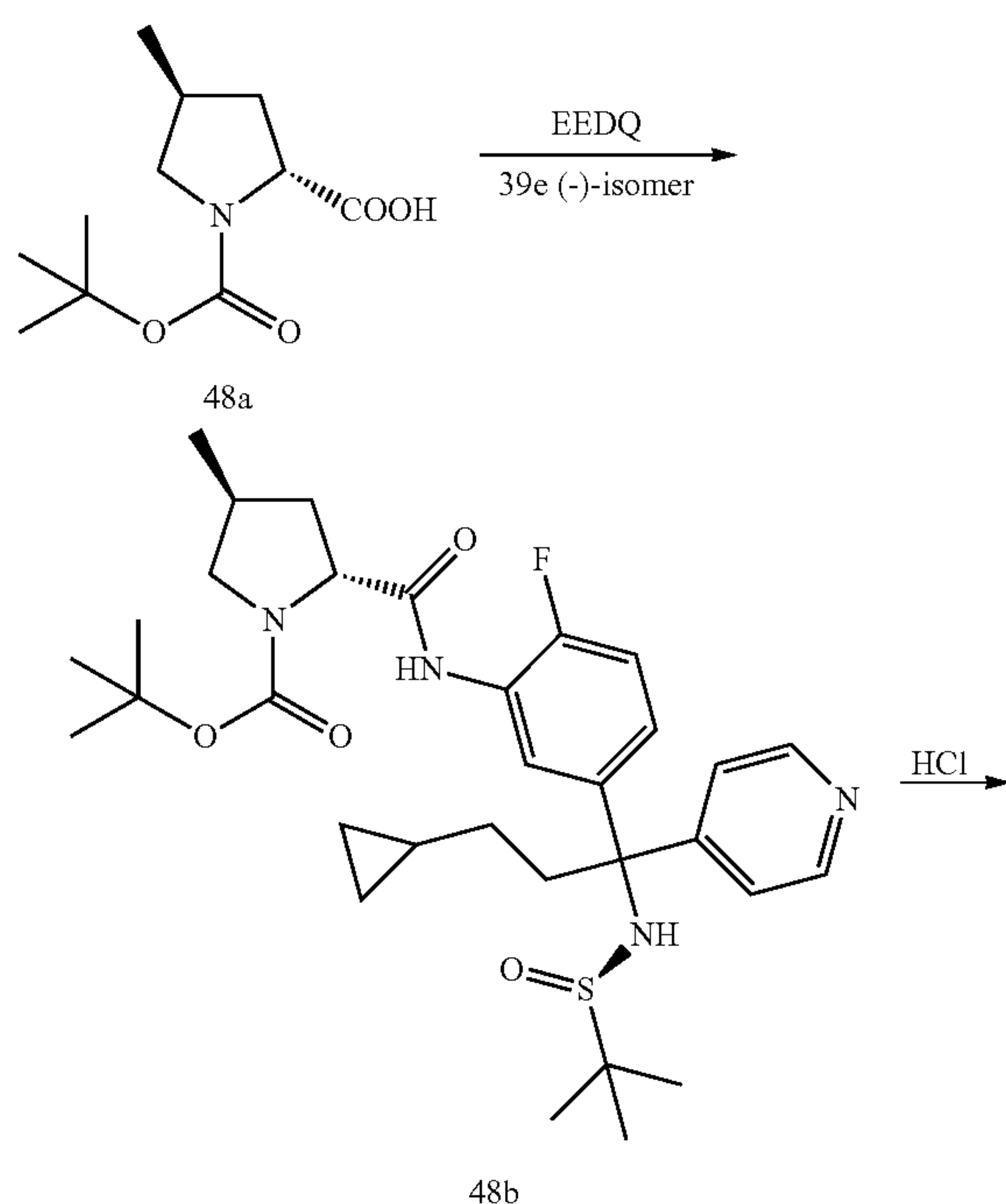
Scheme 48
