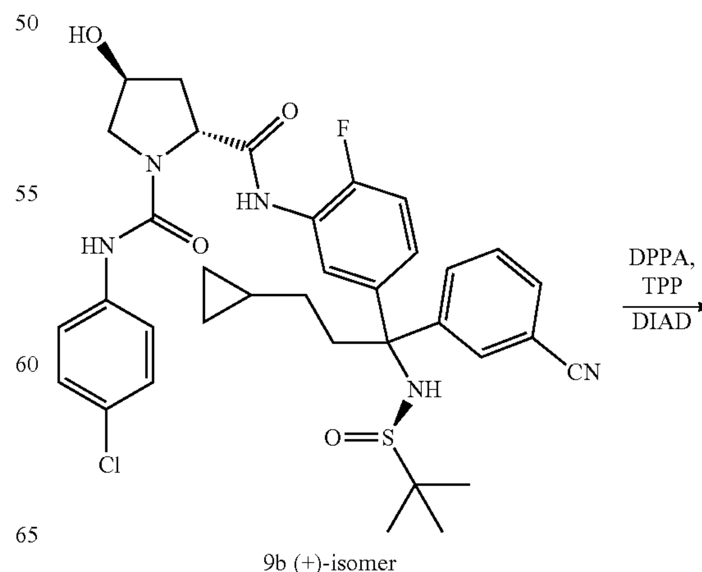
Scheme 19
