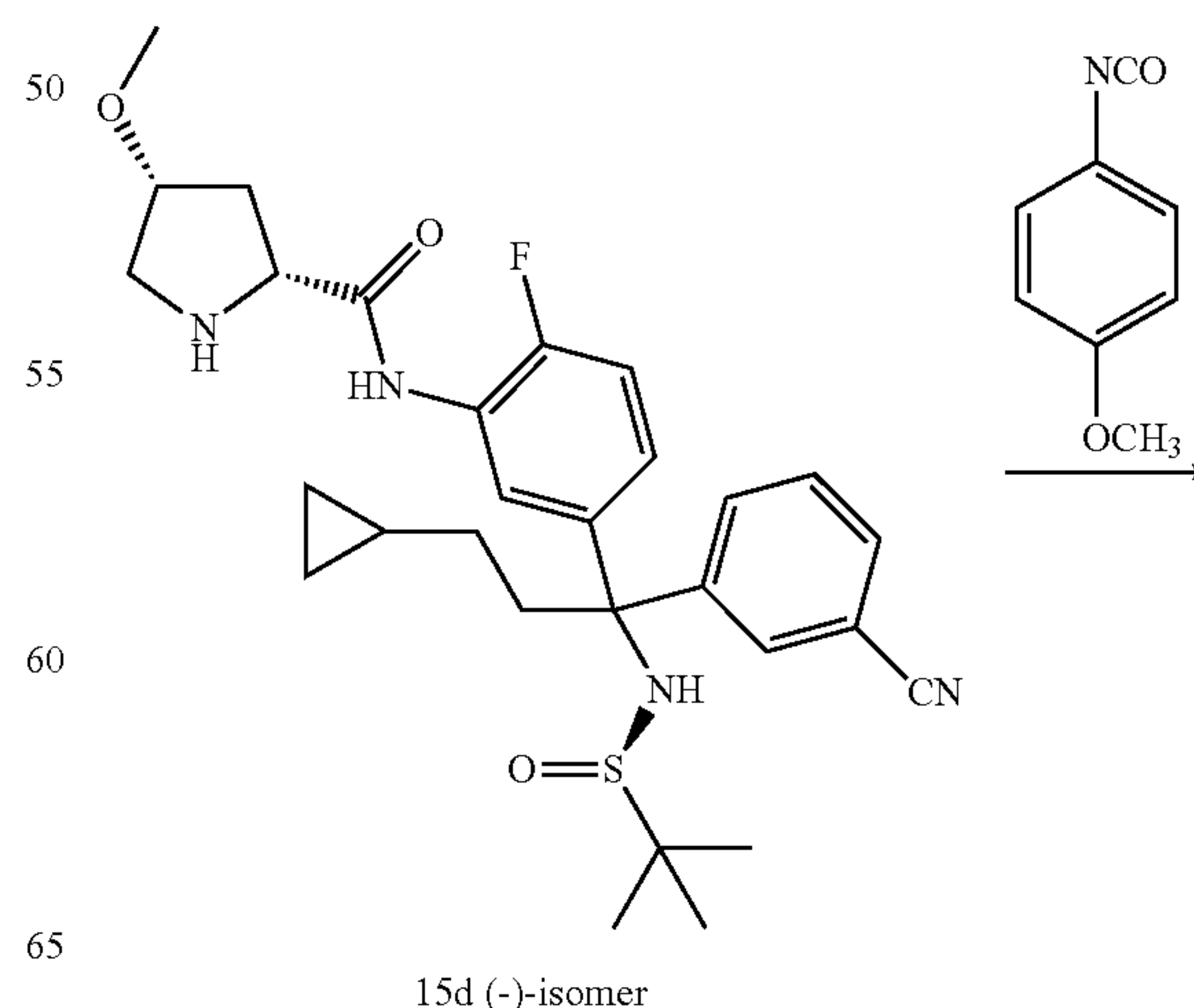
Scheme 16
