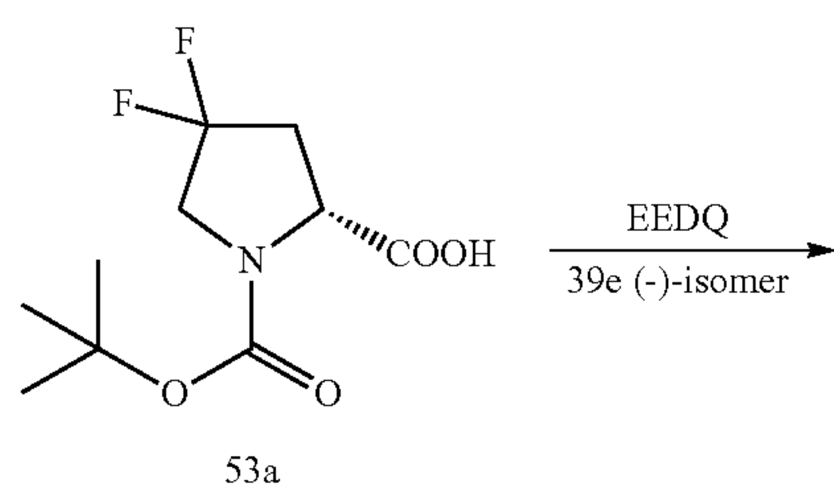
Scheme 53
