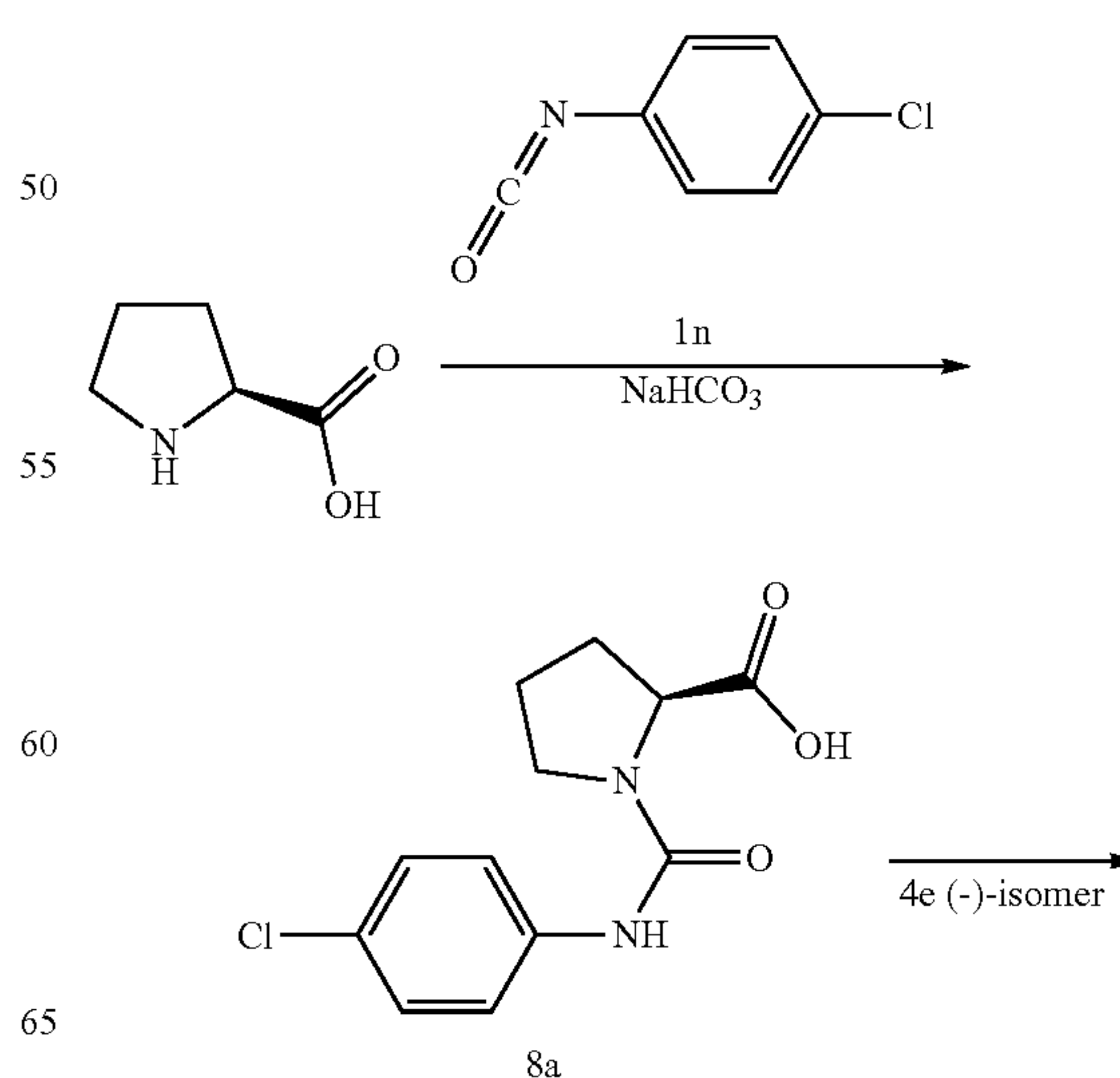
Scheme 8
