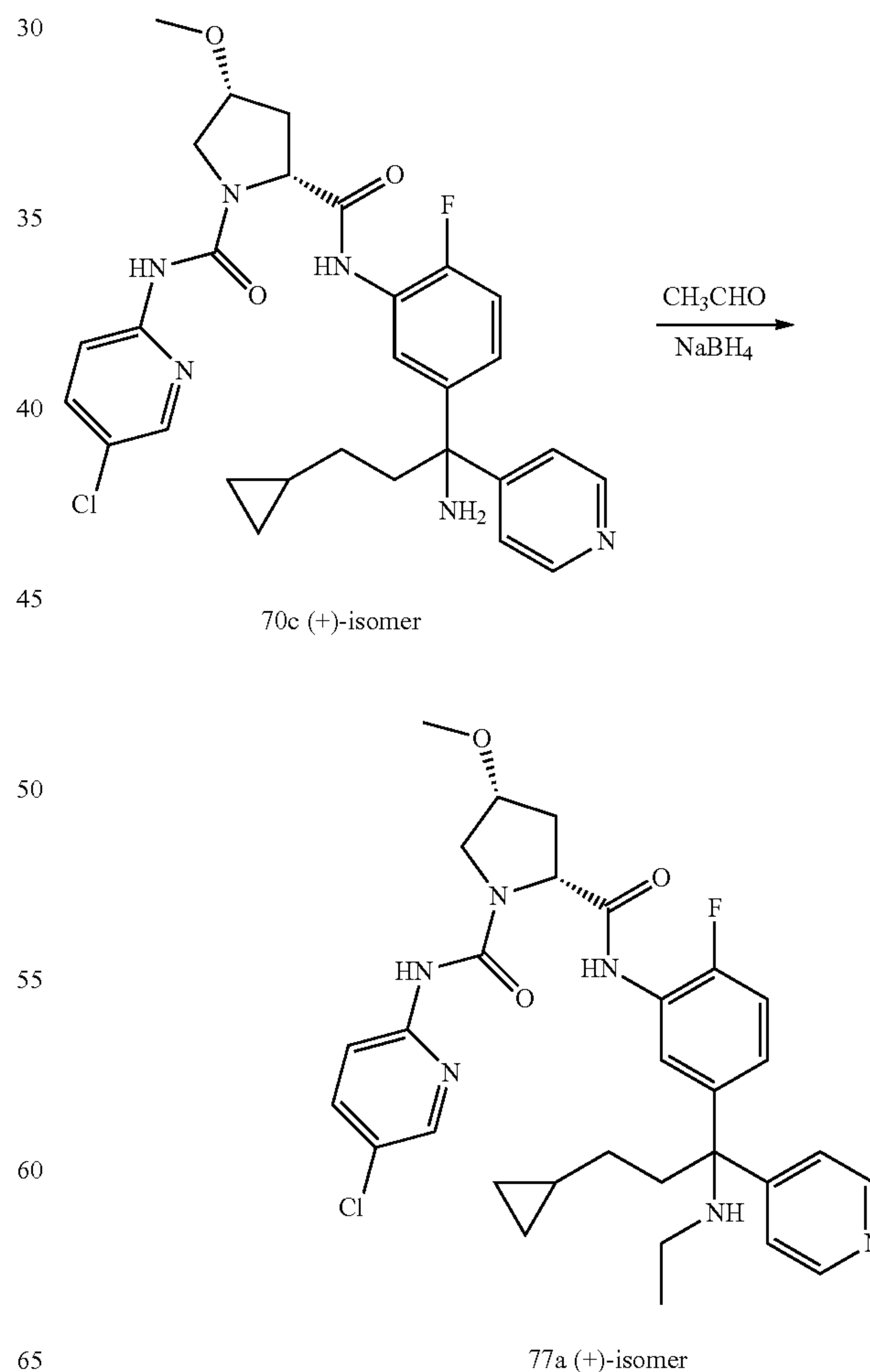
Scheme 77
