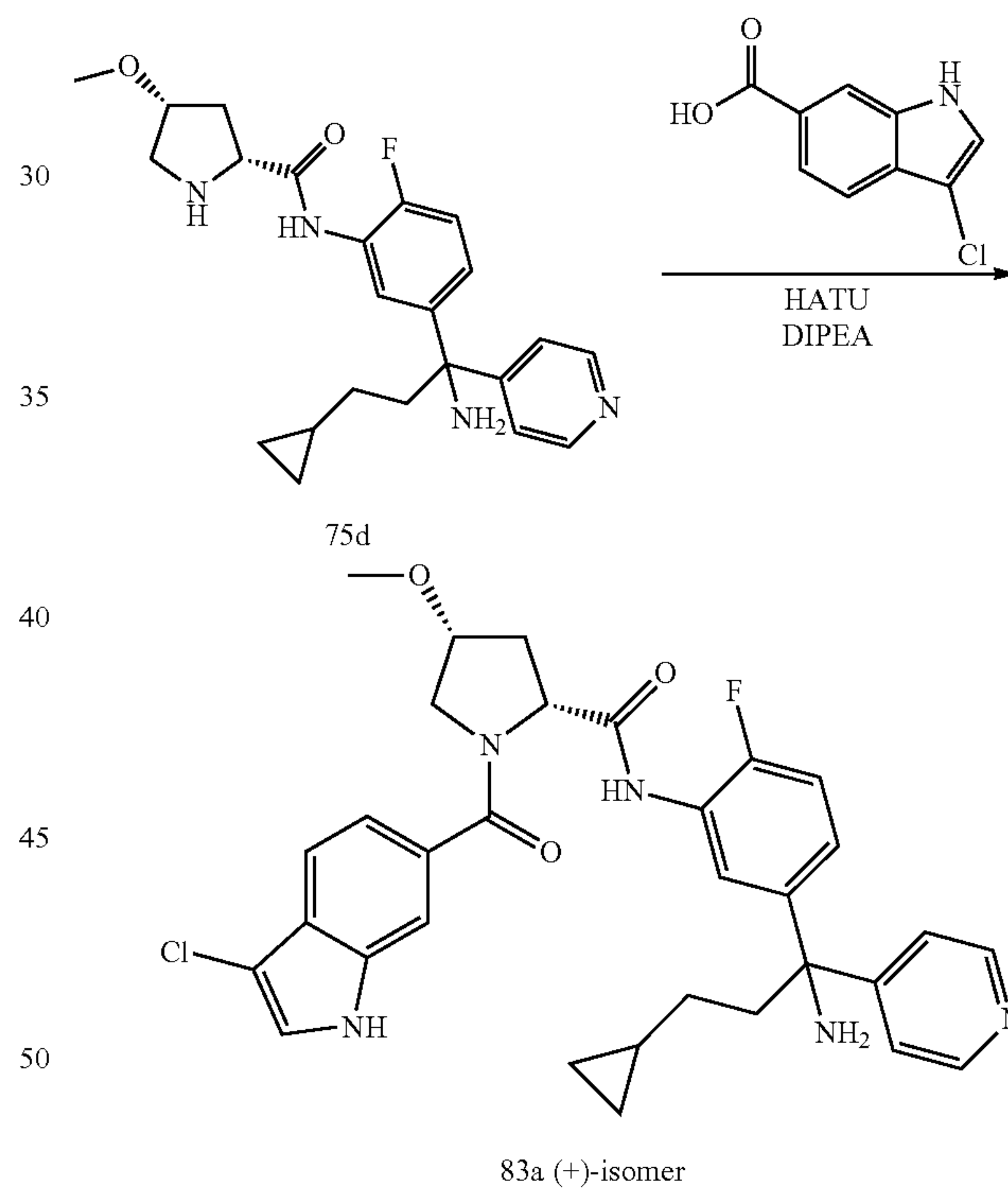
Scheme 83
