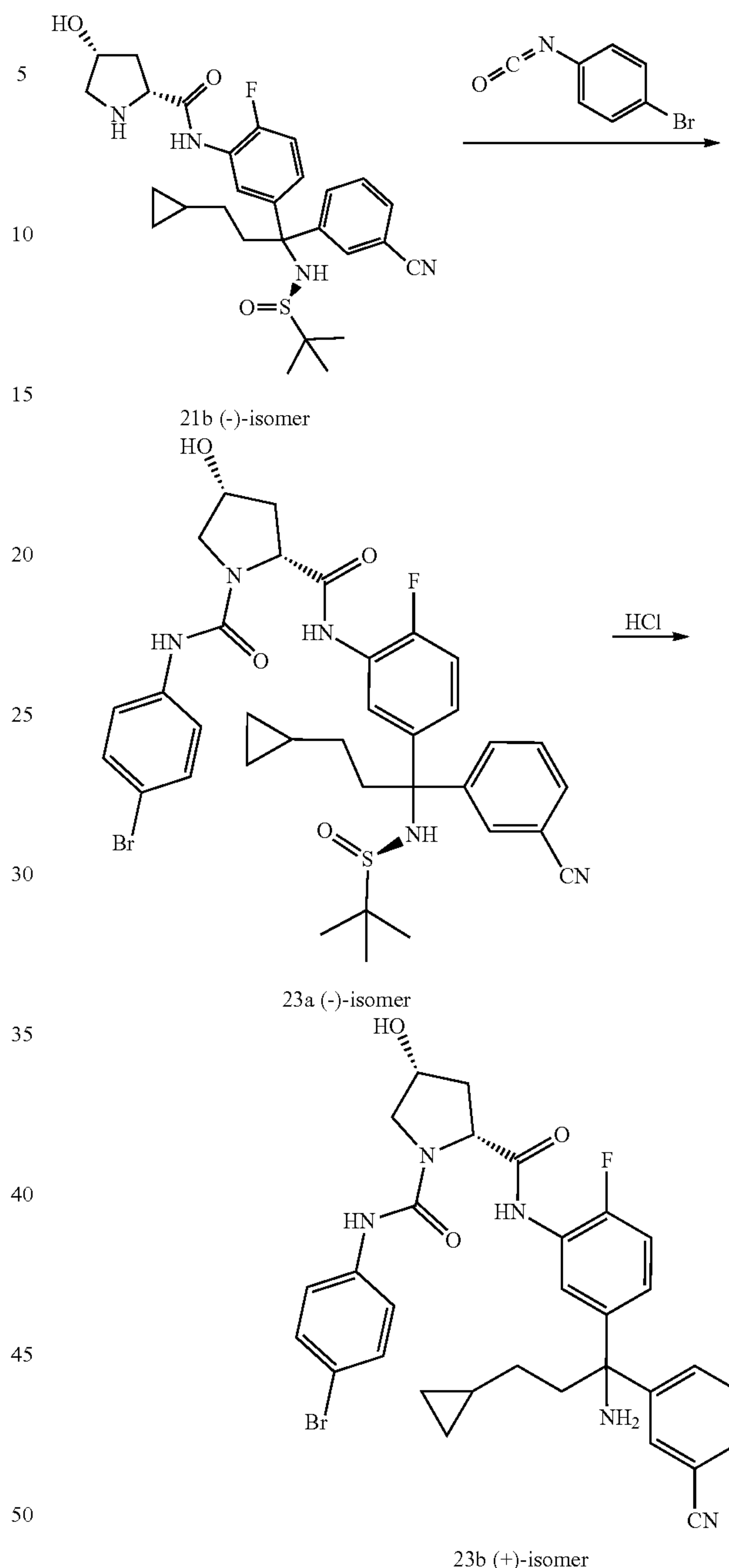
Scheme 23
