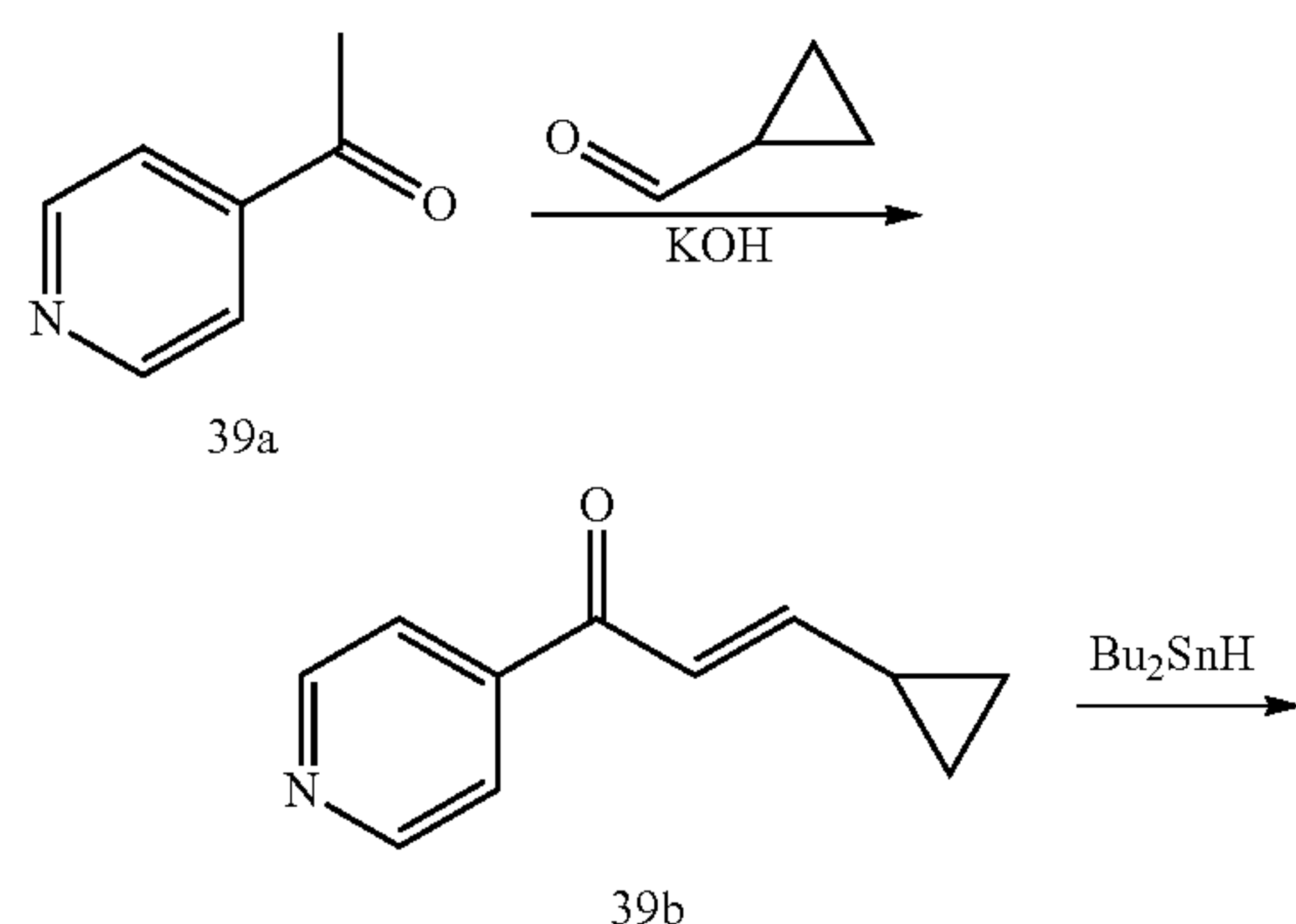
Scheme 39
