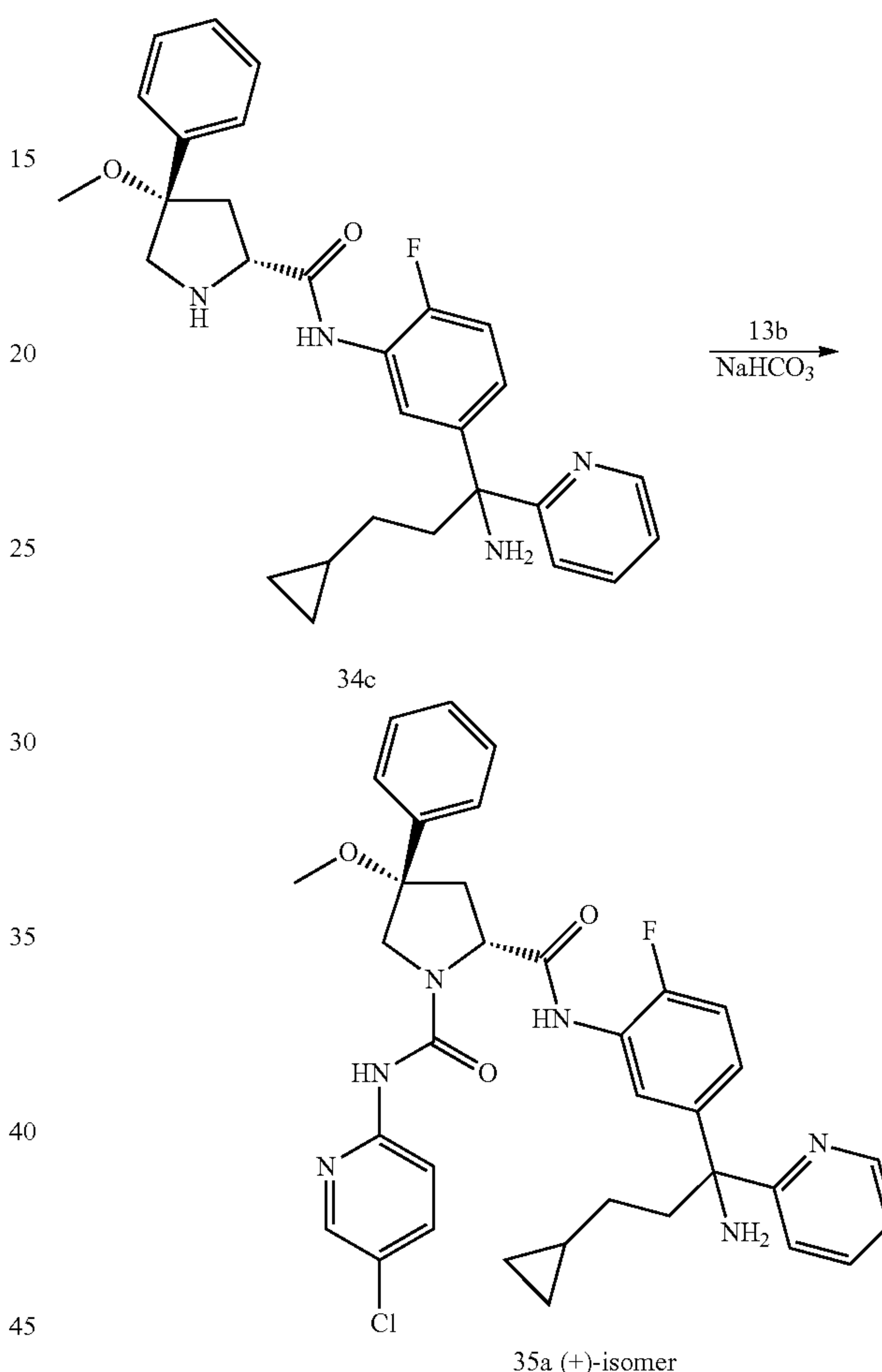
Scheme 35
