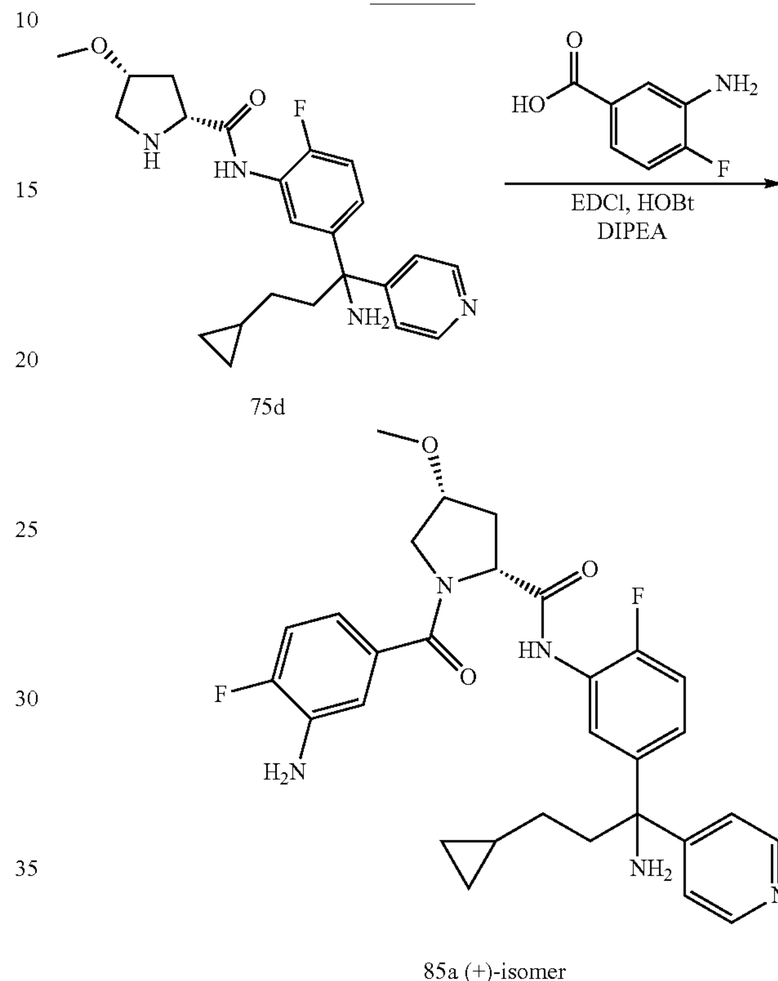
Scheme 85
