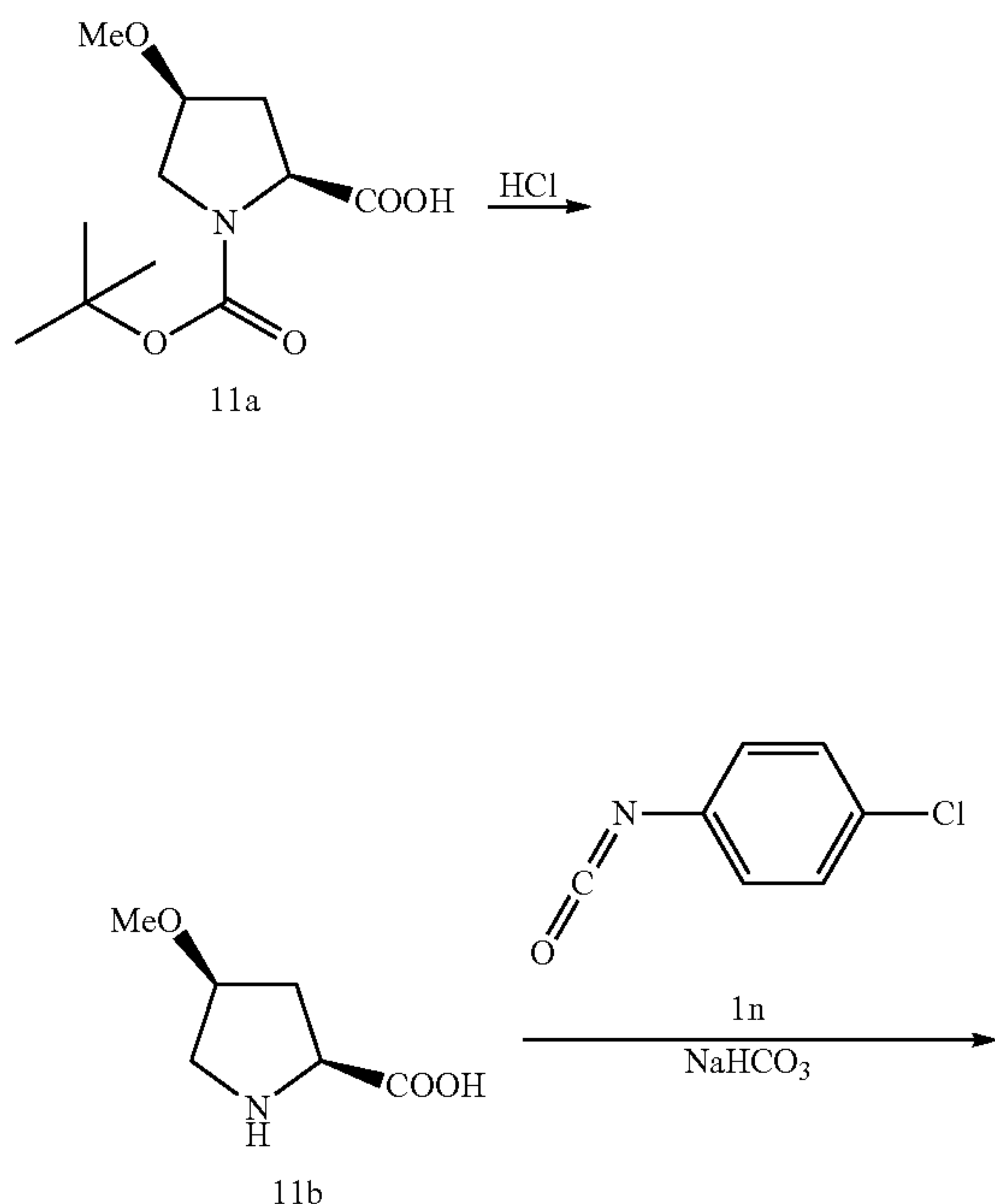
Scheme 11
