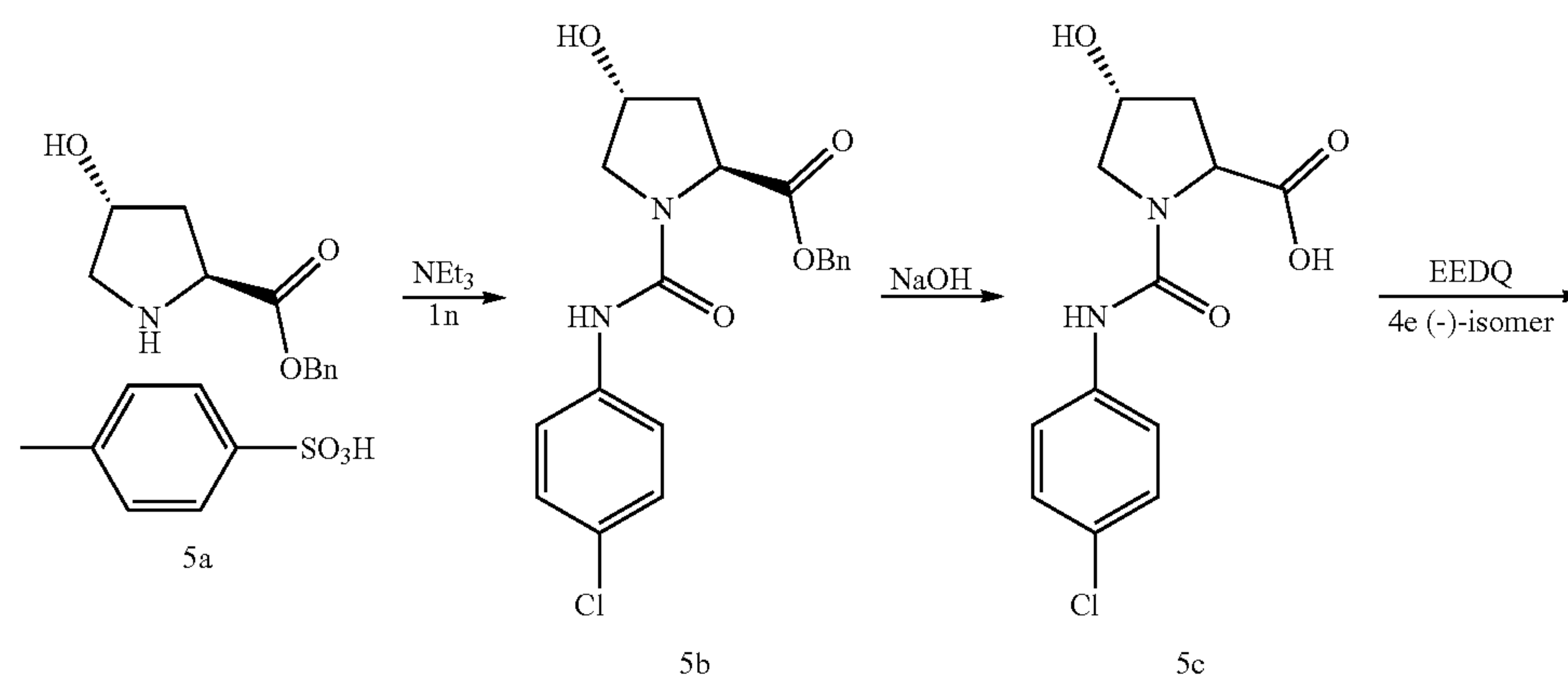
Scheme 5
