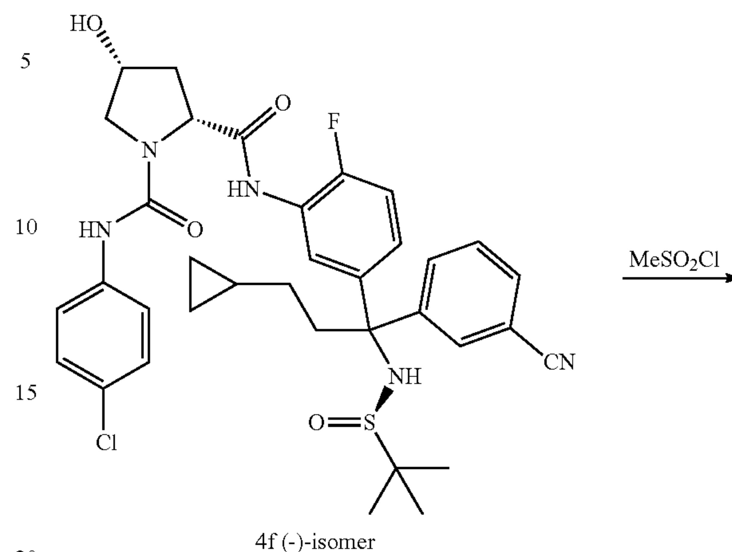
Scheme 33
