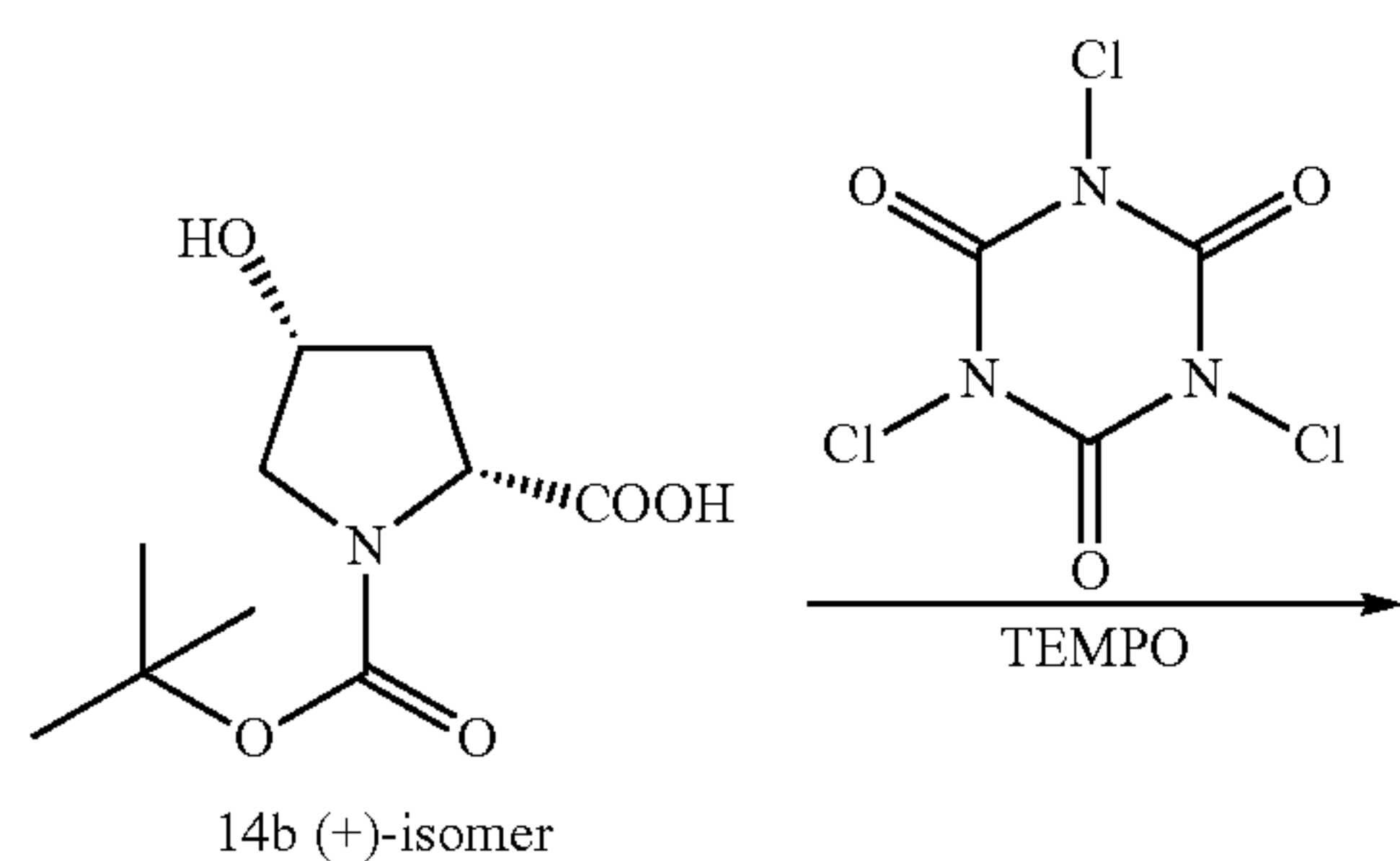
Scheme 29
