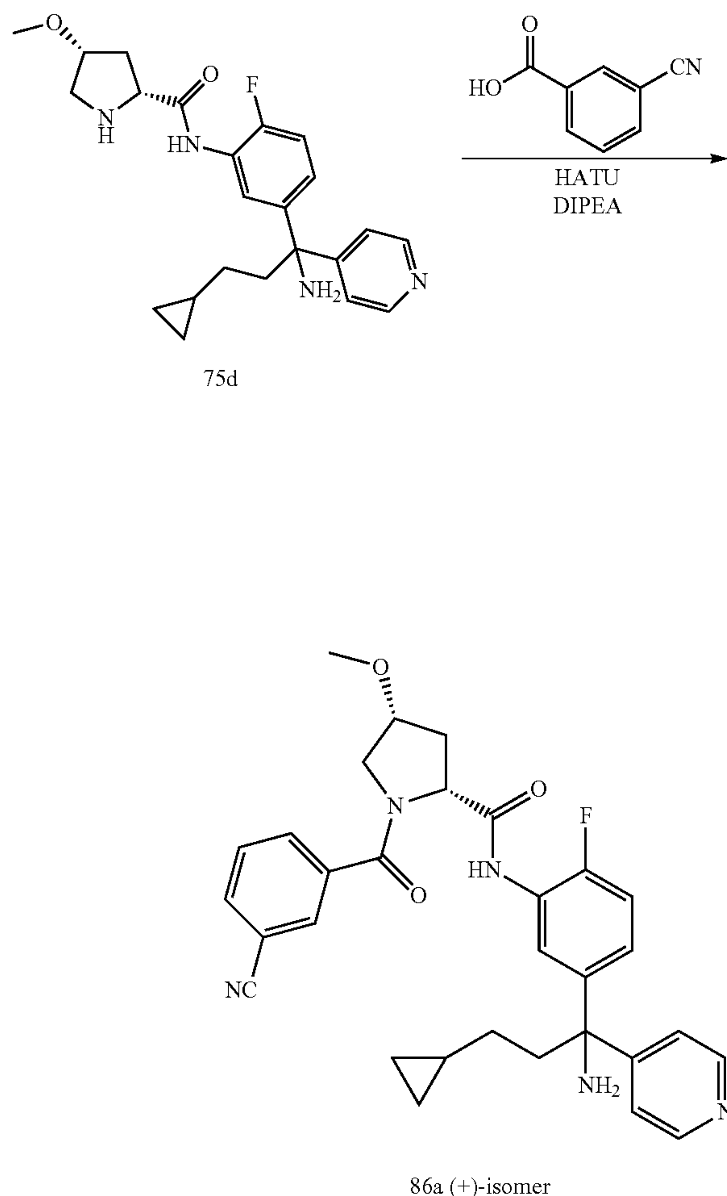
Scheme 86
