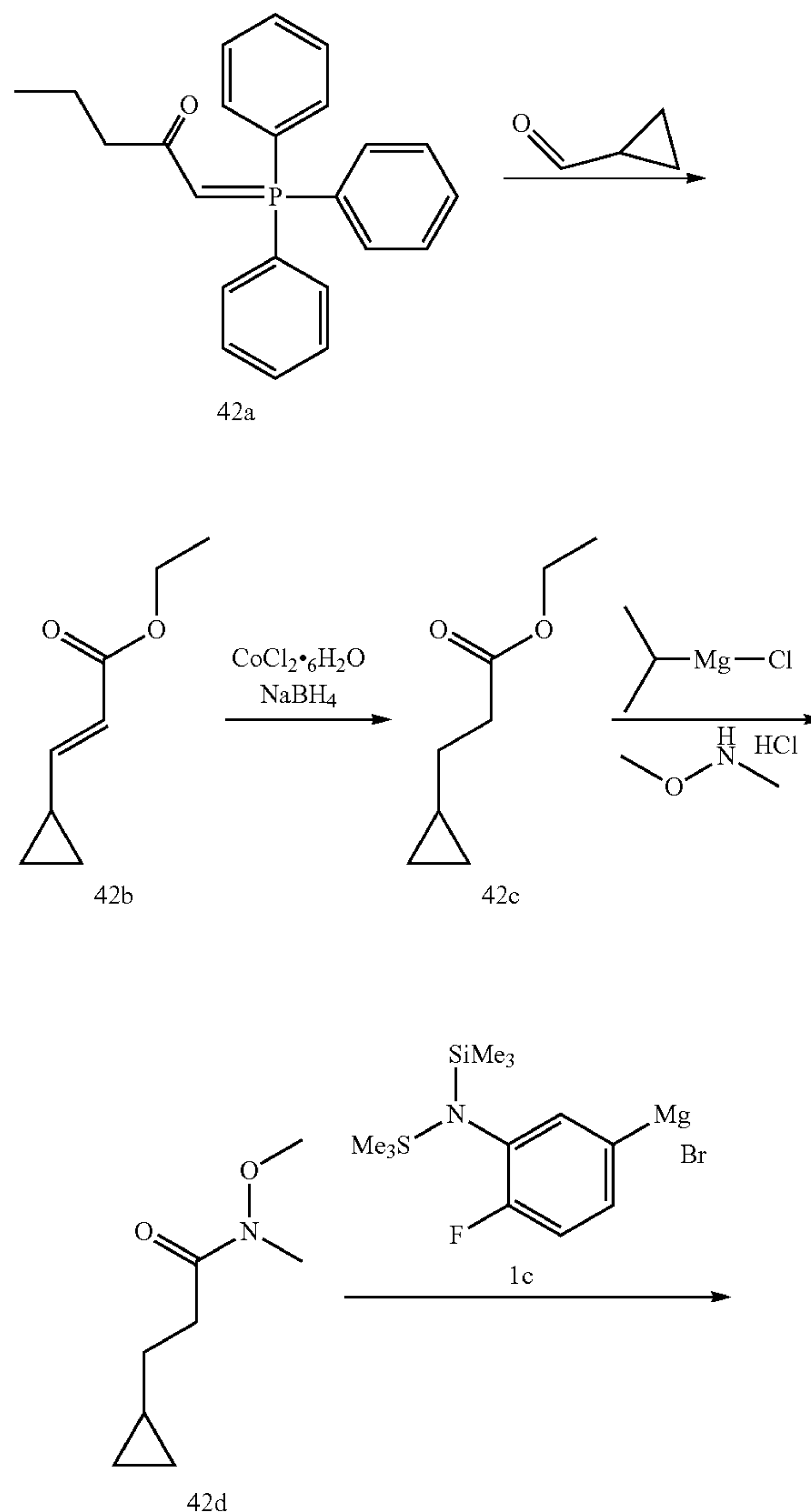
Scheme 42
