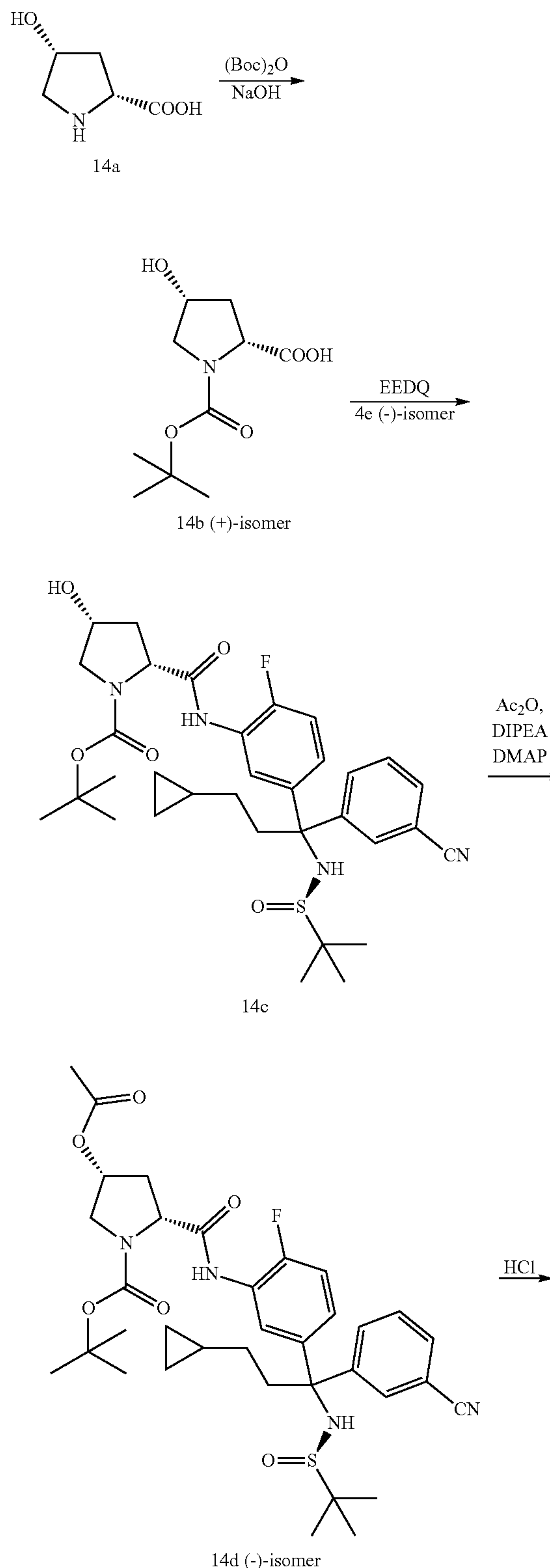
Scheme 14
