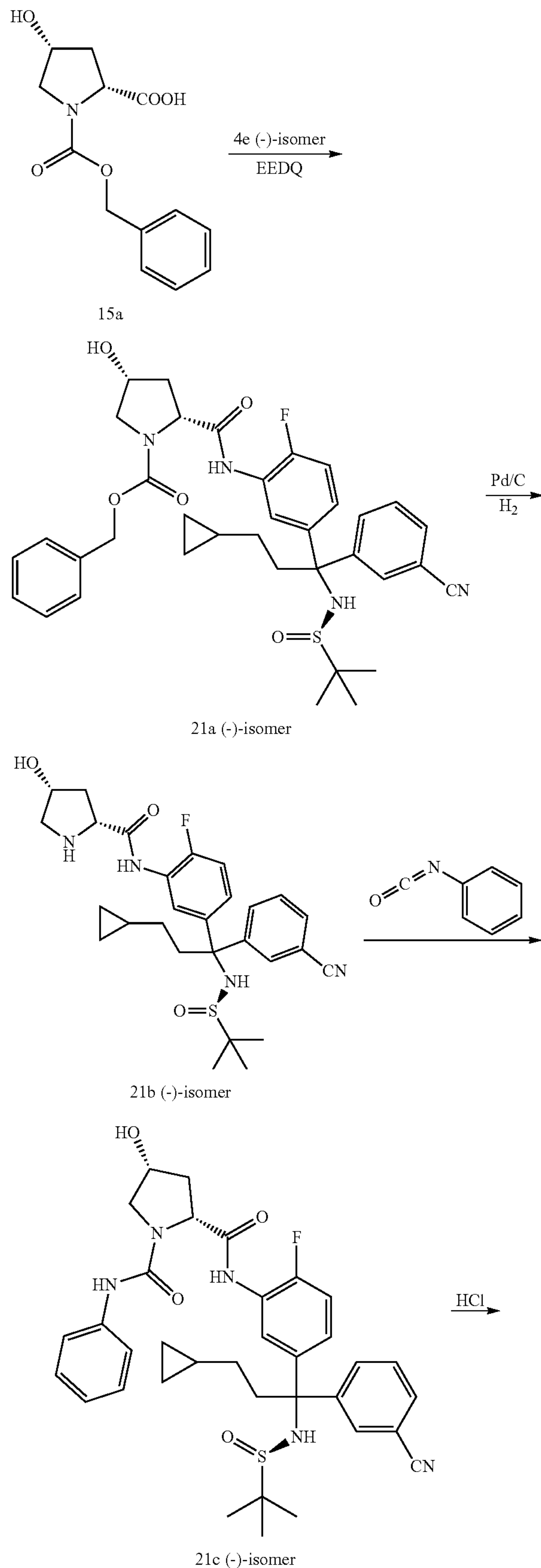
Scheme 21
