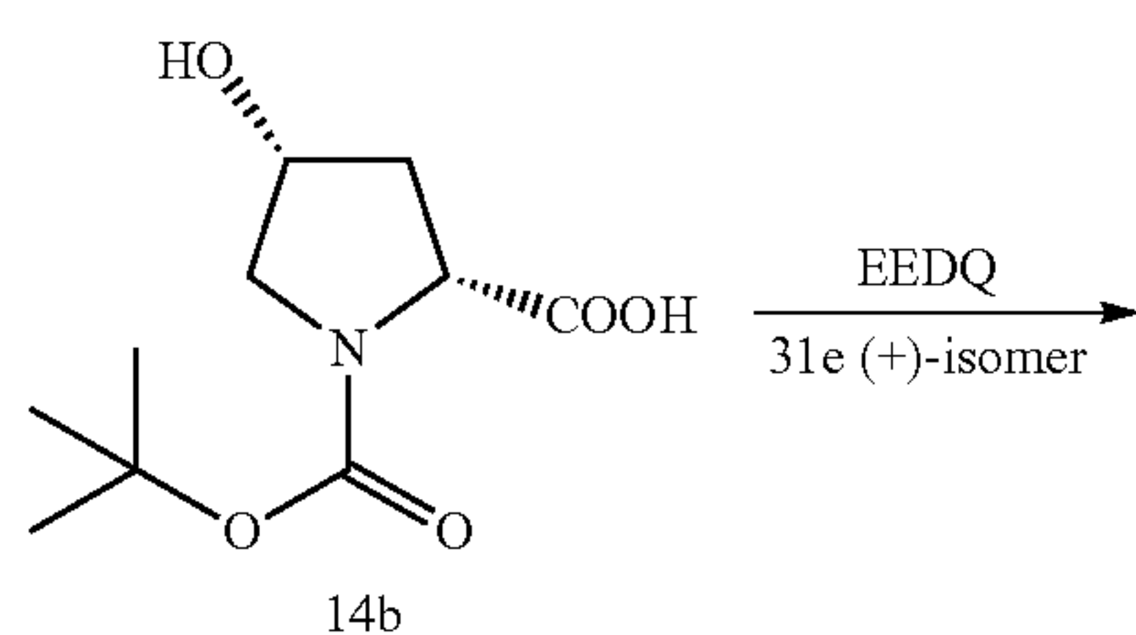
Scheme 62
