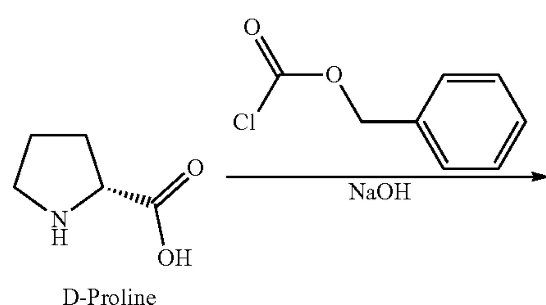
Scheme 12
