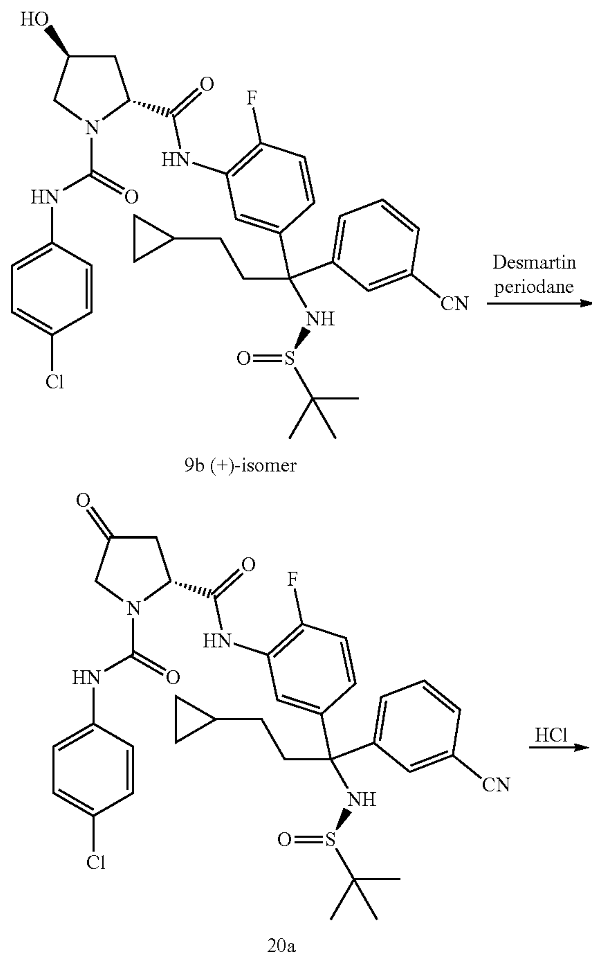
Scheme 20
