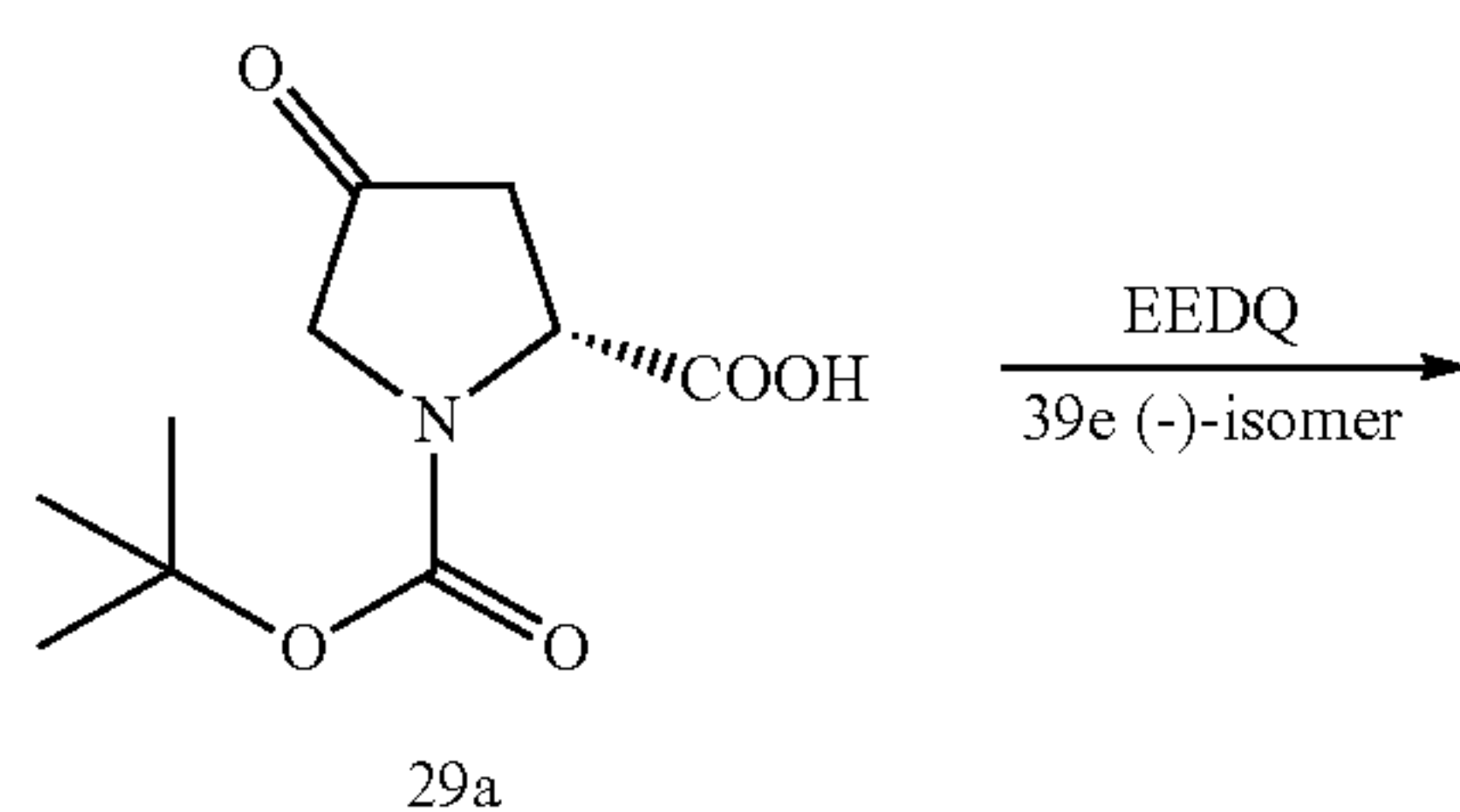
Scheme 59
