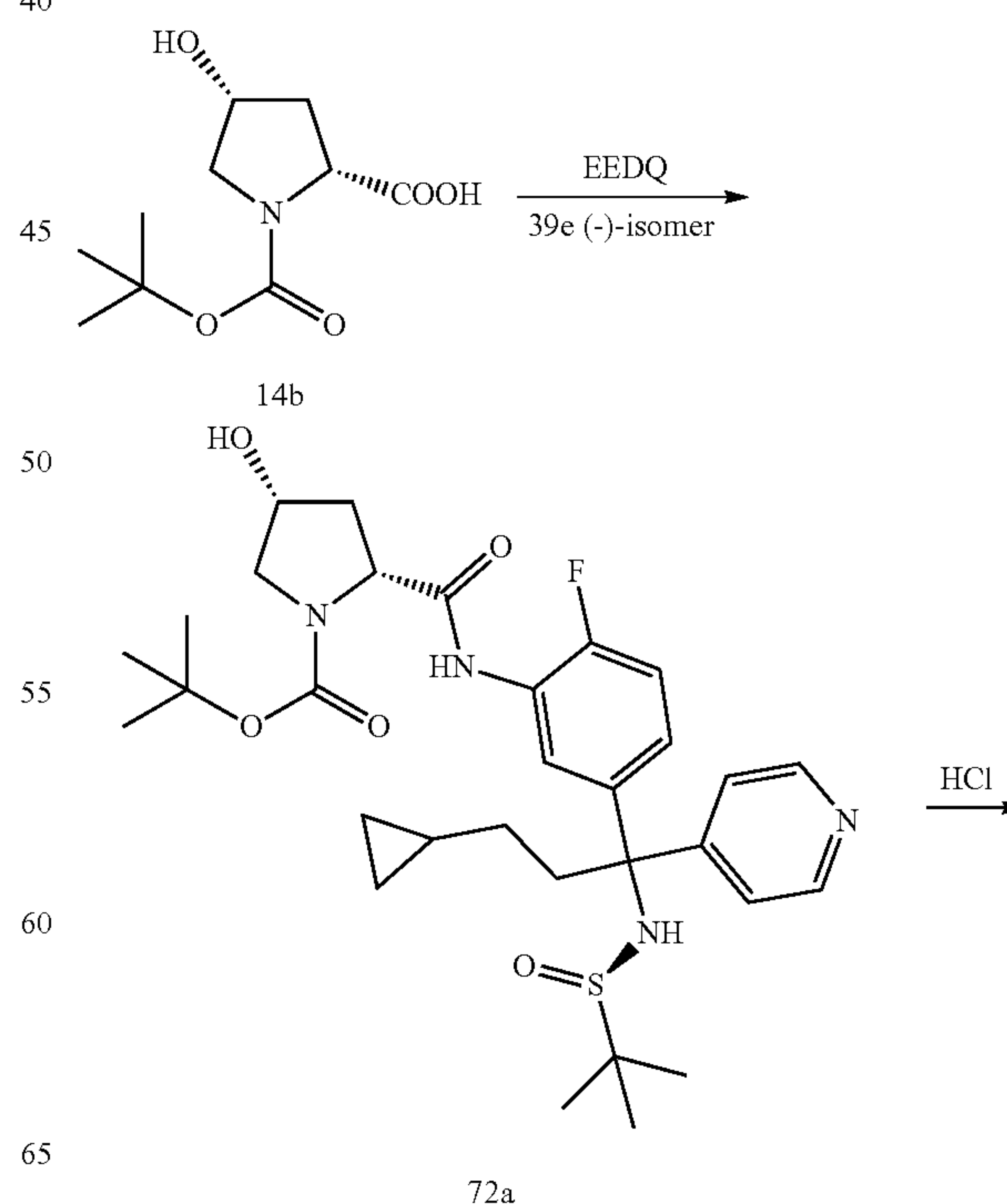
Scheme 72
