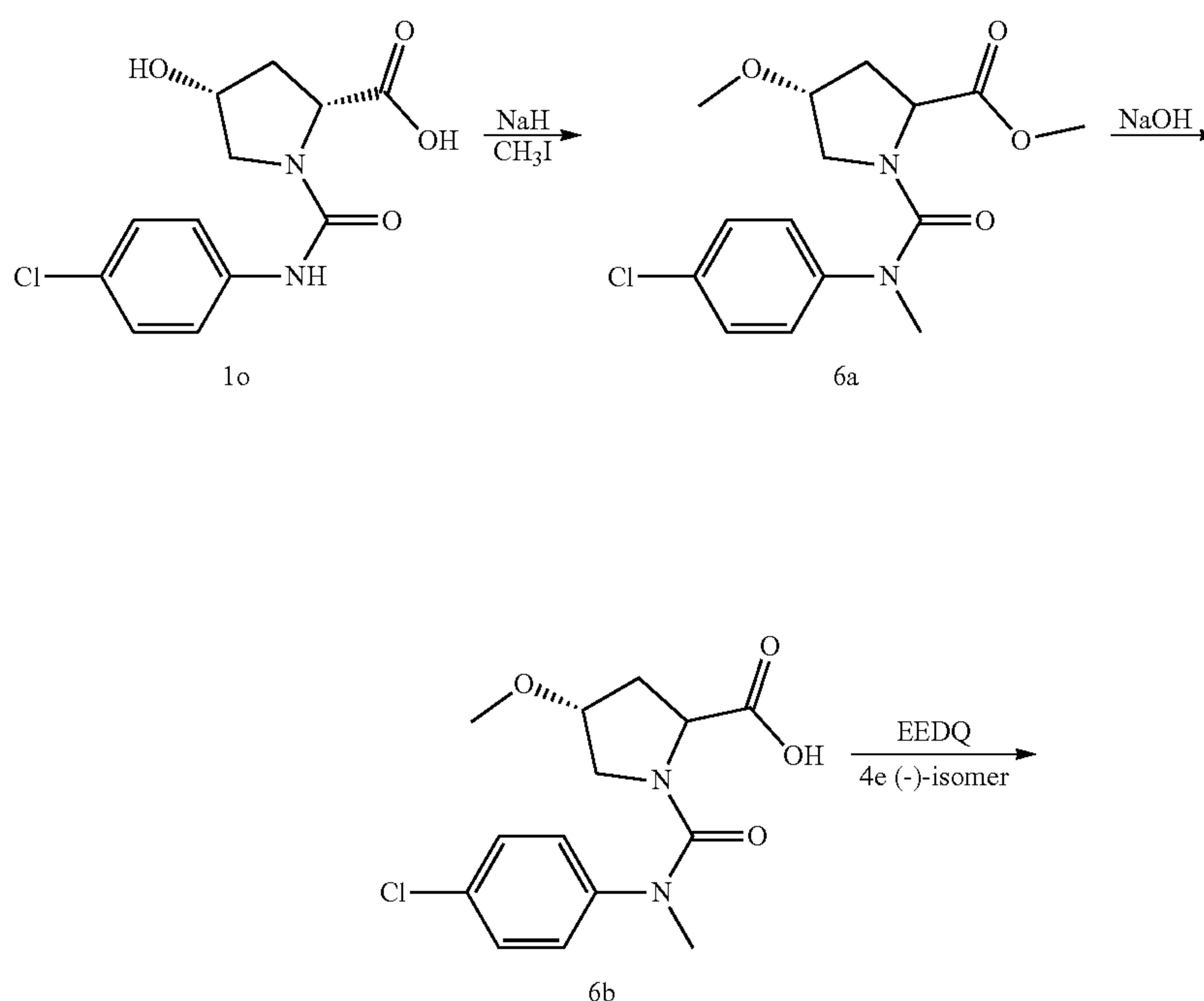
Scheme 6
