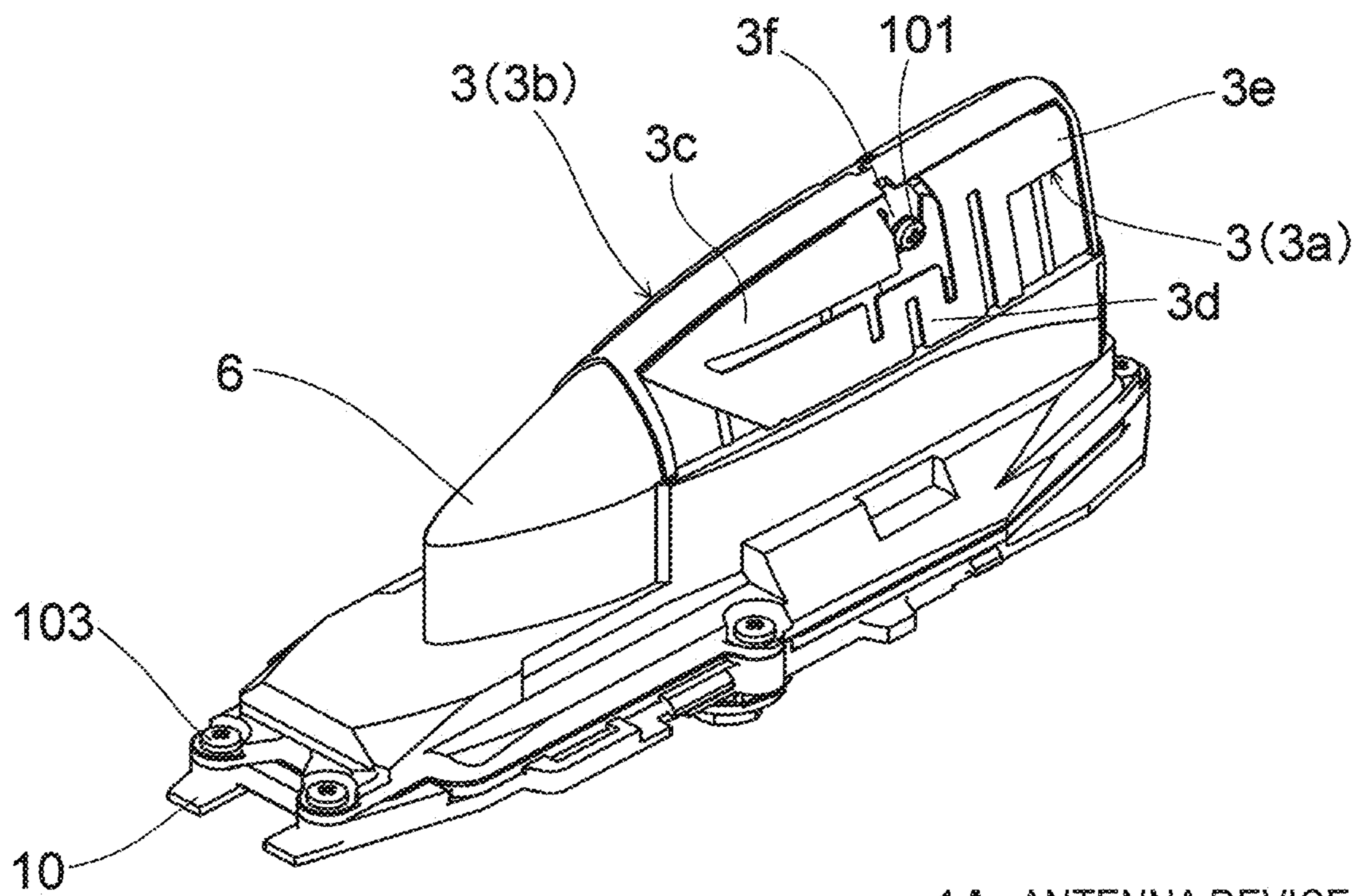
1A: ANTENNA DEVICE
