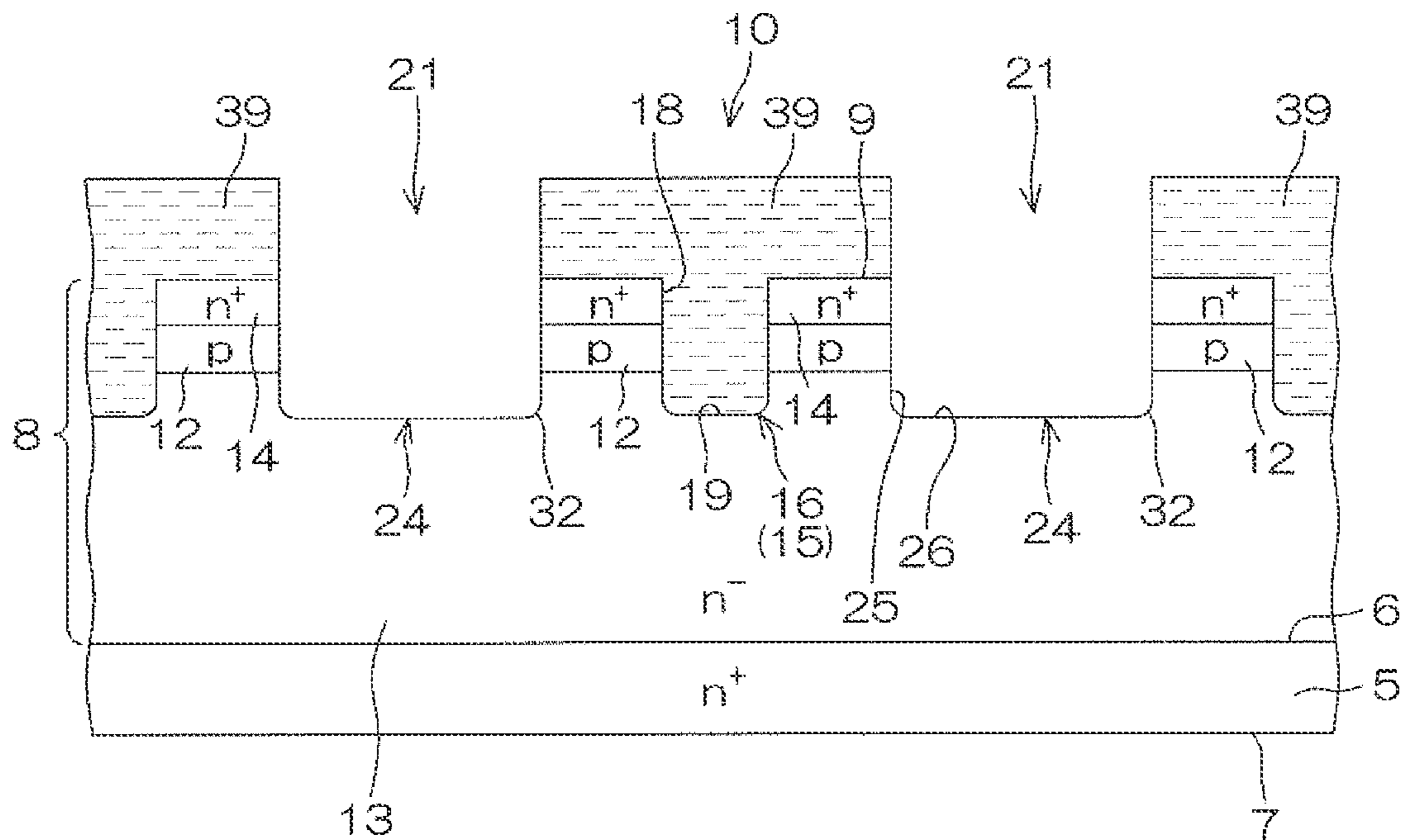
B-B SECTION
