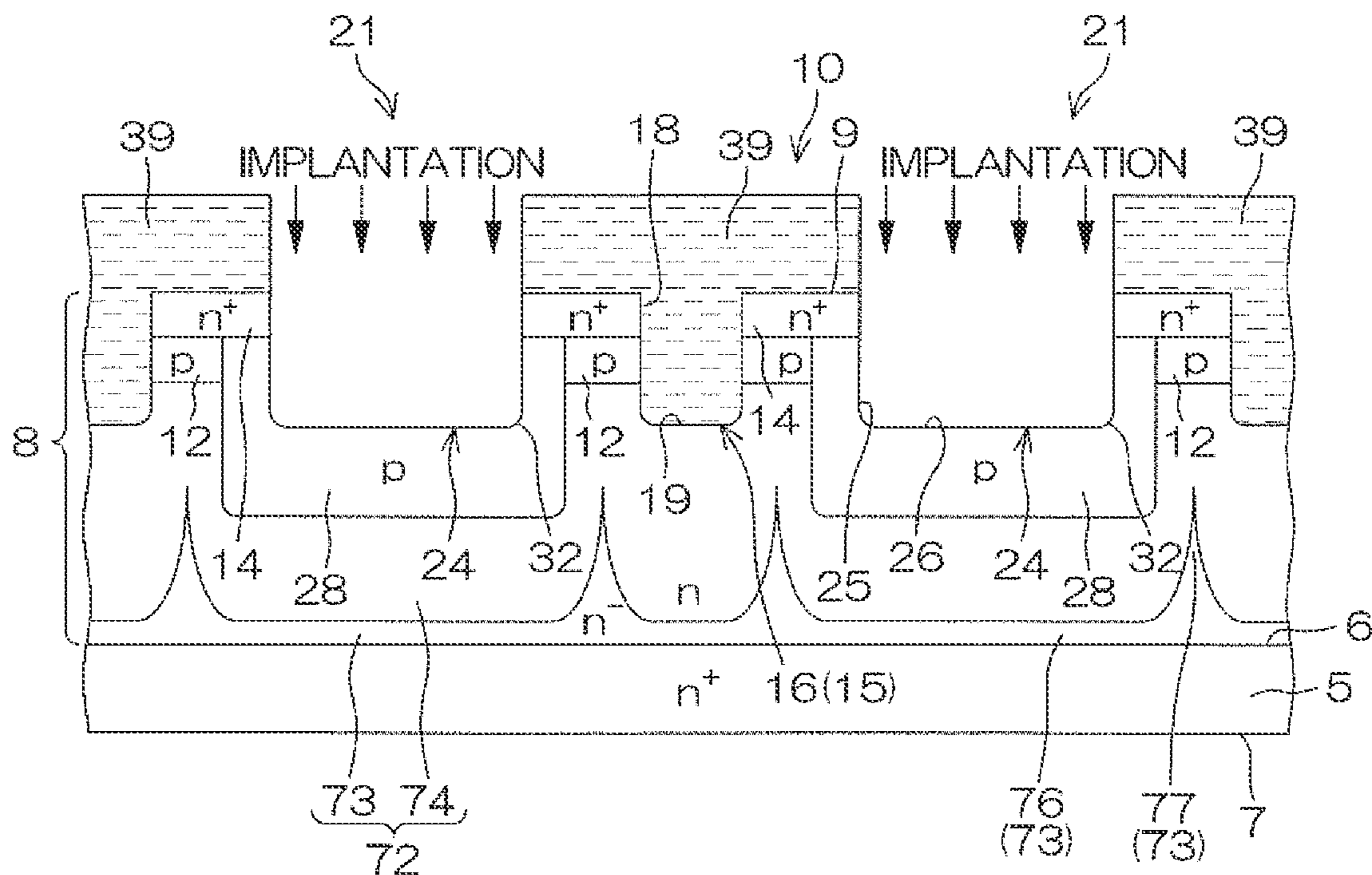
B-B SECTION
