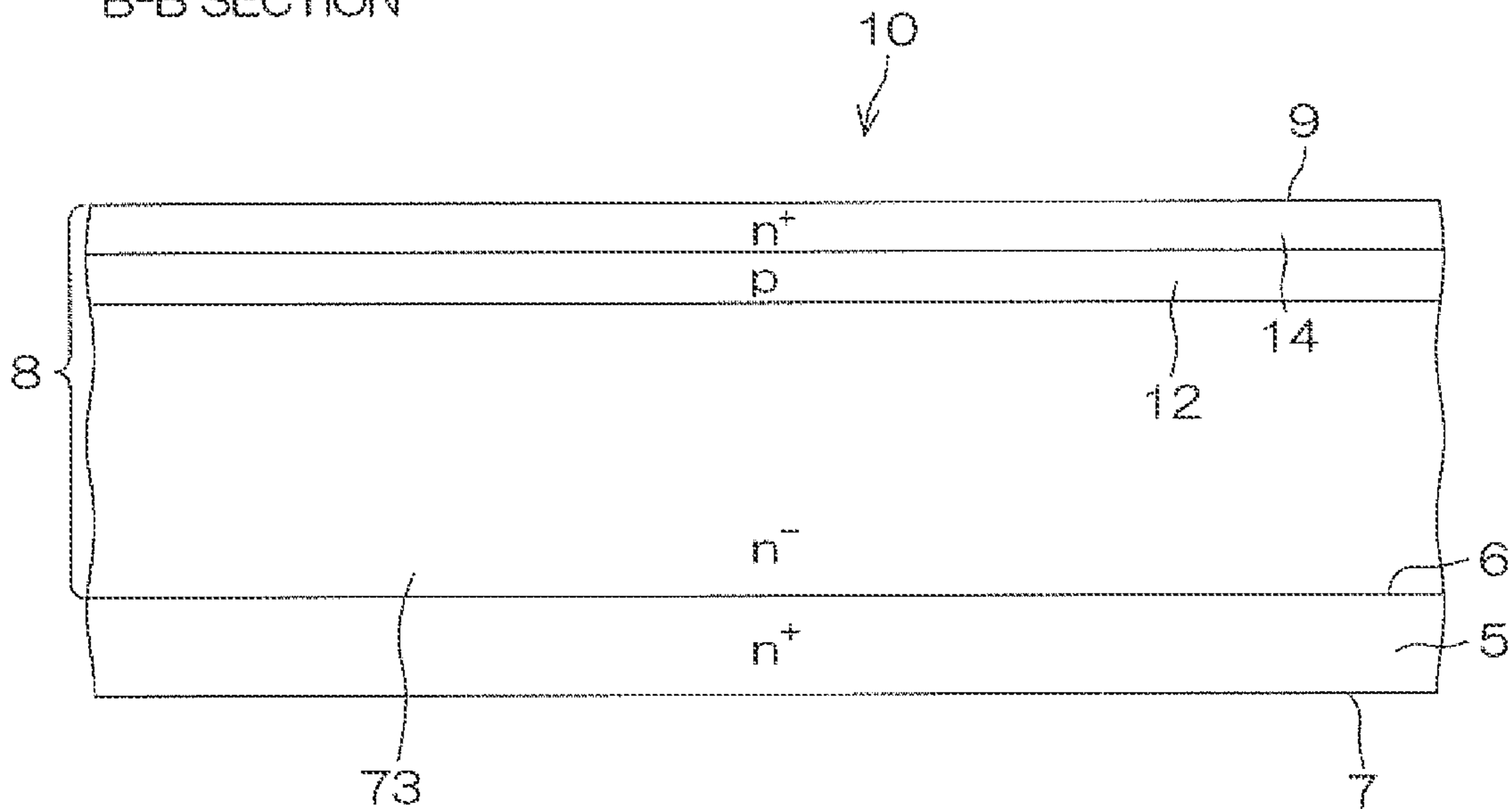
B-B SECTION
