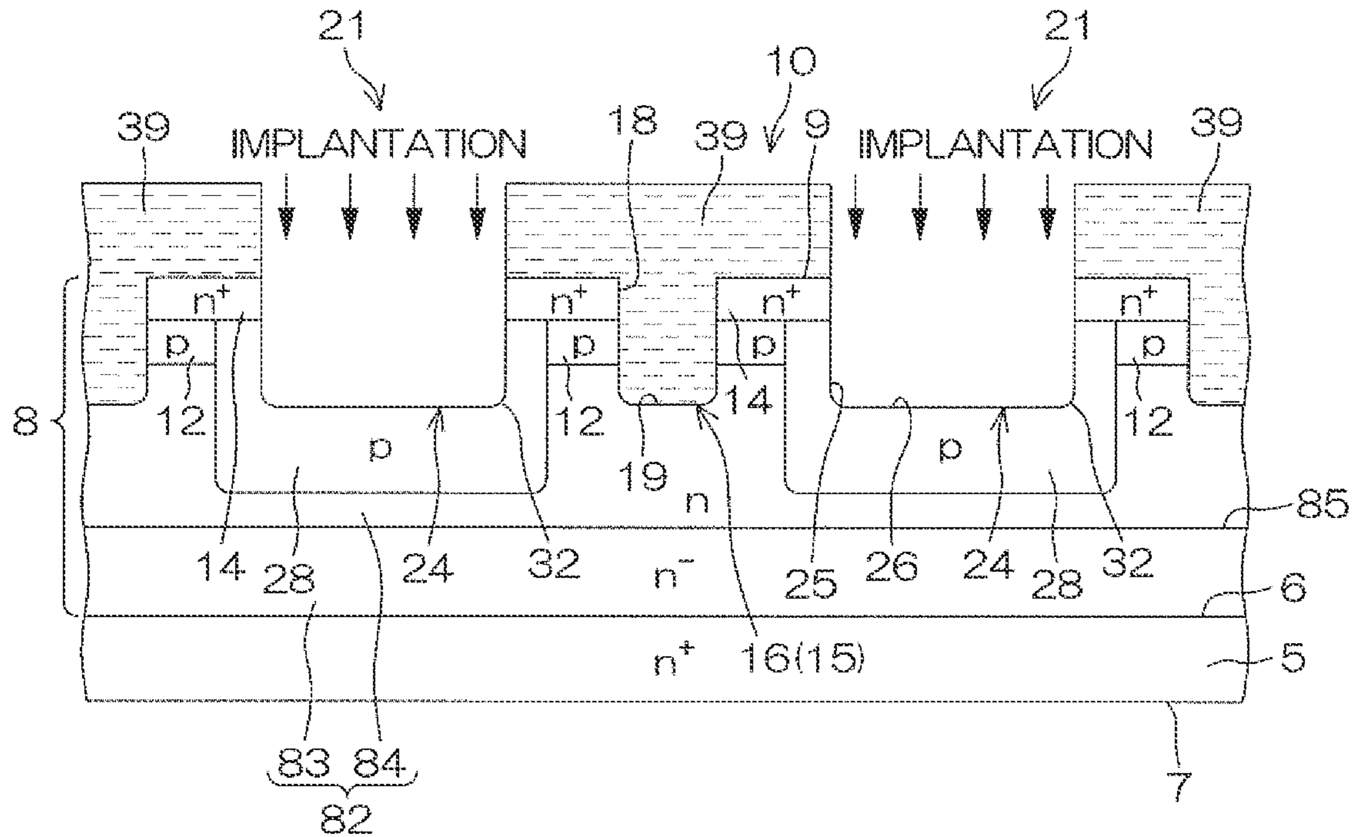
B-B SECTION
