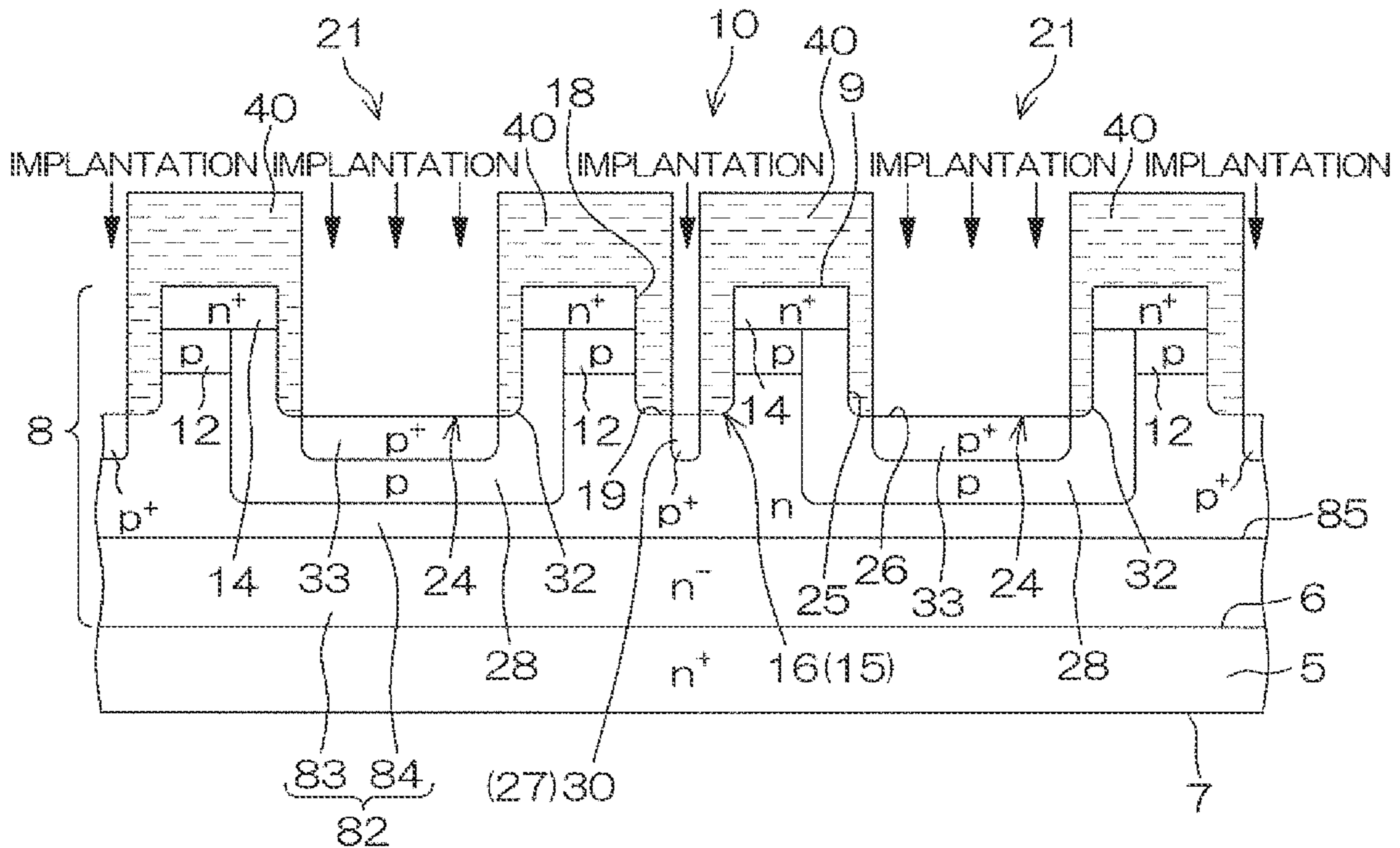
B-B SECTION
