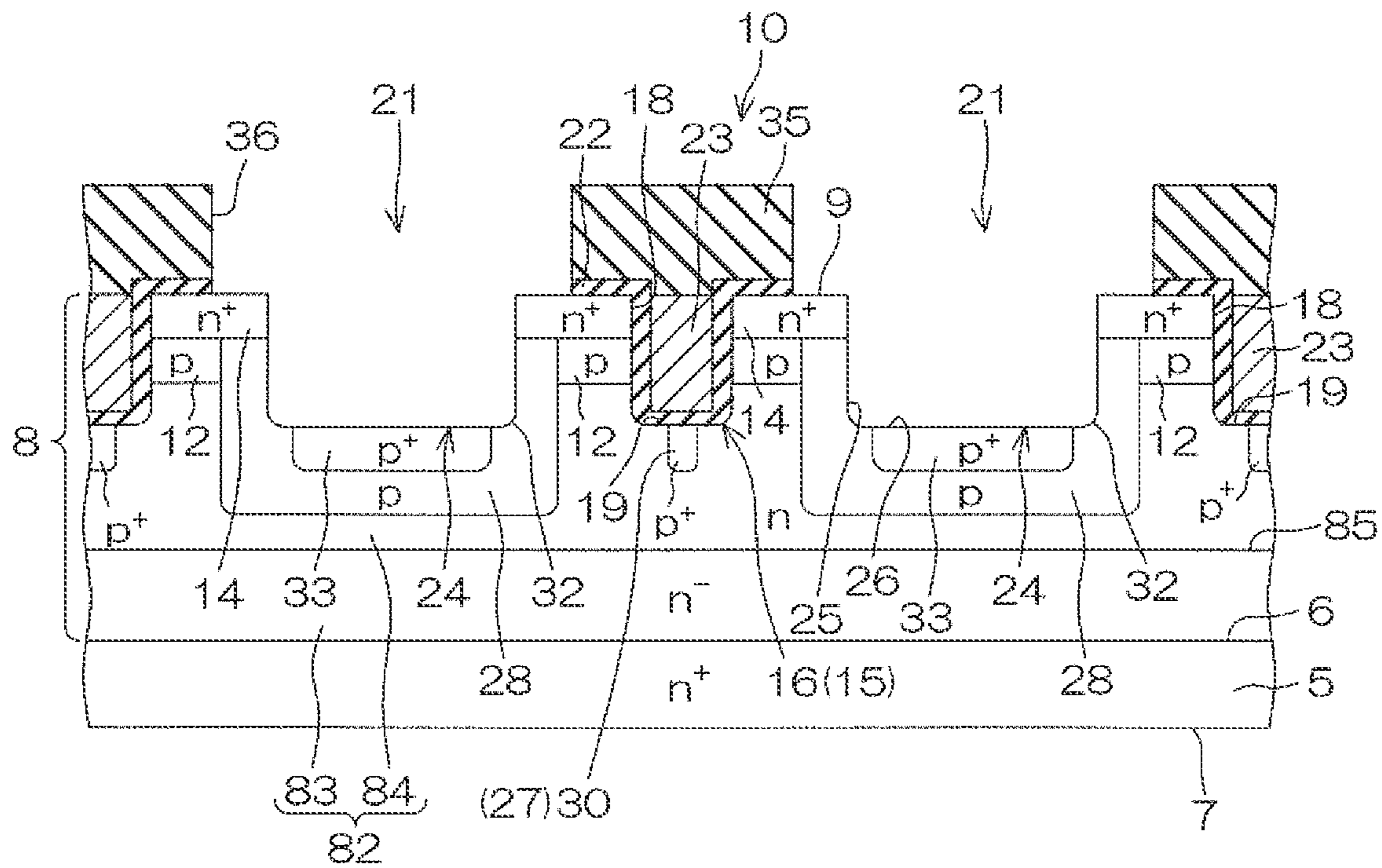
B-B SECTION
