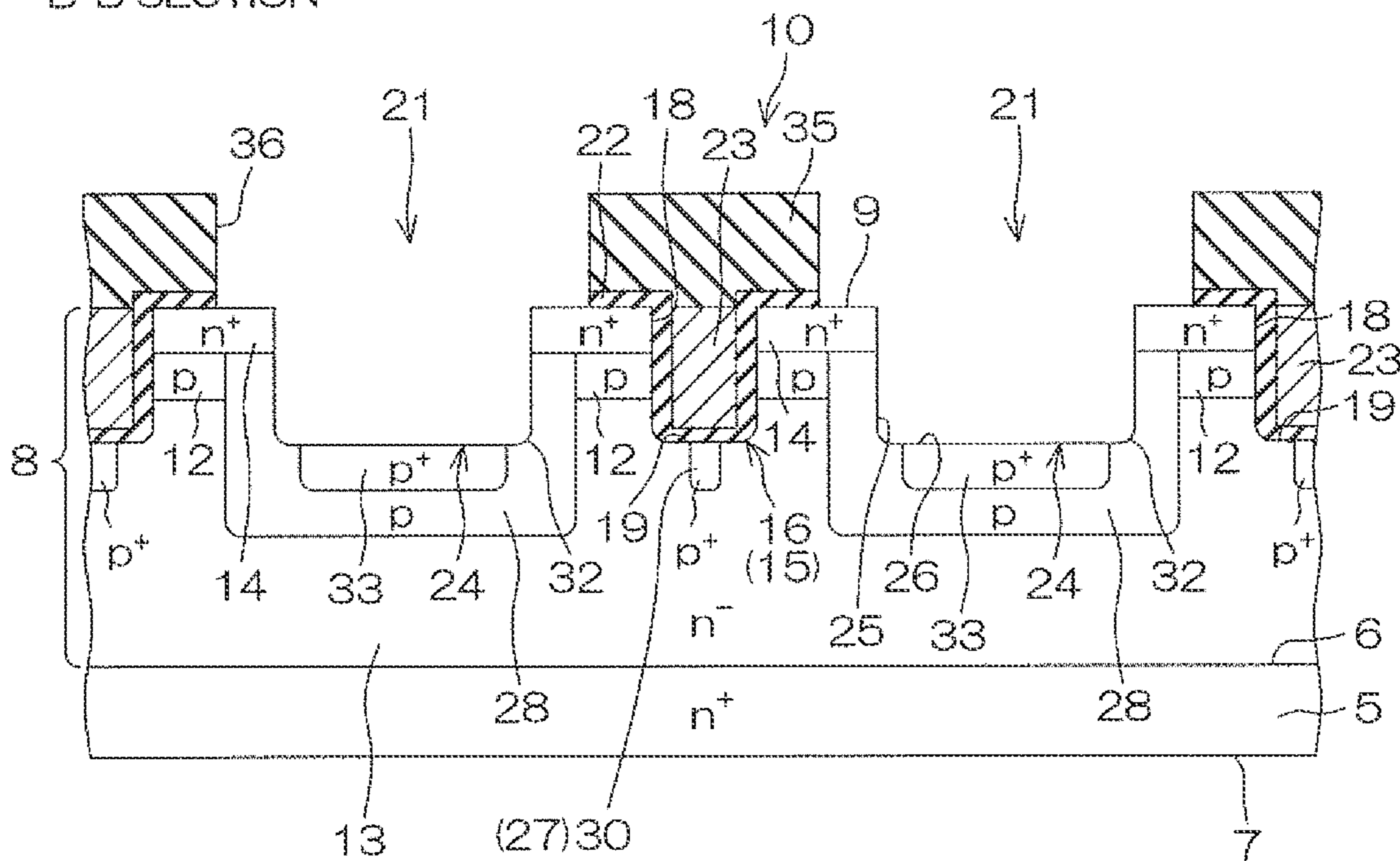
B-B SECTION
