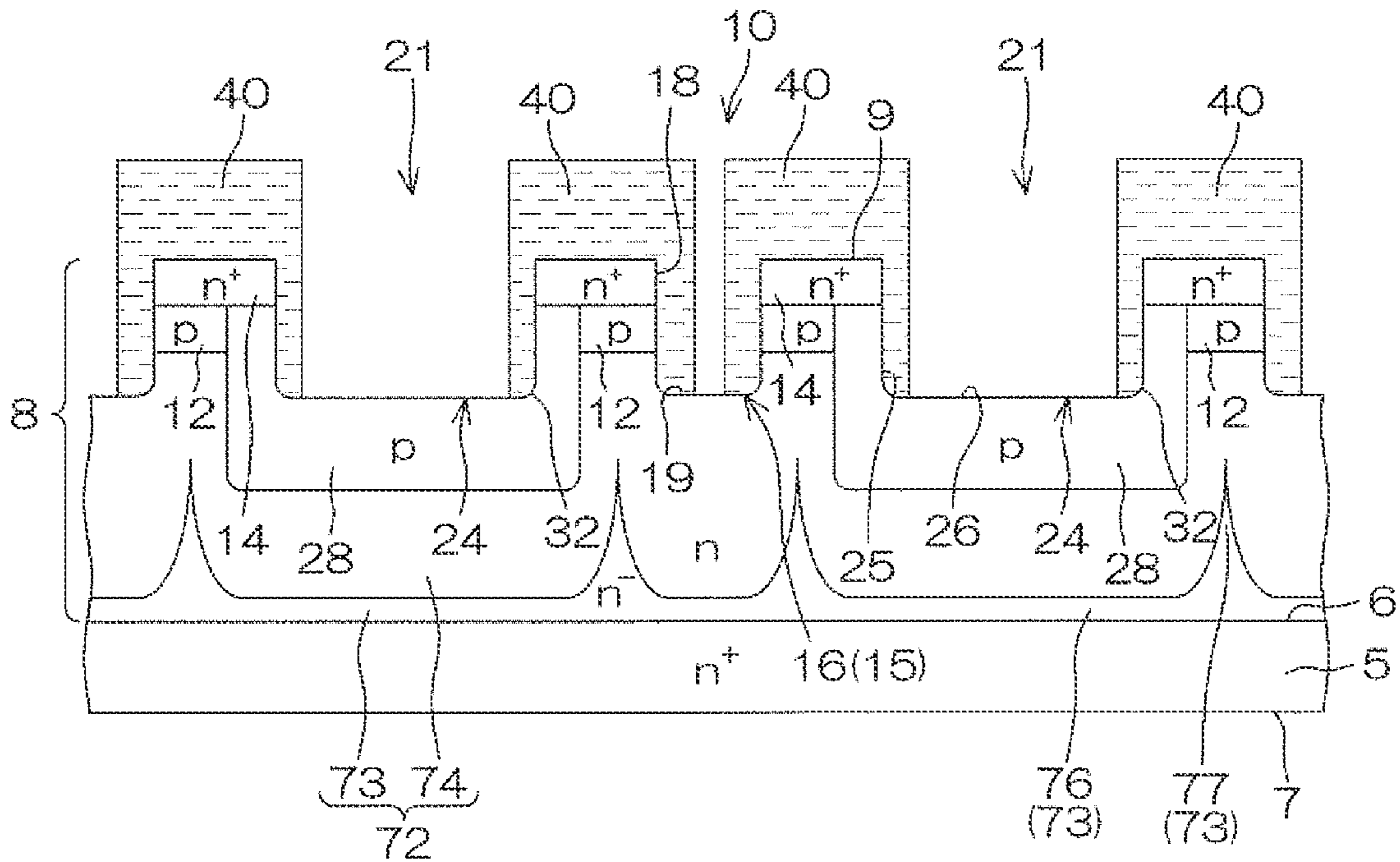
B-B SECTION
