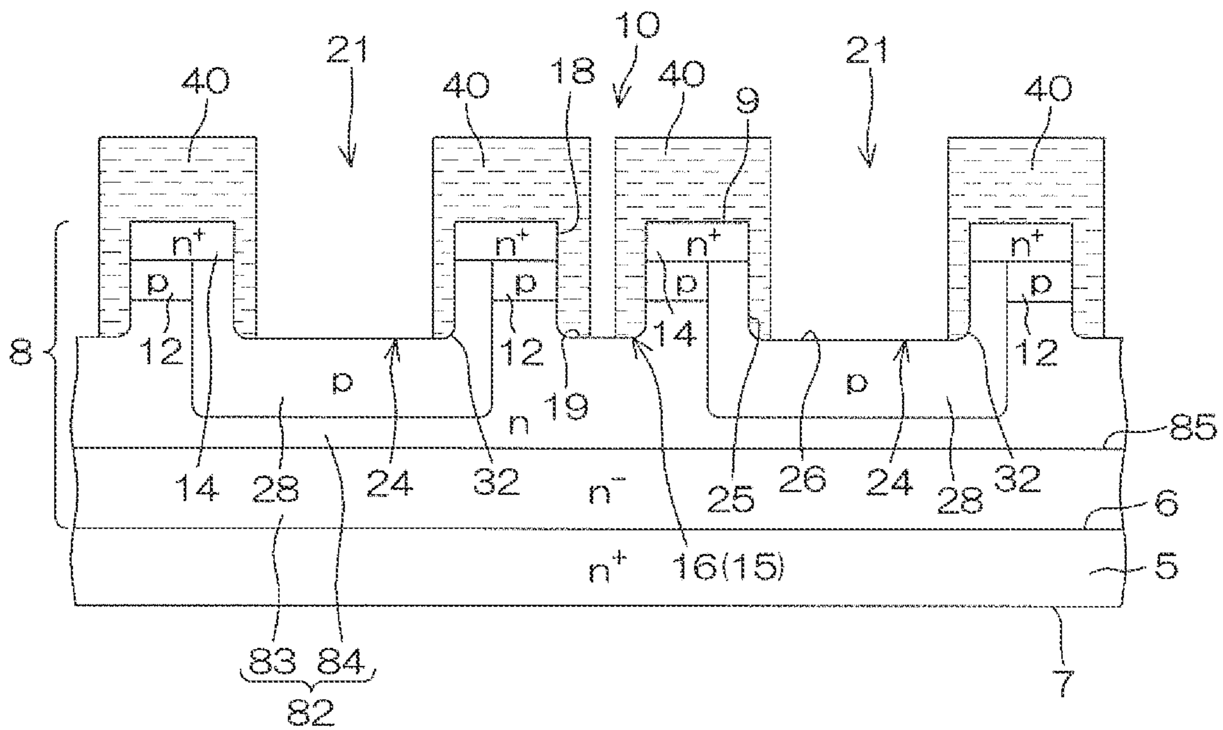
B-B SECTION
