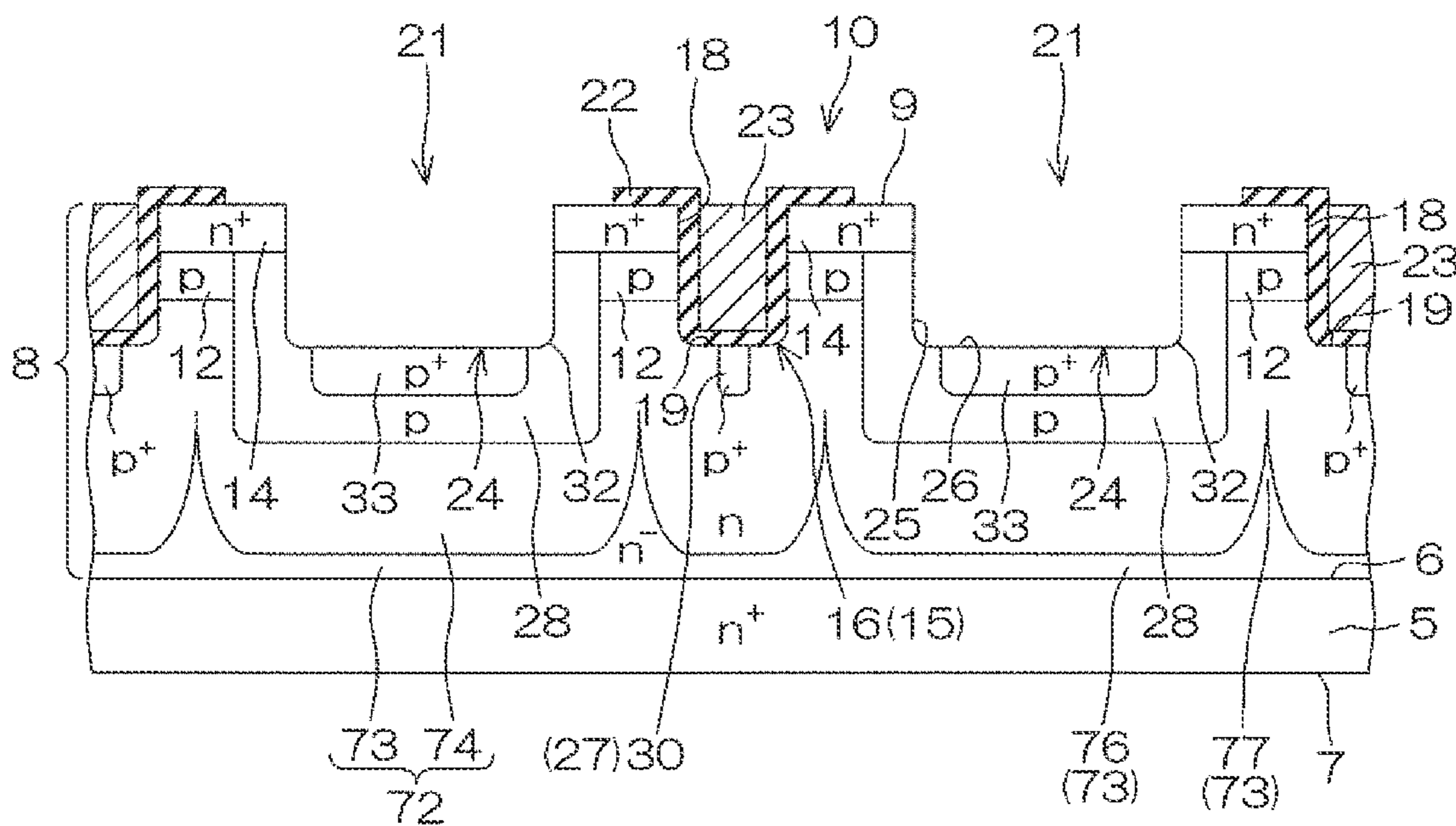
B-B SECTION
