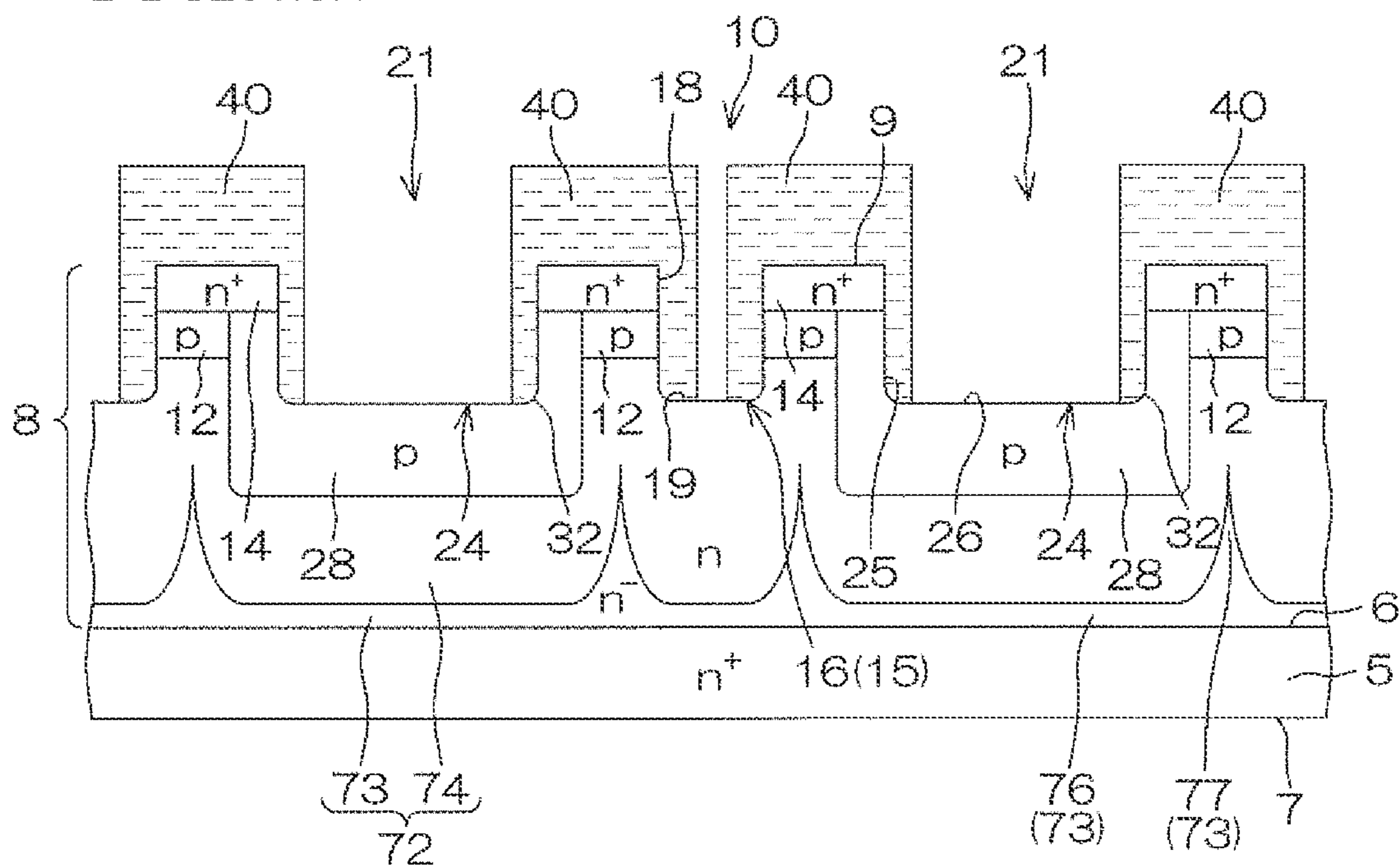
B-B SECTION
