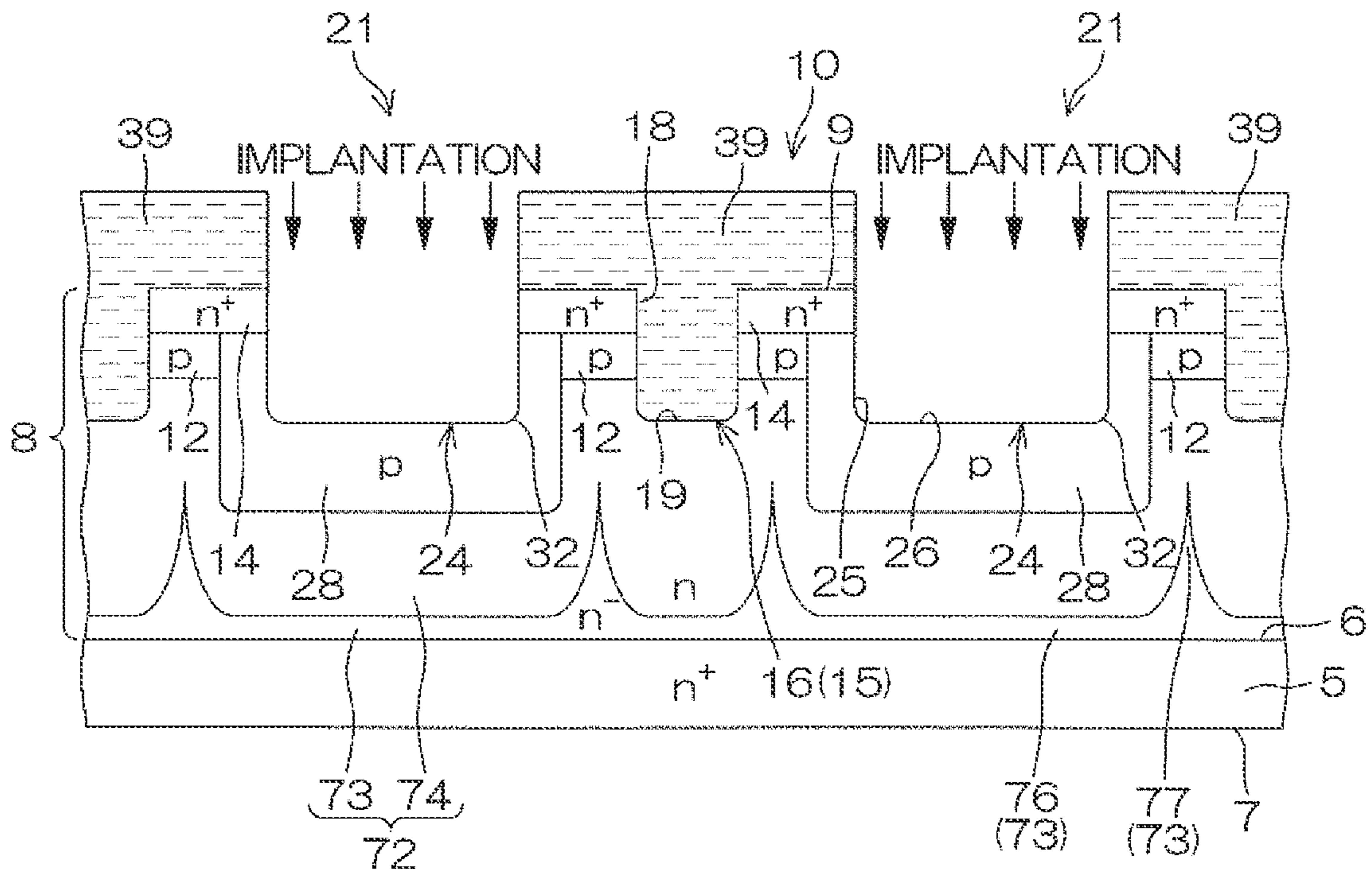
B-B SECTION
