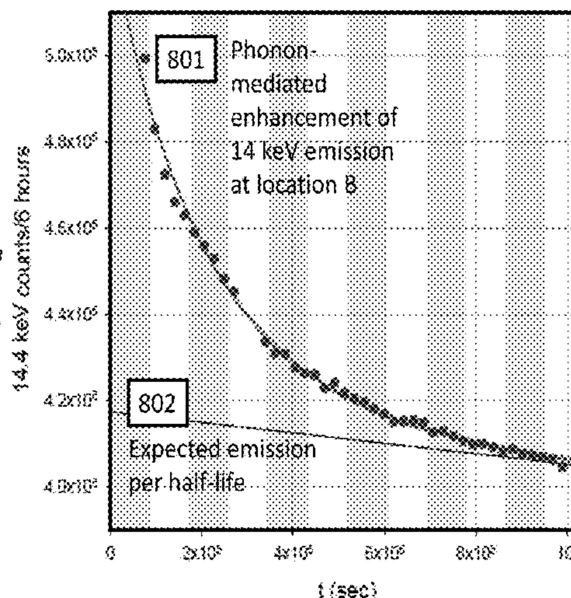
X123 Gamma spectrometer at Location B; during operation
