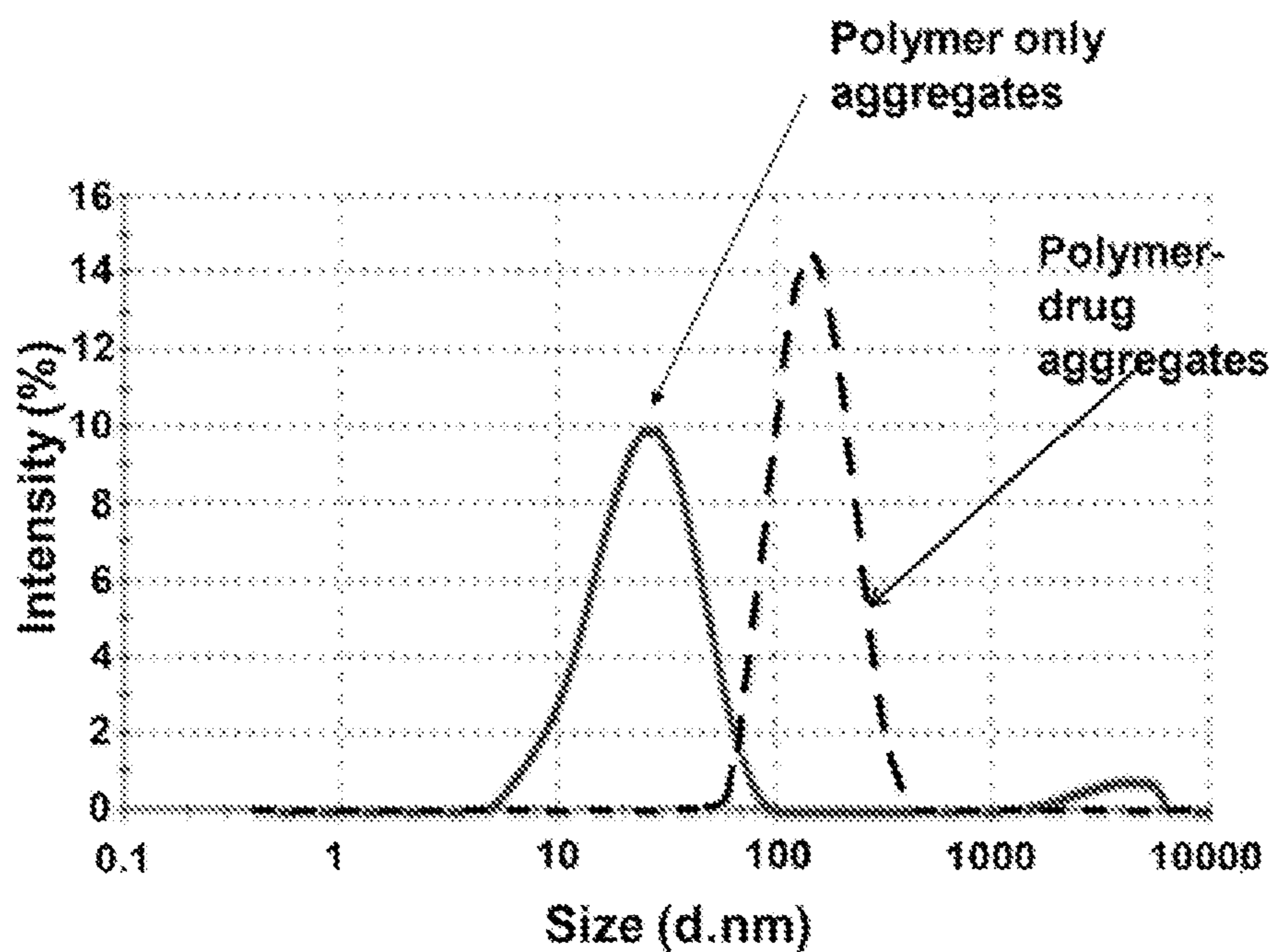
Polymer and polymer-drug aggregates with the polymer concentration at 25 mg/mL in saline
