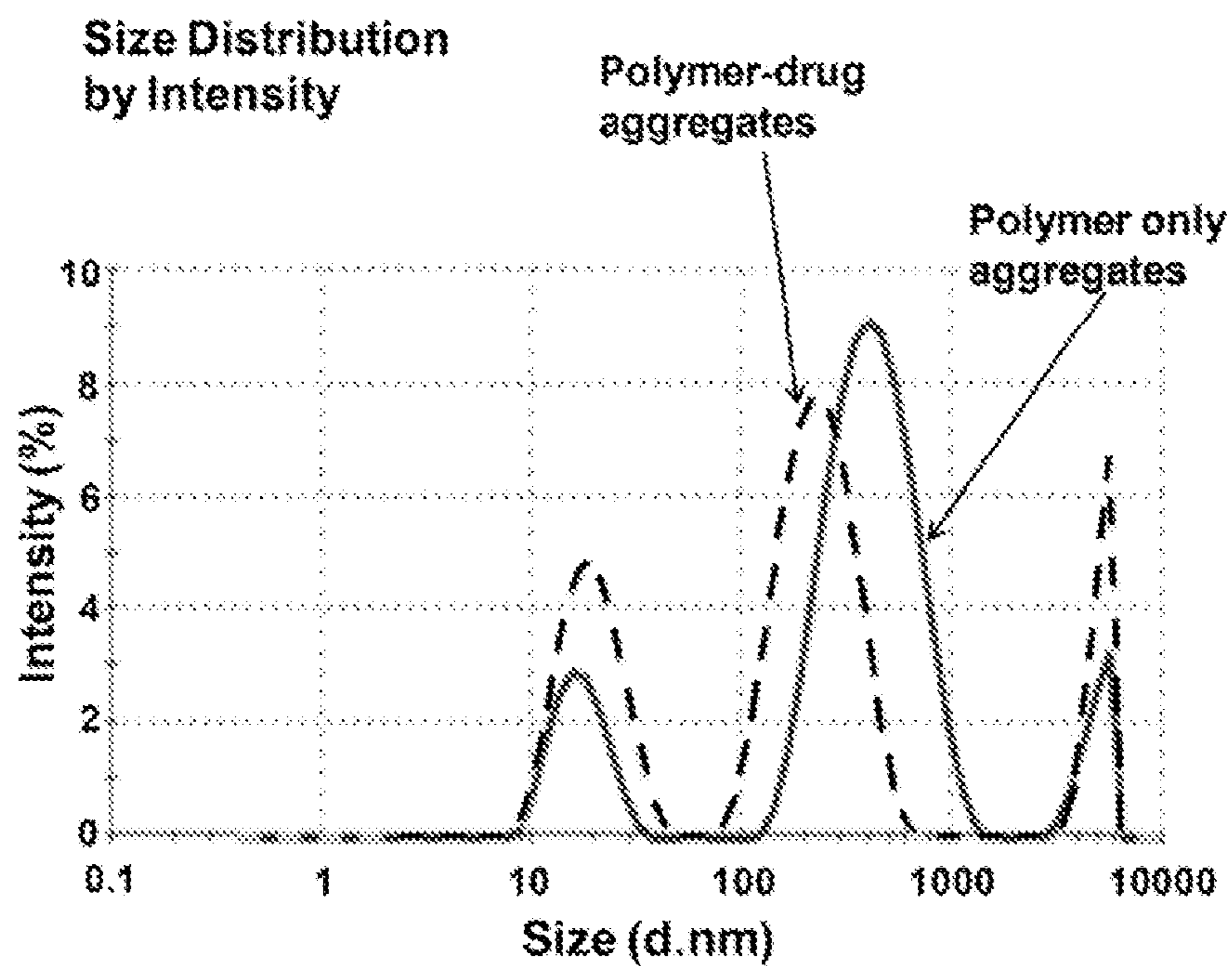
Polymer and Polymer-Drug Aggregates at 25 \mu\text{g}/\text{mL} in Saline
