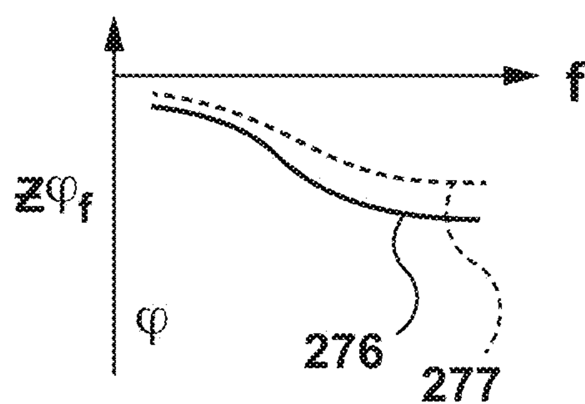
Frequency profile of Z_{\phi_f} during safe state
