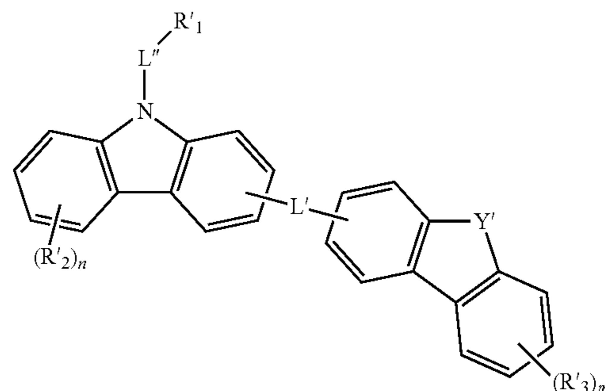
[Chemical Formula 2]
