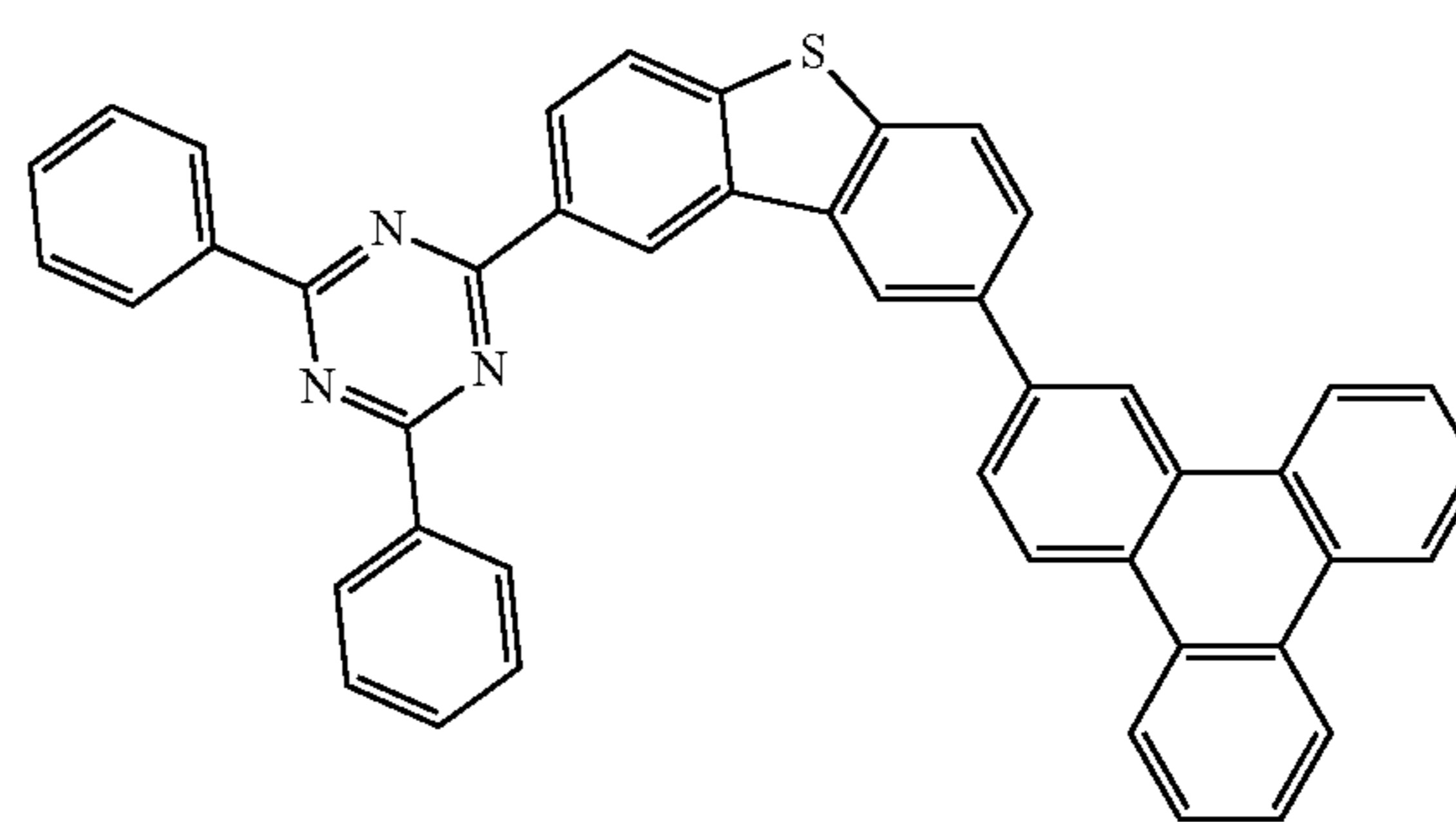
Compound A
