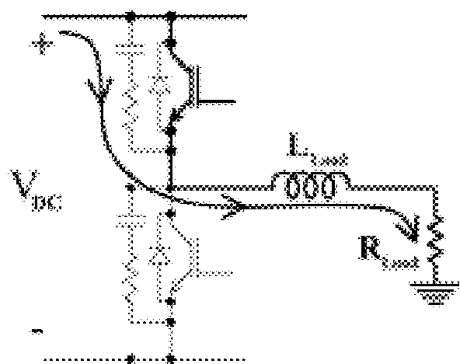
FIG. 3c (Prior art)
