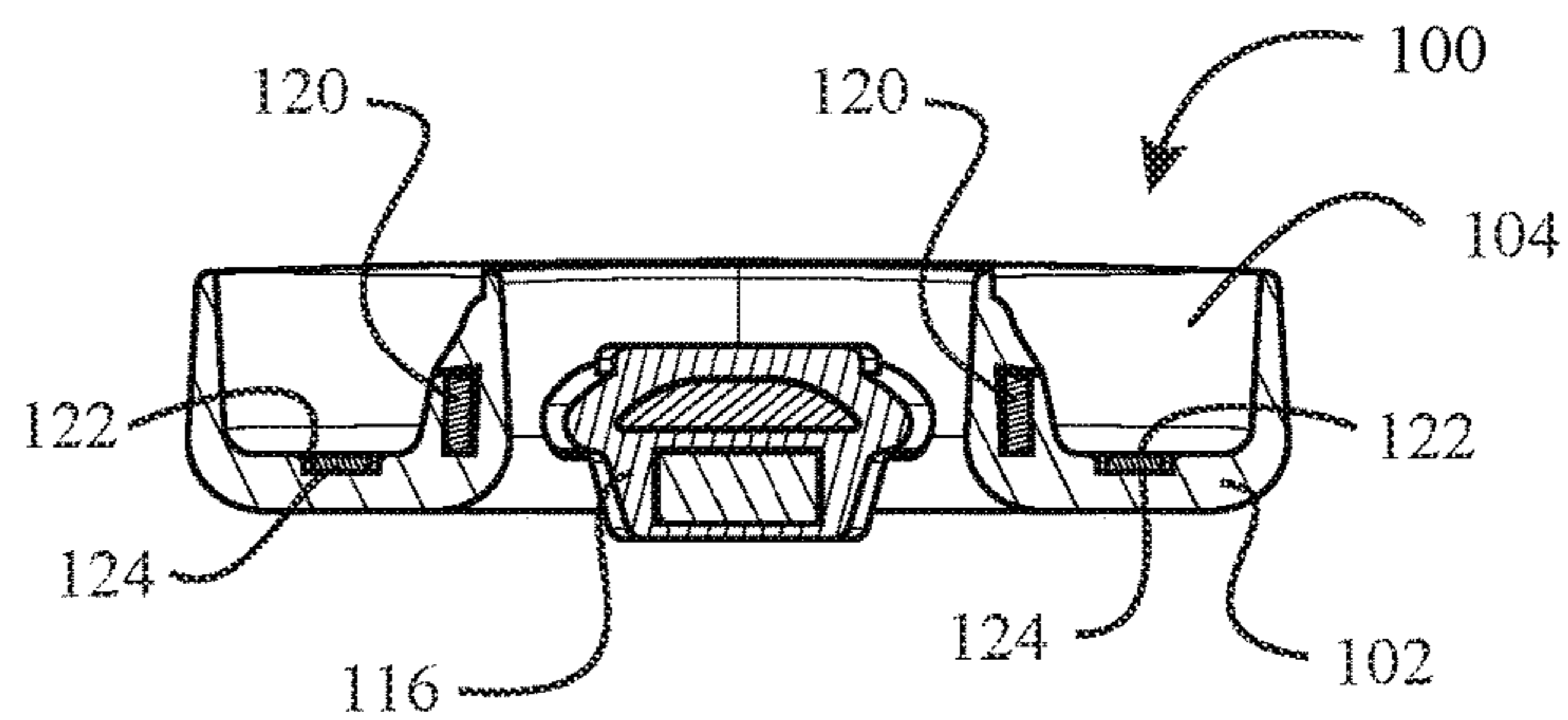
SECTION C-C
