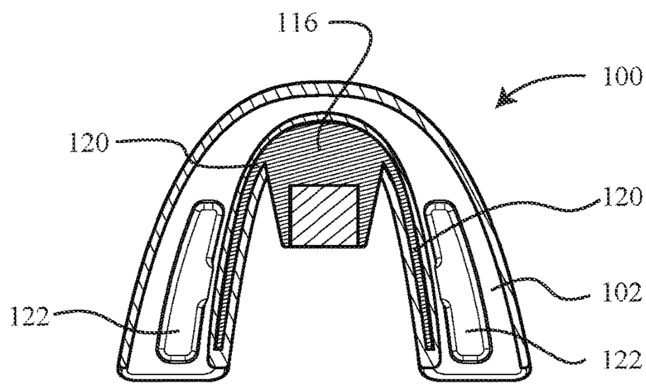
SECTION B-B
