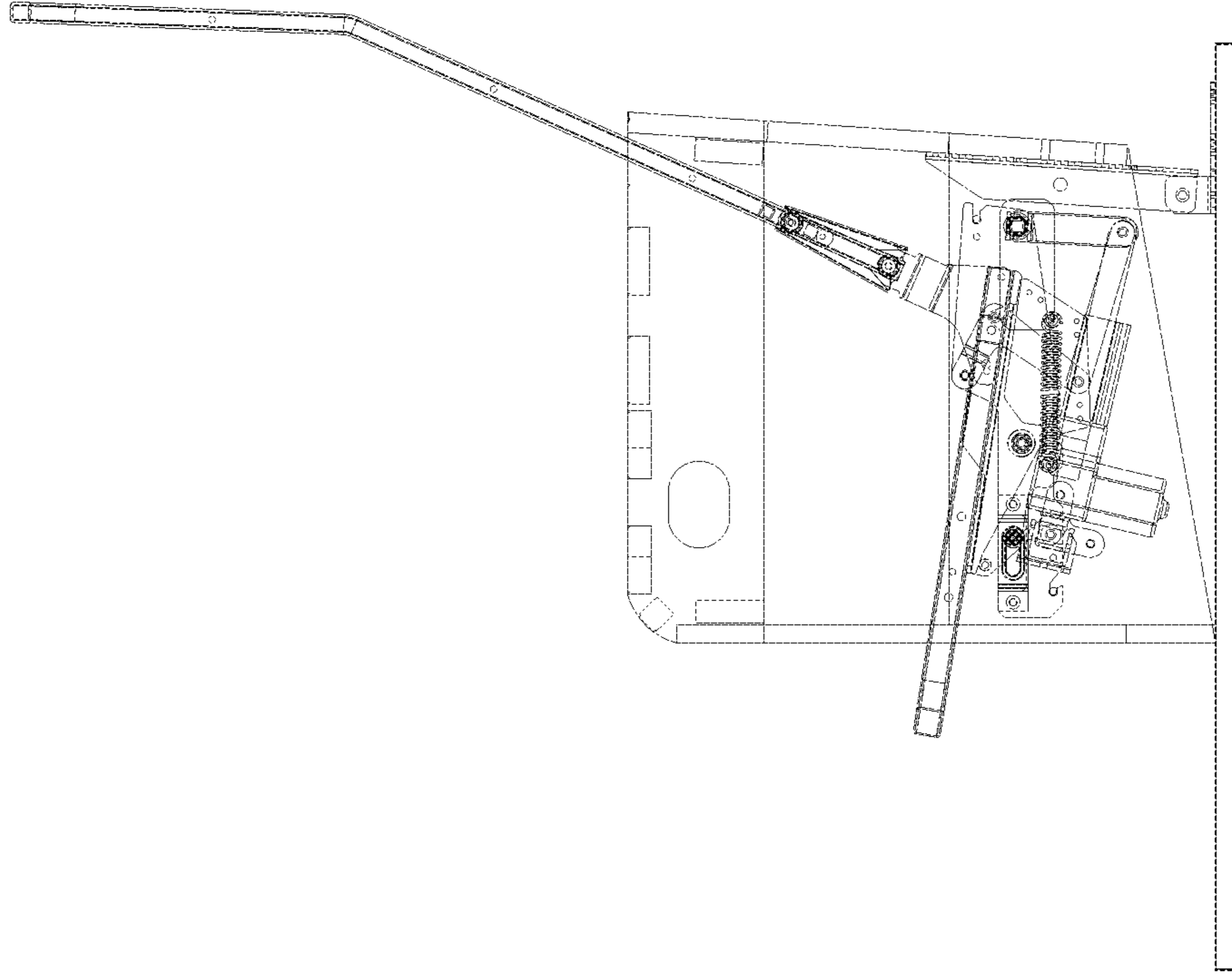
Closed and Upright Position (Occupied)--Side View
