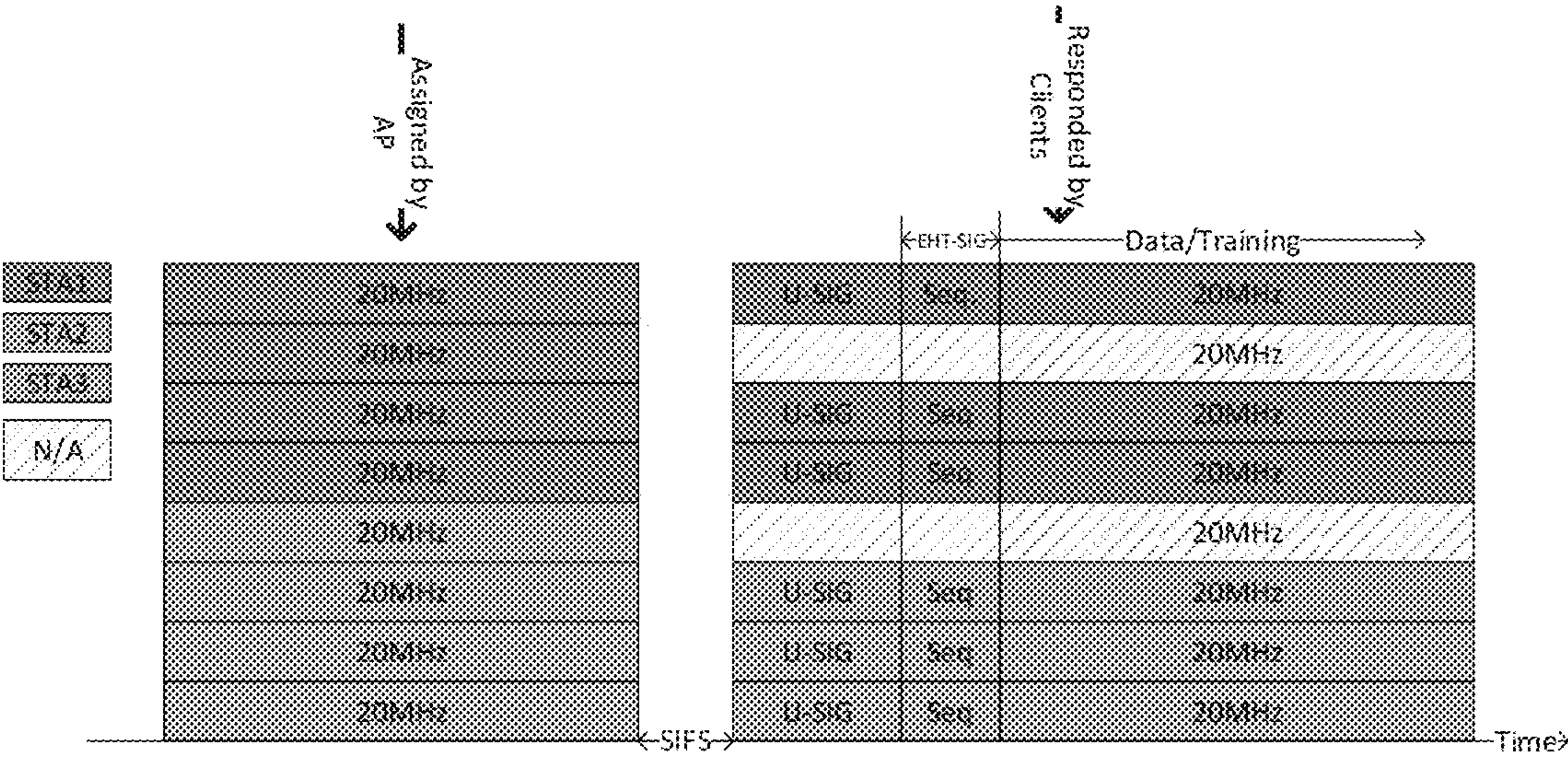
FIG. 3 - Channel availability information in EHT-SIG
