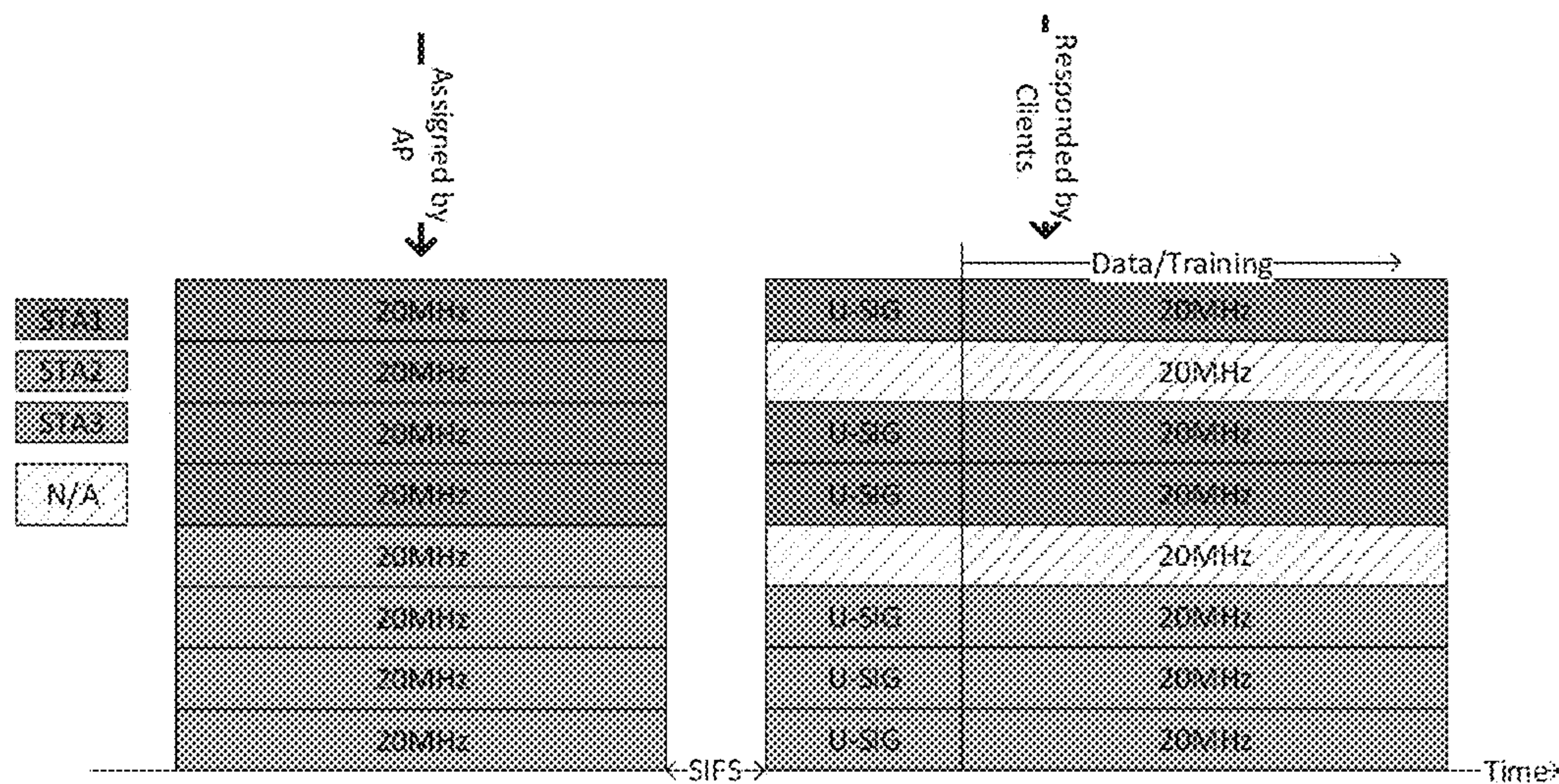
FIG 2 - Channel availability information in U-SIG
