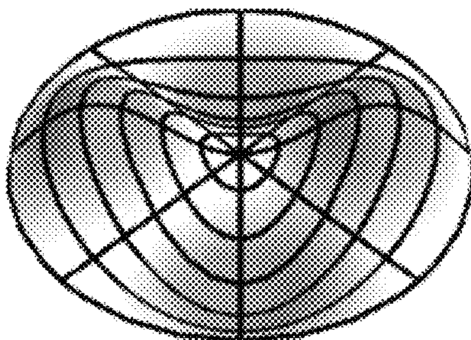
mode (2,1)
