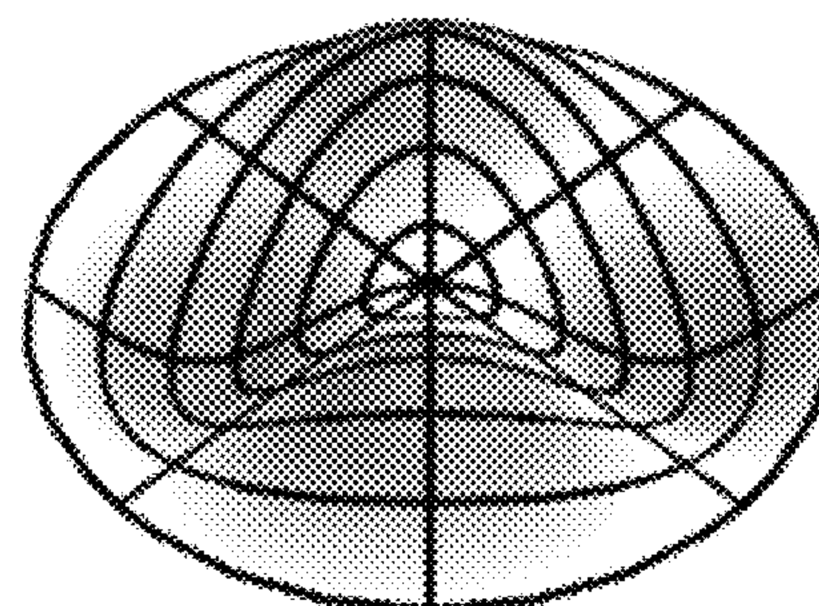
mode (2,1)
