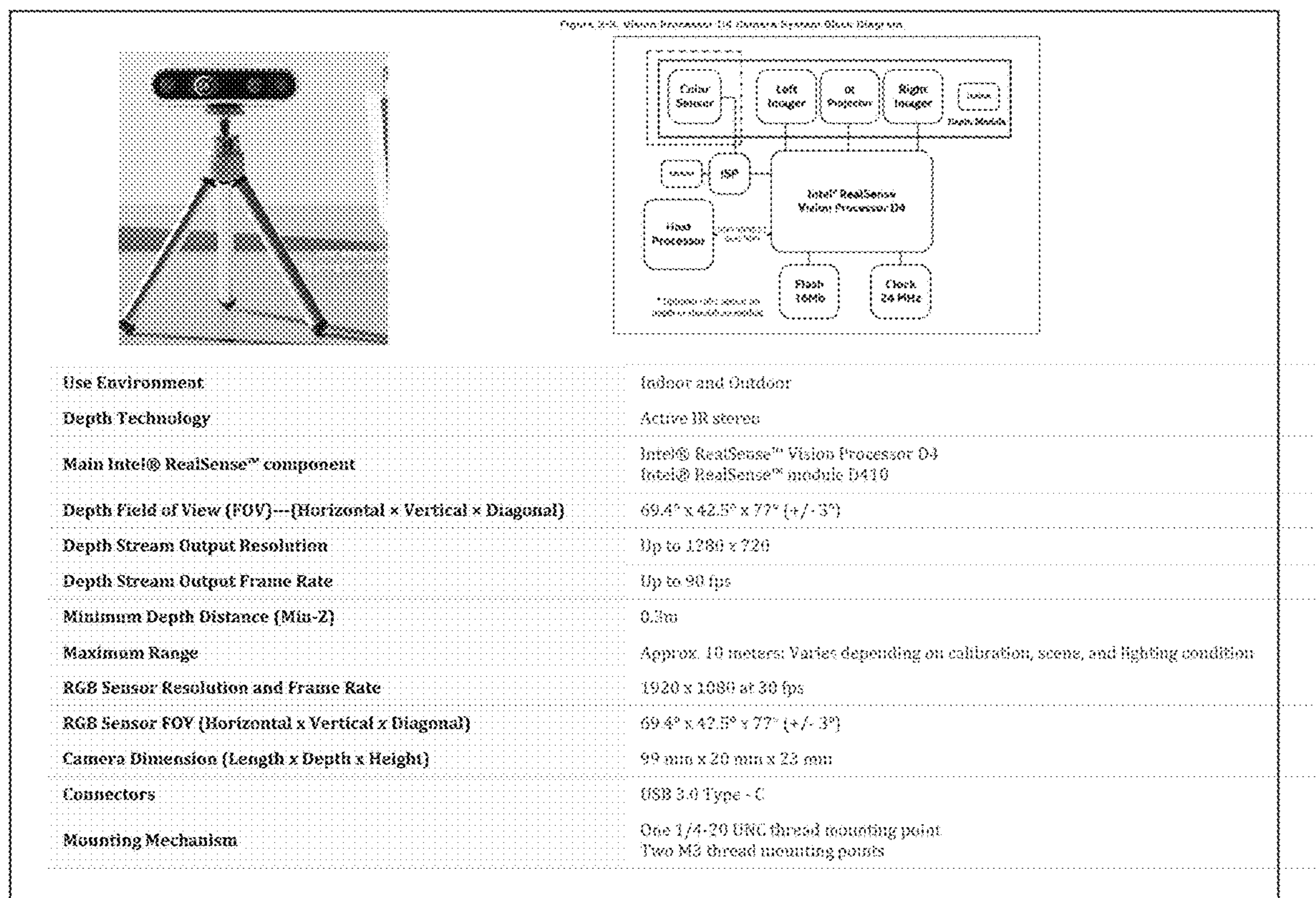
FIG. 10 (camera with depth sensing)
