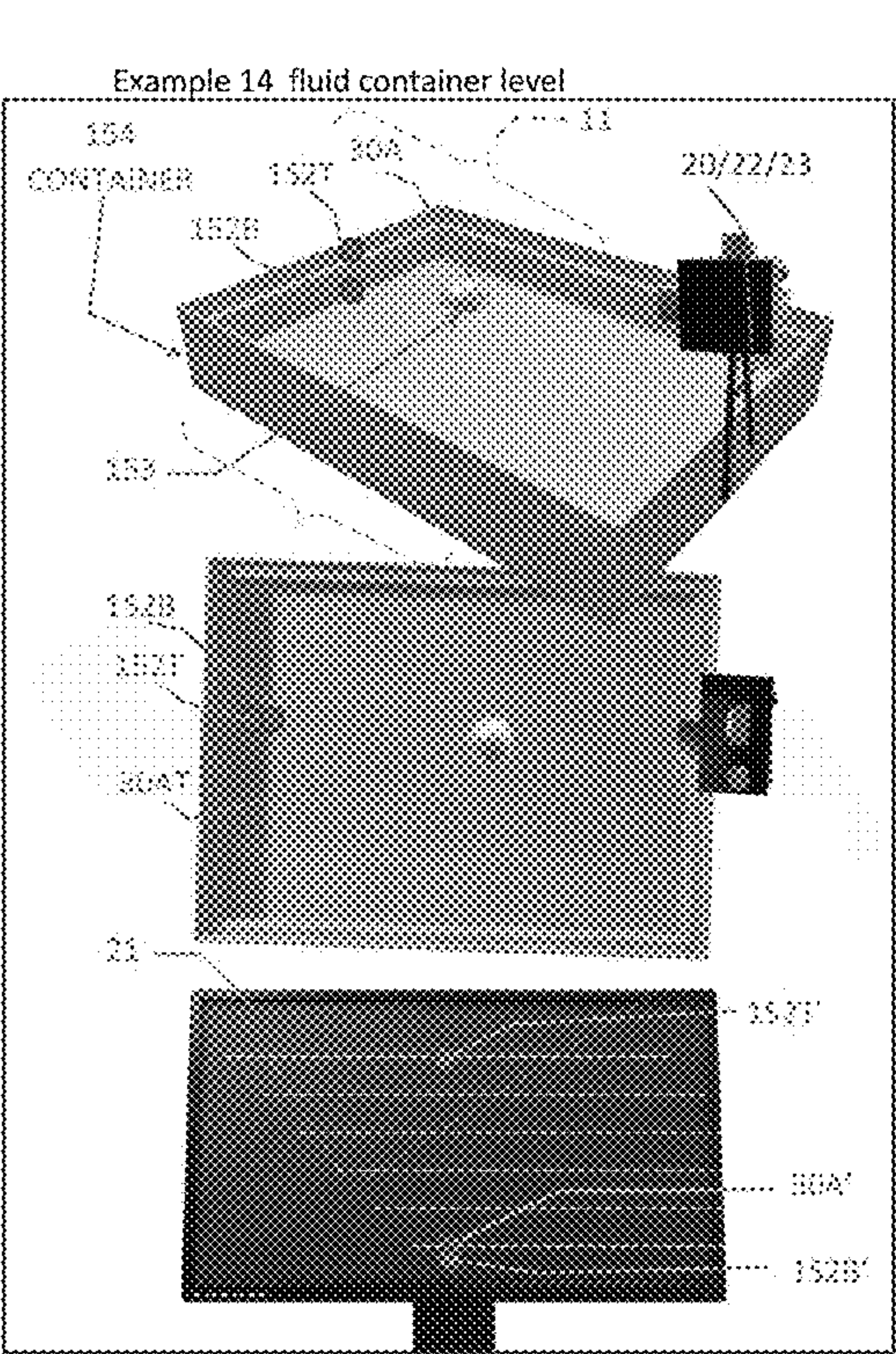
FIG. 34A (empty fluid container)
