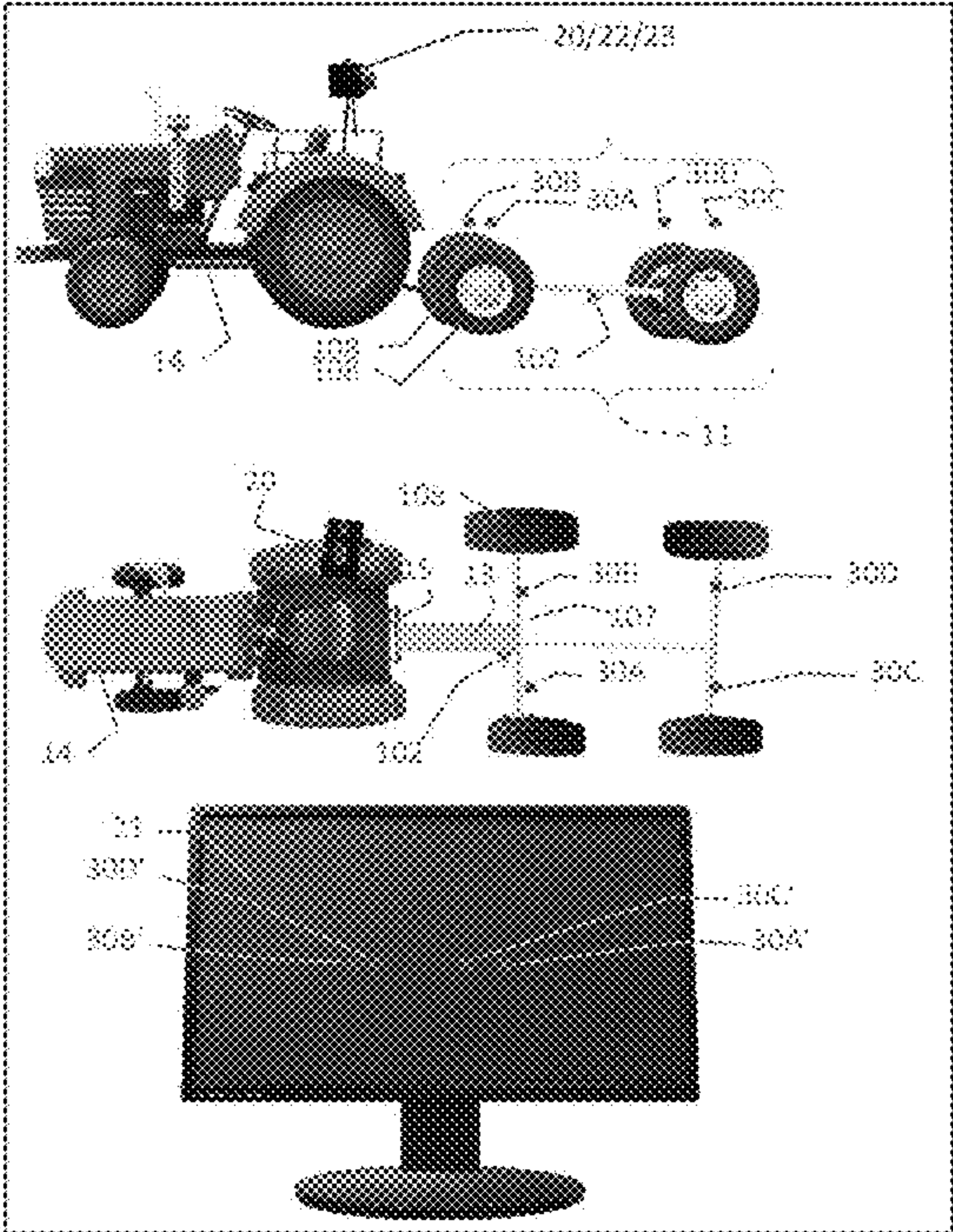
FIG. 28A (four-wheeled trailer aligned with tractor)
