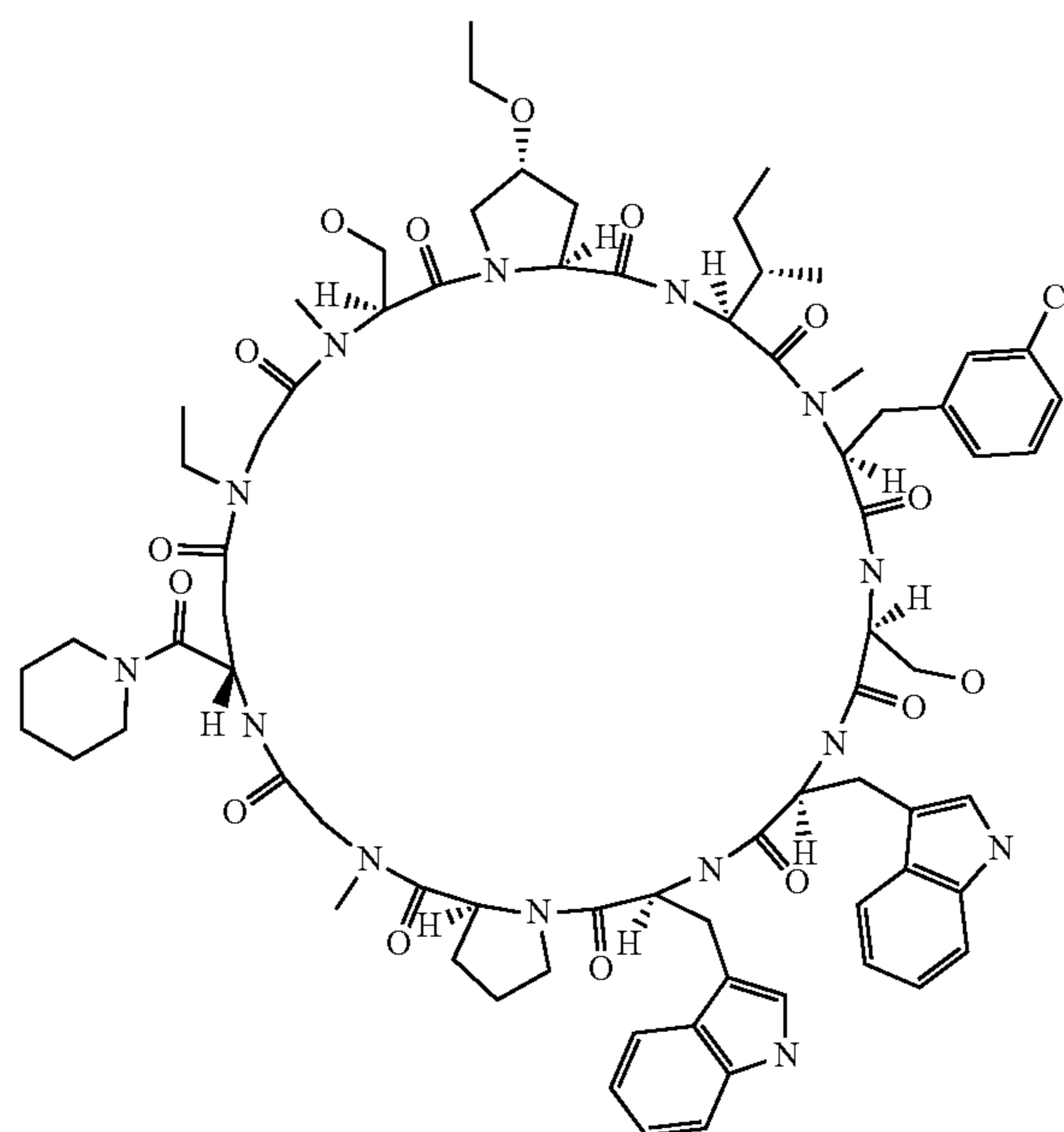
Compound 133
