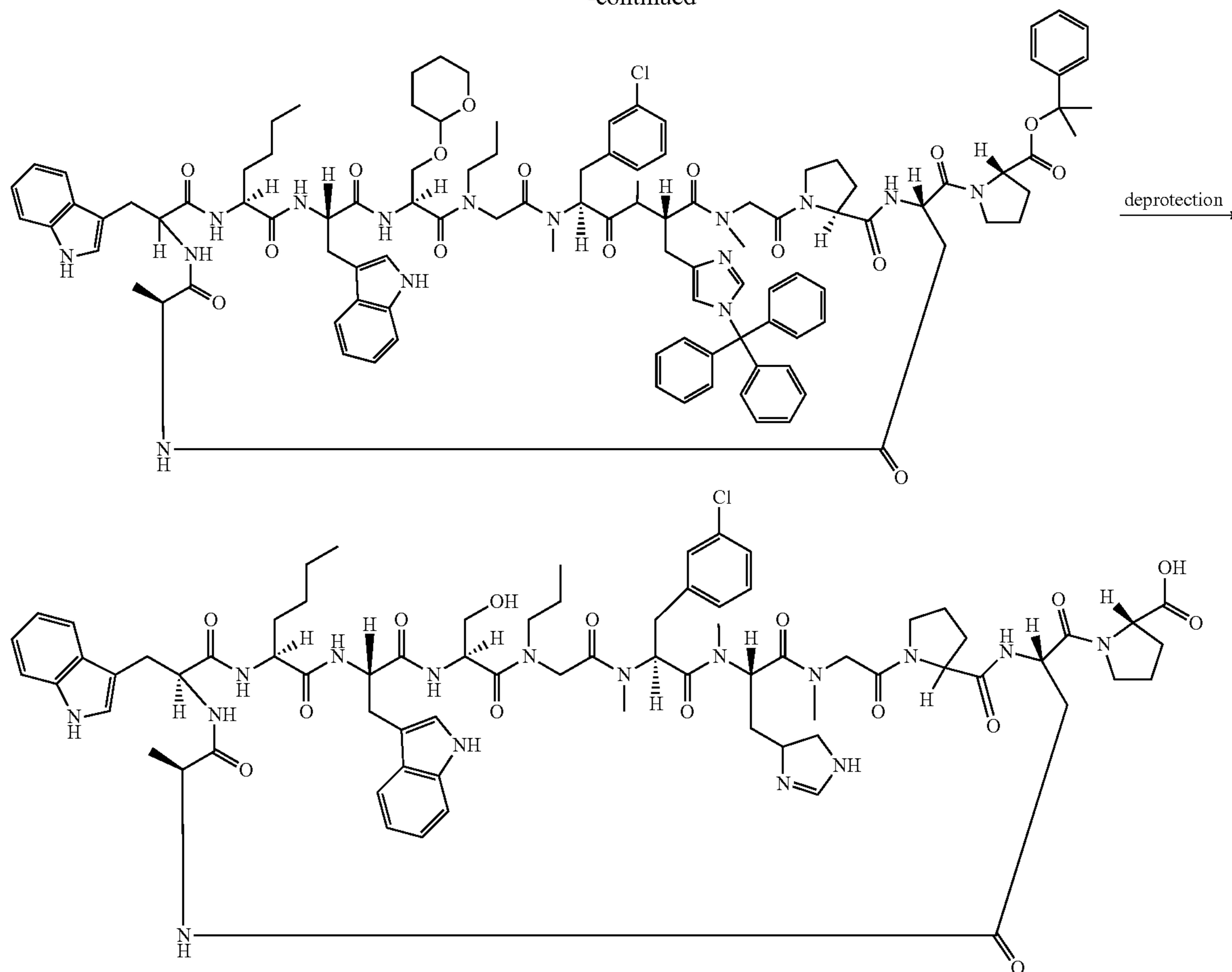
Compound 154
