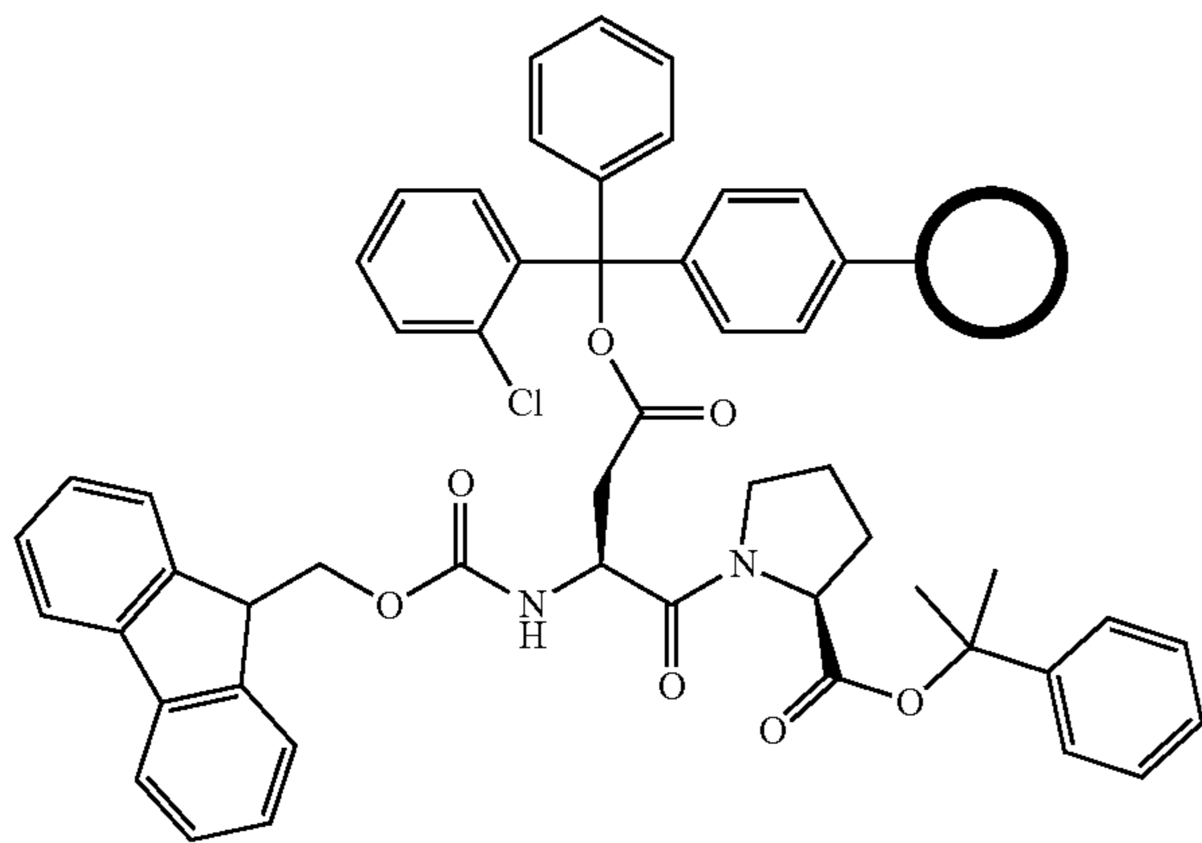
Compound 58
