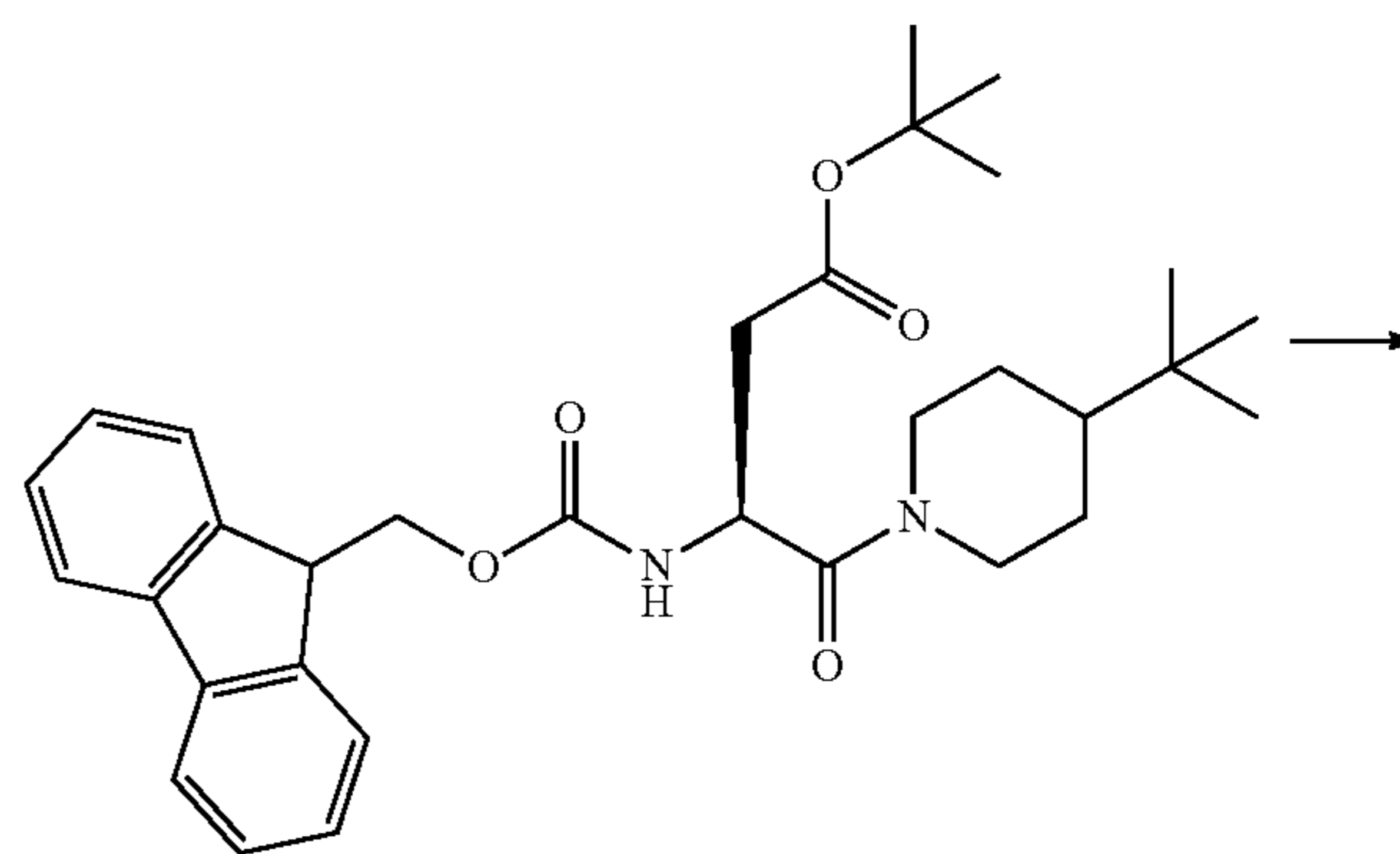
Compound 53
