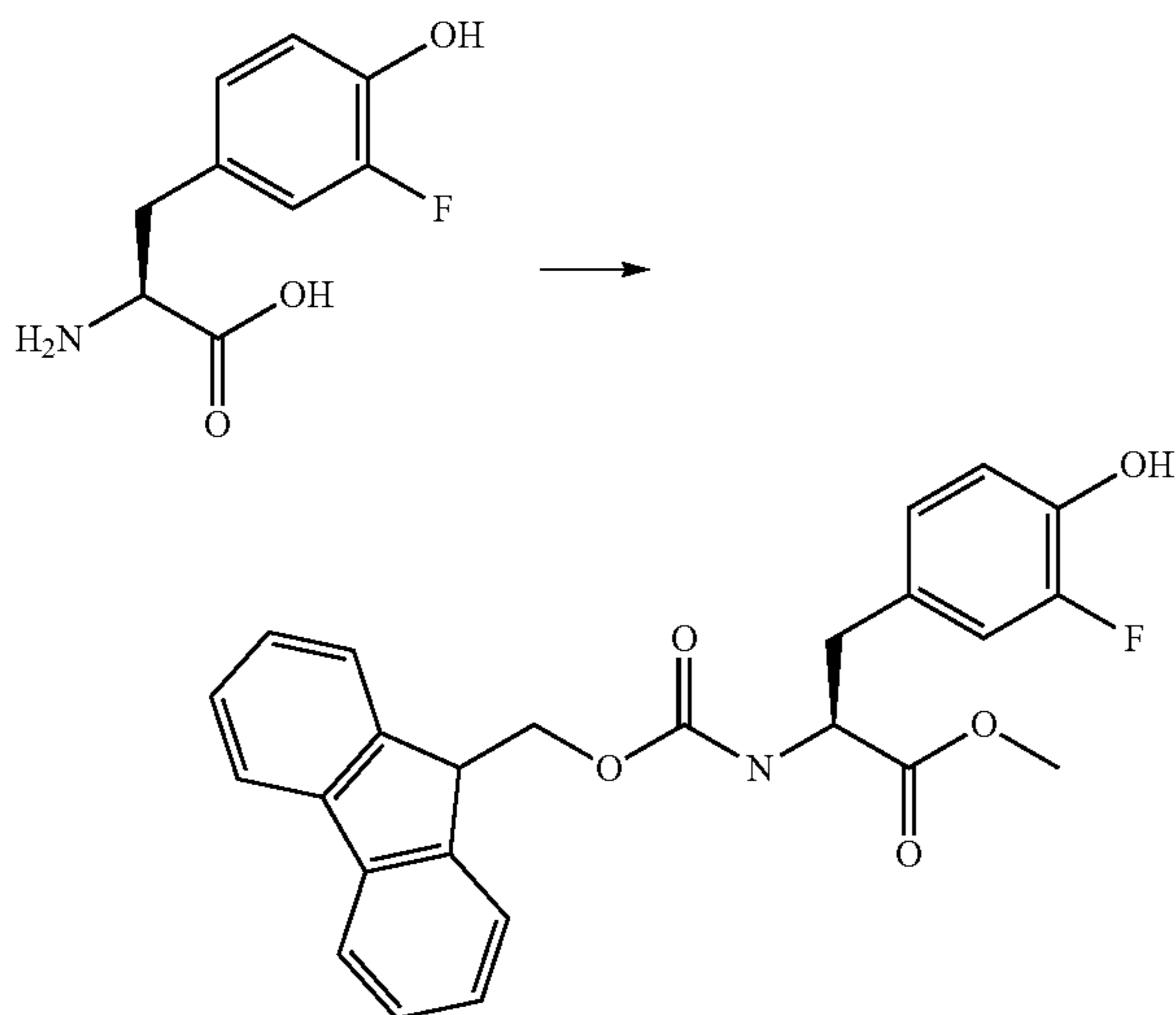
Compound 12
