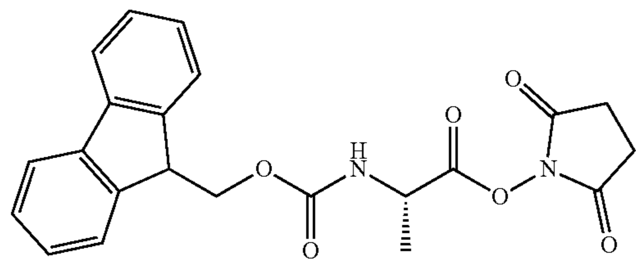
Compound 152
