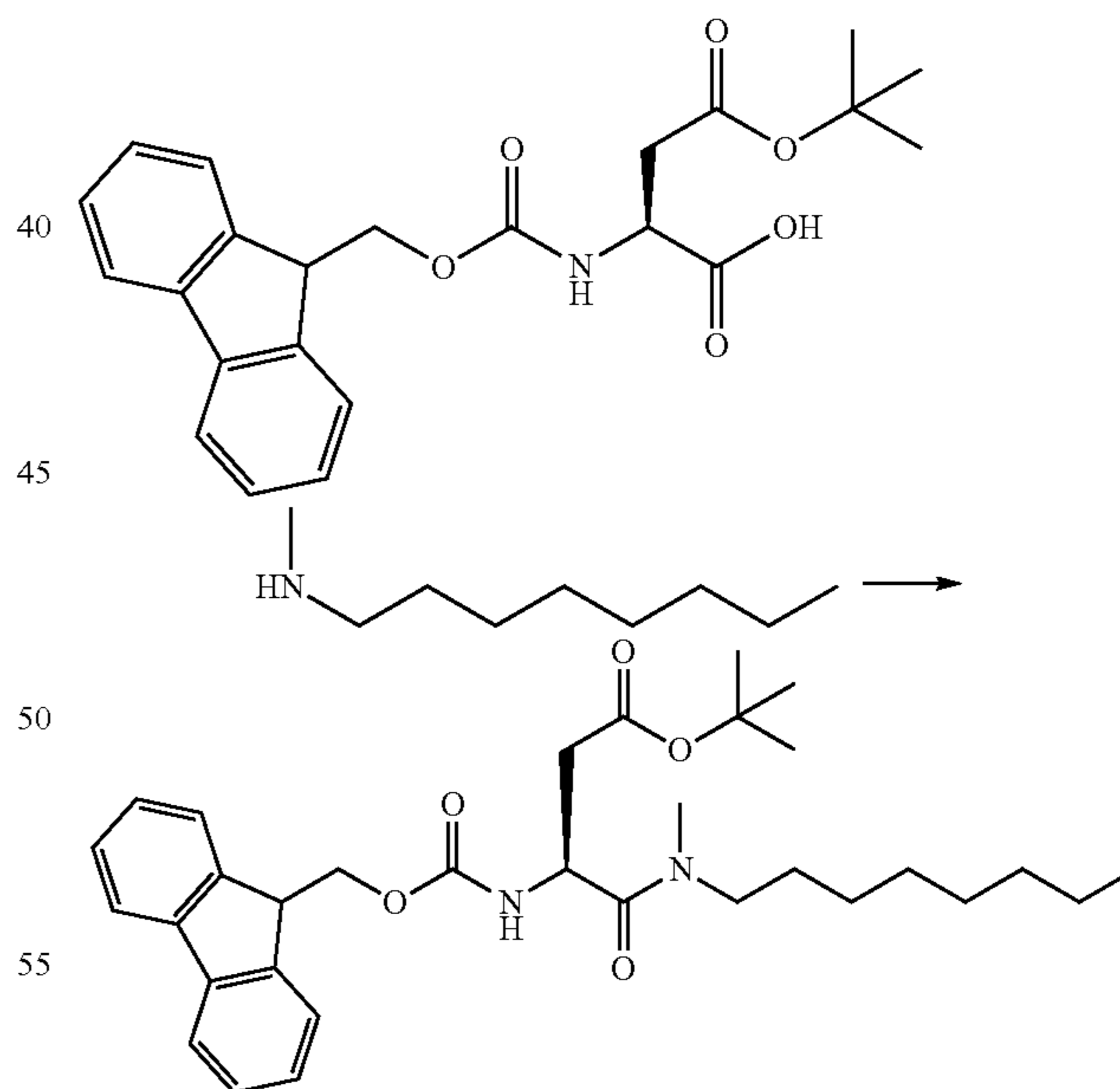
Compound 56
