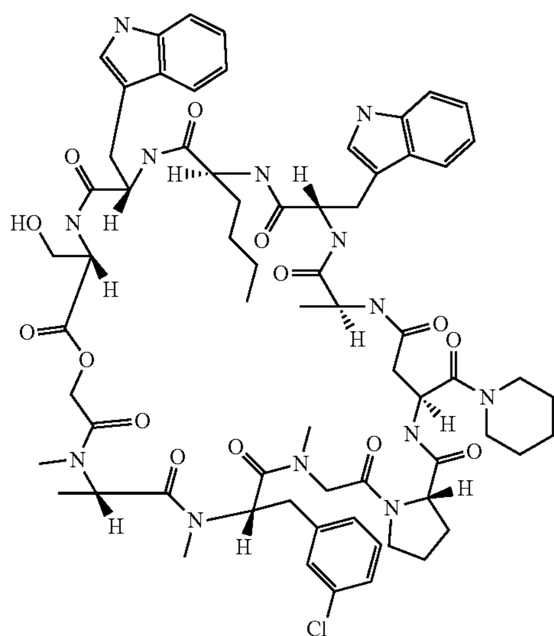
Compound 135
