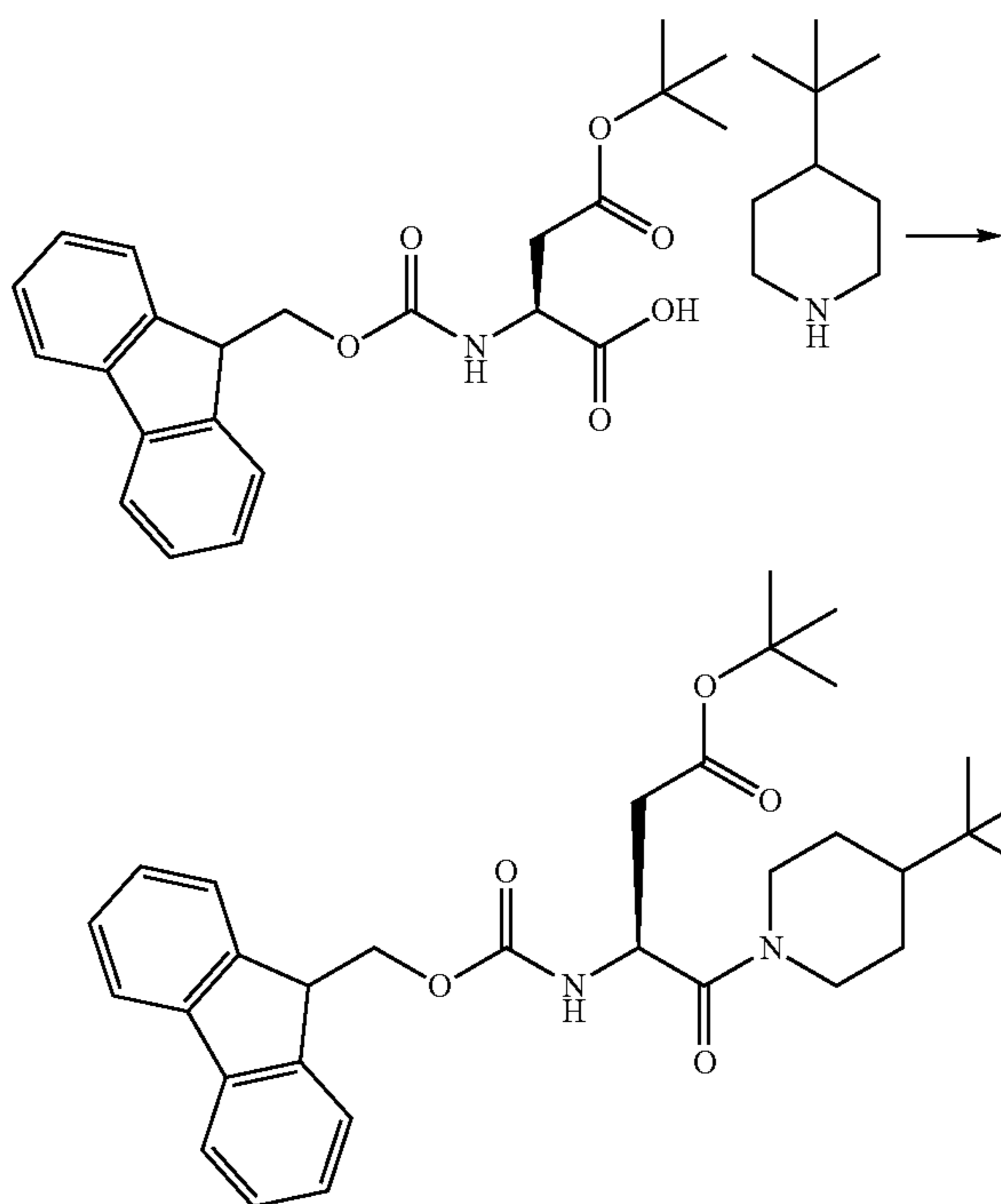
Compound 53
