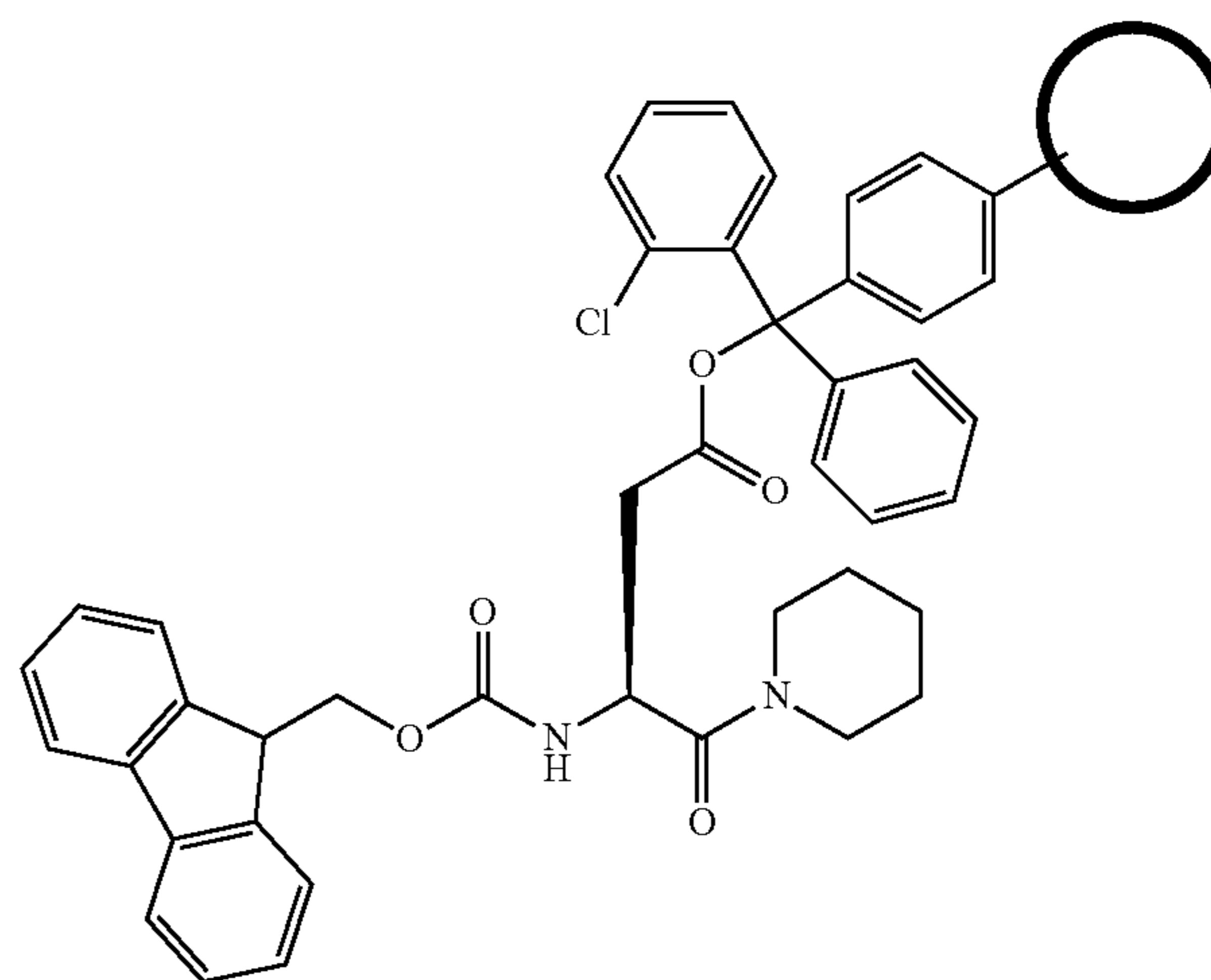
Compound 50
