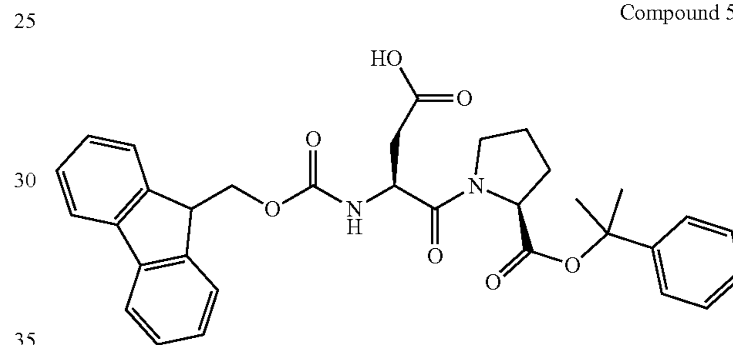
Compound 57
