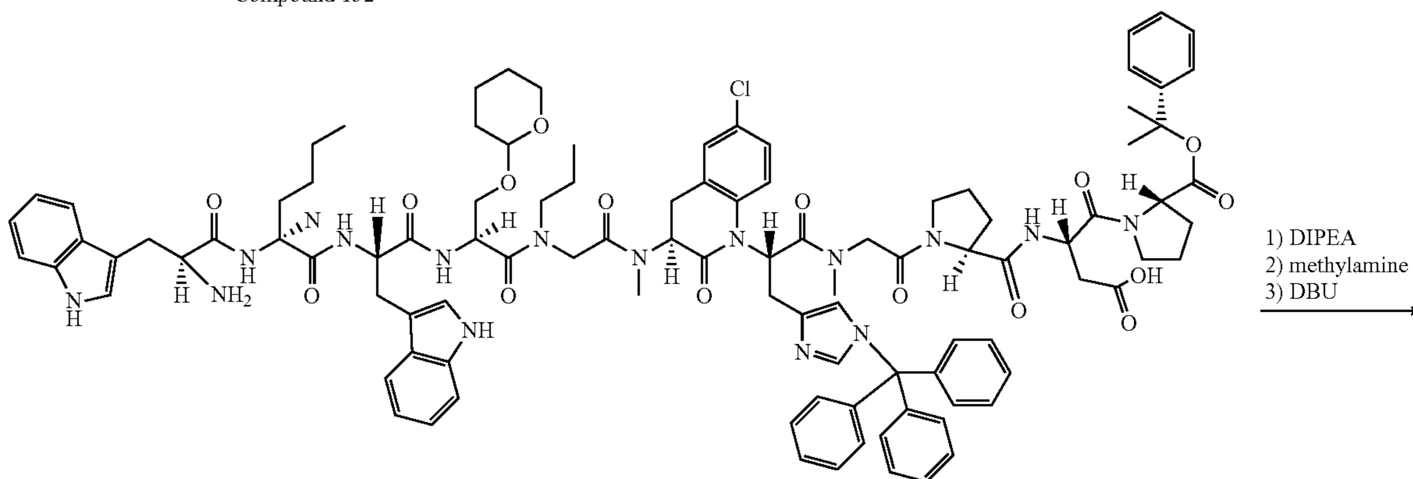
Compound 151
