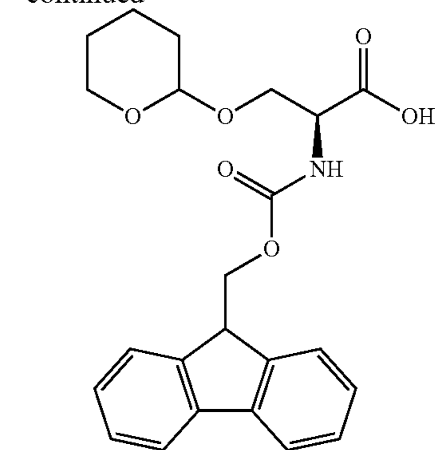
Compound 1
