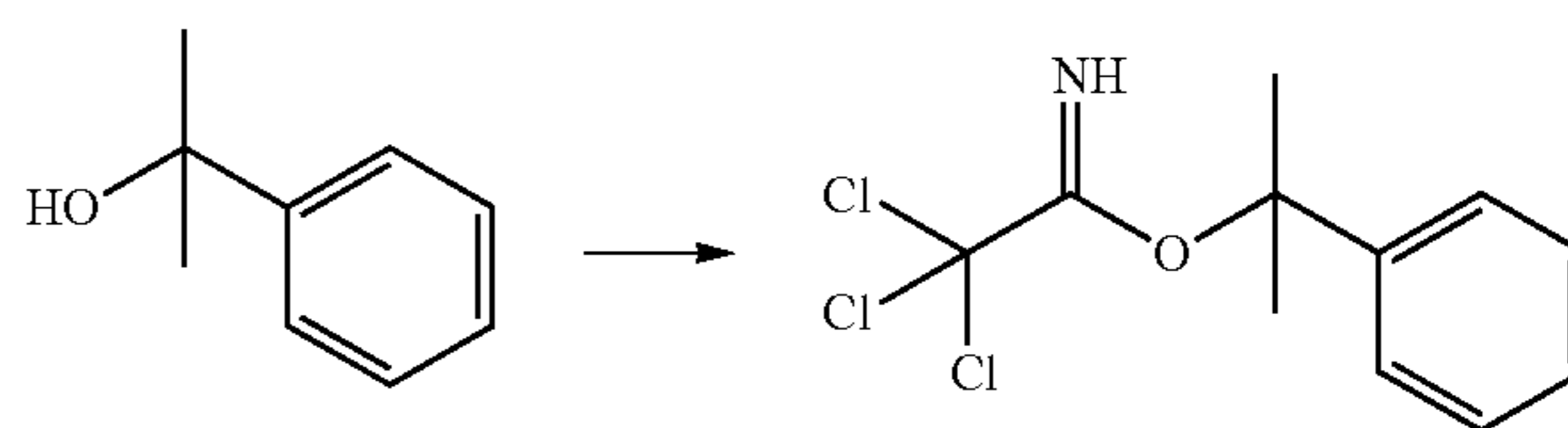
Compound 9
