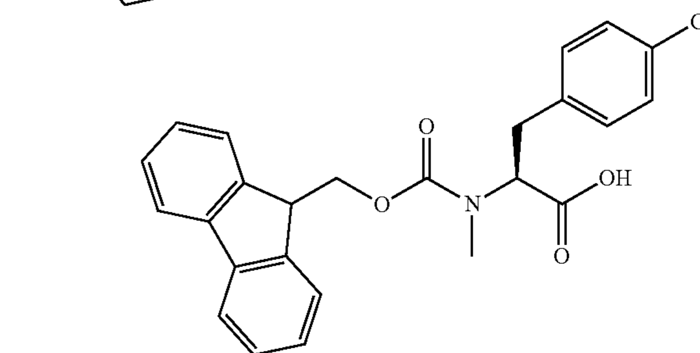
Compound 16
