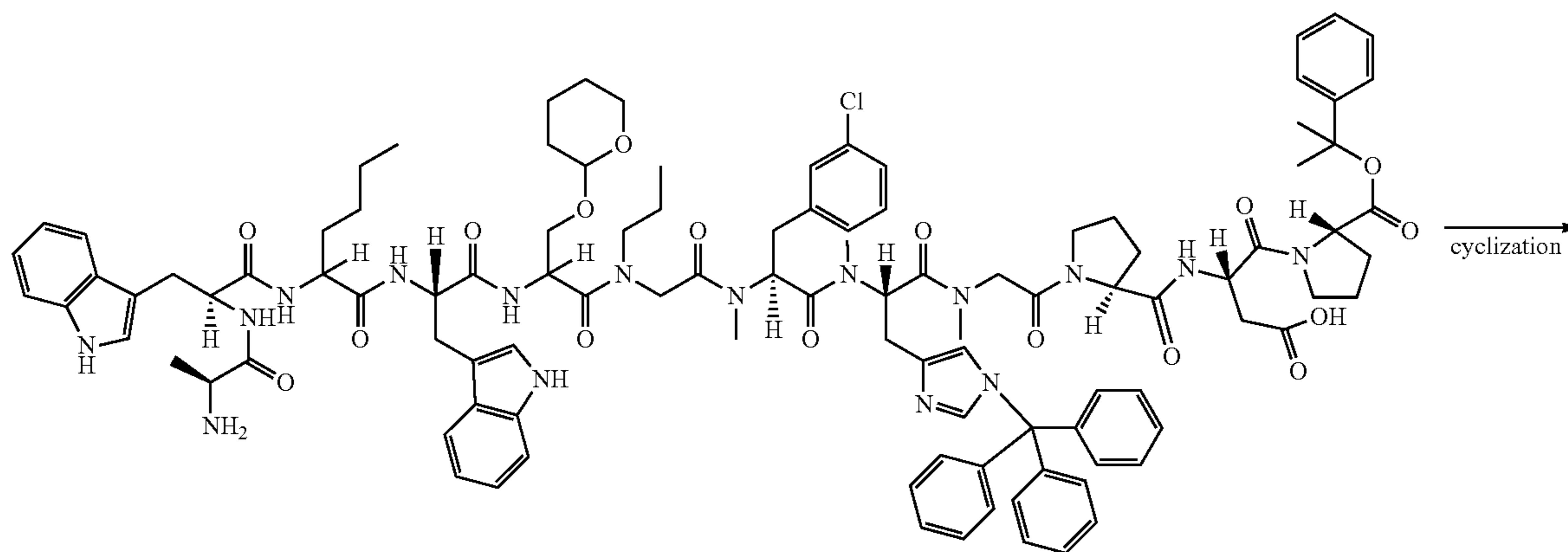
Compound 153
