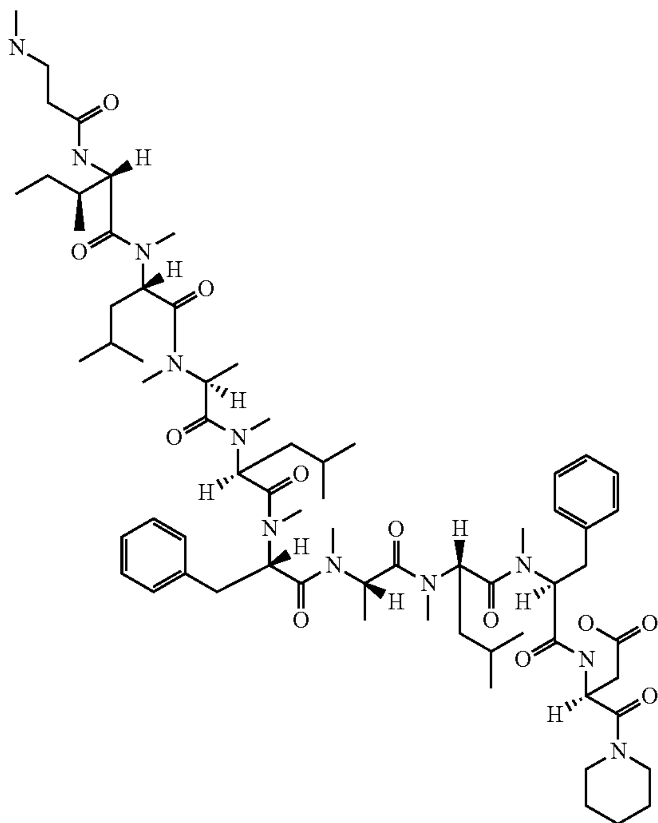
Compound 113
