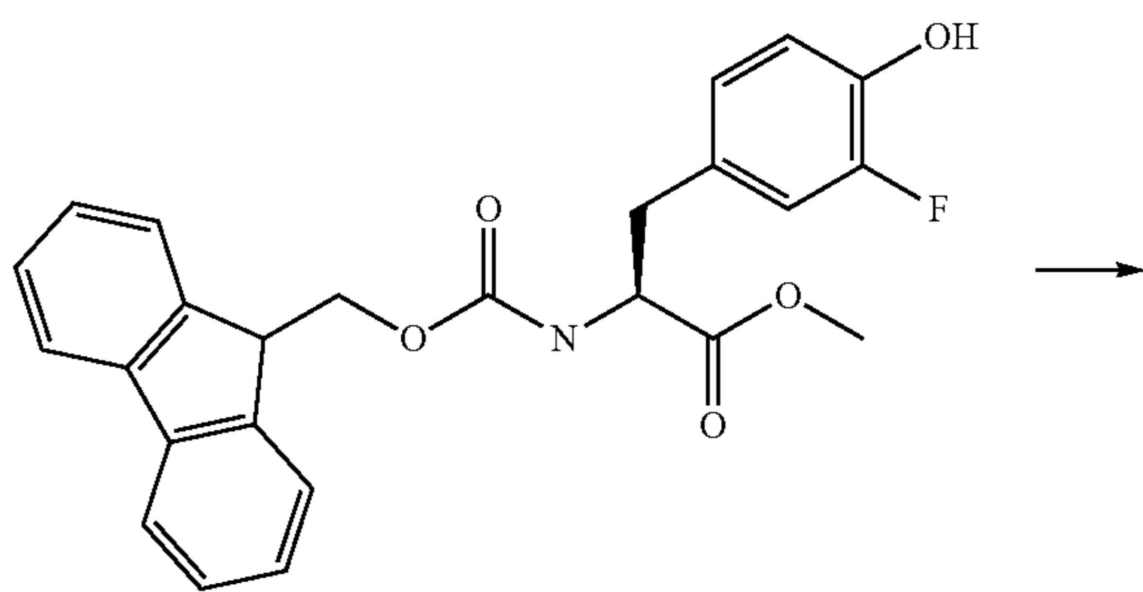
Compound 12
