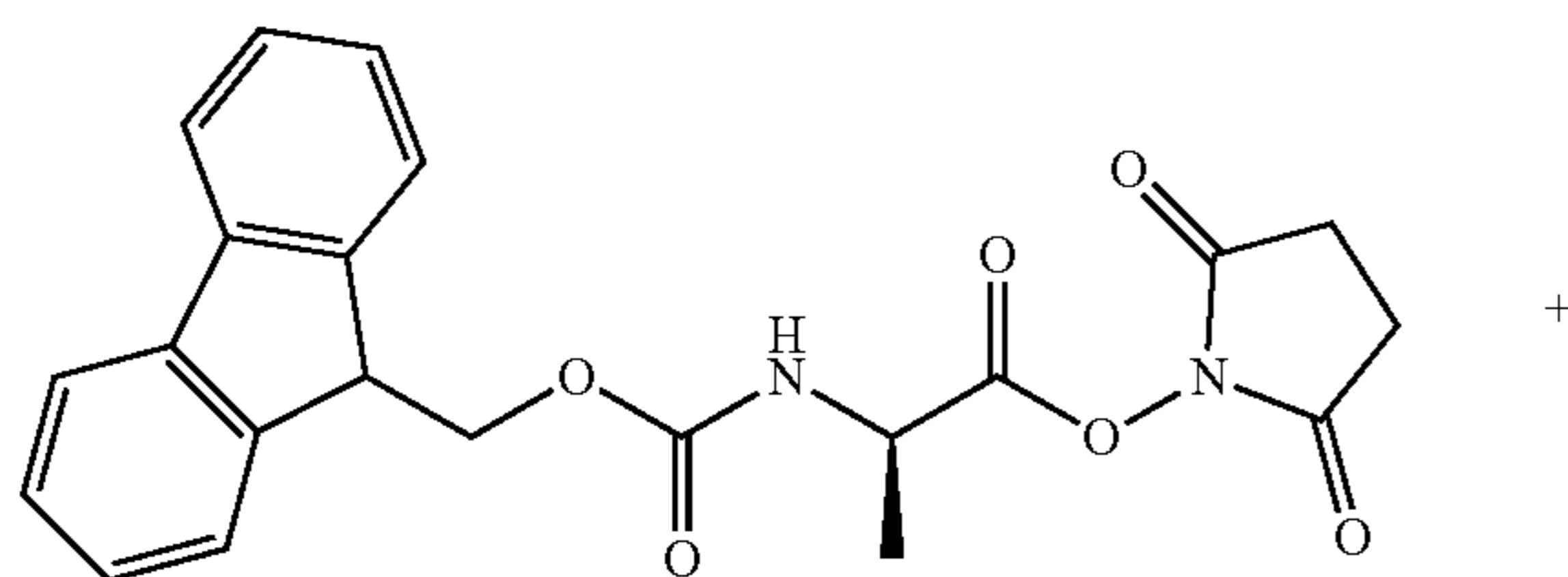
Compound 152
