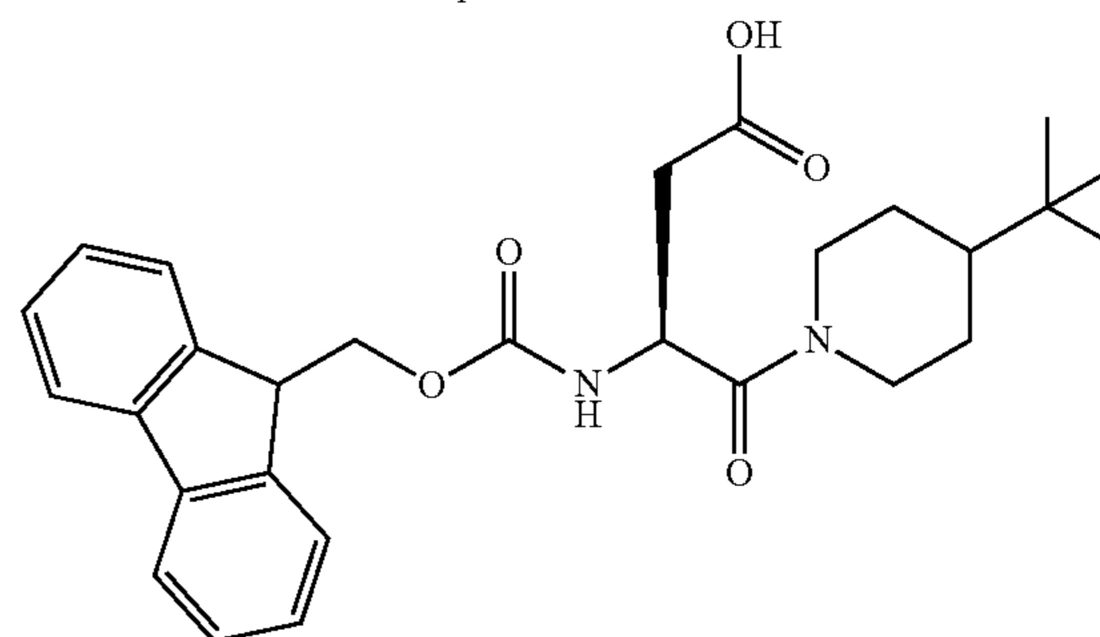
Compound 51
