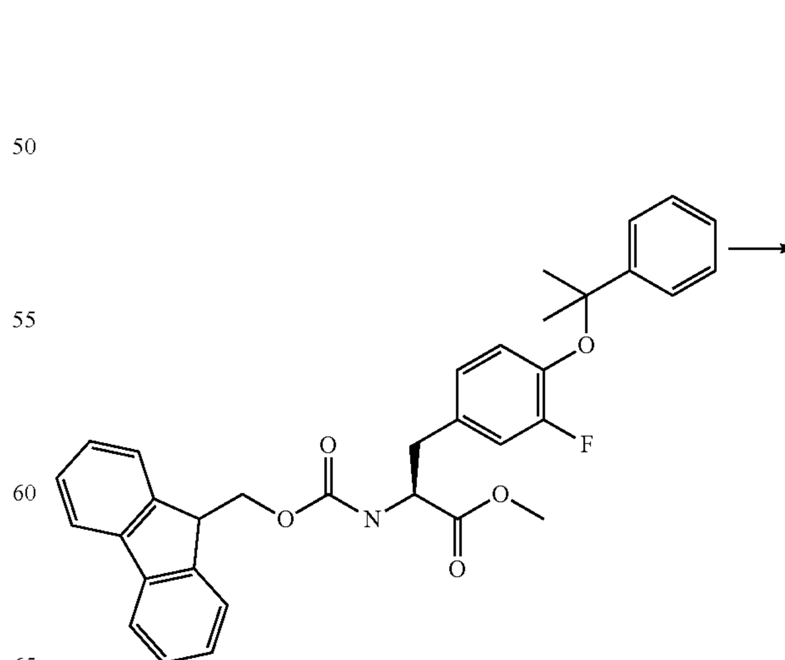
Compound 21
