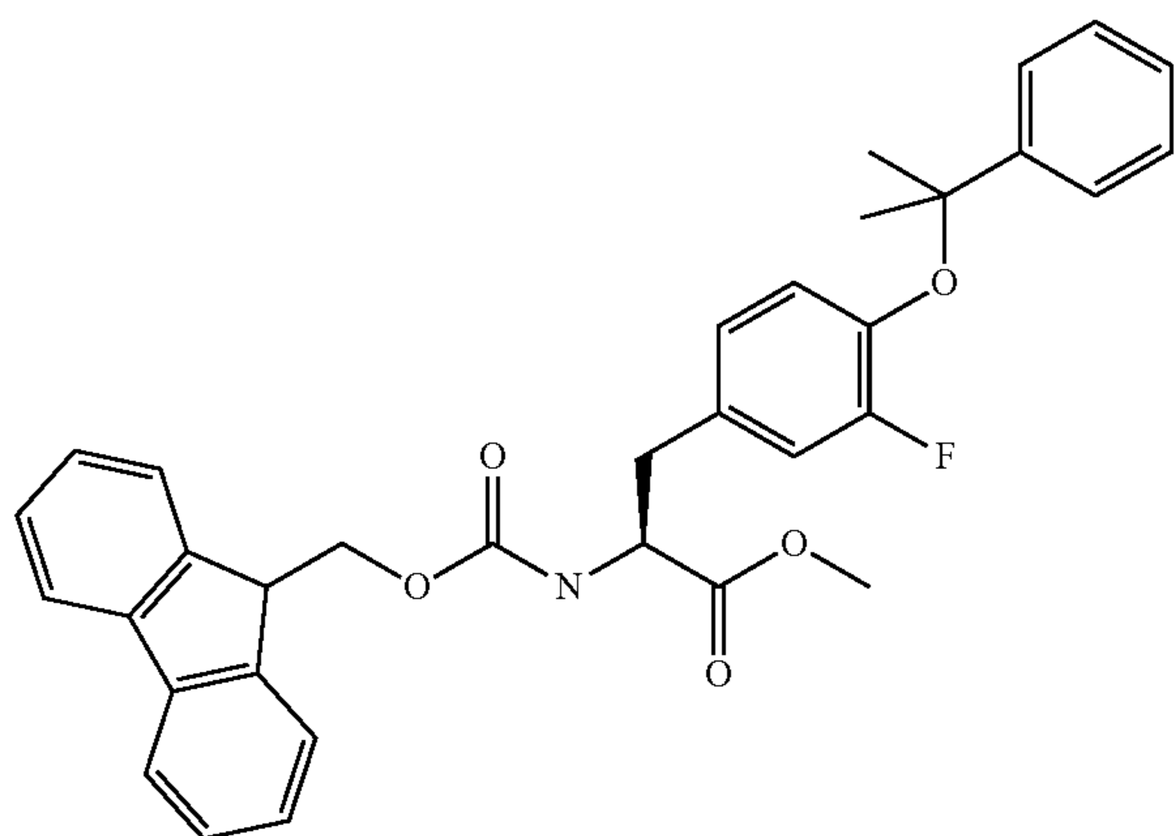
Compound 21
