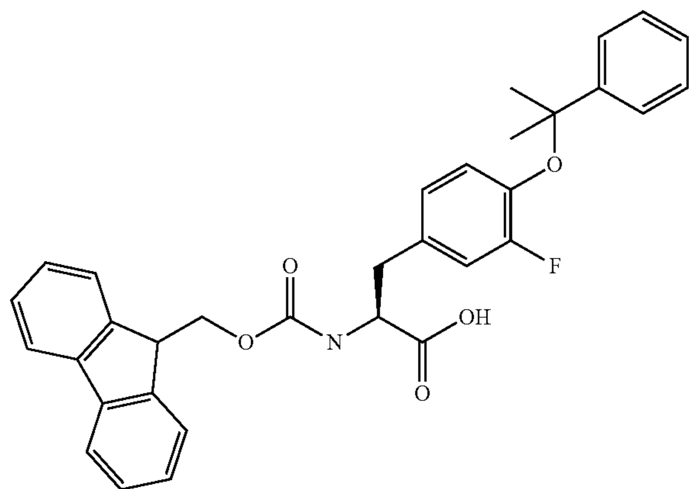
Compound 22
