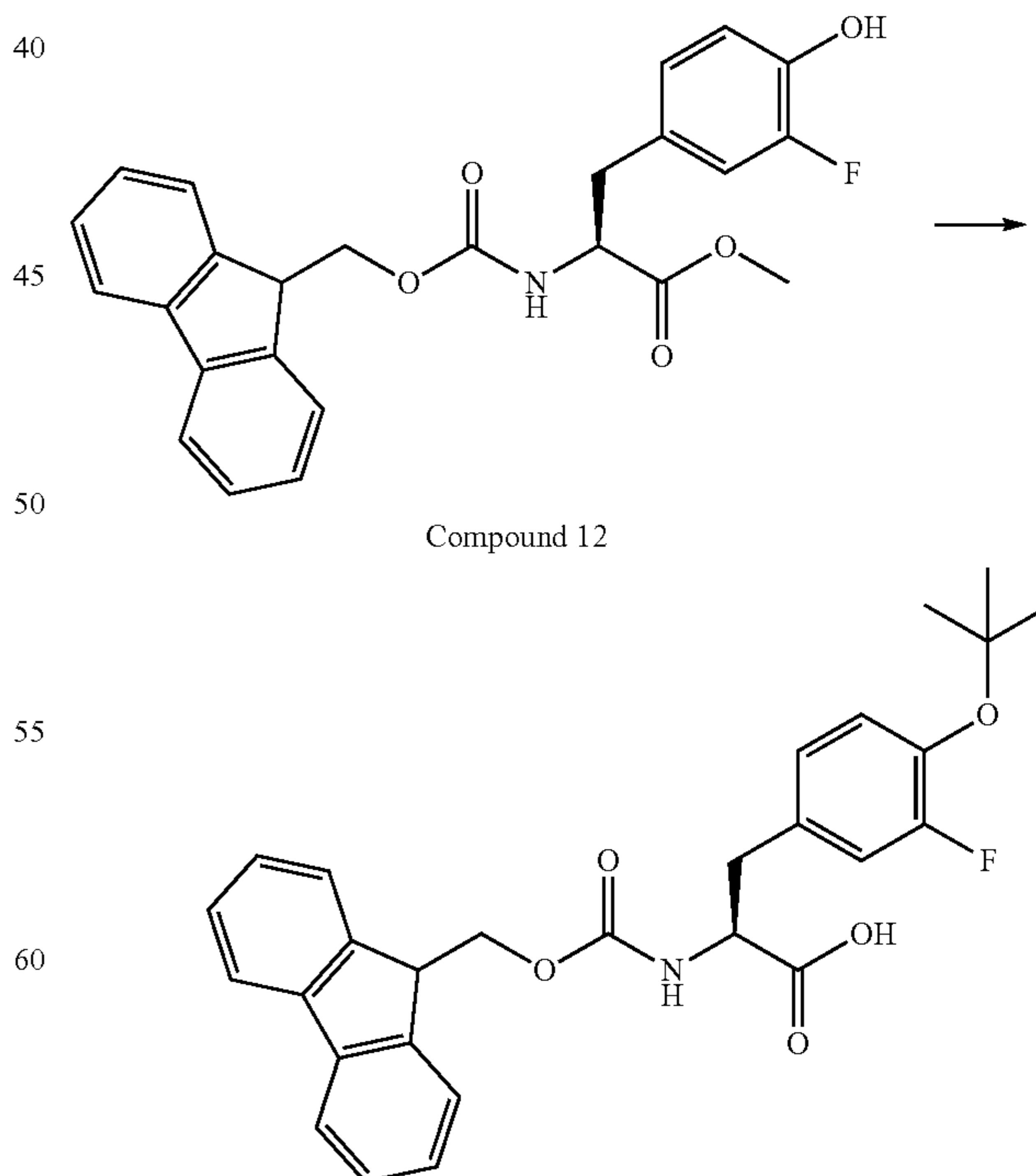
Compound 13
