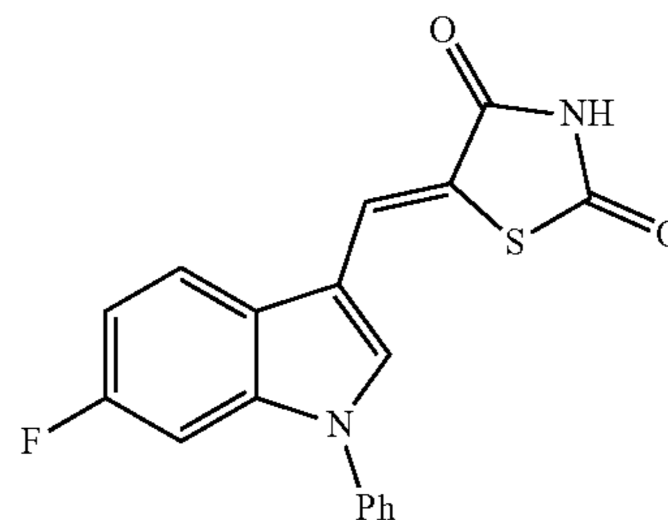
(Z)-5-((6-Fluoro-1-phenyl-1H-indol-3-yl)methylene)thiazolidine-2,4-dione (JXL071)
