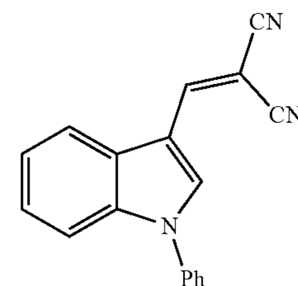
2-((1-Phenyl-1H-indol-3-yl)methylene)malononitrile (JXL021)
