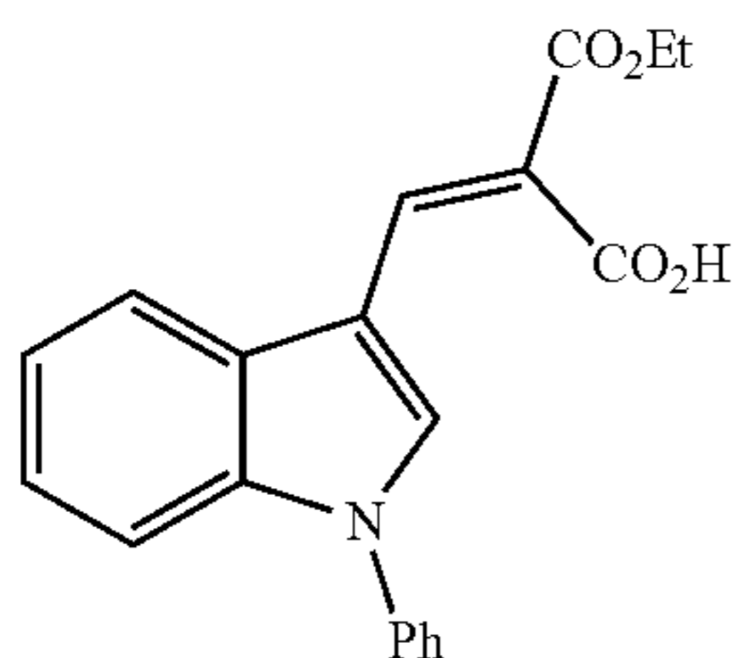
2-(Ethoxycarbonyl)-3-(1-phenyl-1H-indol-3-yl) acrylic Acid (a Mixture of E/Z Isomers, 1:1 Ratio) (JXL025)
