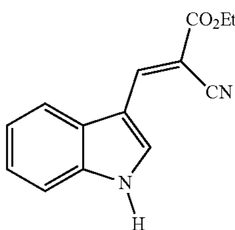
Ethyl (E)-2-cyano-3-(1H-indol-3-yl)acrylate
