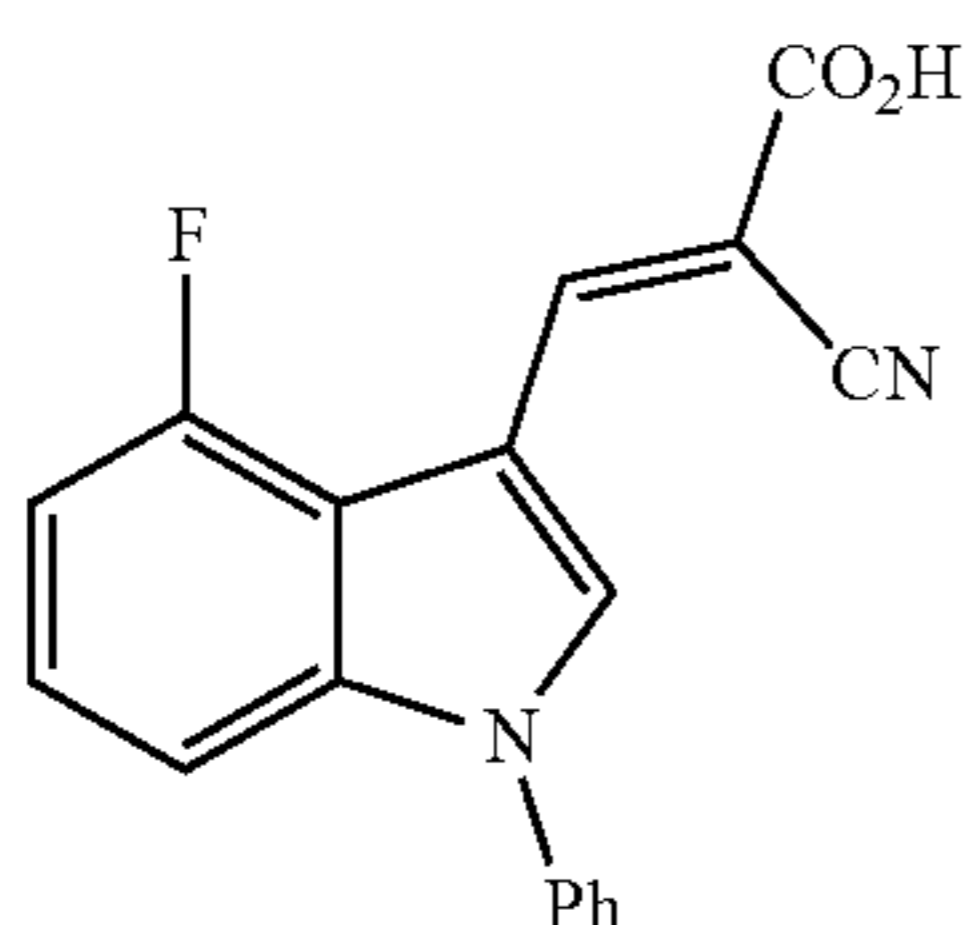
(E)-2-Cyano-3-(4-fluoro-1-phenyl-1H-indol-3-yl) acrylic Acid (JXL026)
