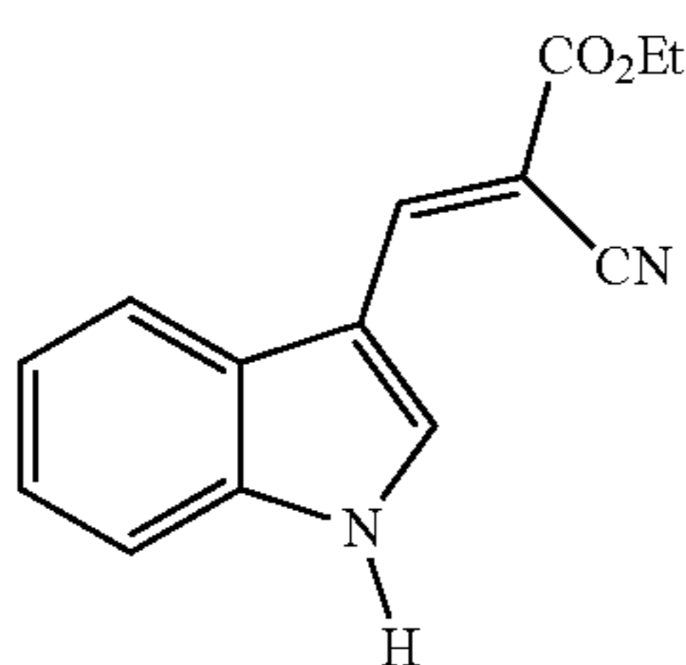
Ethyl (E)-2-cyano-3-(1H-indol-3-yl)acrylate
