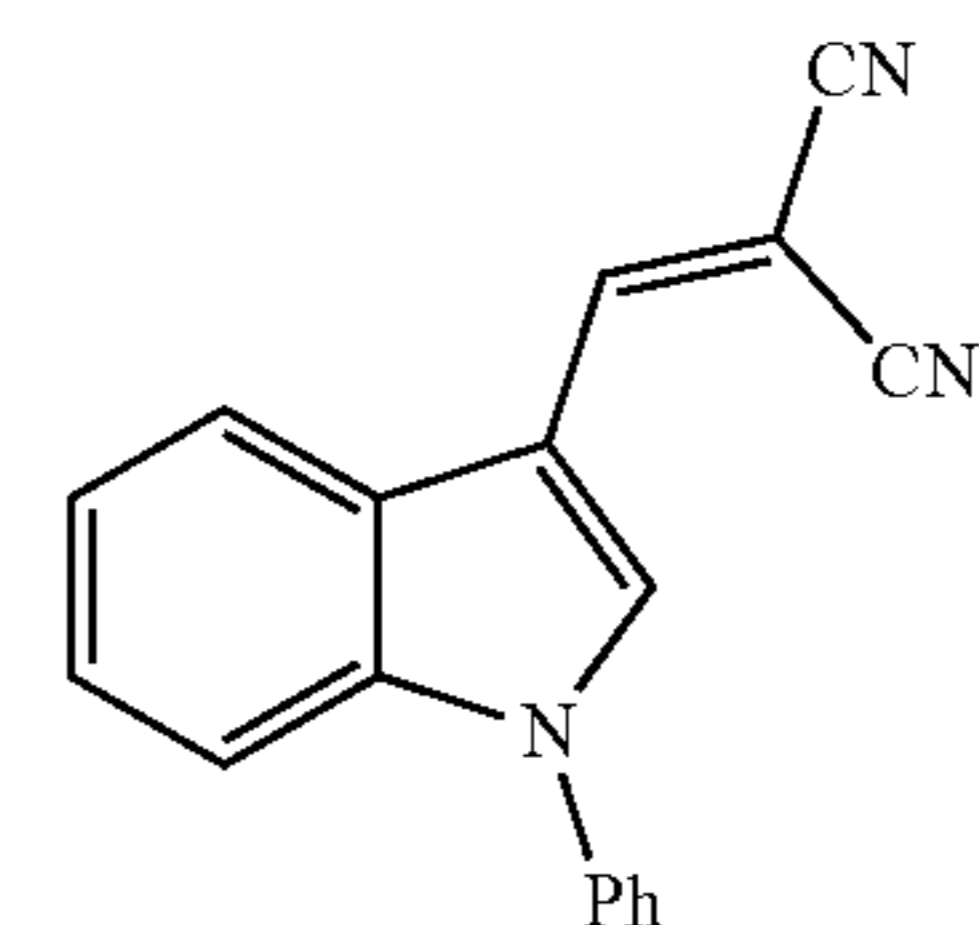
2-((1-Phenyl-1H-indol-3-yl)methylene)malononitrile (JXL021)
