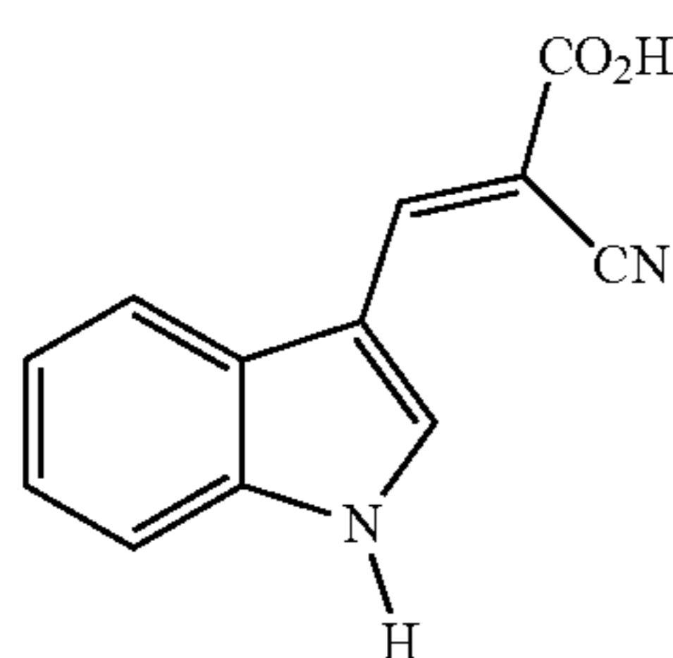
(E)-2-Cyano-3-(1H-indol-3-yl)acrylic Acid (JXL002)
