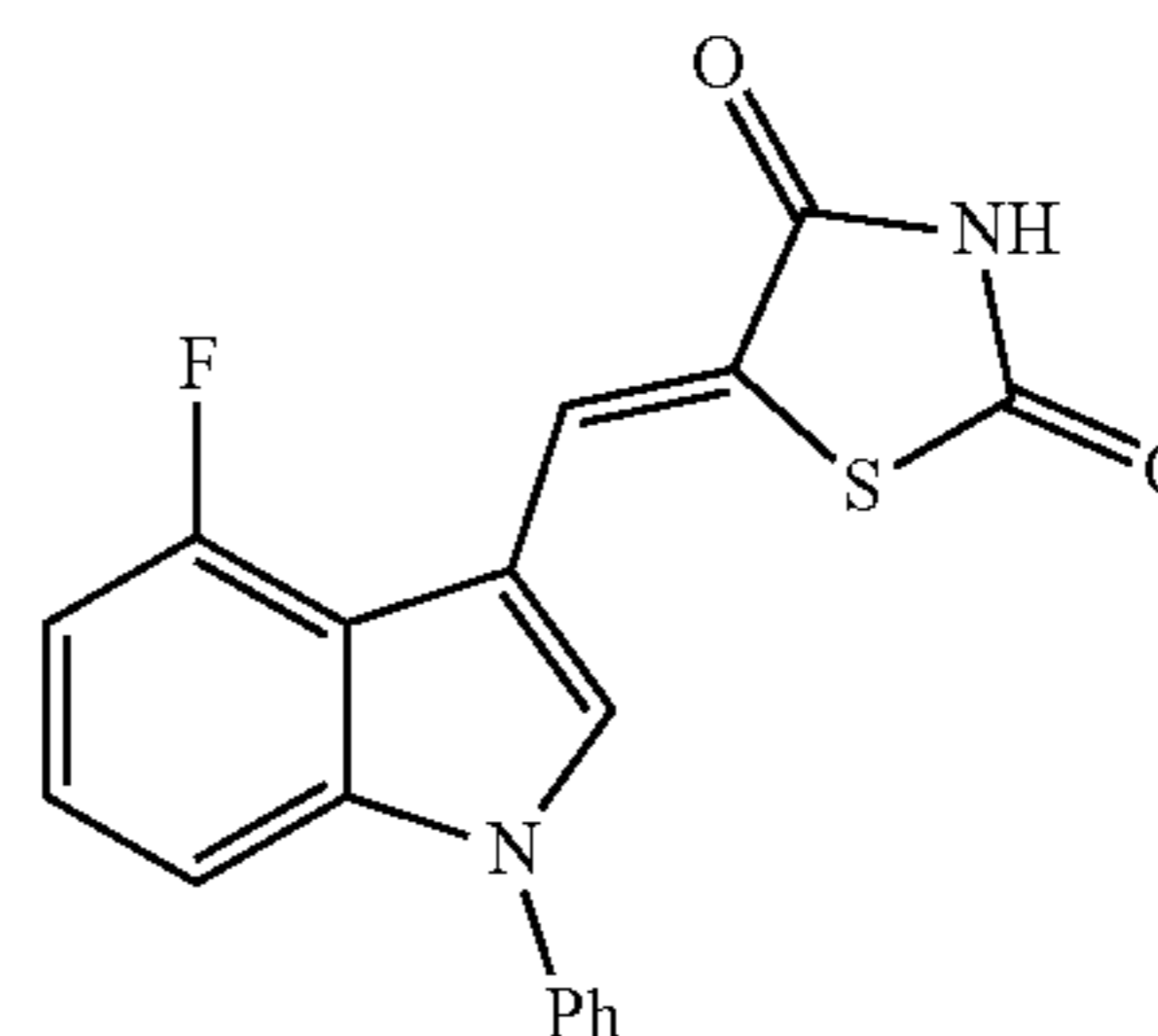
(Z)-5-((4-Fluoro-1-phenyl-1H-indol-3-yl)methylene)thiazolidine-2,4-dione (JXL070)
