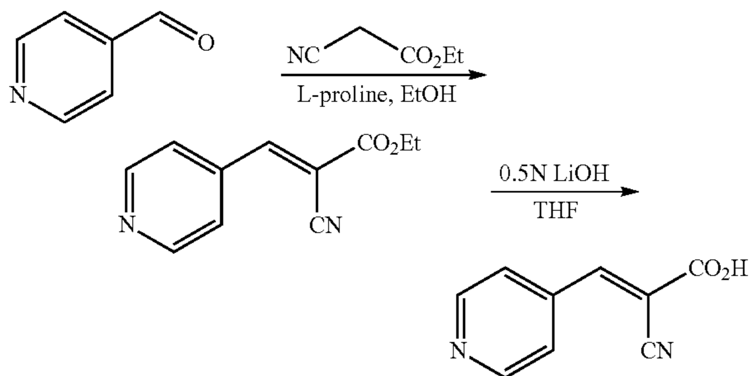
JXL022
