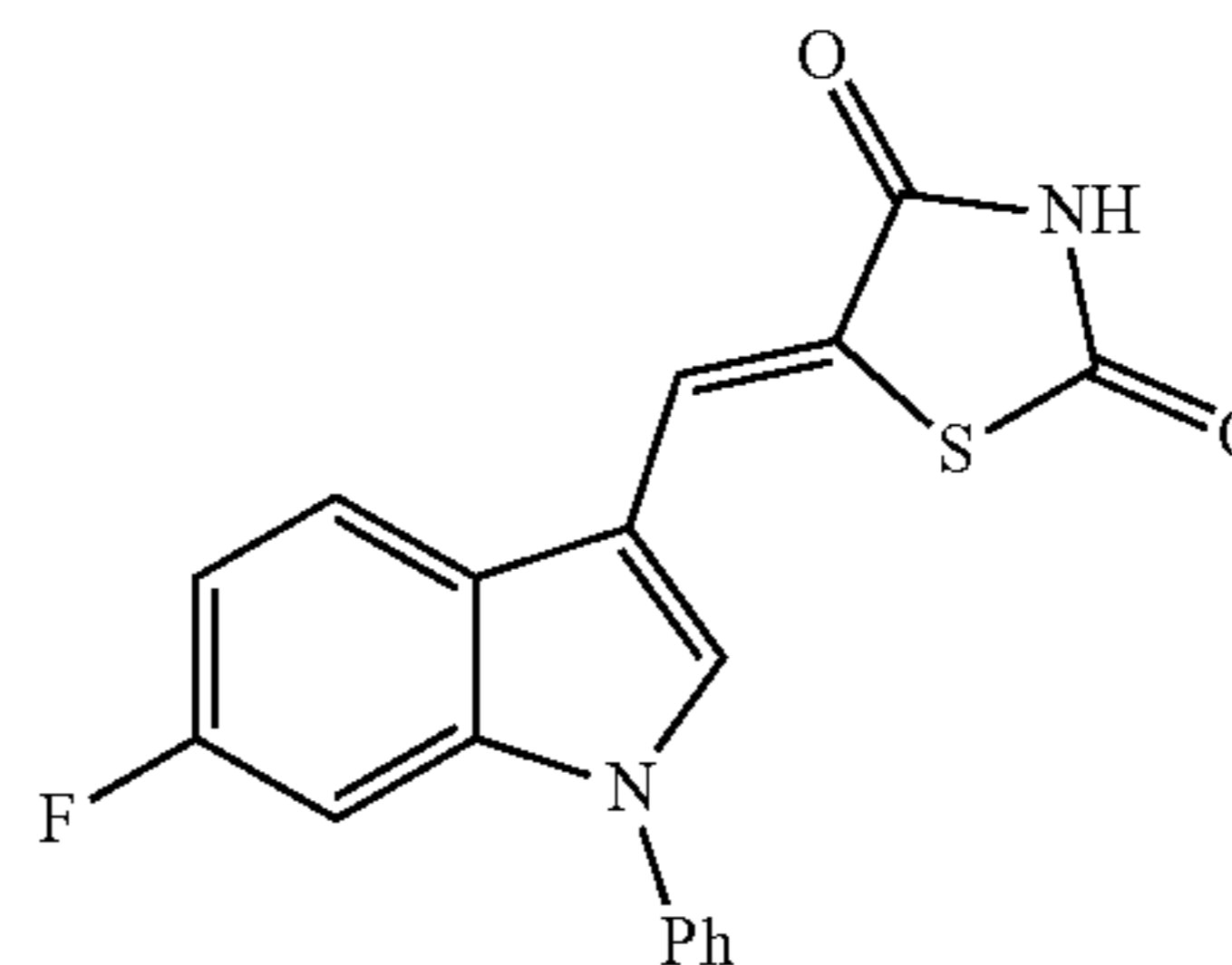
(Z)-5-((6-Fluoro-1-phenyl-1H-indol-3-yl)methylene)thiazolidine-2,4-dione (JXL071)
