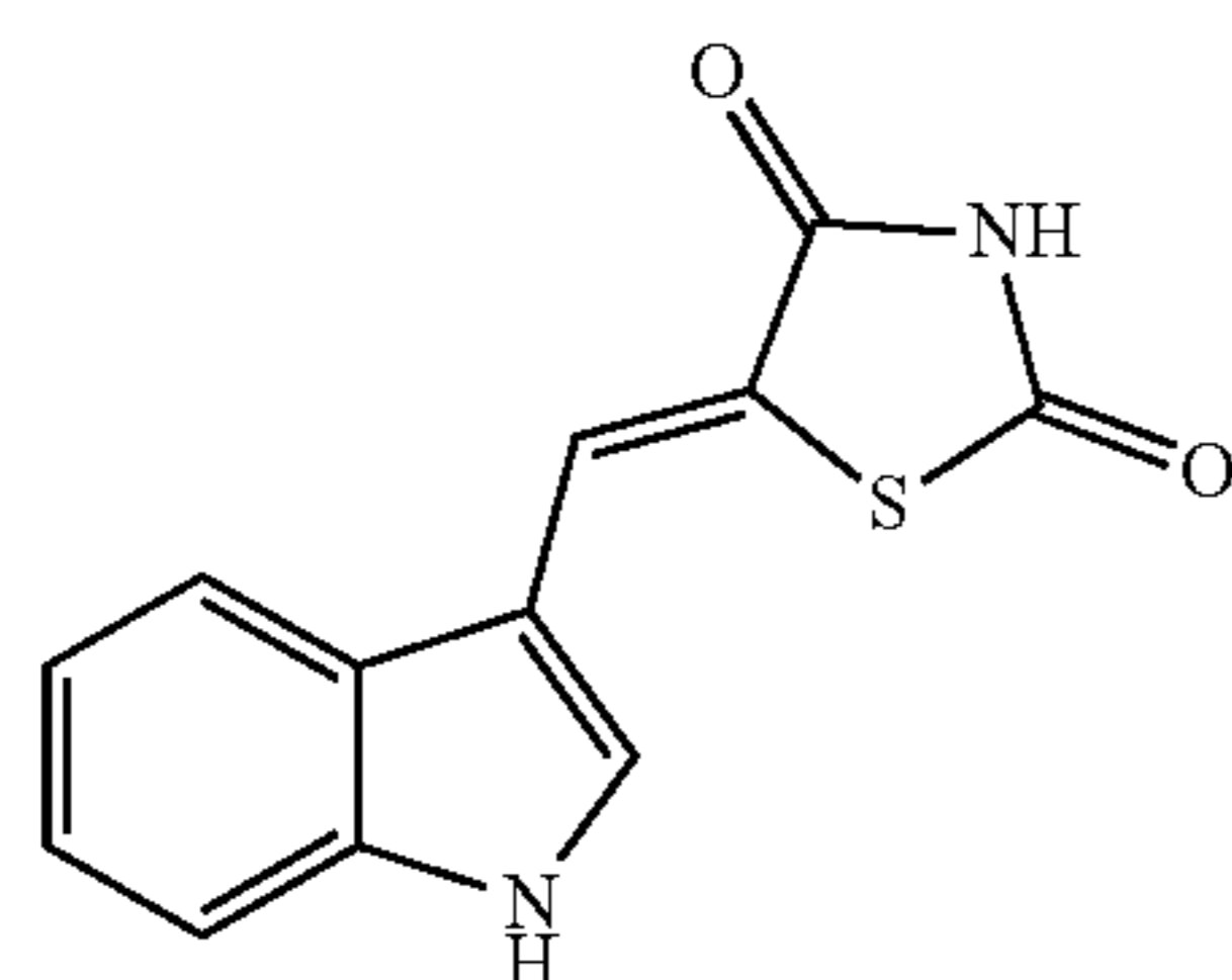
(Z)-5-((1H-Indol-3-yl)methylene)thiazolidine-2,4-dione (JXL075)
